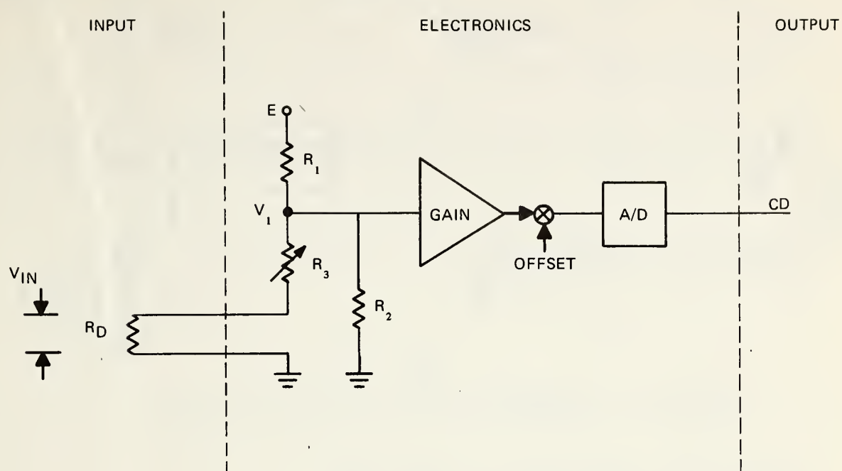
Figure 3-4.--Representation of buoy dewpoint sensor.
