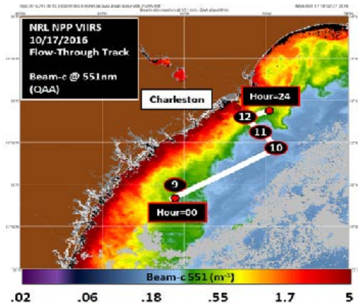
Figure 12. NPP VIIRS image for 17 October 2016 of beam-c showing the flow-through track for a 24 hour period along with the station locations and station numbers (black ovals) for that day.
