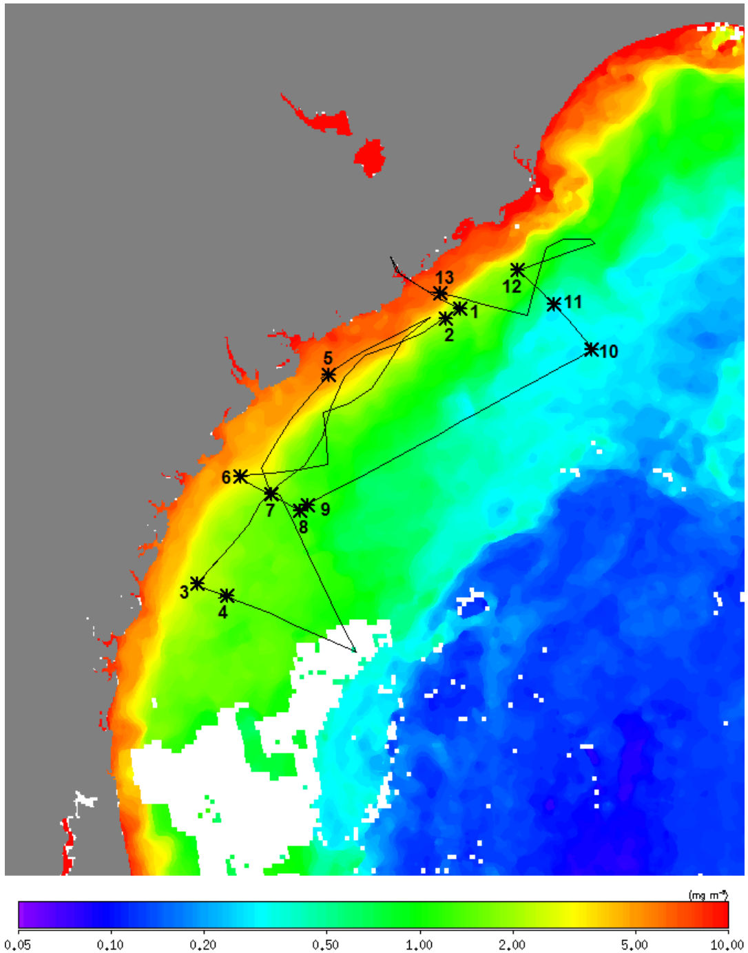
Figure 3. Cruise track and station locations overlaid onto an image of VIIRS MSL12 Science Quality Chl- a merged data covering the period 12 October 2017 to 19 October 2017. Units for colorbar are \text{mg m}^{-3} .
