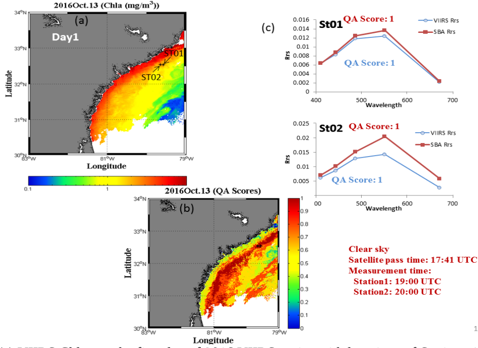
Figure 28. (a) VIIRS Chl- a on the first day of 2016 VIIRS cruise with locations of Stations 1 and 2 marked; (b) QA score images for the same day generated following the method developed by Wei et al. [2016]; (c) RISBA R_{rs} and match-up VIIRS level 2 R_{rs} . R_{rs} is shown in units of \text{sr}^{-1} .
