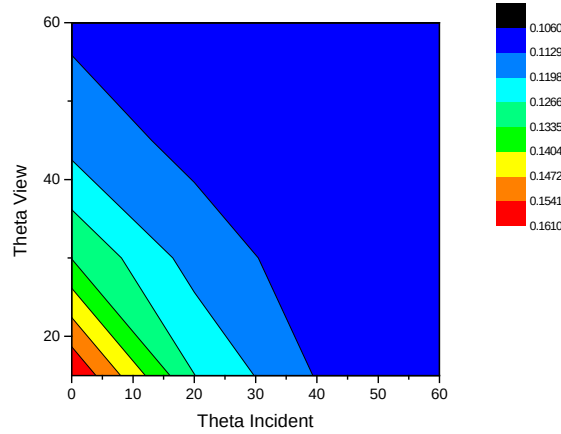
Figure 26. Blue tile bi-directional reflectance factor dependence on incident and reflected zenith angles at 90^\circ to the plane of incidence and at 410 nm.
