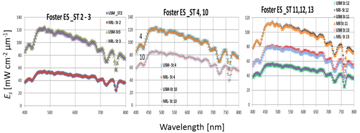
Figure 10. Preliminary results for multiple E_s sensors at several stations showing good agreement.
