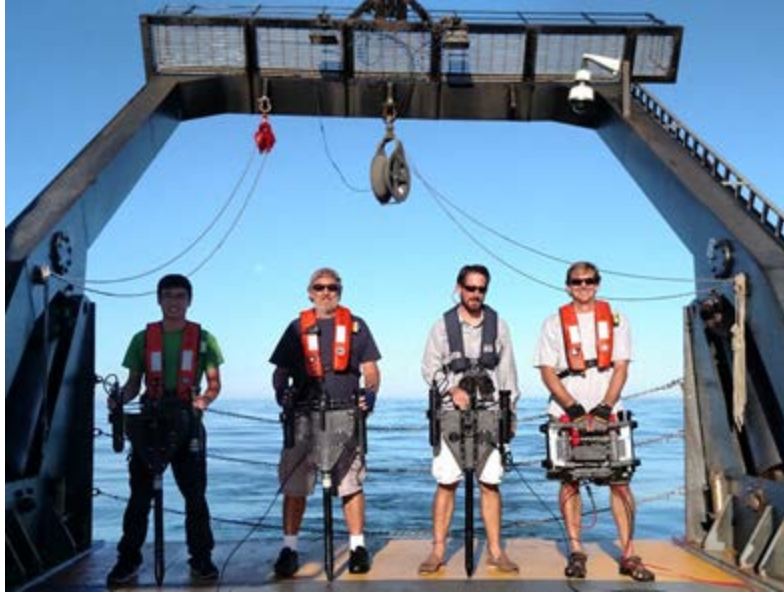
Figure 6. Four profiling radiometers were deployed simultaneously from the stern. The 3 HyperPro instruments are pictured on the left. The C-OPS is on the right.
