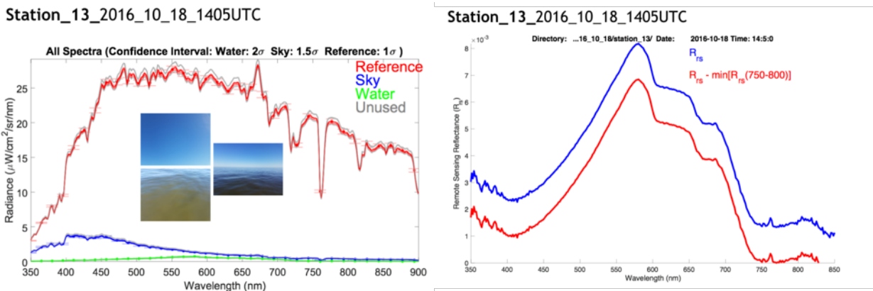
Figure 33. (Left) Initial screen display for automated processing software to compute R_{rs} for the Spectral Evolution spectrometer. The red line is the reference 99% reflectance plaque, the blue line is sky L_{sky} , the green line is L_w . The gray line are spectra that fall outside a 2 sigma variance window and are not used in final calculations. (Right) Station 13 computed R_{rs} after automated removal of outliers (blue line) and after adjusting the baseline at 750 nm to 0 (red line).
