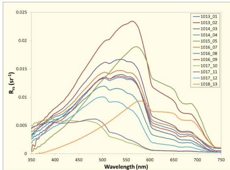
Figure 22. Preliminary R_{rs}(\lambda) estimates from shipboard (above-water) remote sensing reflectance measurements made at 12 stations on NF-16-08.
