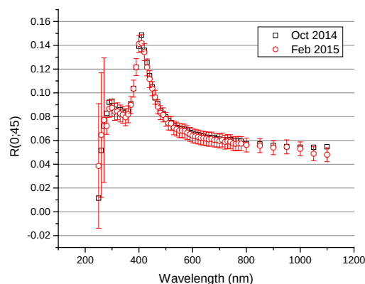
Figure 25. NIST STARR bi-directional reflectance values for the blue glass assembly.
