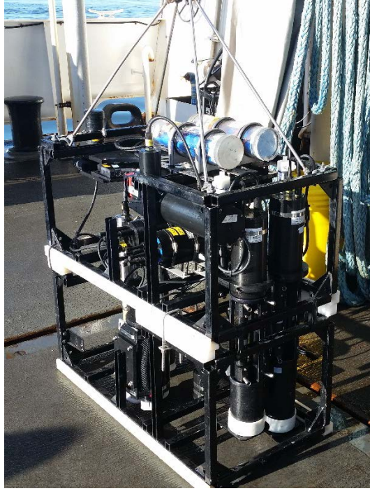
Figure 38. HBOI in situ IOP instrument package.
