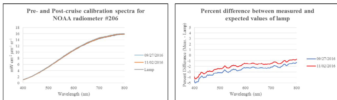
Figure 5. Example of the pre- and post-cruise calibration results for the NOAA/STAR L_u 206 radiance sensor (left) along with expected values for the lamp and (right) the percent difference between the expected lamp values and those measured by the radiometers.
