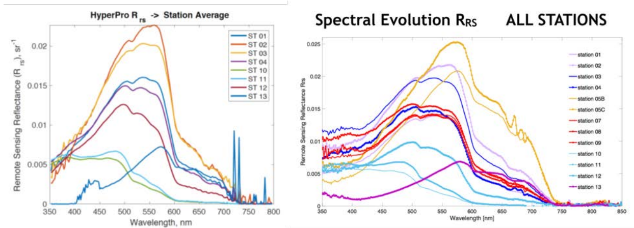
Figure 34. R_{rs} spectra from all stations (left) collected with HyperPro and (right) collected with Spectral Evolution. Stations 10 and 11 show relatively clear open water about 80 km east of Charleston.
