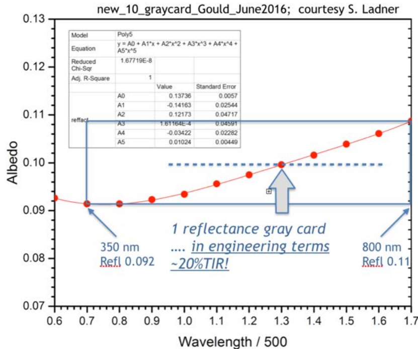
Figure 37. Measurement of NRL gray plaque across full bandwidth shows wavelength dependence in reflectance. Albedo is the dimensionless ratio of reflectance from a black body (=0) to a white body (=1).
