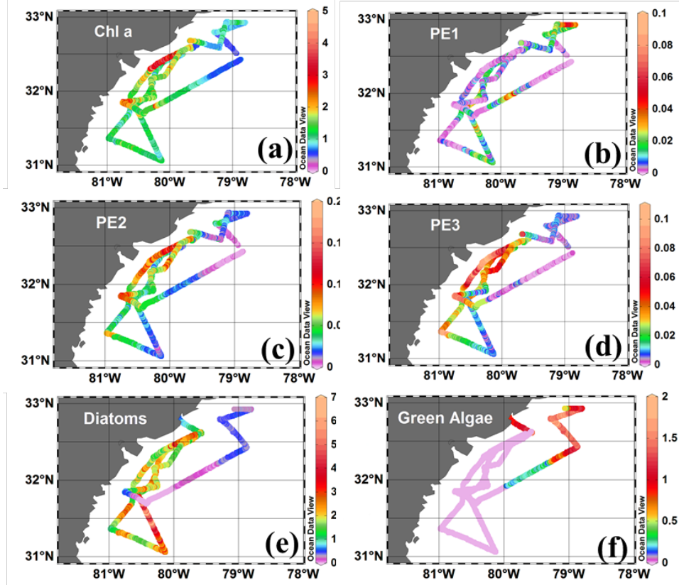
Figure 20. Distribution along the cruise track of parameters all in relative fluorescence units: (a) Chl- a ; (b) PE1, open ocean cyanobacteria; (c) PE2, coastal water cyanobacteria; (d) PE3, cryptophytes; (e) diatoms and (f) green algae.
