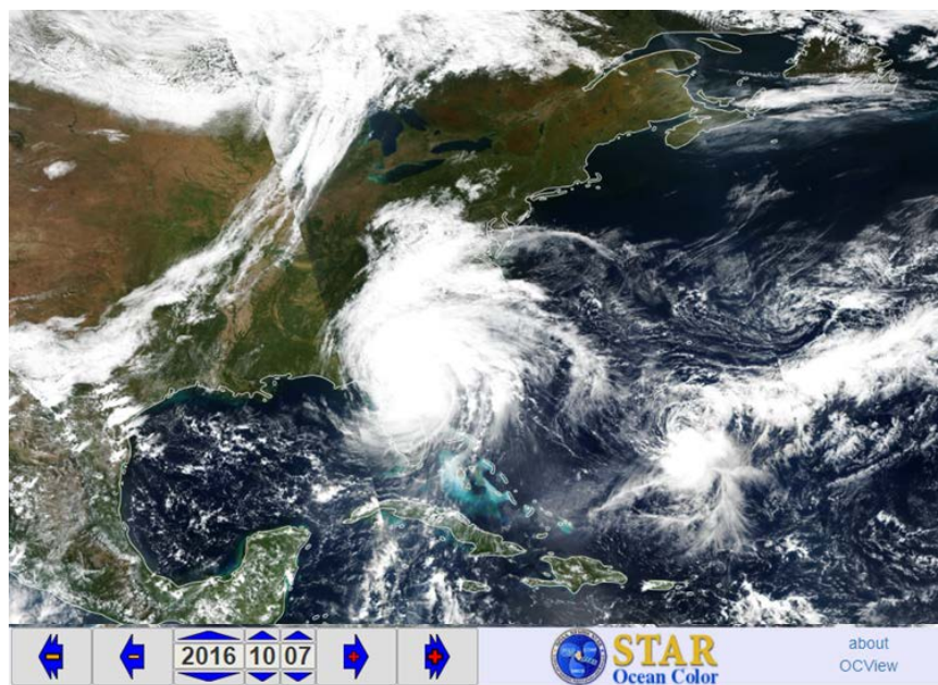
Figure 1. VIIRS SNPP true color image taken from NOAA/STAR Ocean Color OCView monitoring tool 7 October showing the approach of Hurricane Matthew toward the Charleston, SC area.
