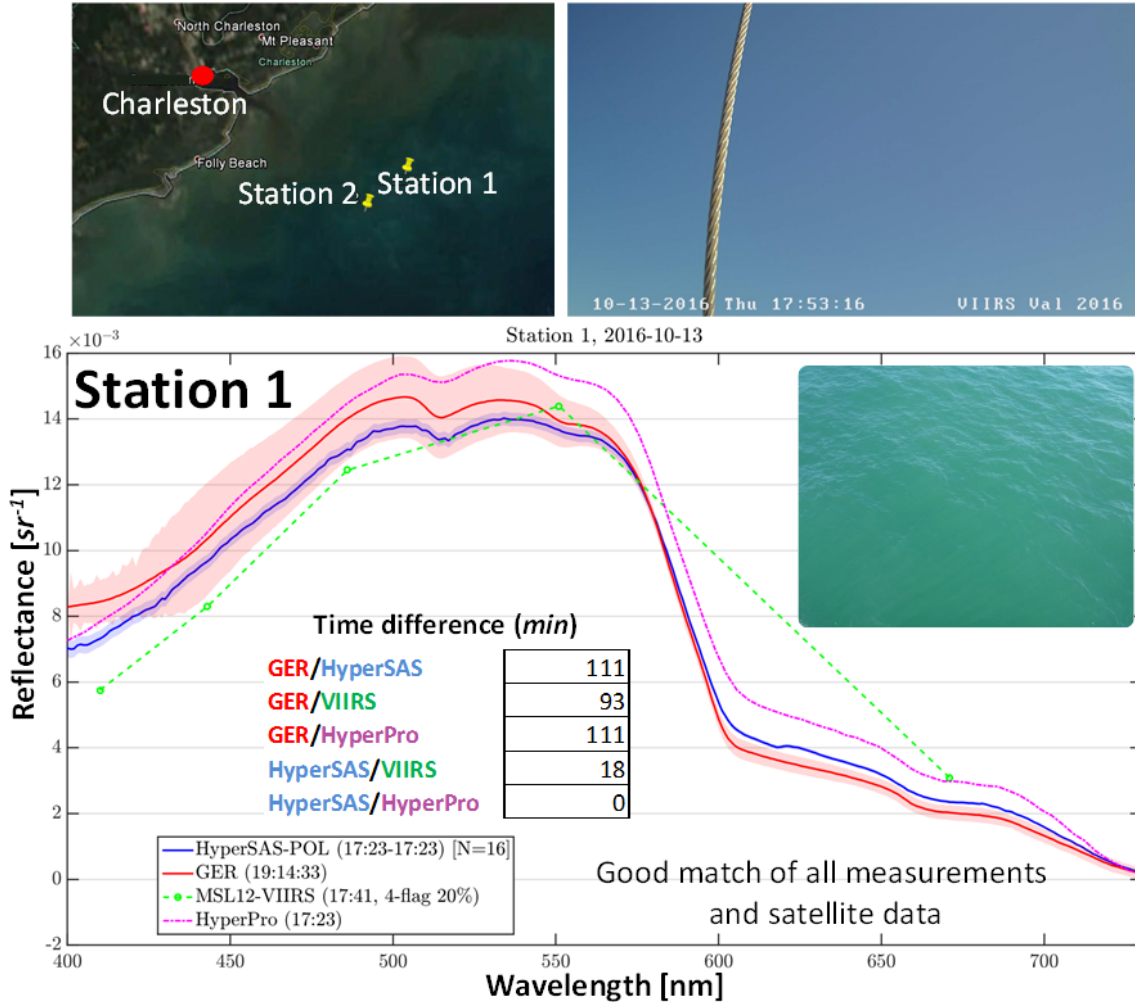
Figure 16. Station 1, coastal waters comparisons. Measured spectra by GER, HyperSAS-POL and HyperPro instruments are shown in comparison with VIIRS data. The top panel contains (top left): True
