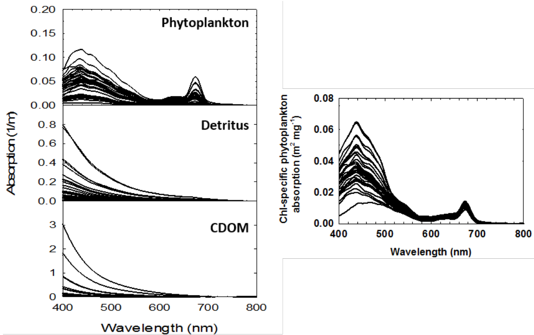
Figure 21. The measured a_p , a_d and a_{CDOM} spectra of water samples collected on this cruise. The figure to the right is the a^*_{ph} spectra derived from the water sample measurements.
