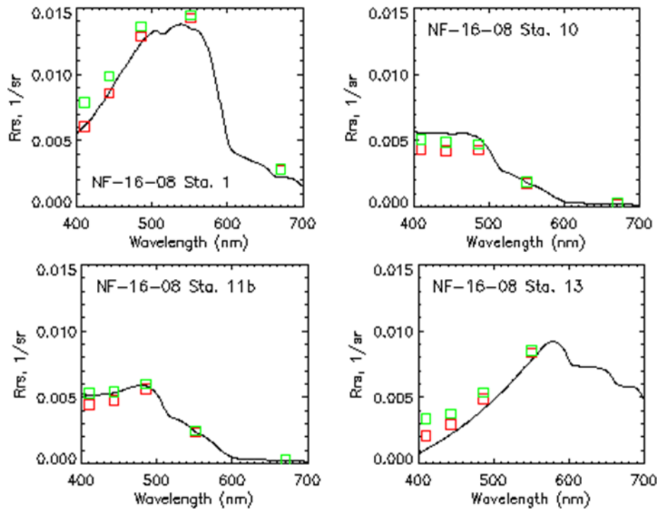
Figure 23. Comparisons between field R_{rs}(\lambda) (solid line) and VIIRS R_{rs}(\lambda) processed before (red squares) and after (green squares) the MSL12 routine was updated and the VIIRS SDR was improved in early 2017. These improvements included correction of the blue-band polarization effects.
