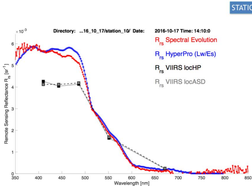
Figure 35. Comparison of in situ and VIIRS R_{rs} spectra at Station 10, clear open ocean 80 km east of Charleston
