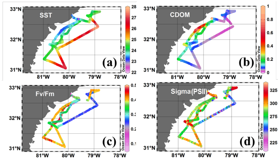
Figure 19. Distribution along cruise track of parameters: (a) SST in units of °C; (b) CDOM in relative fluorescence units; and photo-physiological properties of phytoplankton (c) F_v/F_m , a dimensionless ratio, the colorbar range is 0 to 0.5; and (d) \sigma_{PSII} in units of 0.1 \text{ nm}^2 \text{ quanta}^{-1} .
