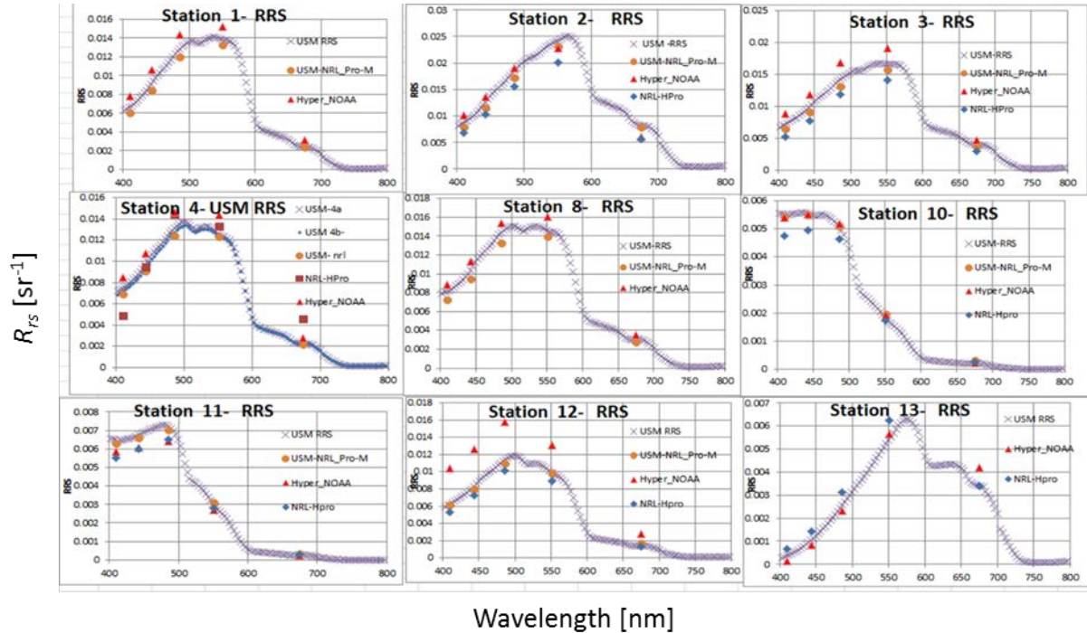
Figure 11. Preliminary comparisons of R_{rs} measured by Stennis floating HyperPro radiometers showing good agreement.
