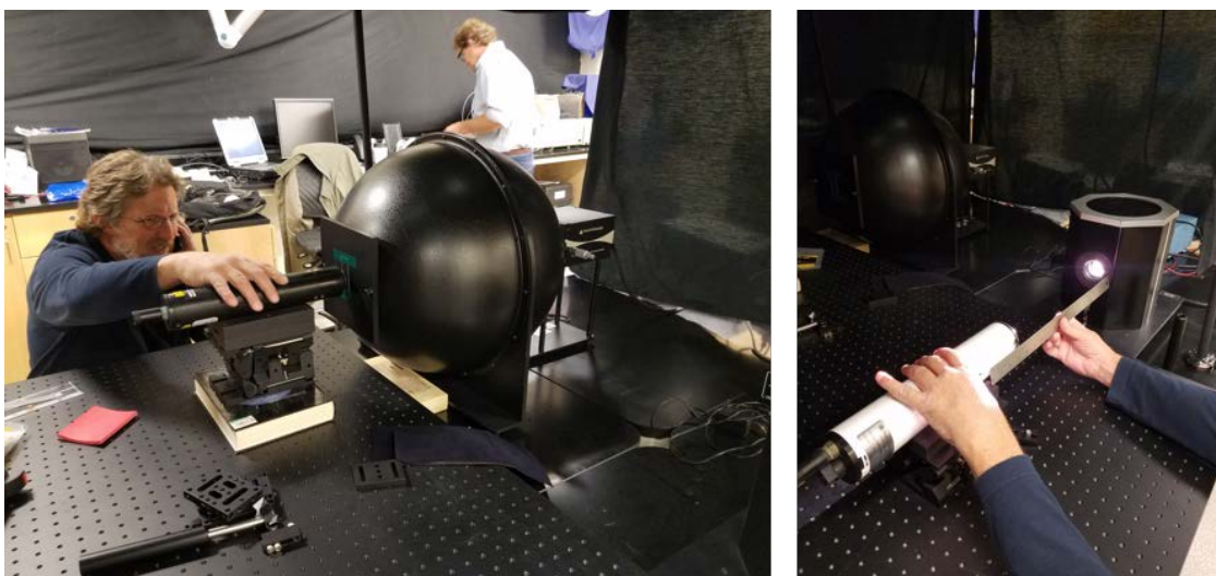
Figure 4. Calibration activities at the NOAA/STAR optical laboratory.
