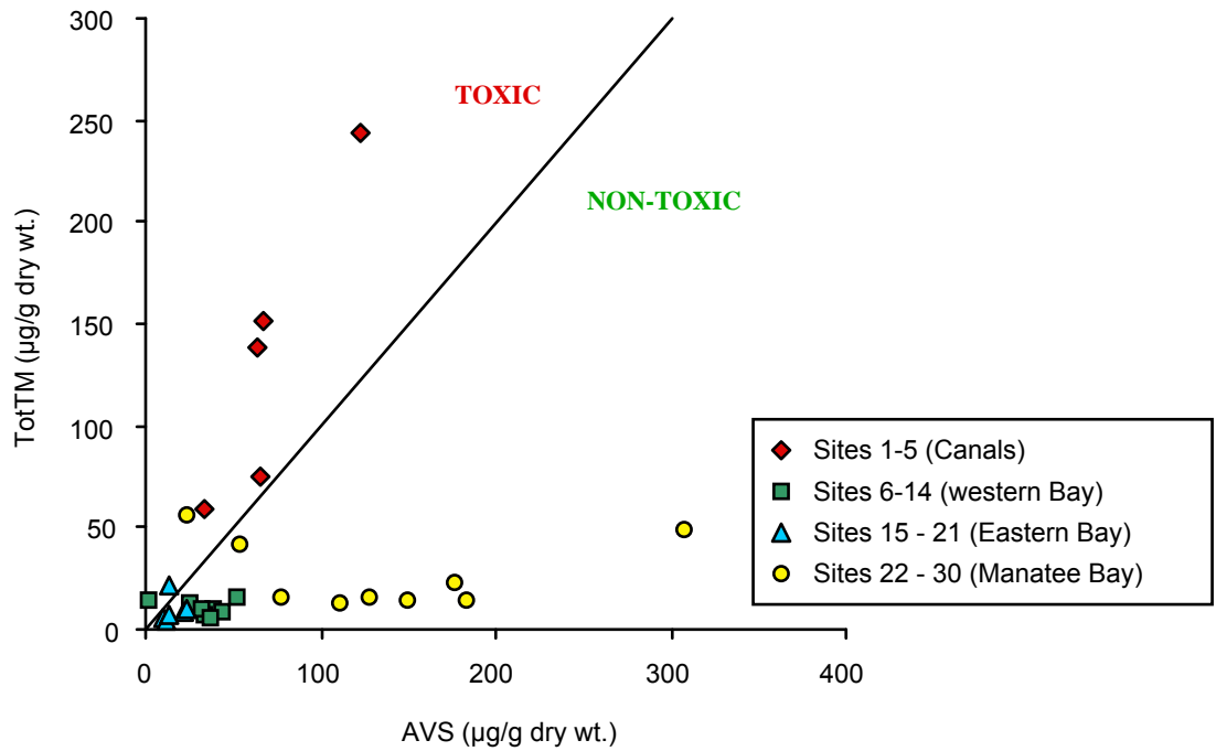
Figure 4. Sum of the concentrations of trace metals (TotTM = [Cu] + [Zn] + [Ni] + [Pb] + [Cd] + [Hg] + [Ag]) versus AVS concentration (µg/g dry wt.).
