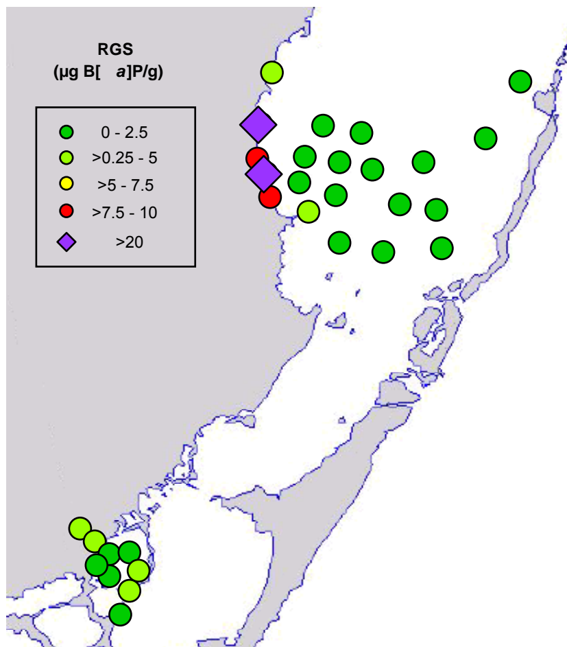
Figure 10. Distribution of HRGS P450 in benzo[a]pyrene equivalent units in Biscayne Bay sediments ( \mu\text{g B[a]PEq/g} ).
