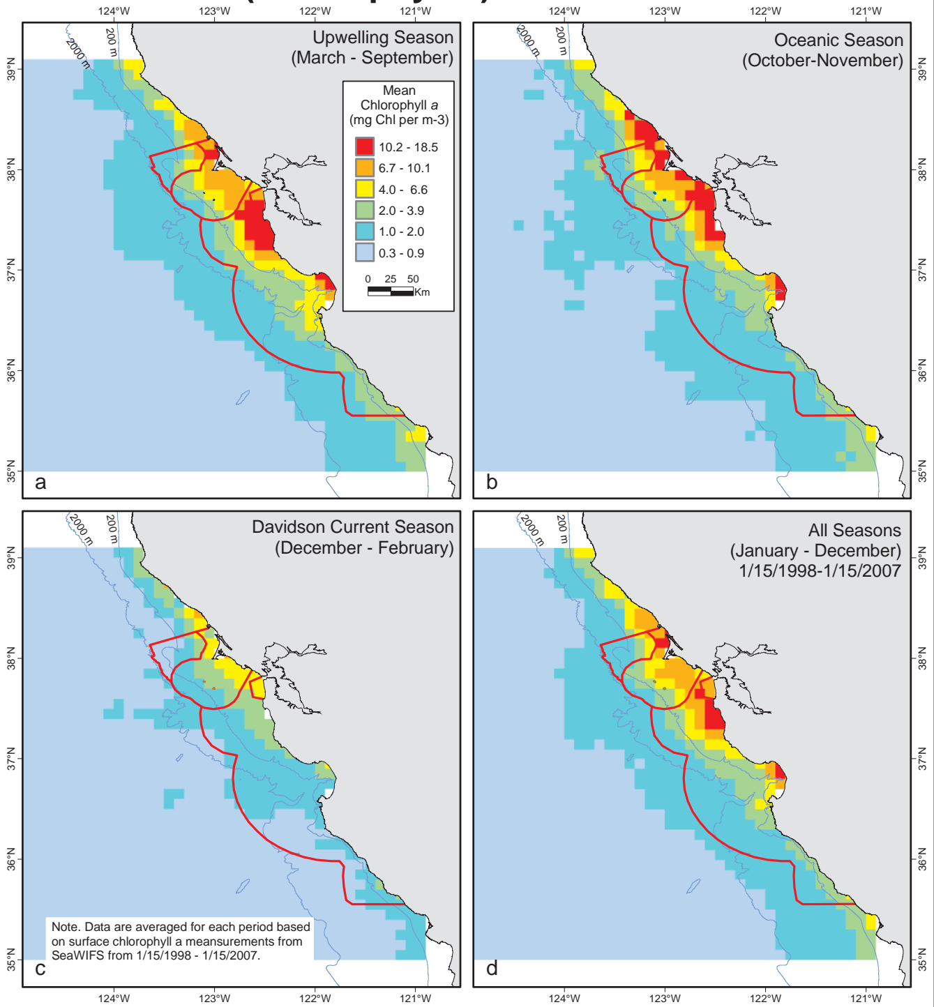
Map Citation: NOAA National Centers for Coastal Ocean Science (NCCOS) 2007. Data from the SeaWiFS sensor on the Orbview-2 satellite, provided by NASA/Goddard Space Flight Center and GeoEye, Inc. Regional analysis provided by NOAA CoastWatch, West Coast Node.
