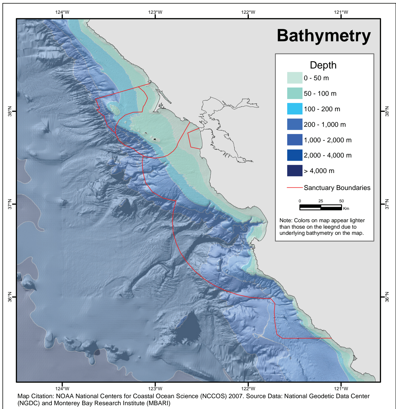
Figure 2.2. Bathymetry and depth zones of the study area.
