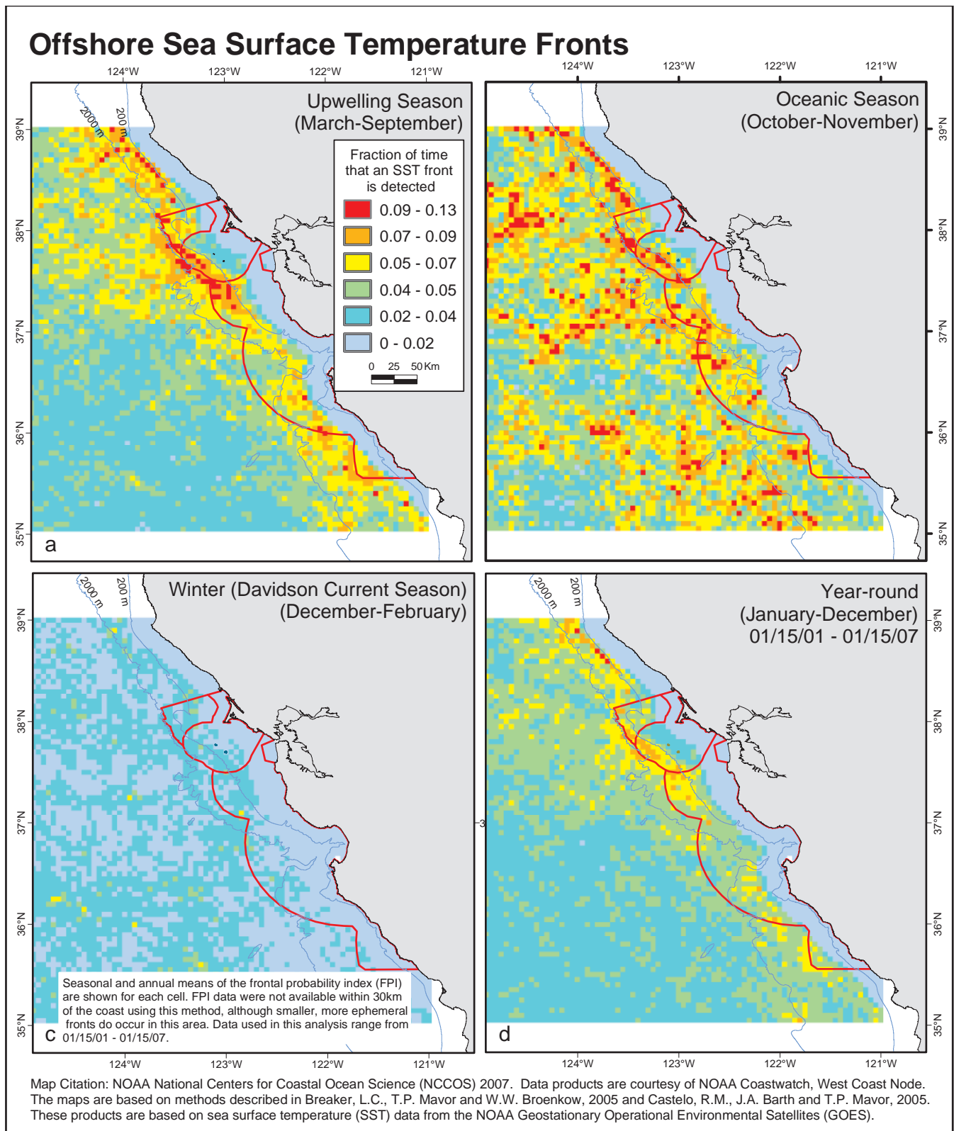
Figure 2.13. Offshore sea surface temperature fronts, by ocean season and year-round.
