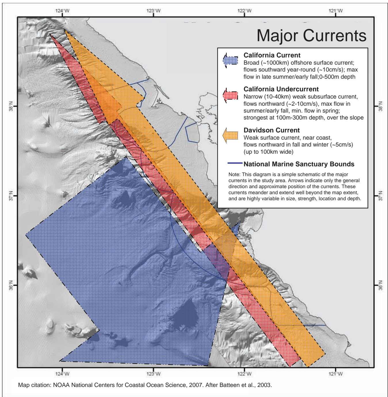
Figure 2.11. A schematic of two major surface currents and a subsurface current in the study area.
