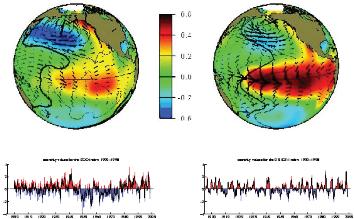
Figure 2.10. Comparing sea surface temperatures during a warm phase of the Pacific Decadal Oscillation and the El Niño Southern Oscillation. Figures provided courtesy of Nathan Mantua, University of Washington Climate Impacts Group, and Steven Hare, International Pacific Halibut Commission.
