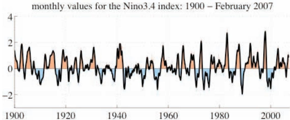
Figure 2.7. Tracking El Niño's and La Niña's in the North Pacific – red is warm and represents an El Niño, blue is cool and represents a La Niña. 1998 was a strong El Niño year. Figure provided courtesy of Nathan Mantua, University of Washington Climate Impacts Group, and Steven Hare, International Pacific Halibut Commission.
