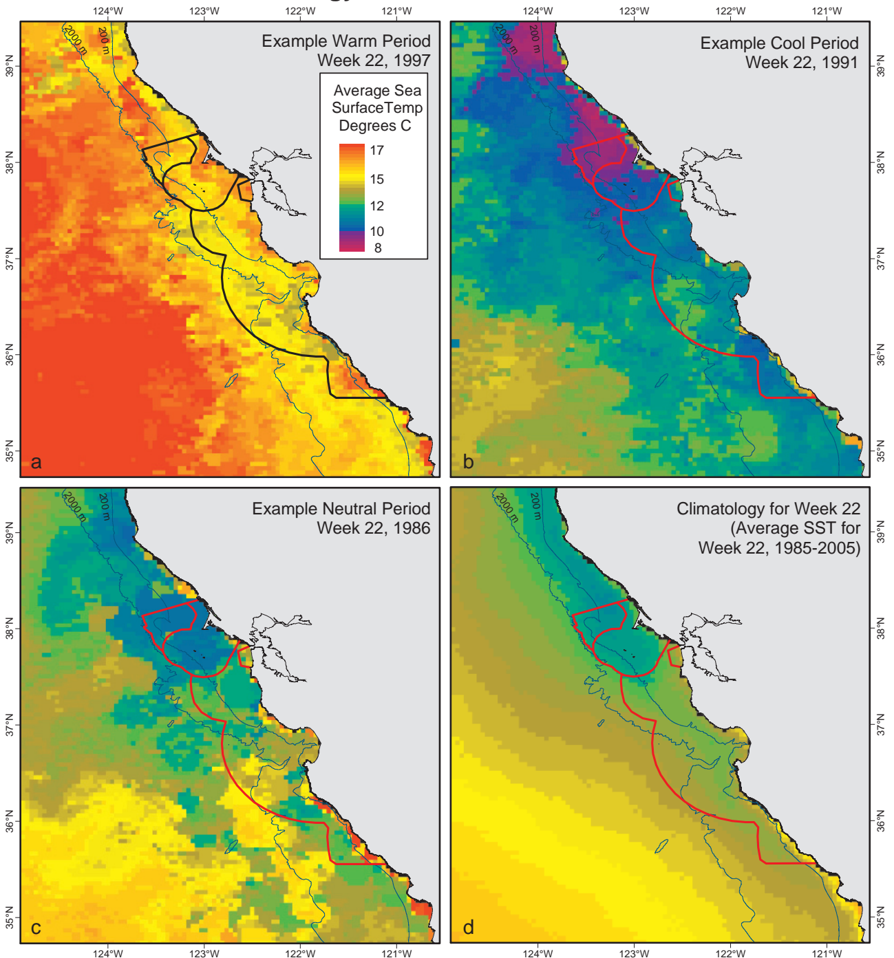
Map Citation: NOAA National Centers for Coastal Ocean Science (NCCOS) 2007. Data Source: Ken Casey and Varis Ransi, both from NOAA, provided the Pathfinder Version 5.0 data set, derived from Advanced Very High Resolution Radiometer (AVHRR) data from NOAA polar-orbiting satellites, from NOAA's National Oceanographic Data Center ( http://pathfinder.nodc.noaa.gov ).
