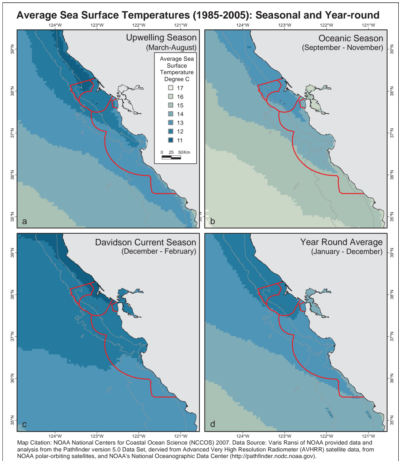
Figure 2.6. Average sea surface temperature (1985-2005): by ocean season and year-round average.
