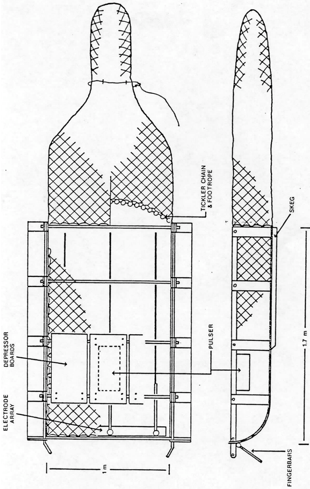
Figure 1. Electrified shrimp trawl.
