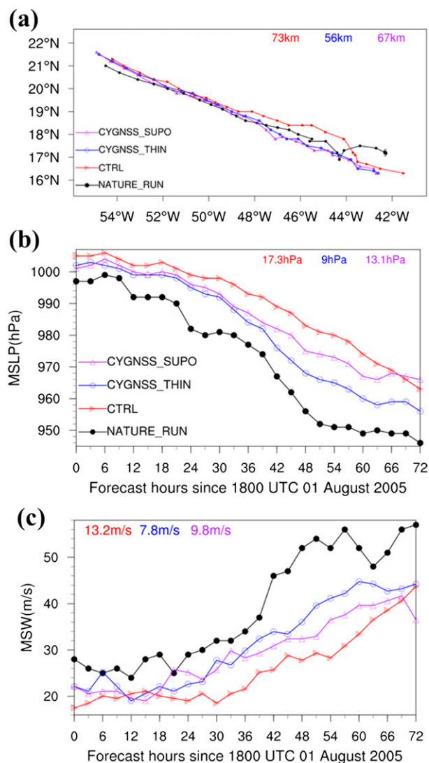
FIG. 2. Time series of (a) track, (b) MSLP, and (c) maximum surface wind between 1800 UTC 1 Aug 2005 and 1800 UTC 4 Aug 2005 from CTRL (red) and CYGNSS (SUPO in pink and THIN in blue) data assimilation experiments compared against the hurricane NR (black). The colored numbers at the top of (a) denote the averaged track errors during the first 36-h forecast and those in (b), (c) represent the averaged absolute intensity errors during the whole simulation period (72 h) for the experiments corresponding to the same colored lines.
