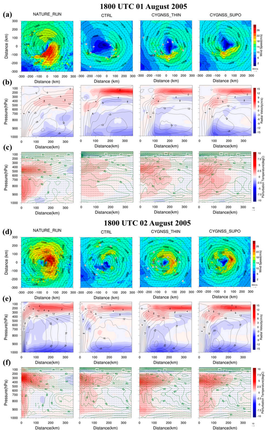
FIG. 3. Comparison of the structure of the hurricane vortices from (left to right) the hurricane NR vs the CTRL, CYGNSS_THIN, and CYGNSS_SUPO at (a)–(c) 1800 UTC 1 Aug 2005 and (d)–(f) 1800 UTC 2 Aug 2005. (a),(d) Sea level pressure (hPa, black contour), 10-m wind field ( m s^{-1} , black vectors with reference vector below color bar), and wind speed ( m s^{-1} , color shaded contours). (b), (e) Vertical cross section of azimuthally averaged tangential wind ( m s^{-1} , black contours) and radial wind ( m s^{-1} , color shaded contours). (c),(f) Vertical cross section of azimuthally averaged temperature perturbations ( ^{\circ}C , color shading), relative humidity (%), and secondary circulations [represented by u-w vectors, where u is the radial velocity ( m s^{-1} ) and w is the vertical velocity ( cm s^{-1} )] with the vector magnitude legend below the color bar.
