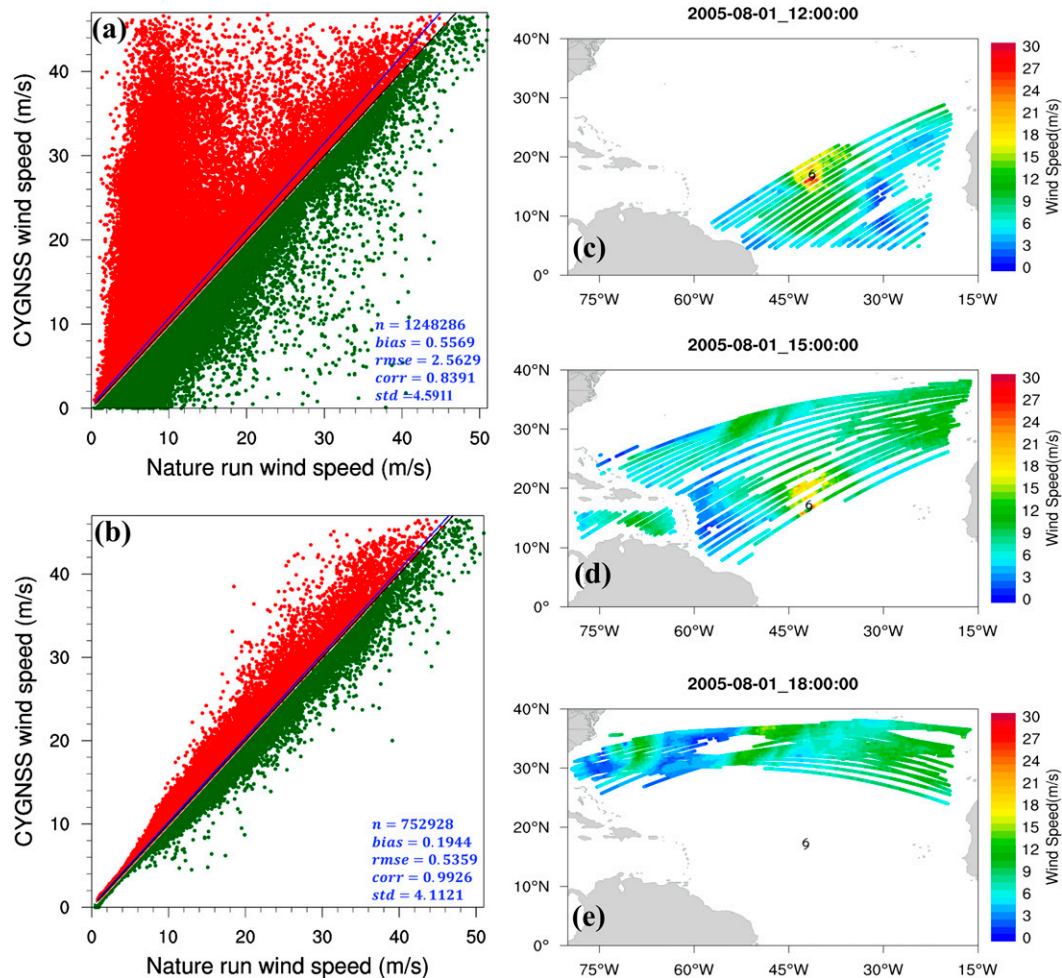
FIG. 1. (a),(b) Scatterplots of CYGNSS wind speed vs hurricane NR wind speed (a) before and (b) after quality control; red (green) dots indicate that CYGNSS wind speed has a positive (negative) observational error. All the data available during 0000 UTC 1 to 0000 UTC 11 Aug 2005 are counted. (c)–(e) CYGNSS data distribution and corresponding wind speeds at (c) 1200, (d) 1500, and (e) 1800 UTC 1 Aug 2005; the small black tropical cyclone symbols denote the storm center location.
