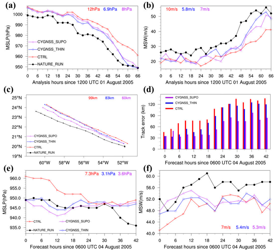
FIG. 5. Time series of (a) MSLP and (b) maximum surface wind between 1200 UTC 1 and 0600 UTC 4 Aug 2005 for the analysis during the cycled DA period: CTRL (red) and CYGNSS (SUPO pink and THIN blue) DA experiments vs the hurricane NR (black). (c)–(f) As in (a),(b), but for track, track errors, MSLP, and maximum surface wind, respectively, for the forecasts between 0600 UTC 4 and 0000 UTC 6 Aug 2005. The colored numbers in each panel denote the averaged absolute errors for track or intensity over the whole period of analysis or simulation for the experiments corresponding to the line colors.
