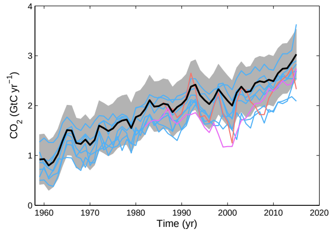
Figure 7. Comparison of the anthropogenic atmosphere–ocean \text{CO}_2 flux showing the budget values of S_{\text{OCEAN}} (black; with \pm 1\sigma uncertainty in grey shading), individual ocean models before normalisation (blue), and the two ocean data-based products (Rödenbeck et al. (2014) in salmon and Landschützer et al. (2015) in purple; see Table 6). Both data-based products were adjusted for the pre-industrial ocean source of \text{CO}_2 from river input to the ocean, which is not present in the models, by adding a sink of 0.45 \text{ GtC yr}^{-1} (Jacobson et al., 2007), to make them comparable to S_{\text{OCEAN}} . This adjustment does not take into account the anthropogenic contribution to river fluxes (see Sect. 2.7.2).
