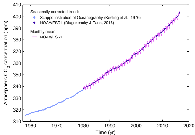
Figure 1. Surface average atmospheric \text{CO}_2 concentration, de-seasonalised (ppm). The 1980–2016 monthly data are from NOAA/ESRL (Dlugokencky and Tans, 2016) and are based on an average of direct atmospheric \text{CO}_2 measurements from multiple stations in the marine boundary layer (Masarie and Tans, 1995). The 1958–1979 monthly data are from the Scripps Institution of Oceanography, based on an average of direct atmospheric \text{CO}_2 measurements from the Mauna Loa and South Pole stations (Keeling et al., 1976). To take into account the difference of mean \text{CO}_2 between the NOAA/ESRL and the Scripps station networks used here, the Scripps surface average (from two stations) was harmonised to match the NOAA/ESRL surface average (from multiple stations) by adding the mean difference of 0.542 ppm, calculated here from overlapping data during 1980–2012. The mean seasonal cycle is also shown from 1980 (in pink).
