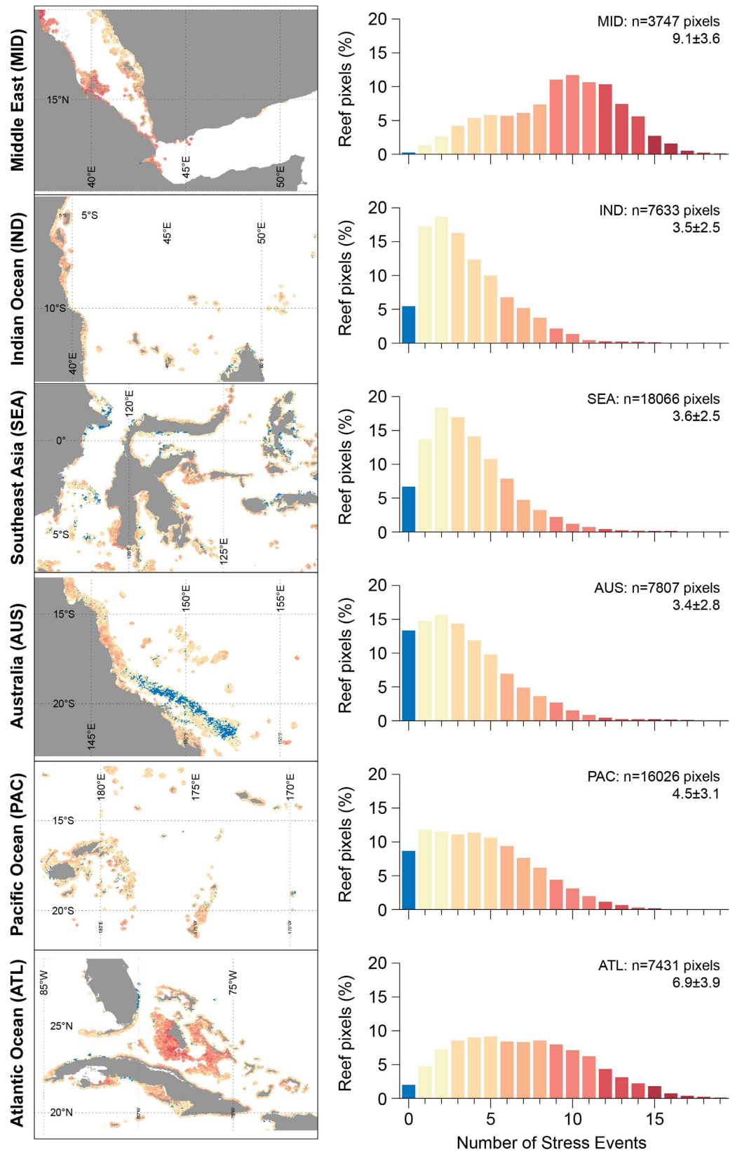
Figure 5. Frequency of bleaching-level thermal stress events among reef regions, 1985–2012. Bleaching-level stress is defined as DHW \geq 4^{\circ}C\text{-weeks} . Maps (left) show results for a subset of each region; histograms (right) show the distribution of results in the full region with the regional average \pm one standard deviation. Reef regions are as per Burke et al. 2011. Data are provided for each histogram in Table S5. Data visualisations produced using IDL [8.3] (Exelis Visual Information Solutions, Boulder, Colorado).
