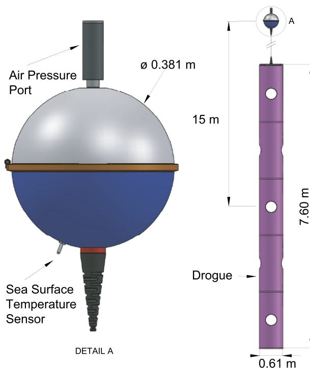
FIG. 1. Schematic of the SVPB drifter manufactured at the Scripps Institution of Oceanography.
