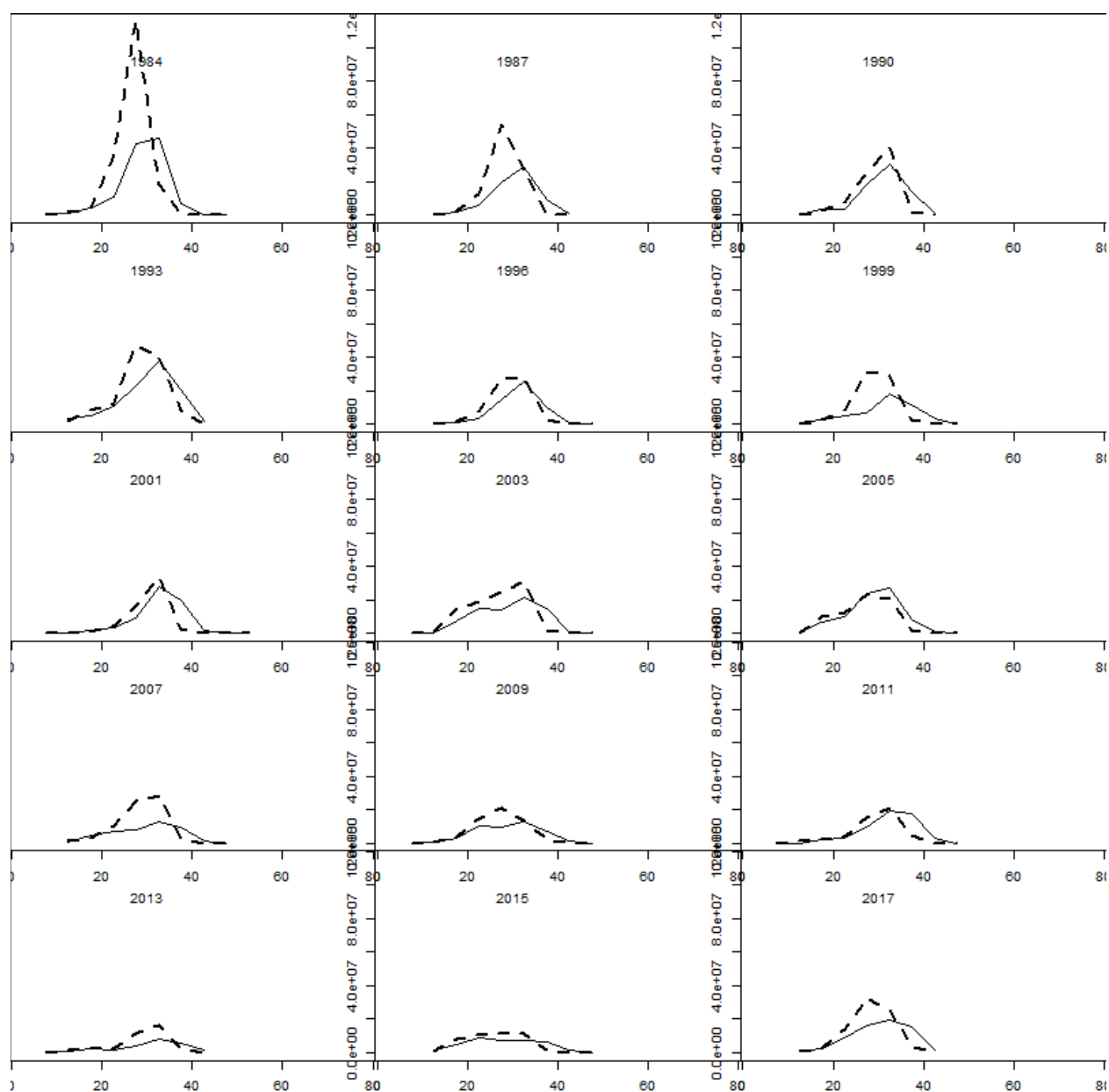
Figure 4.4. Population size composition (females solid line, males dashed line) of yellowfin sole as estimated from the NMFS bottom trawl surveys, 1984-2017.
