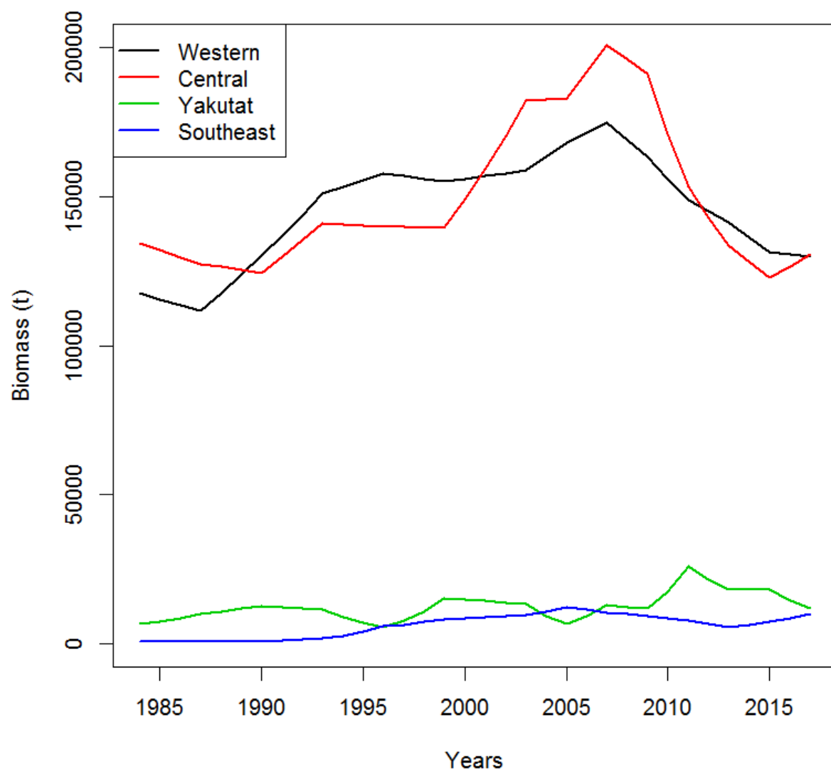
Figure 4.13. Random effects model estimates of biomass by area for shallow-water flatfish 1984 to 2017 (including Rock sole).
