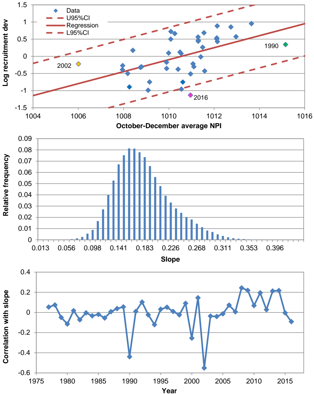
Figure 2.34—Environmental effects on recruitment. Upper panel: Estimated log recruitment deviations (age 0) versus same-year October-December average of the NPI, with regression line and 95% confidence interval. Middle panel: Distribution of the regression slope, as generated by a cross-validation analysis. Lower panel: Correlation between individual data points and regression slope. See text for details.
