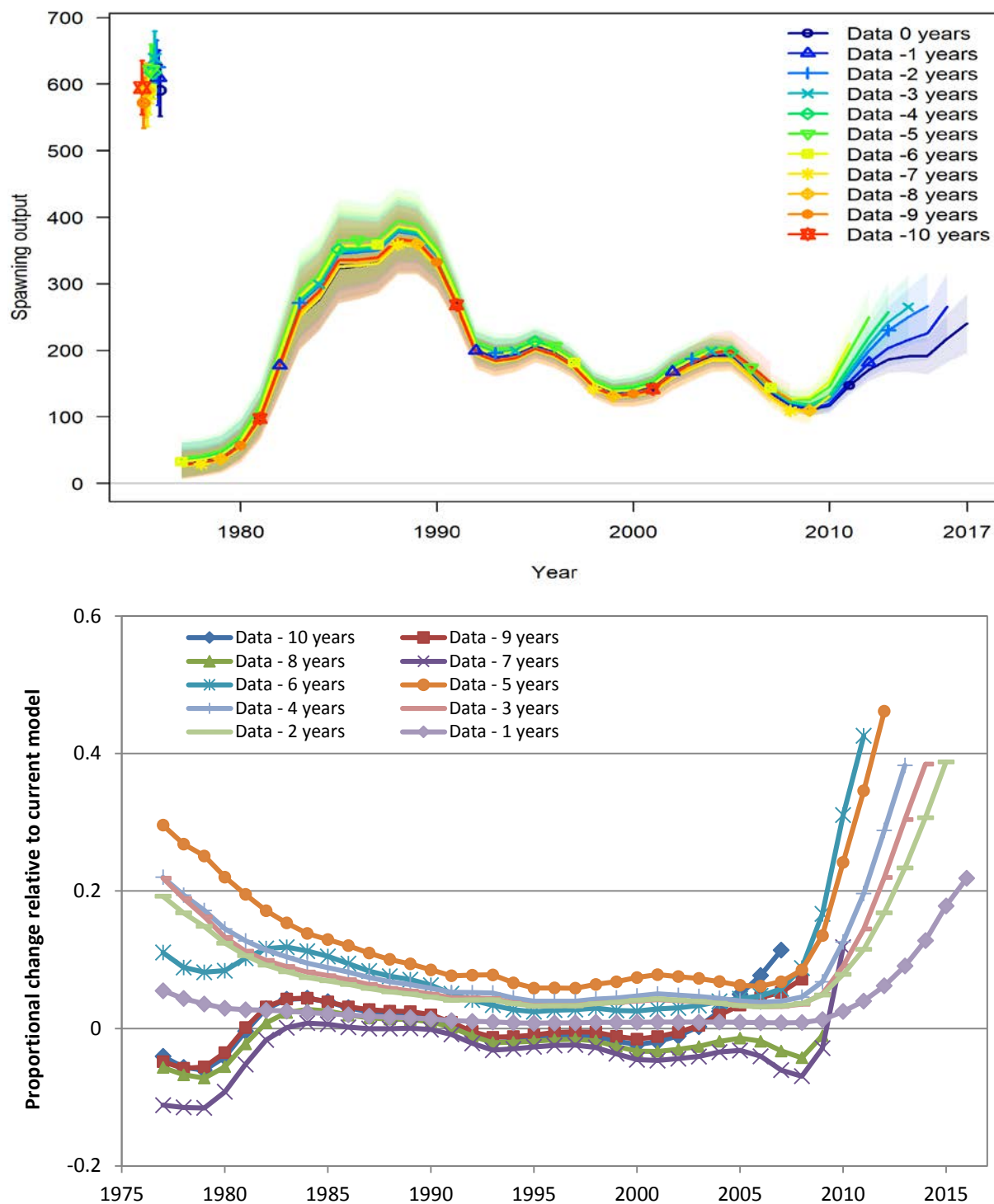
Figure 2.30c—Retrospective analysis of spawning biomass estimates from Model 17.2. Top panel: spawning biomass time series with 95% confidence intervals from the current version of Model 17.2 (2017) and 10 retrospective runs (2007-2016) obtained by dropping one year of data at a time. Bottom panel: change in spawning biomass relative to the current version of Model 17.2 for each of 10 retrospective runs. Mohn's \rho = 0.255 .
