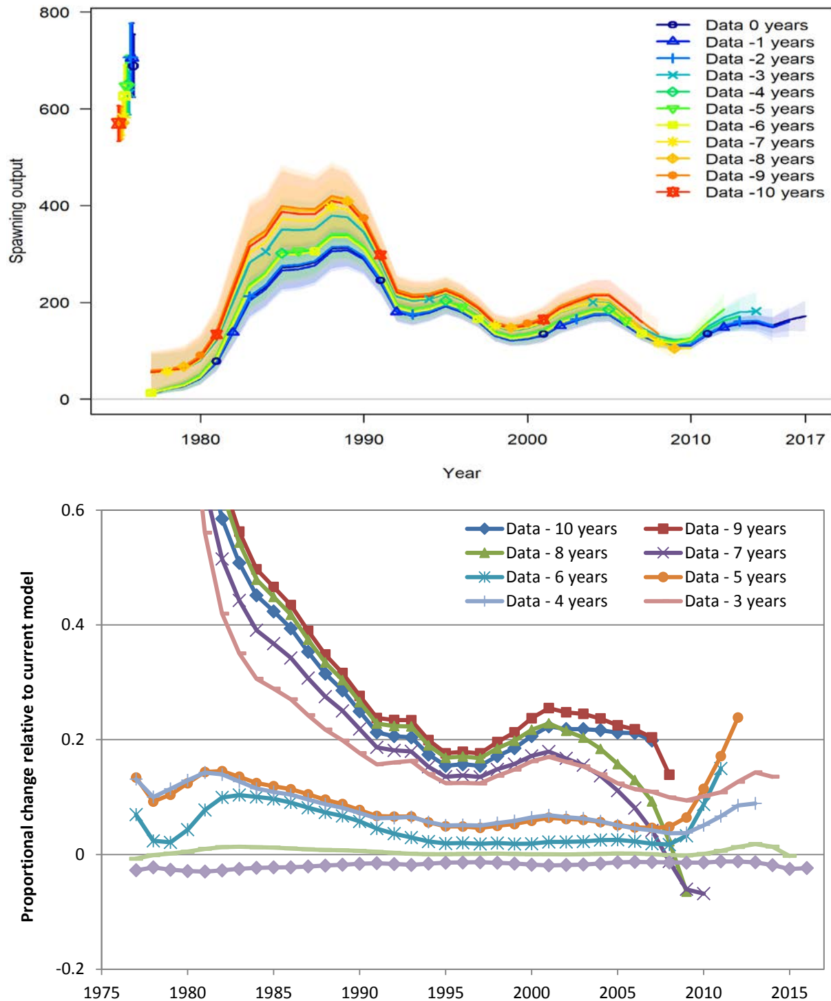
Figure 2.30f—Retrospective analysis of spawning biomass estimates from Model 17.7. Top panel: spawning biomass time series with 95% confidence intervals from the current version of Model 17.7 (2017) and 10 retrospective runs (2007-2016) obtained by dropping one year of data at a time. Bottom panel: change in spawning biomass relative to the current version of Model 17.7 for each of 10 retrospective runs. Mohn's \rho = 0.079 .
