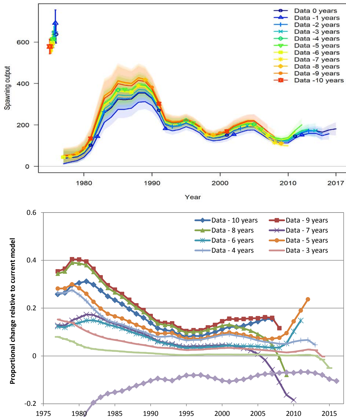
Figure 2.30e—Retrospective analysis of spawning biomass estimates from Model 17.6. Top panel: spawning biomass time series with 95% confidence intervals from the current version of Model 17.6 (2017) and 10 retrospective runs (2007-2016) obtained by dropping one year of data at a time. Bottom panel: change in spawning biomass relative to the current version of Model 17.6 for each of 10 retrospective runs. Mohn's \rho = 0.028 .
