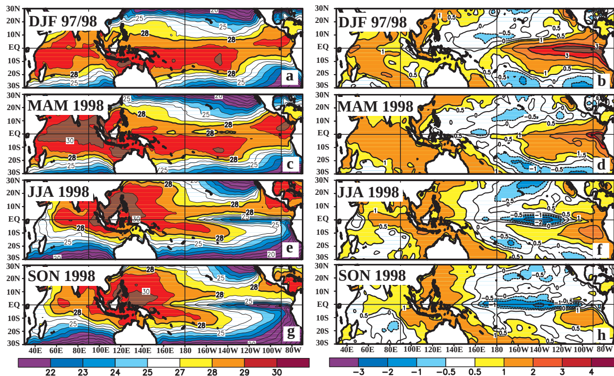
FIG. 24. Seasonal SST (left) and anomaly (right) for (a, b) DJF 1997/98, (c, d) MAM 1998, (e, f) JJA 1998 and (g, h) SON 1998. Contour interval is 1°C, with the 0.5°C anomaly contour included. Anomalies are departures from the 1950–79 adjusted OI climatology (Reynolds and Smith 1995).
