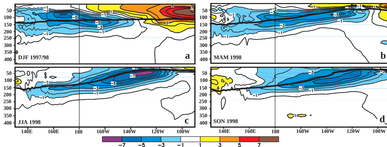
FIG. 25. Equatorial depth–longitude section of ocean temperature anomalies for (a) DJF 1997/98, (b) MAM 1998, (c) JJA 1998, and (d) SON 1998. Contour interval is 1°C. The dark line is the 20°C isotherm. Data are derived from an analysis system that assimilates oceanic observations into an oceanic GCM (Behringer et al. 1998). Anomalies are departures from the 1983–92 base period means.
