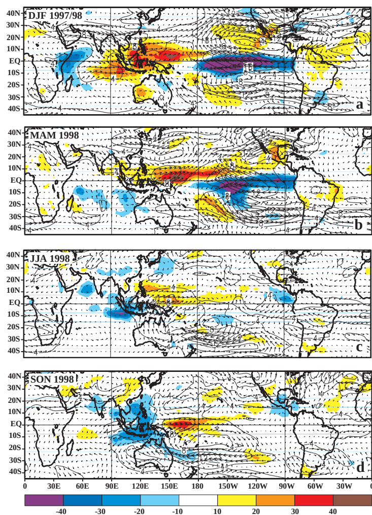
FIG. 27. OLR anomalies (shaded) and 200-hPa vector wind anomalies and isotachs for (a) DJF 1997/98, (b) MAM 1998, (c) JJA 1998, and (d) SON 1998. Contour interval for isotachs is 4 \text{ m s}^{-1} . Shading interval for OLR anomalies is 10 \text{ W m}^{-2} . Anomalies are departures from the 1979–95 base period monthly means.
