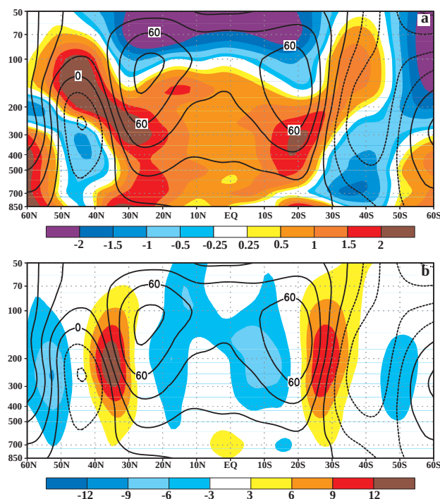
FIG. 41. April–June 1998 height–latitude section at 115°W of (a) height anomalies (m, contours) and temperature anomalies (°C, shading), and (b) height anomalies and zonal wind speed anomalies (m s -1 , shading). Anomalies are departures from the 1979–95 base period means.
