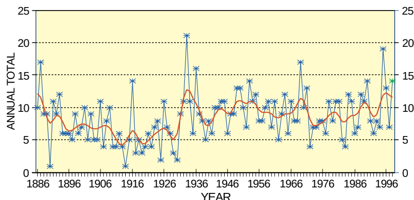
FIG. 32. Number of hurricanes and tropical storms for the North Atlantic basin: 1998 is shown in green. (Source: National Climatic Data Center.)
