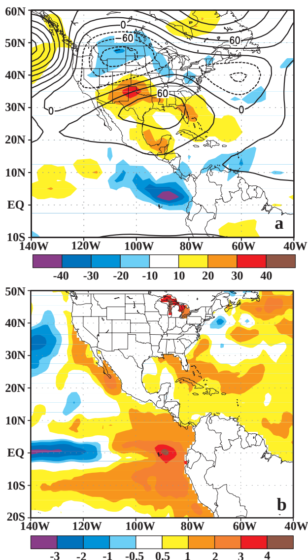
FIG. 42. June 1998 upper-level (200 hPa) (a) height anomalies (m, contours) and OLR anomalies ( \text{W m}^{-2} , shaded), and (b) SST anomalies (°C, shaded). Anomalies are departures from the (a) 1979–95 and (b) 1950–79 base period means.
