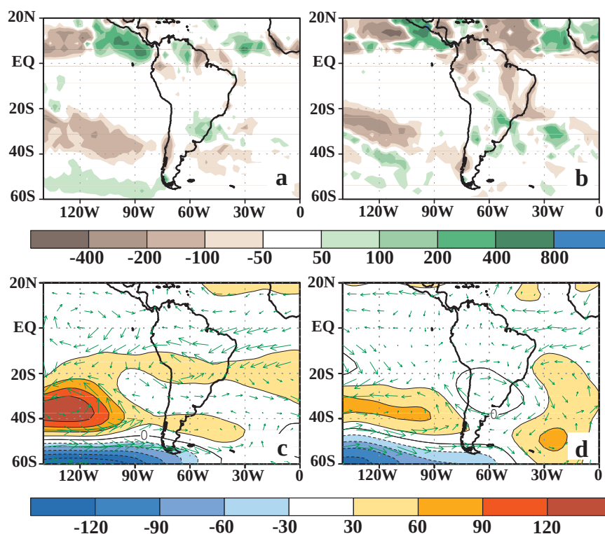
FIG. 60. (top) Precipitation anomalies during (a) JJA 1998 and (b) SON 1998. (bottom) 200-hPa height and wind vector anomalies during (c) JJA 1998 and (d) SON 1998. Anomalies are departures from the 1979–95 base period means.
