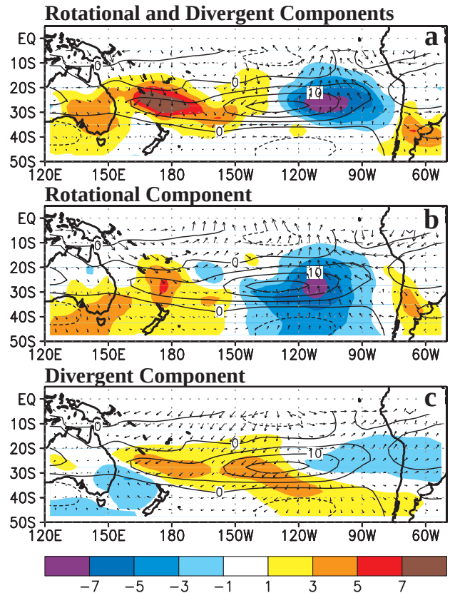
FIG. 30. Anomalous Lagrangian tendency of kinetic energy (shading, interval is 1 \times 10^{13} \text{ m}^2 \text{ s}^{-3} ) and ageostrophic wind vector during July–September 1997, associated with (a) both the rotational and divergent components of the horizontal ageostrophic flow, (b) the rotational component of the horizontal ageostrophic flow, and (c) the divergent component of the horizontal ageostrophic flow. Also shown in all panels is the anomalous geostrophic wind speed (contours, interval is 5 \text{ m s}^{-1} ). Lagrangian kinetic energy tendency results from the ageostrophic flow directed across the geopotential height contours. Anomalous tendencies are calculated as the difference between the observed and the climatological mean. Climatology is the 1979–95 base period monthly means.
