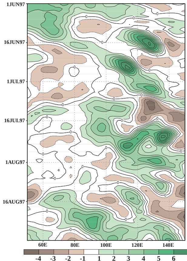
FIG. 51. Time-longitude section at 30°N of anomalous 200-hPa relative vorticity 1 June–31 August 1997. Units are 10^{10} \text{ s}^{-1} . A five-day running mean smoother has been applied to the data. Anomalies are departures from the 1979–95 base period daily means.
