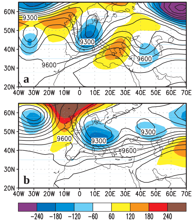
FIG. 55. The 300-hPa geopotential height (contours, units are m) and anomalies (shaded) for (a) 5 July and (b) 19 July 1997. Anomalies are departures from the 1979–95 base period daily means.
