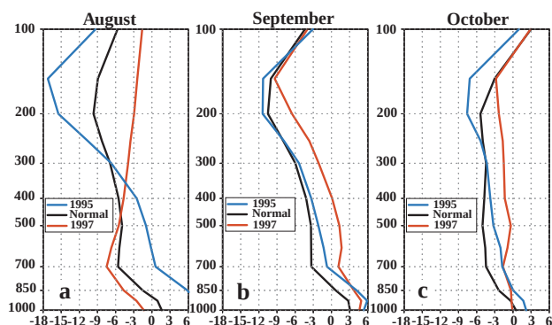
FIG. 41. Vertical profile of atmospheric zonal winds ( \text{m s}^{-1} ) averaged over the eastern North Pacific sector during (a) August, (b) September, and (c) October. Negative values indicate easterly winds and positive values indicate westerly winds. The black curve indicates the 1979–95 normal conditions, the red curve indicates 1997 conditions, and the blue curve indicates 1995 conditions.
