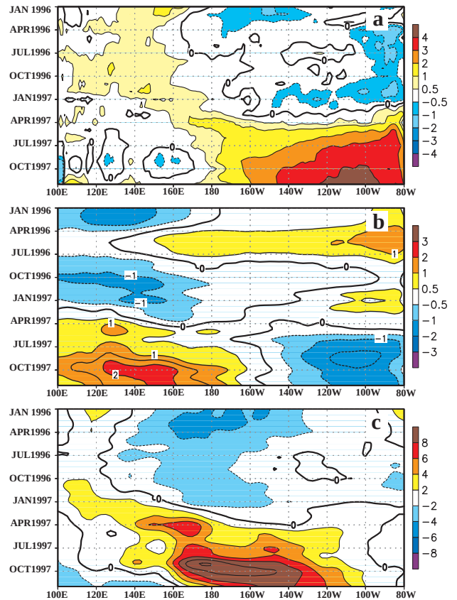
FIG. 21. Time–longitude sections ( 5^{\circ}\text{N} – 5^{\circ}\text{S} ) of anomalous (a) SST ( ^{\circ}\text{C} ), (b) SLP (hPa), and (c) zonal wind ( \text{m s}^{-1} ). SST anomalies are departures from the 1950–79 adjusted OI climatology (Reynolds and Smith 1995); SLP and wind anomalies are departures from the 1979–95 base period monthly means. A three-month running mean smoother has been applied to the SLP and wind data.
