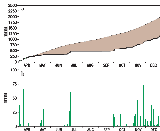
FIG. 62. Daily rainfall (mm) at Menado, Celebes, during April–December 1997: (a) accumulated observed (thick line) and accumulated climatological mean (1961–90 base period), and (b) observed daily total. Shading in (a) shows the accumulated departure from normal, with brown shading indicating negative departures.
