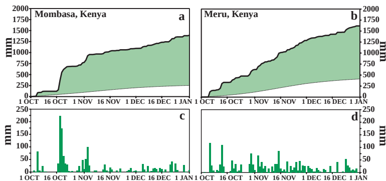
FIG. 45. (a),(b) Accumulated observed precipitation (solid curve) and accumulated climatological precipitation (1961–90 base period) (dashed curve) beginning 1 October 1997 and ending 1 January 1998 at (a) Mombasa, Kenya, and (b) Meru, Kenya. (c),(d) Daily precipitation totals during October 1997–1 January 1998 at (c) Mombasa, Kenya, and (d) Meru, Kenya. Green shading in (a),(b) indicates the difference between the observed and normal accumulated rainfall.
