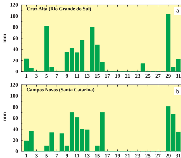
FIG. 57. Observed daily precipitation (mm) during October 1997 for (a) Cruz Alta and (b) Campos Novos, both in southern Brazil. [Source: CPTEC.]
