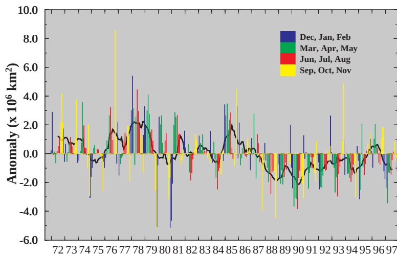
FIG. 18. Anomalies of monthly snow cover extent over the Northern Hemisphere. Smoothed curve is a 12-month running mean. Anomalies are departures from the 1972–96 base period means. (Analysis provided by Rutgers University.)
