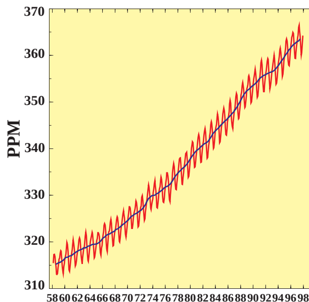
FIG. 17. Monthly mean carbon dioxide concentrations (red curve, ppm) measured at Mauna Loa, HI. Blue line is the 12-month running mean. The data through 1973 are from C. D. Keeling at Scripps Institute of Oceanography. [Analysis provided by CMDL.]
