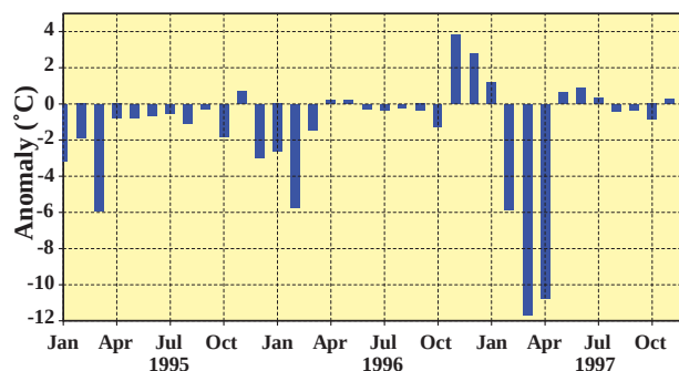
FIG. 9. Monthly Northern Hemisphere polar stratospheric temperature anomalies ( ^{\circ}\text{C} , 60^{\circ} – 90^{\circ}\text{N} ) derived from the MSU channel 4. Anomalies are departures from the 1979–95 base period means. (MSU data provided by the University of Alabama in Huntsville.)
