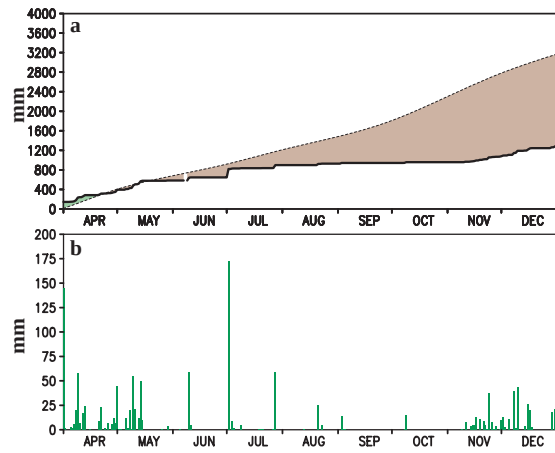
FIG. 63. Daily rainfall (mm) at Pedana Tabing, Sumatra, during April–December 1997: (a) accumulated observed (thick line) and accumulated climatological mean (1961–90 base period), and (b) observed daily total. Shading in (a) shows the accumulated departure from normal, with brown shading indicating negative departures.
