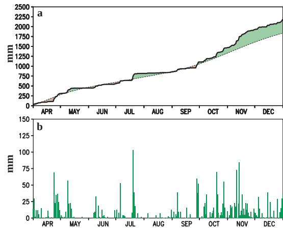
FIG. 64. Daily rainfall (mm) at Kuala Lumpur, Sumatra, during April–December 1997: (a) accumulated observed (thick line) and accumulated climatological mean (1961–90 base period), and (b) observed daily total. Shading in (a) shows the accumulated departure from normal, with green shading indicating positive departures.
