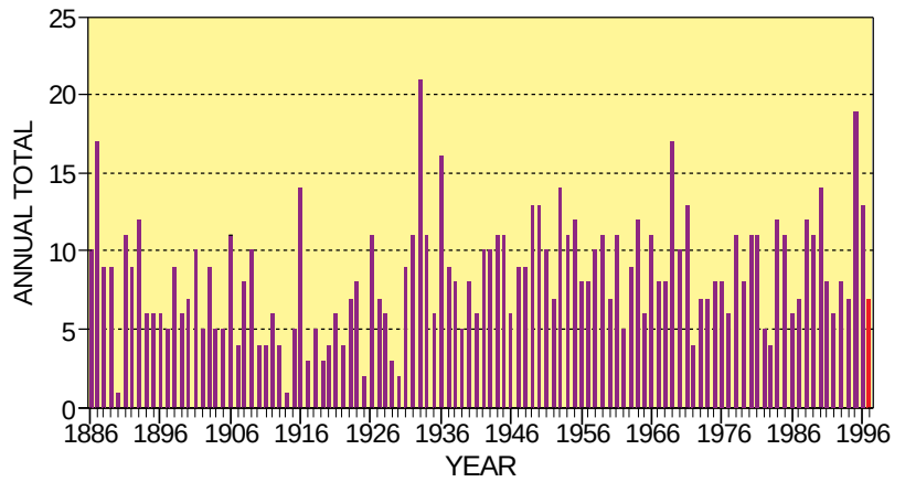
FIG. 38. Number of hurricanes and tropical storms for the North Atlantic basin: 1997 is shown in red. (Source: National Climatic Data Center.)
