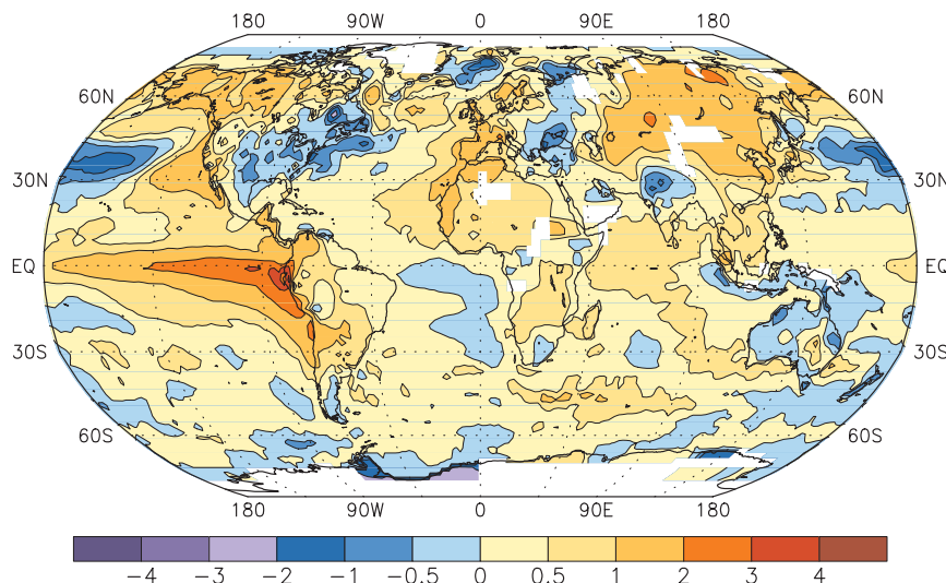
FIG. 4. Annual surface temperature anomalies ( ^{\circ}\text{C} ) for 1997. Analysis is based on station data over land and on SST data over the oceans. Anomalies are departures from the 1961–90 base period means. White areas are regions with insufficient data for analysis.
