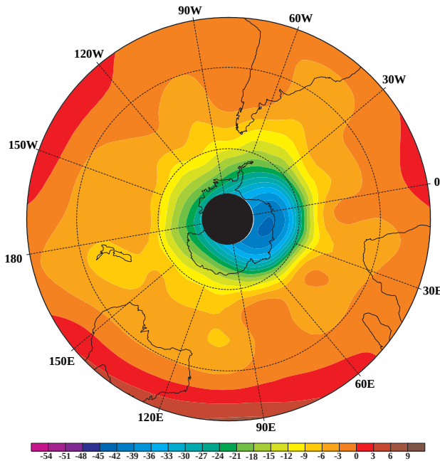
FIG. 13. Total ozone percent difference between October 1997 and the October 1979–86 based period means. Regions with no data are shown in black.
