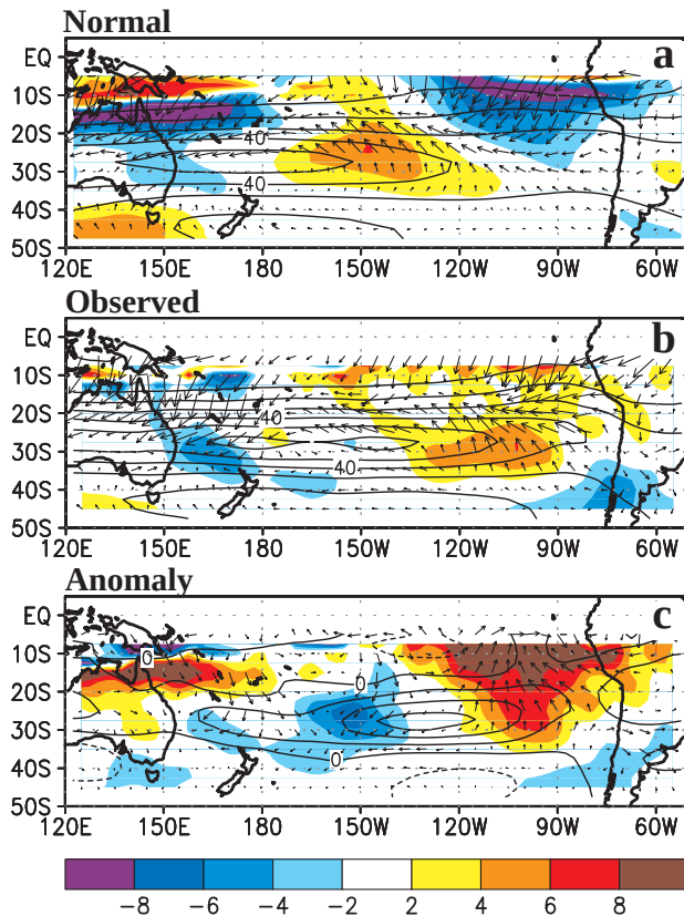
FIG. 29. Analysis of the South Pacific jet stream at 200 hPa during July–September 1997 showing geostrophic wind speed (contours), geostrophic diffuence/confluence (shading, interval is 2 \times 10^{16} \text{ s}^2 ), and horizontal component of the ageostrophic wind vector for (a) climatological mean and (b) observed, and (c) anomaly. Contour interval for isotachs in (a), (b) is 10 \text{ m s}^{-1} and in (c) is 5 \text{ m s}^{-1} . Diffuence and confluence are indicated by positive and negative values, respectively. Diffuence is calculated in Cartesian coordinates based on the transformation equations from the natural coordinate system provided by Bell and Keyser (1993). Anomalous diffuence is calculated as the numerical difference between the observed and the climatological mean. Climatology is the 1979–95 base period monthly means.
