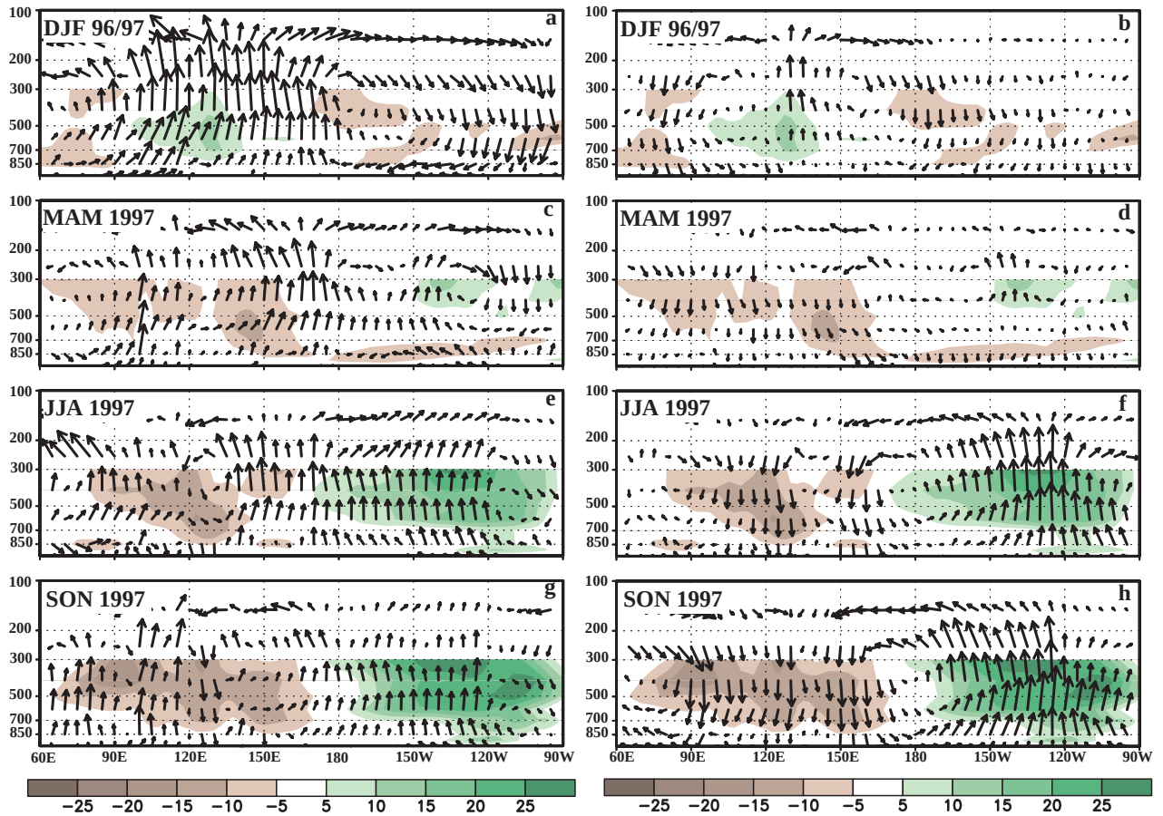
FIG. 28. Mean (left) and anomalies (right) pressure–longitude sections of the equatorial Walker circulation for (a),(b) DJF 1996/97, (c),(d) MAM 1997, (e),(f) JJA 1997, and (g),(h) SON 1997. Vertical component of vectors is the scaled pressure vertical velocity, and horizontal component is the zonal component of the divergent wind. The pressure vertical velocity was subjectively scaled to give a sense of the relative vertical motion in the equatorial plane. Shading in all panels shows relative humidity anomalies (%). Note that the relative humidity in the NCEP–NCAR reanalysis extends upward to only the 300-hPa level.
