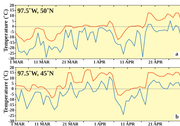
FIG. 35. Estimated daily maximum (red curve) and minimum (blue curve) temperatures ( ^{\circ}\text{C} ) during March and April 1997 over (a) the northern part of the Red River in southern Canada ( 50^{\circ}\text{N} , 97.5^{\circ}\text{W} ), and (b) eastern North Dakota near the central part of the Red River ( 45^{\circ}\text{N} , 97.5^{\circ}\text{W} ). Temperatures are from the NCEP–NCAR reanalysis dataset.
