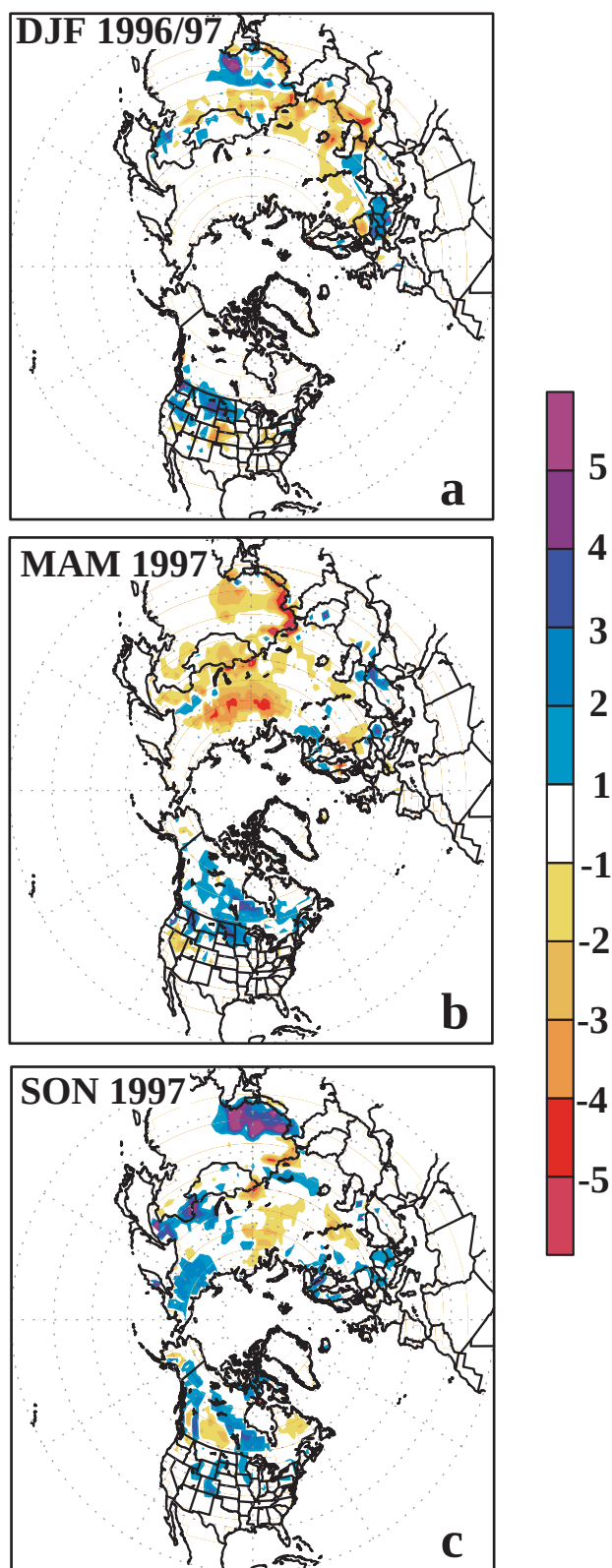
FIG. 19. Snow cover duration anomaly in weeks derived from operational analysis of visual imagery by NOAA/NESDIS: (a) December 1996–February 1997, (b) March–May 1997, and (c) September–November 1997.
