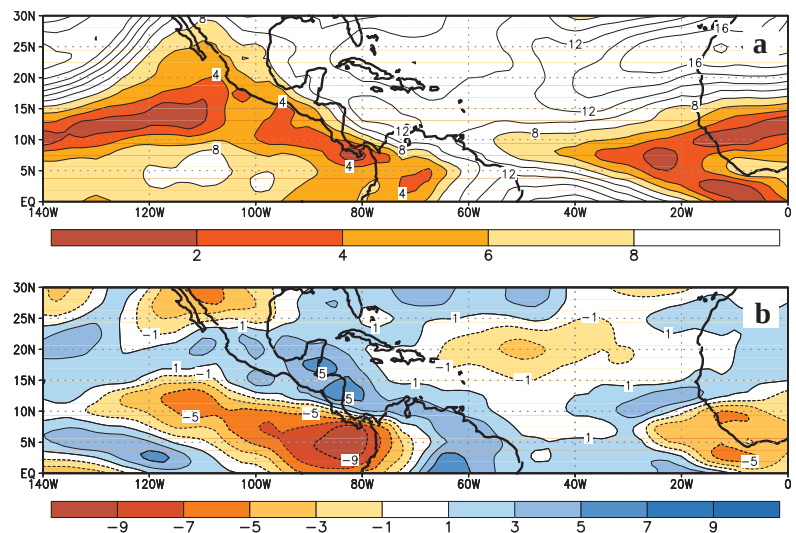
FIG. 39. (a) Vertical wind shear and (b) departure from normal during August–October 1997. Wind shear is calculated as the difference in wind speeds between 200 and 850 hPa (contour interval is 2 \text{ m s}^{-1} ). Shaded areas in (a) indicate where the vertical wind shear is less than 8 \text{ m s}^{-1} and are considered favorable for tropical cyclone formation.
