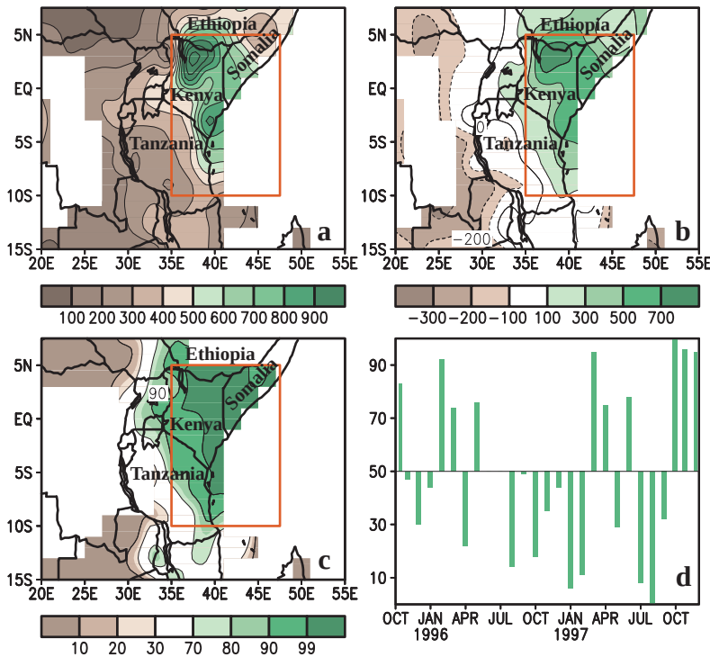
FIG. 44. October–December 1997 (a) total precipitation (mm), (b) precipitation anomalies (mm), and (c) precipitation percentiles based on a gamma distribution fit to the 1961–90 base period. (d) Monthly time series of precipitation percentiles, based on precipitation totals averaged over the boxed region depicted in (a)–(c).
