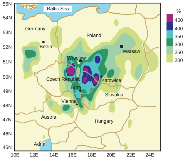
FIG. 54. July 1997 percent of normal rainfall relative to the 1961–90 base period means. (Source: Deutscher Wetterdienst, Hamburg, Germany).
