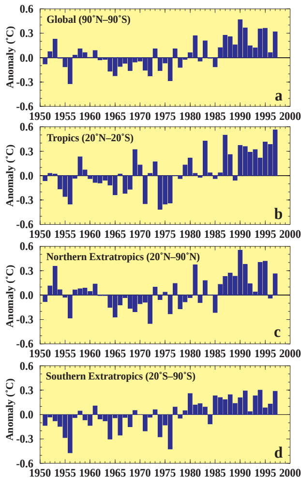
FIG. 3. Annual temperature anomalies (land only, °C): (a) global, (b) Tropics, (c) Northern Hemisphere extratropics, and (d) Southern Hemisphere extratropics. Anomalies are departures from the 1961–90 base period means.
