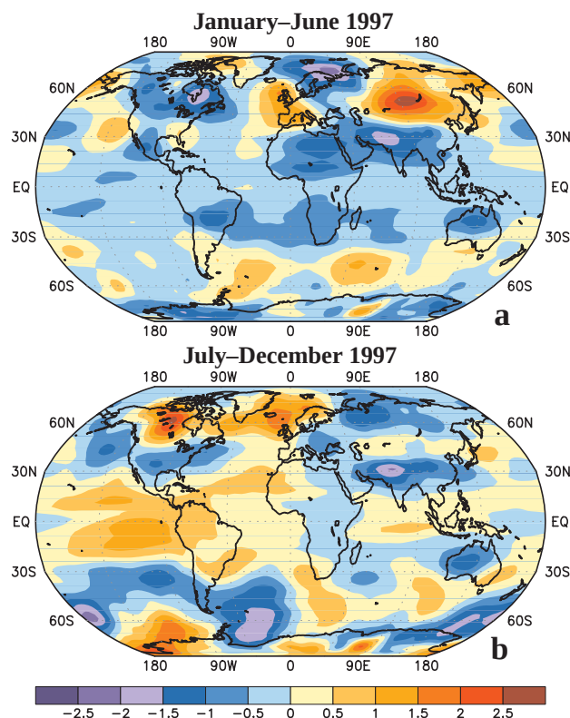
FIG. 6. Mean tropospheric temperature anomalies ( ^{\circ}\text{C} ) for (a) January–June 1997 and (b) July–December 1997 derived from the MSU channel 2R. Anomalies are departures from the 1979–95 base period means. (MSU data provided by the University of Alabama in Huntsville.)
