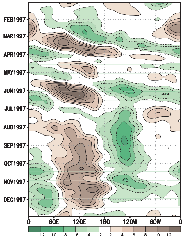
FIG. 32. Time-longitude section ( 5^{\circ}\text{N} – 5^{\circ}\text{S} ) of 200-hPa velocity potential anomalies ( 10^6 \text{ m}^2 \text{ s}^{-1} ). The period mean anomalies have been removed at each longitude.
