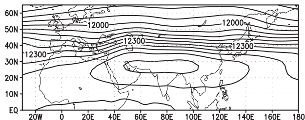
FIG. 50. June–August climatological mean 200-hPa geopotential height field (m) calculated for the 1979–95 period. Contour interval is 60 m.
