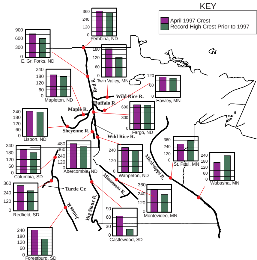
FIG. 33. Crests above flood stage (cm) for selected rivers in the north-central United States for April 1997 (purple) and for the previous record high crest (green). State abbreviations are North Dakota, ND; South Dakota, SD; and Minnesota, MN.
