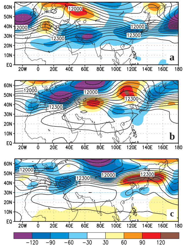
FIG. 52. The 200-hPa geopotential height (contours, units are m) and anomalies (shaded) for (a) 1–16 June, (b) 10–21 July, and (c) 22–30 July 1997. Anomalies are departures from the 1979–95 base period daily means.
