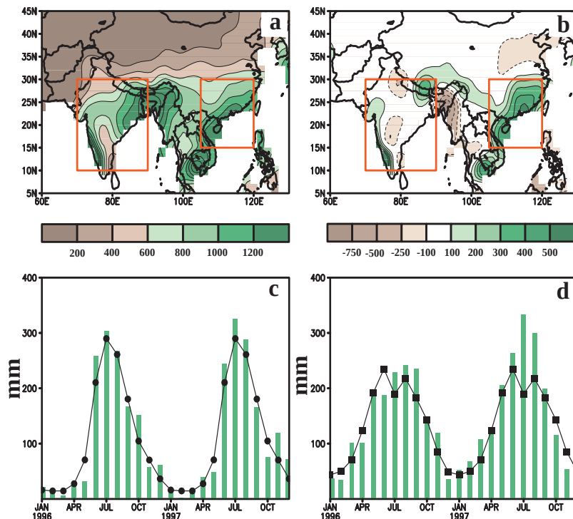
FIG. 49. (a) Total precipitation (mm) and (b) precipitation anomalies (mm) for June–September 1997. Monthly time series of total precipitation (mm, bars) and the 1961–90 mean (mm, line) averaged over (c) the boxed region centered on India and (d) the boxed region centered on southeastern Asia.
