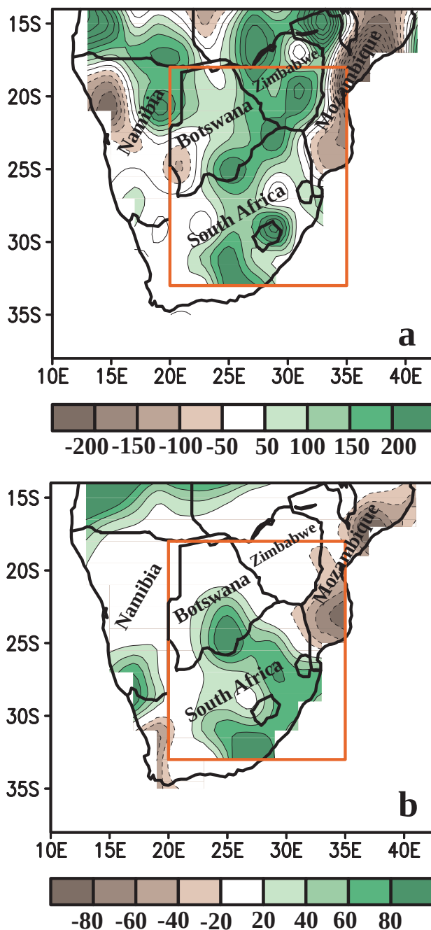
FIG. 46. (a) October 1996–April 1997 precipitation anomalies (mm) and (b) May–July 1997 precipitation anomalies (mm). Anomalies are departures from the 1961–90 base period means.
