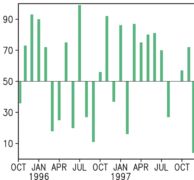
FIG. 47. Southern Africa monthly time series of precipitation percentiles based on a gamma distribution fit to the 1961–90 base period, calculated from precipitation totals averaged over the boxed region depicted in Fig. 46.
