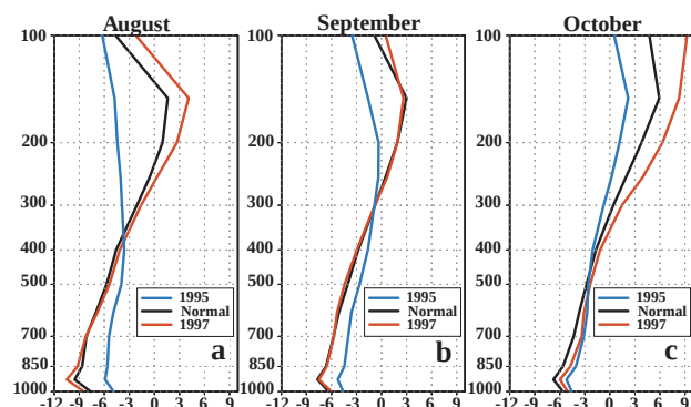
FIG. 40. Vertical profile of atmospheric zonal winds ( \text{m s}^{-1} ) averaged over the Caribbean Sea sector during (a) August, (b) September, and (c) October. Negative values indicate easterly winds and positive values indicate westerly winds. The black curve indicates the 1979–95 normal conditions, the red curve indicates 1997 conditions, and the blue curve indicates 1995 conditions.
