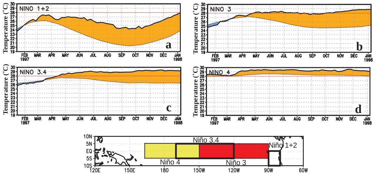
FIG. 24. Pentad (five-day averages) time series of tropical Pacific SSTs averaged over the following regions: (a) the Niño 1+2 region, (b) the Niño 3 region, (c) the Niño 3.4 region, (d) the Niño 4 region. In all panels, solid curve shows observed SST and dashed curve shows climatological mean SST. Orange shading indicates positive anomalies and blue shading indicates negative anomalies. The Niño regions are depicted in bottom panel. Climatological SSTs are derived from the 1950–79 adjusted OI climatology (Reynolds and Smith 1995).
