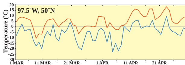
FIG. 37. Estimated daily maximum (red curve) and minimum (blue curve) temperatures ( ^{\circ}\text{C} ) during March and April 1994 over the northern part of the Red River in southern Canada ( 50^{\circ}\text{N} , 97.5^{\circ}\text{W} ). Temperatures are from the NCEP–NCAR reanalysis dataset.
