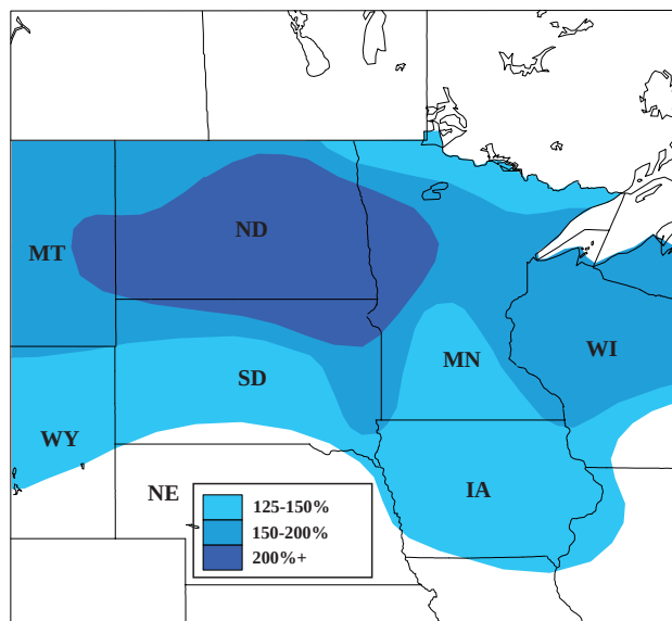
FIG. 34. Percent of normal accumulated snowfall during 1 September 1996–12 April 1997, compared to the 1961–90 base period means.
