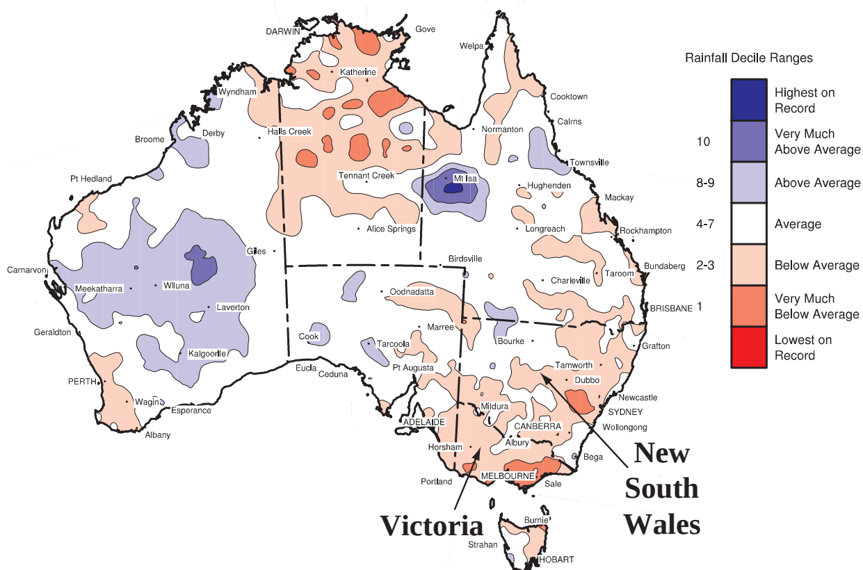
FIG. 66. March–November 1997 precipitation deciles. (Source: Australian Bureau of Meteorology.)
