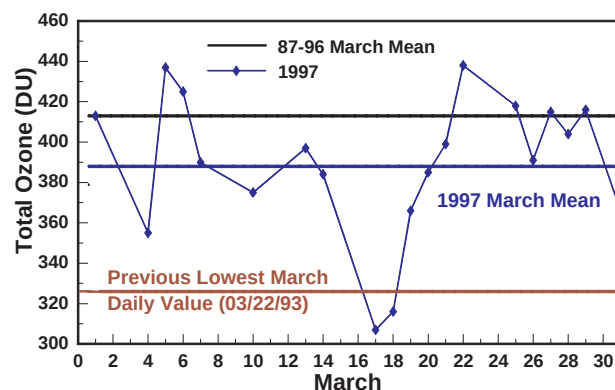
FIG. 12. Dobson spectrophotometer total ozone measurements at Point Barrow, AK, during March 1997. Values (blue) are daily averages for days when weather permitted observations. The 1987–96 March mean is drawn in black with the previous March daily low value shown in red.
