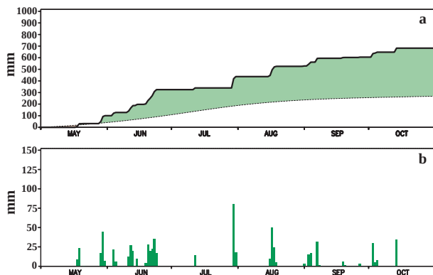
FIG. 59. Daily rainfall (mm) at Santiago, Chile, during May–October 1997: (a) accumulated observed (thick line) and accumulated normal (1961–90 base period), and (b) observed daily total. Shading in (a) shows the accumulated departure from normal, with green shading indicating positive departures.
