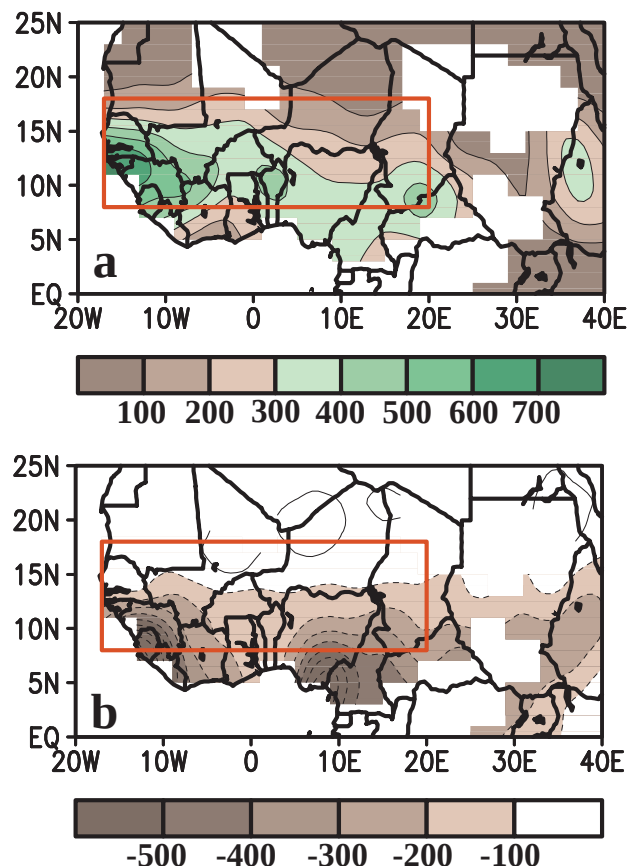
FIG. 48. July–September 1997 (a) total precipitation (mm) and (b) anomalies (mm) for the African Sahel region. The boxed region denotes the approximate boundaries of the African Sahel region.
