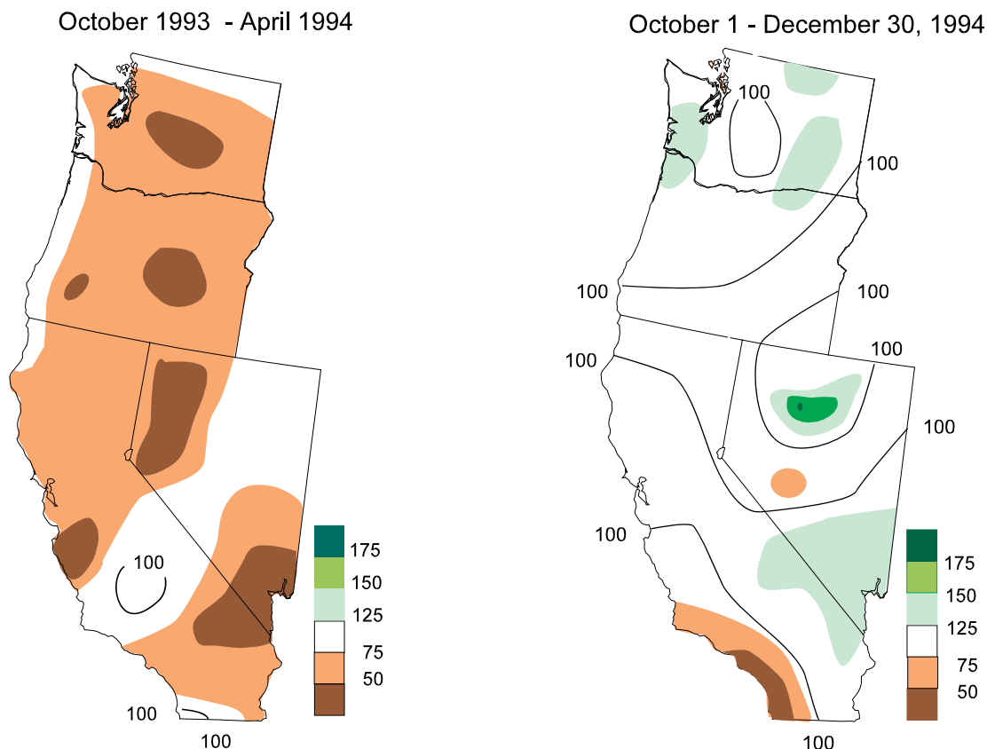
Figure 4.31 Percent of normal precipitation for October 1993 - April 1994 (left) and for October - December 1994, relative to the 1961-1990 base period. (Source: CAC).
