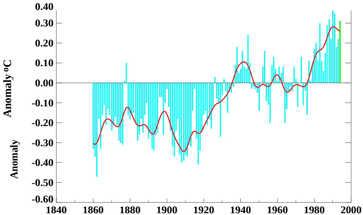
Figure 1.3 Global annual averages of combined land-air and sea surface temperature (SST) anomalies for each year from 1861-1994. Anomalies are computed with respect to the 1951-1980 base period. The red curve is a 13-term Gaussian filter designed to suppress variations on time scales less than 10 years. (Source: Hadley Centre for Climate Prediction and Research, UK)
