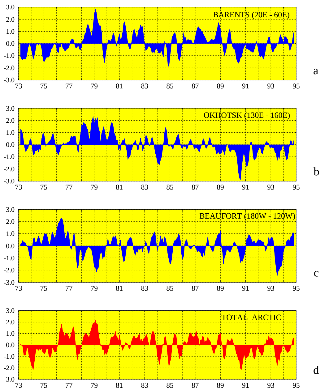
Figure 1.25 Standardized sea-ice area anomalies for the a) Barents Sea, b) Okhotsk Sea, c) Beaufort Sea, and d) Total Arctic. Values are standardized by the standard deviation for the 1973-1994 period. (Source: CAC)
