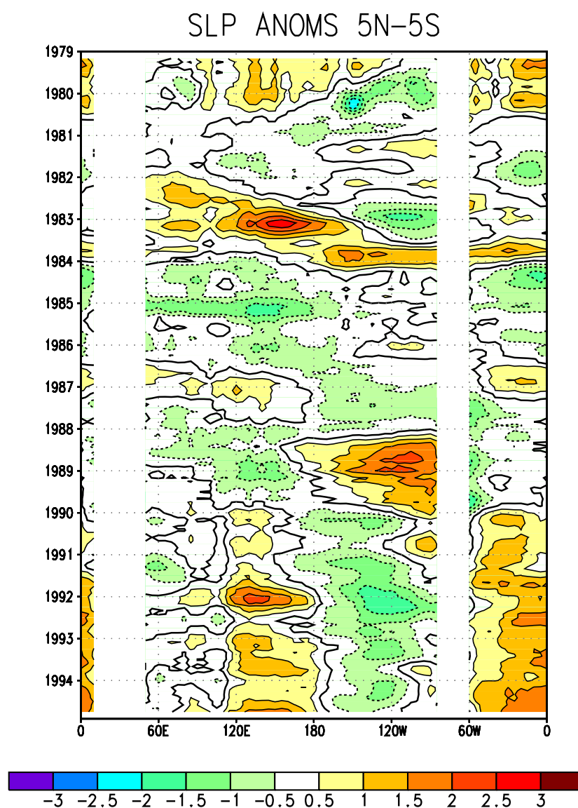
Figure 2.1 Time-longitude section of monthly sea level pressure anomalies averaged for 5°N-5°S. Contour interval is 0.5 mb. Anomalies are departures from the 1979-1988 base period means. Elevated regions are masked out. (Source: CAC)
