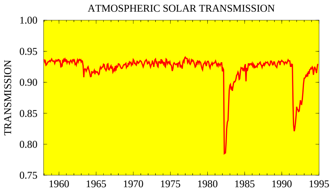
Figure 1.5 “Apparent” atmospheric solar transmission at Mauna Loa Observatory, Hawaii as determined from direct solar radiation measurements. The ratio is derived from broadband (0.3 to 2.8 \mu\text{m} ) direct solar irradiance observations and shows the effects of volcanic eruptions of aerosol concentrations over Mauna Loa. (Data provided by the Climate Monitoring and Diagnostics Laboratory.)
