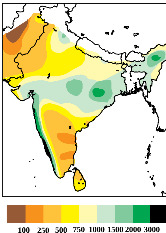
Figure 4.14 Total precipitation (mm) in India for June - September 1994. (Source: CAC)
