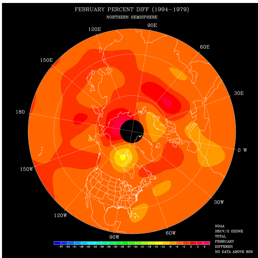
Figure 1.14 Total ozone percent difference between February 1994 and February 1979. Regions of no data are shown in black. (Source: CAC)
