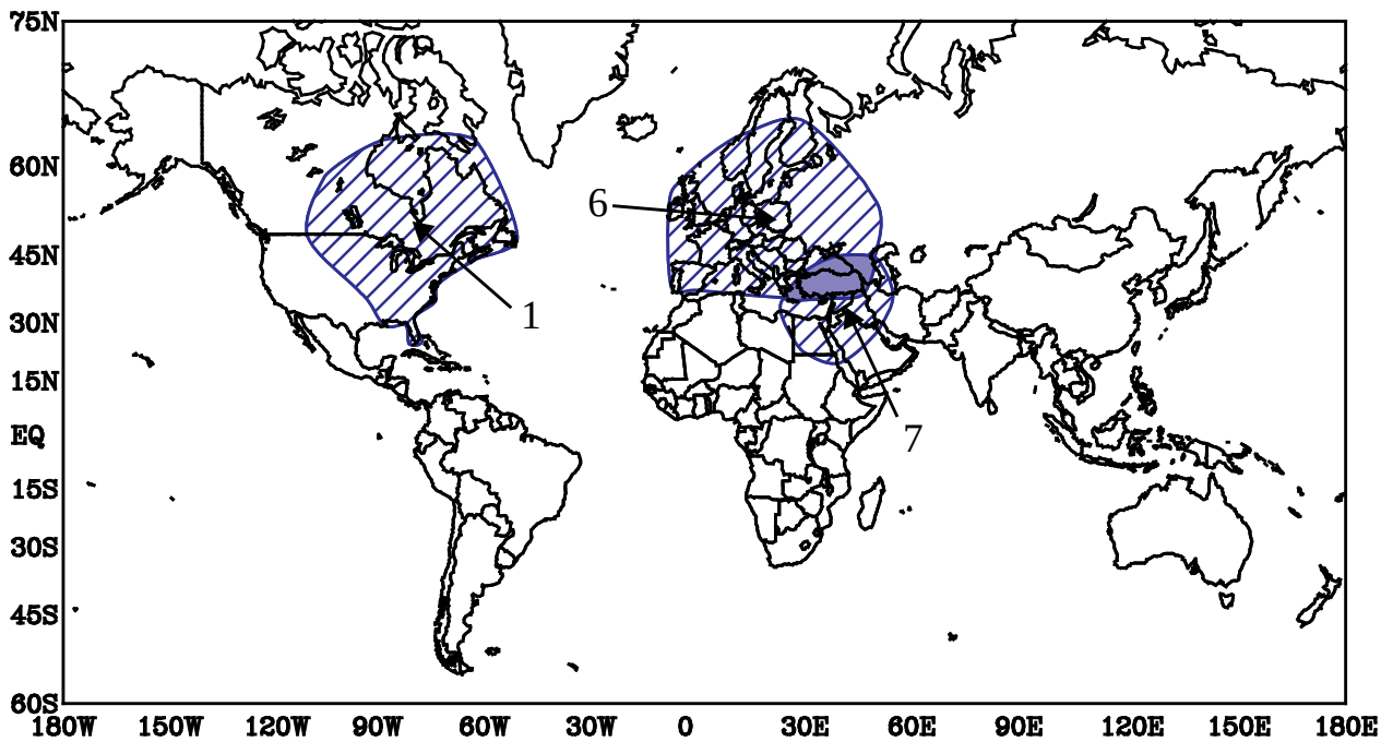
Figure 5.2 Significant above-normal temperature anomalies (top) and below-normal temperature anomalies (bottom) during 1994. The numbers are keyed to the descriptive paragraphs. (Source: CAC)
