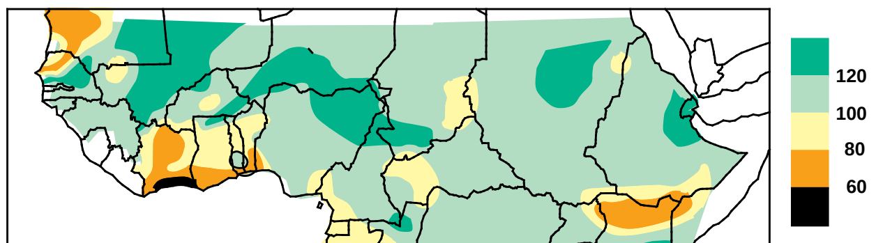
Figure 4.17 Percent of normal precipitation in the African Sahel for May - September 1994, relative to the 1961-1990 base period. (Source: CAC)
