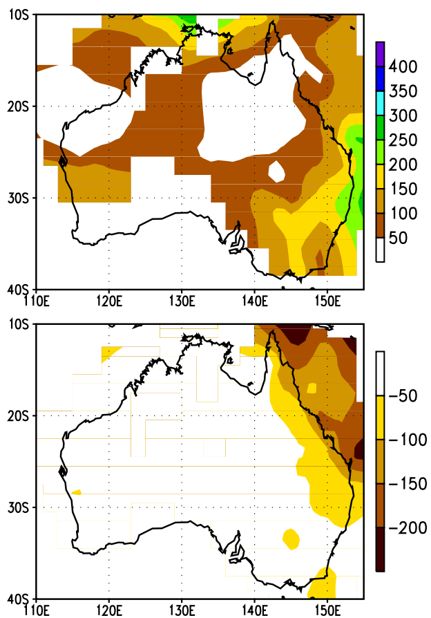
Figure 4.12 Total precipitation (mm, top) and anomalies (mm, bottom) during October - December 1994. Anomalies are departures from the 1961-1990 base period means. (Source: CAC)
