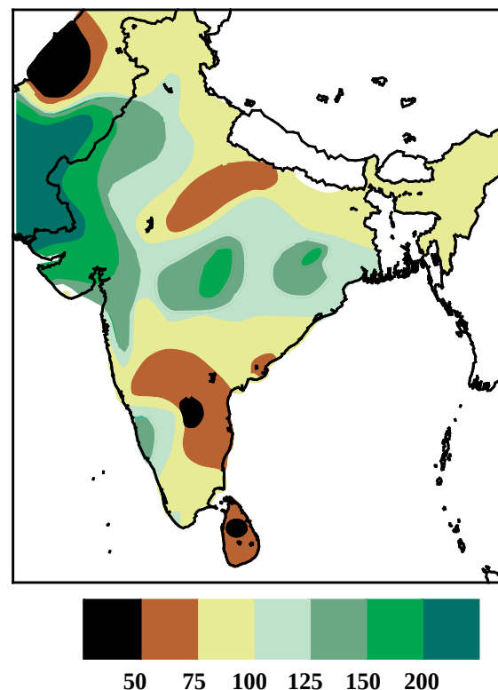
Figure 4.15 Percent of normal precipitation in India for June - September 1994, relative to the 1961-1990 base period. (Source: CAC)
