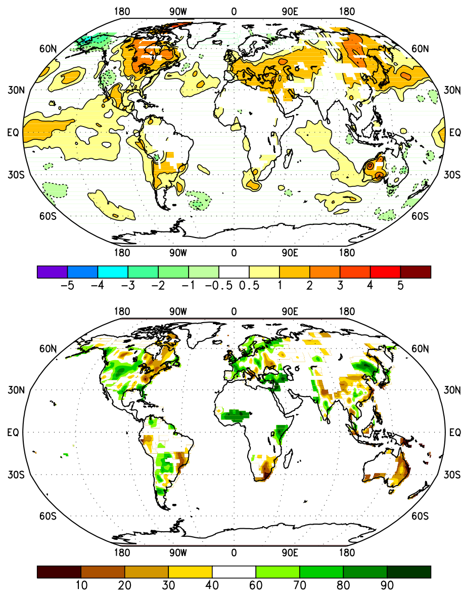
Figure 3.10 Surface temperature anomalies (°C) (top) and precipitation percentiles based on a gamma distribution fit to the 1961-1990 base period (bottom) for September - November 1994. Temperature anomalies are based on station data over land (1961-1990 base period) and sea surface temperature data (SST) over water (COADS/ICE climatology). Analysis omitted in data-sparse regions. (Source: CAC)
