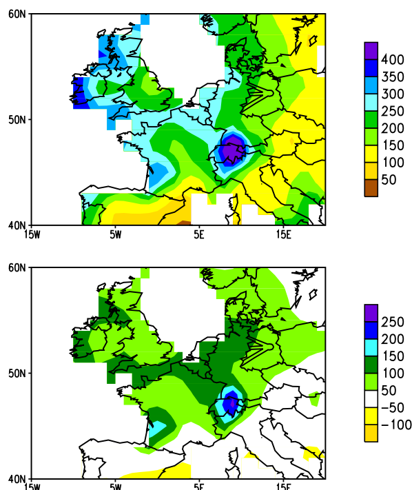
Figure 3.4 Total precipitation (mm, top) and anomalies (mm, bottom) across Europe during December 1993-January 1994. Anomalies are computed with respect to the 1961-1990 base period. (Source: CAC).
