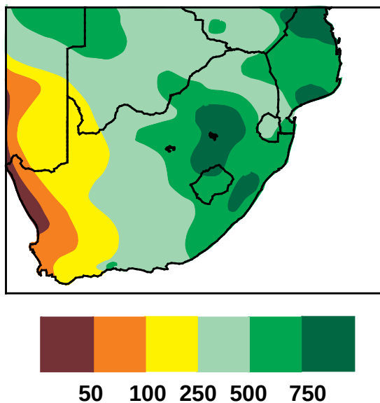
Figure 4.2 Total precipitation (mm) in southern Africa for October 1993 - April 1994. (Source: CAC)
