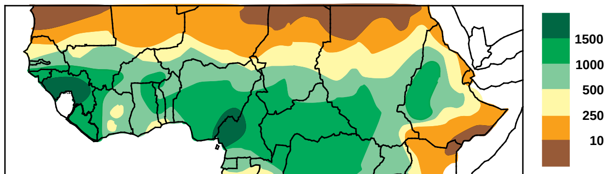
Figure 4.18 Total precipitation (mm) in the African Sahel for May - September 1994 (Source: CAC)
