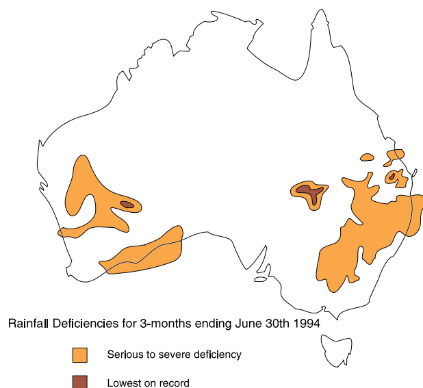
Figure 4.10 Rainfall deficiencies for April - June 1994. (Source: Australian Bureau of Meteorology)
