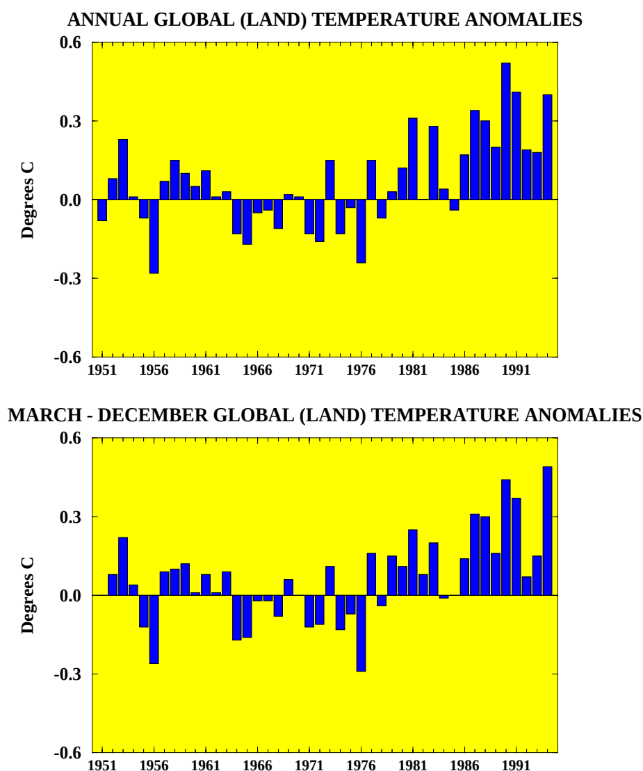
Figure 1.1 Annual (top) and March - December (bottom) global temperature anomalies (land only, °C). Anomalies are departures from the 1951-1980 base period means. (Source: CAC)
