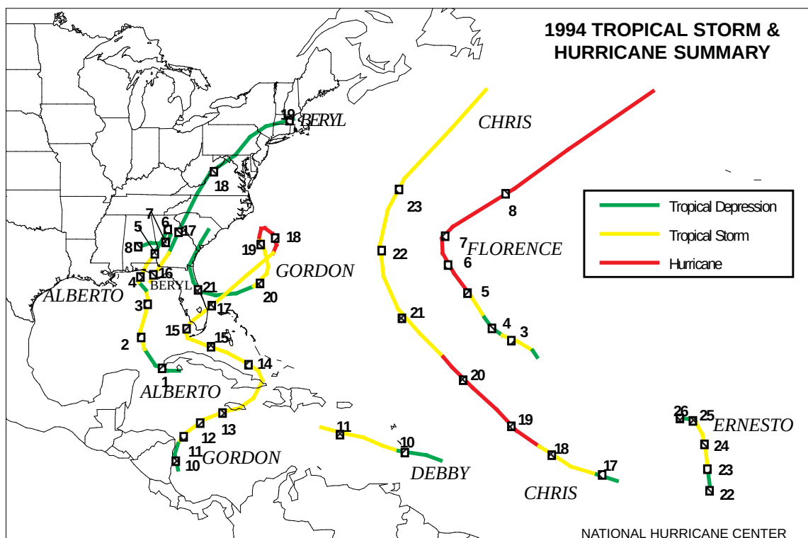
Figure 4.33 Tracks of Atlantic named storms for 1994. Red lines indicate periods of hurricane intensity, yellow lines show periods of tropical storm intensity, and green lines show periods of tropical depression intensity. Numbers pertain to day of month. (Source: National Hurricane Center)
