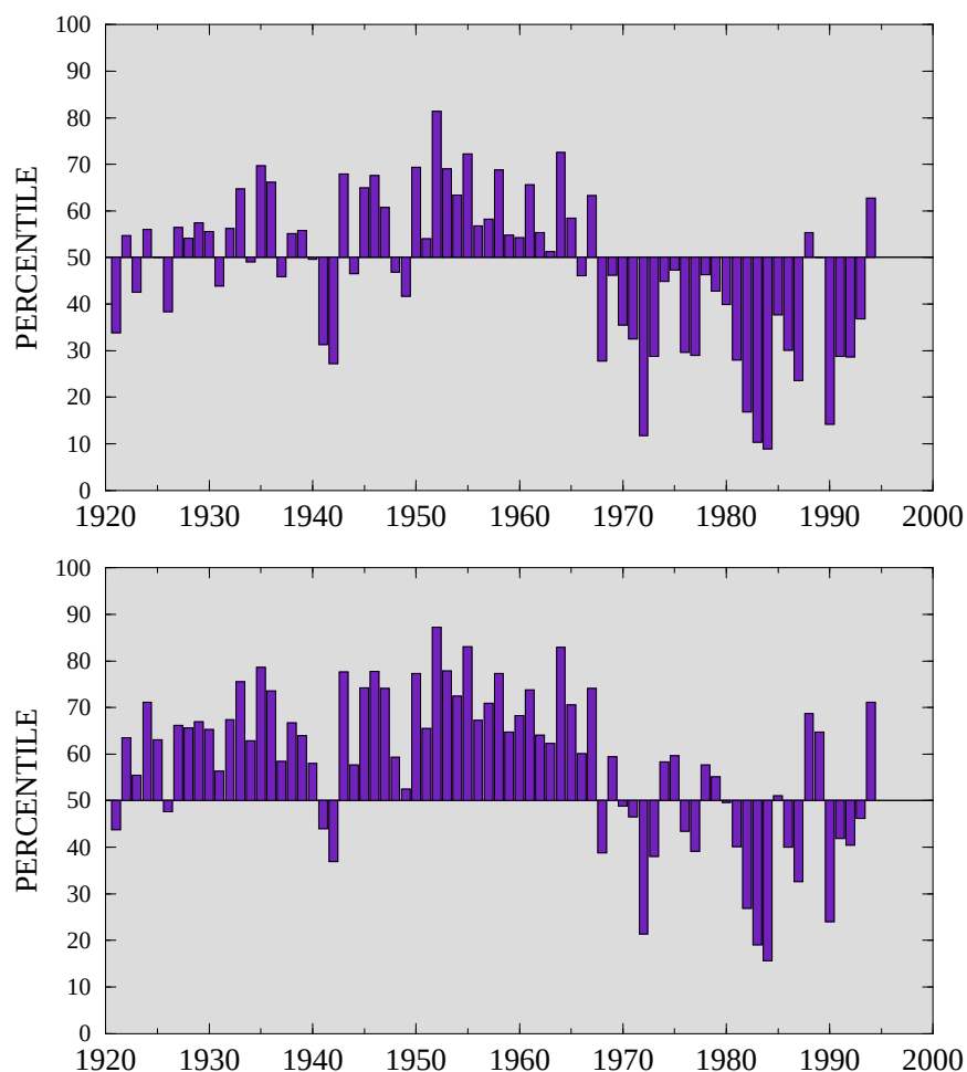
Figure 4.16 Precipitation index (average gamma percentiles of station precipitation within the region) for the western Sahel for June - September based on normals for 1951-1980 (top) and for 1961-1990 (bottom). (Source: CAC)
