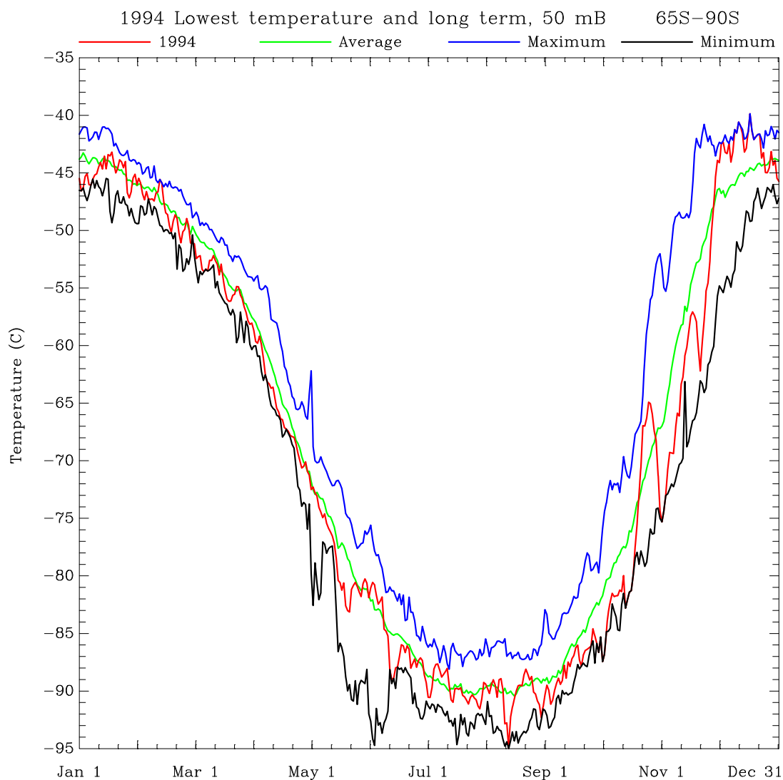
Figure 1.17 Daily minimum temperatures at 50 mb (19 km) in the region 65^{\circ}\text{S} to 90^{\circ}\text{S} for 1994 (red line). Mean daily values for the period 1978-1994 are shown in green, daily extreme minima for any year (black), and daily maxima for any year (blue) are also shown. (Source: CAC)
