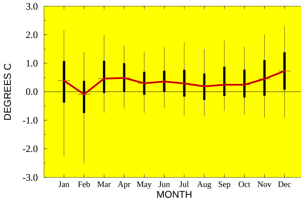
Figure 1.2 Monthly values of the median (land only) temperature anomalies for 1994 (red line). 50% of the 2° latitude by 2° longitude land areas have anomalies above (below) the median. Information about the distribution of monthly temperature anomalies is provided by the solid rectangles, indicating the 30% and 70% levels, and the thin vertical lines, indicating the 10% and 90% levels. The anomalies are departures from the 1961-1990 base period. (Source: CAC)
