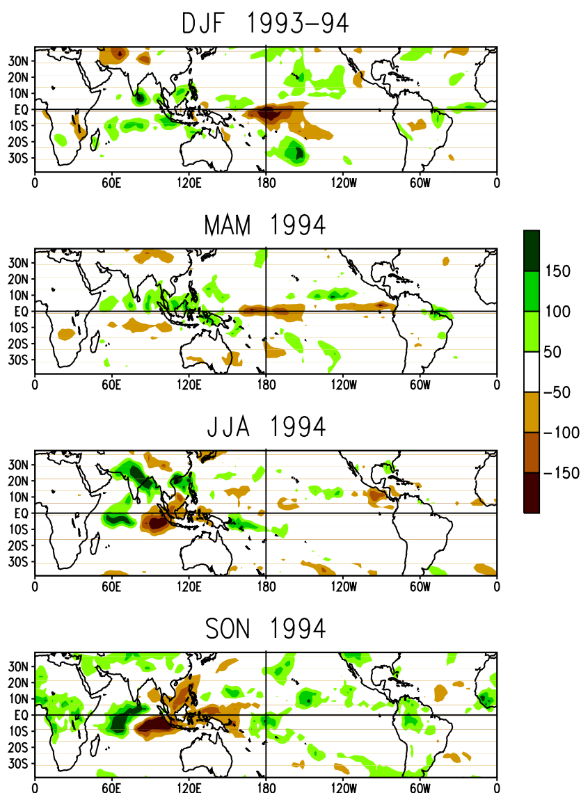
Figure 2.10 Satellite-derived rainfall anomaly estimates in mm per month. Anomalies are departures from the 1986–1993 base period means. (Source: CAC)
