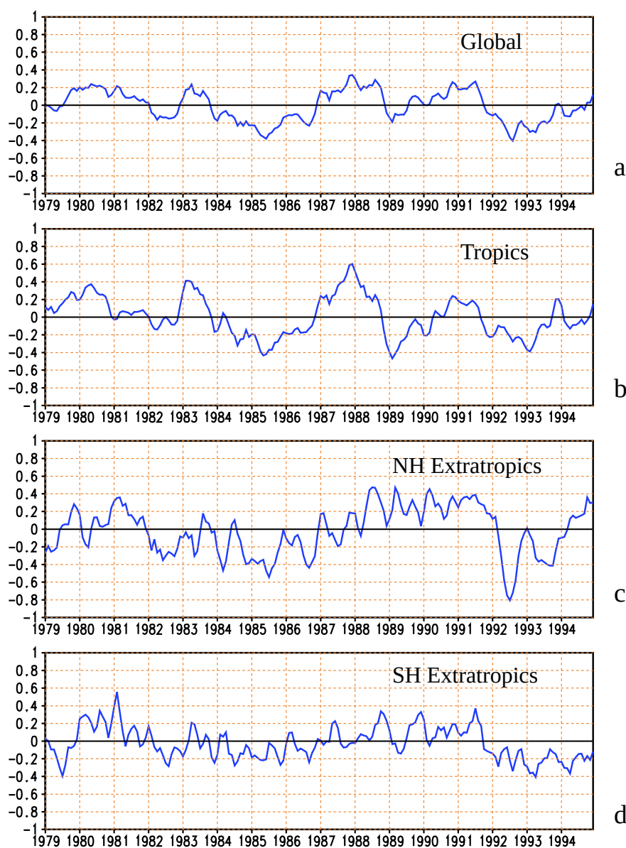
Figure 1.7 Mean tropospheric temperature anomalies ( ^{\circ}\text{C} ) from the Microwave Sounding Unit (MSU) channel 2R for the a) globe ( 85^{\circ}\text{S} - 85^{\circ}\text{N} ), b) tropics ( 30^{\circ}\text{N} - 30^{\circ}\text{S} ), c) Northern Hemisphere extratropics ( 30^{\circ}\text{N} - 85^{\circ}\text{N} ) and d) Southern Hemisphere extratropics ( 30^{\circ}\text{S} - 85^{\circ}\text{S} ). Anomalies are computed from the 1982-1991 base period. (Data provided by the University of Alabama at Huntsville.)
