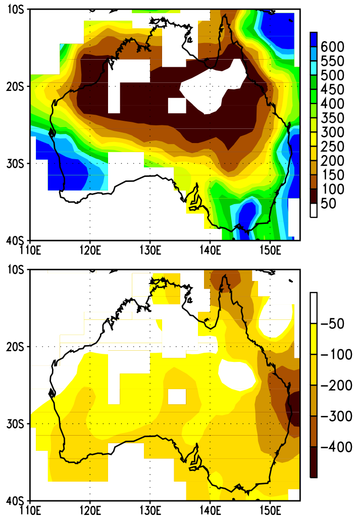
Figure 4.5 Total precipitation (mm, top) and anomalies (mm, bottom) during April - December 1994. Anomalies are departures from the 1961-1990 base period means. (Source: CAC)
