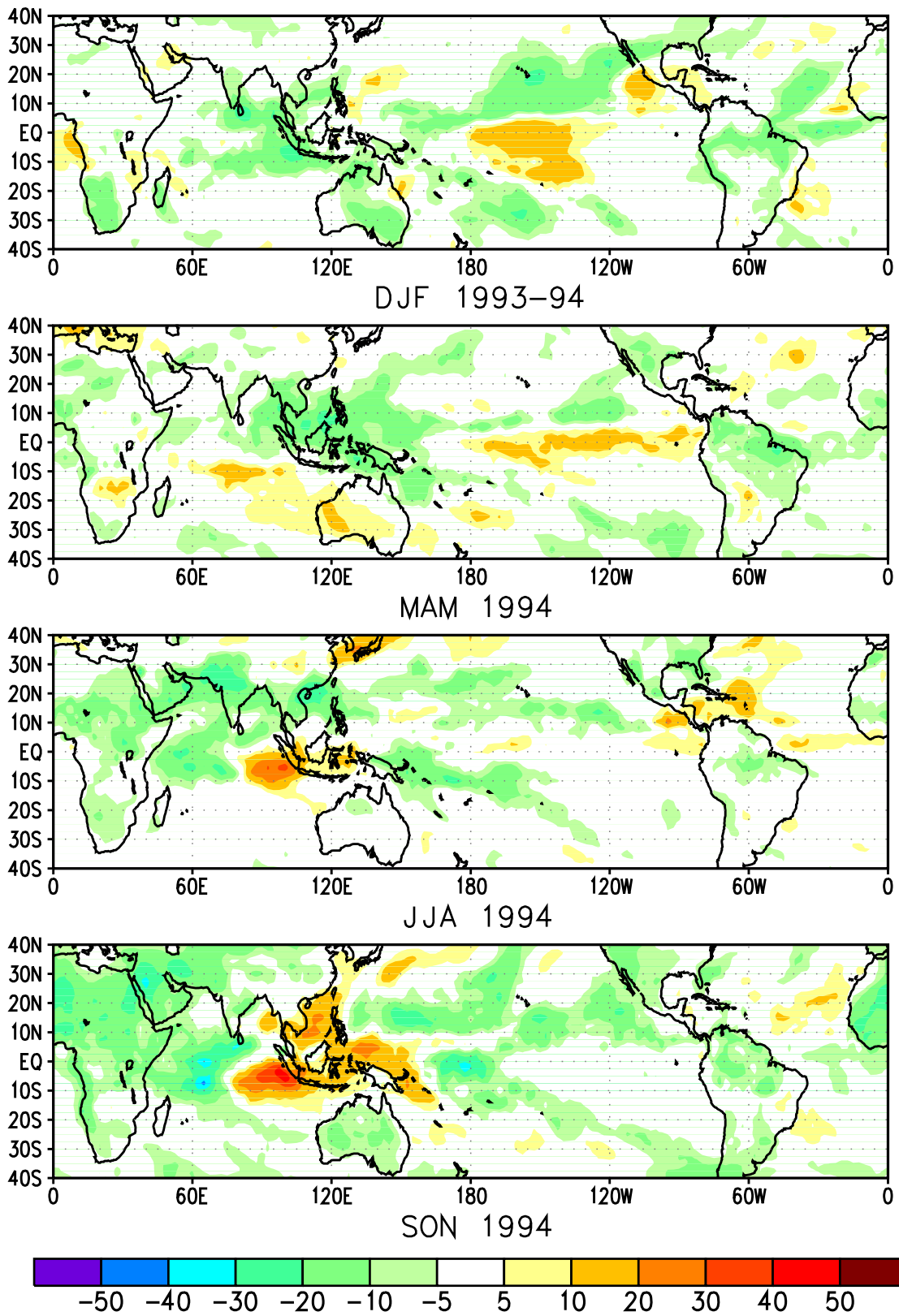
Figure 2.9 Seasonal outgoing longwave radiation (OLR) anomalies ( \text{Wm}^{-2} ) computed as departures from the 1979-1988 base period means. (Source: CAC)
