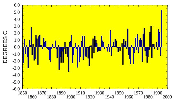
Figure 4.24 July temperature anomalies for Hamburg, Germany. Anomalies are departures from the 1961-1990 base period means. (Data supplied by the Deutscher Wetterdienst, Hamburg, Germany.)
