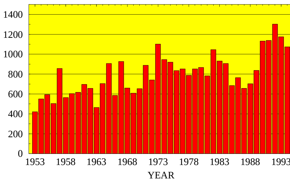
Figure 4.32 Annual number of observed tornadoes in the United States (1953-1994). (Data provided by the National Climate Data Center.)
