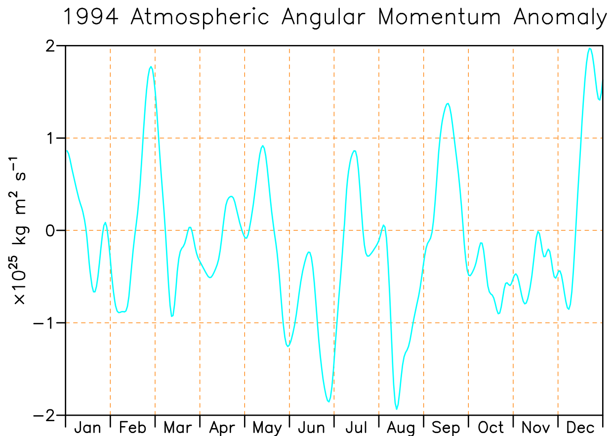
Figure 1.28 Departure of the 1994 daily atmospheric momentum values from the 15-year calendar mean. Values have been smoothed by a filter to damp fluctuations on periods shorter than about 8 days. (Source: Atmospheric and Environmental Research, Inc.)
