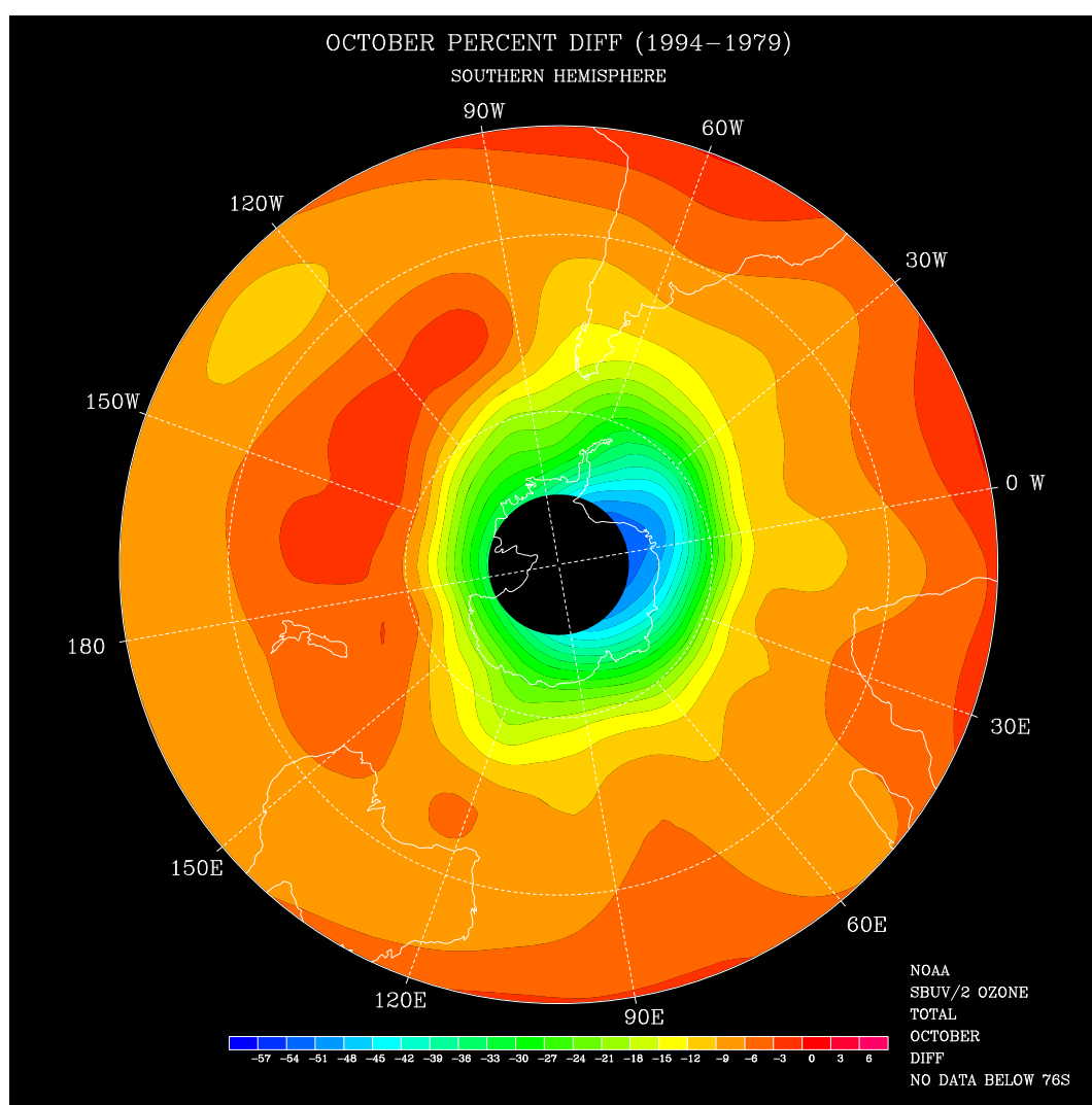
Figure 1.16 Total ozone percent difference between October 1994 and October 1979. Regions of no data are shown in black. (Source: CAC)
