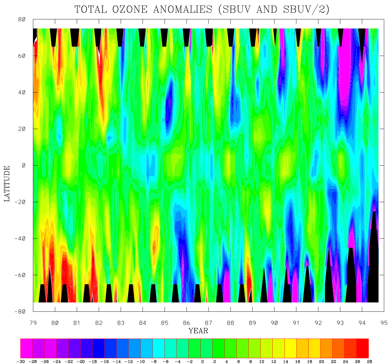
Figure 1.15 Time-latitude section of anomalous monthly average values (Dobson Units) of zonal mean total ozone, derived from Nimbus 7 SBUV from 1979-1988, and from NOAA 11 SBUV/2 from 1989 to 1994. Anomalies are departures from the 1979-1994 base period means. Regions of no data are shown in black. (Source: CAC)
