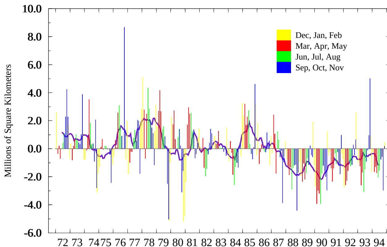
Figure 1.20 Anomalies of monthly snow cover extent over the Northern Hemisphere (including Greenland) between January 1972 and December 1994. Smoothed curve is a twelve-month running mean. Anomalies are departures from the 1972-1994 base period means. (Data provided by Rutgers University.)
