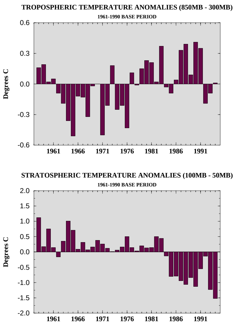
Figure 1.8 Annual global tropospheric (850-300 mb) (top) and stratospheric (100-50 mb) (bottom) temperature anomalies derived from radiosonde data based on a 63-station network. Anomalies are departures from the 1961-1990 base period means (Data provided by the Air Resources Laboratory.)
