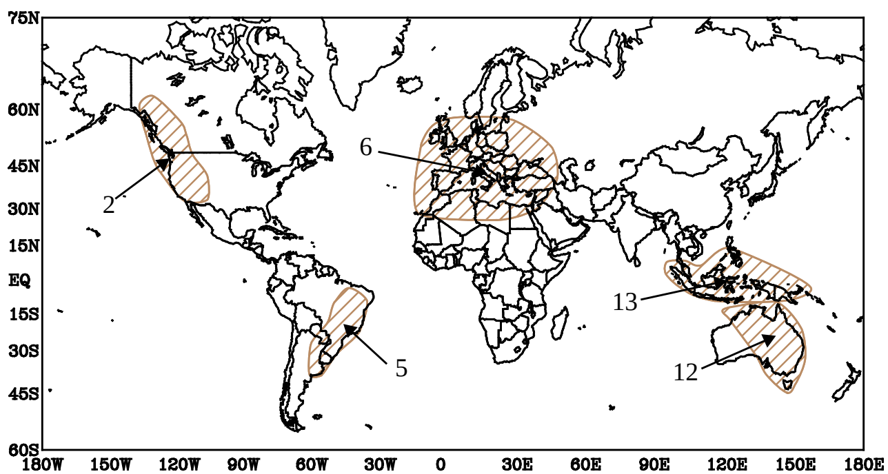
Figure 5.1 Significant above-normal precipitation anomalies (top) and below-normal precipitation anomalies (bottom) during 1994. The numbers are keyed to the descriptive paragraphs. (Source: CAC)
