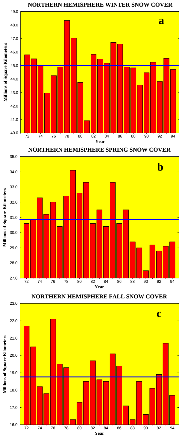
Figure 1.21 Time series of Northern Hemisphere snow-cover area ( 10^6 \text{ km}^2 ) for a) winter (December through February), b) spring (March - May), and c) fall (September - November) estimated from visual satellite imagery. The solid black line depicts normal seasonal snow cover area. (Data provided by NOAA/NESDIS and Rutgers University.)
