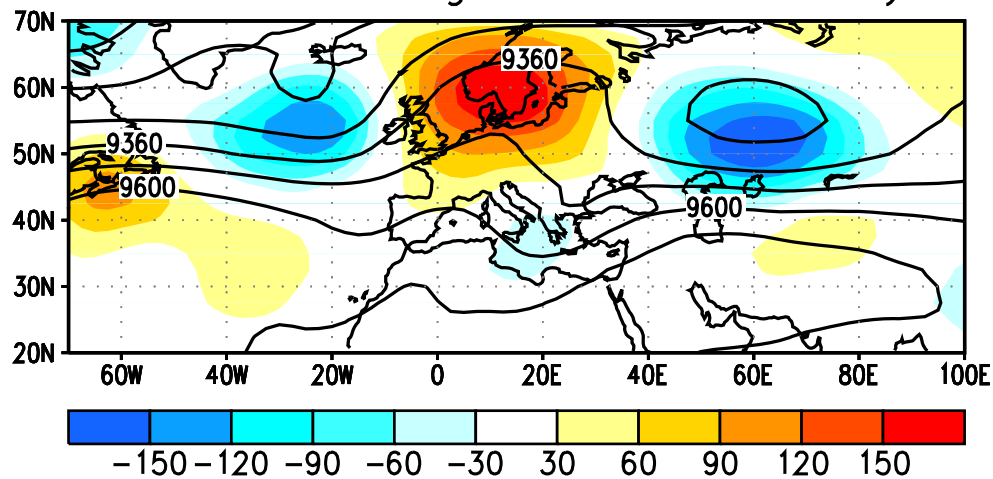
Figure 4.23 300-mb height (m) and anomaly (m) for July 1994. Anomalies are departures from the 1979-1988 base period means. (Source: CAC)
