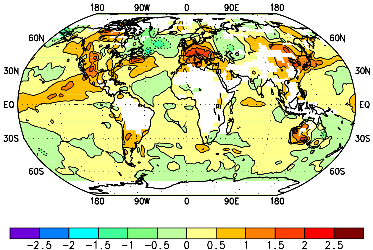
Figure 1.4 Surface temperature anomalies ( ^{\circ}\text{C} ) for January - December 1994. Analysis is based on station data over land and on sea surface temperature (SST) data over the oceans. Anomalies for station data are departures from the 1961-1990 base period means, while SST anomalies are departures from the COADS/ICE climatology (Reynolds 1988). White areas are regions with insufficient data for analysis. (Source: CAC)
