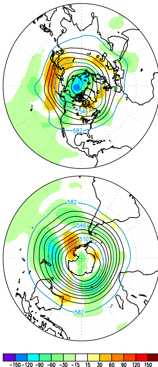
Figure 3.9 Northern Hemisphere (top) and Southern Hemisphere (bottom) 500-mb geopotential height (contours, interval is 9 dm) and anomalies (shading, in m) for September - November 1994. Anomalies are departures from the 1979-1988 base period means. (Source: CAC)
