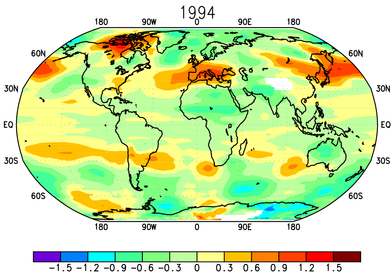
Figure 1.9 Mean annual tropospheric temperature anomalies for 1994 derived from the Microwave Sounding Unit (MSU) channel 2R. Anomalies are departures from the 1982-1991 base period means. (Data provided by the University of Alabama at Huntsville.)
