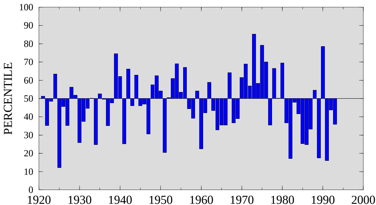
Figure 4.4 Precipitation index (average gamma percentiles of station precipitation within the region) for northeastern Australia for October - April. Percentiles are computed for the 1961-1990 base period. (Source: CAC)
