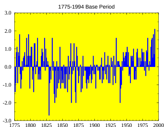
Figure 4.20 Annual temperature anomalies (°C) for Vienna, Austria. Anomalies are departures from the 1775-1994 base period means. (Data supplied by the Deutscher Wetterdienst, Hamburg, Germany.)
