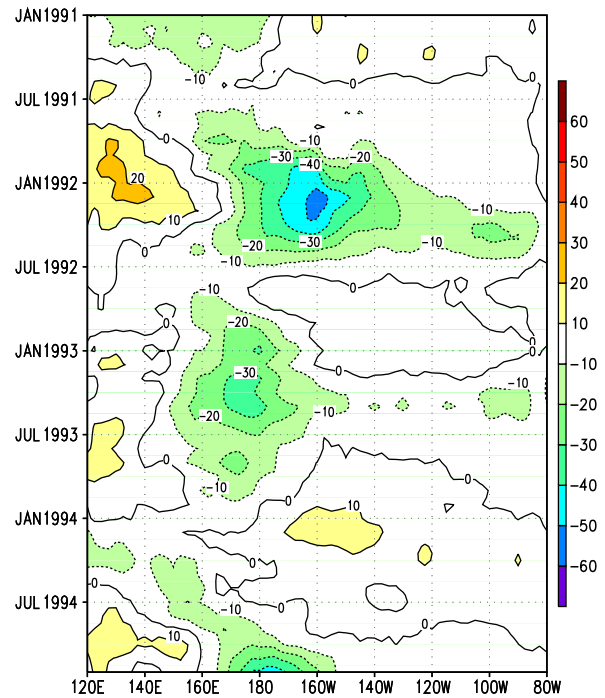
Figure 2.6 Time-longitude section of anomalous outgoing longwave radiation (OLR) \text{Wm}^{-2} averaged from 5^{\circ}\text{N} - 5^{\circ}\text{S} . Anomalies are departures from the 1979-1988 base period means. (Source: CAC)
