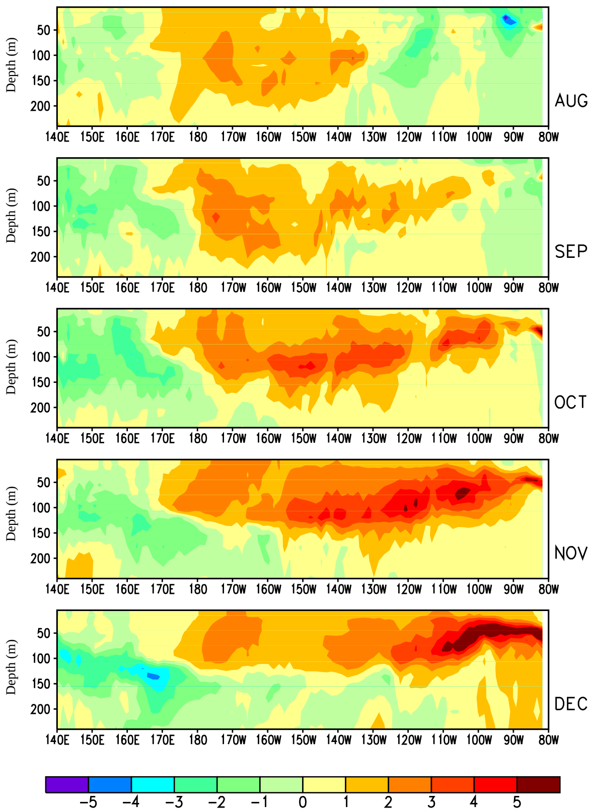
Figure 2.11 Equatorial depth-longitude section of monthly mean ocean temperature anomalies for August through December 1994. Data are derived from an analysis system that assimilates oceanic observations into an oceanic GCM ( Leetmaa and Ji 1989 ). Contour interval is 1°C. Anomalies are departures from the 1983-1992 base period means. (Data provided by the NMC Coupled Model Project.)
