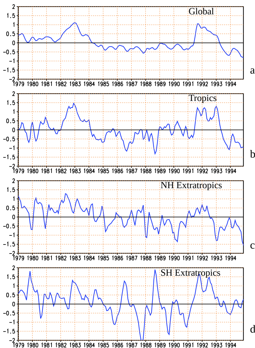
Figure 1.11 Mean stratospheric temperature anomalies ( ^{\circ}\text{C} ) from the Microwave Sounding Unit (MSU) channel 4 for the a) globe ( 85^{\circ}\text{S} - 85^{\circ}\text{N} ), b) tropics ( 30^{\circ}\text{N} - 30^{\circ}\text{S} ), c) Northern Hemisphere extratropics ( 30^{\circ}\text{N} - 85^{\circ}\text{N} ) and d) Southern Hemisphere extratropics ( 30^{\circ}\text{S} - 85^{\circ}\text{S} ). Anomalies are departures from the 1982-1991 base period monthly means. (Data provided by the University of Alabama at Huntsville.)
