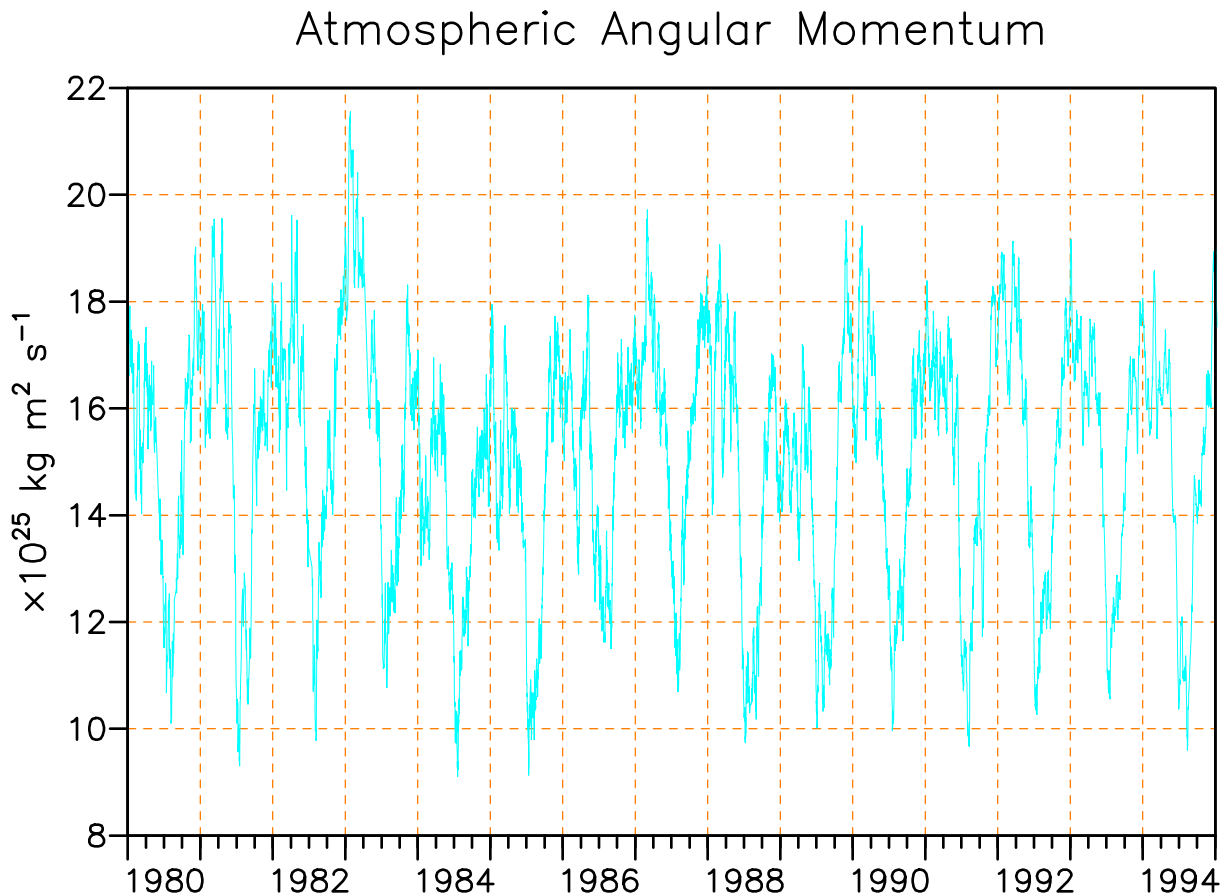
Figure 1.27 Global relative angular momentum of the atmosphere about the Earth's rotation axis during the period 1980-1994, as determined from the National Meteorological Center's daily zonal wind analyses between 50 and 1000 mb. (Source: Atmospheric and Environmental Research, Inc.)
