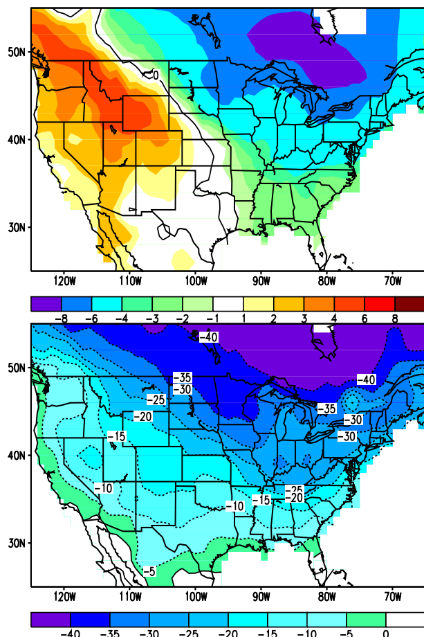
Figure 3.3 Temperature anomalies (top) and extreme minimum temperature (bottom) in °C for the period 23 December 1993-22 January 1994. (Source: CAC)
