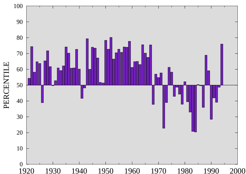
Figure 4.19 Precipitation index (average gamma percentiles of station precipitation within the region) for the western Sahel for August - September normalized by the 1961-1990 base period. (Source: CAC)
