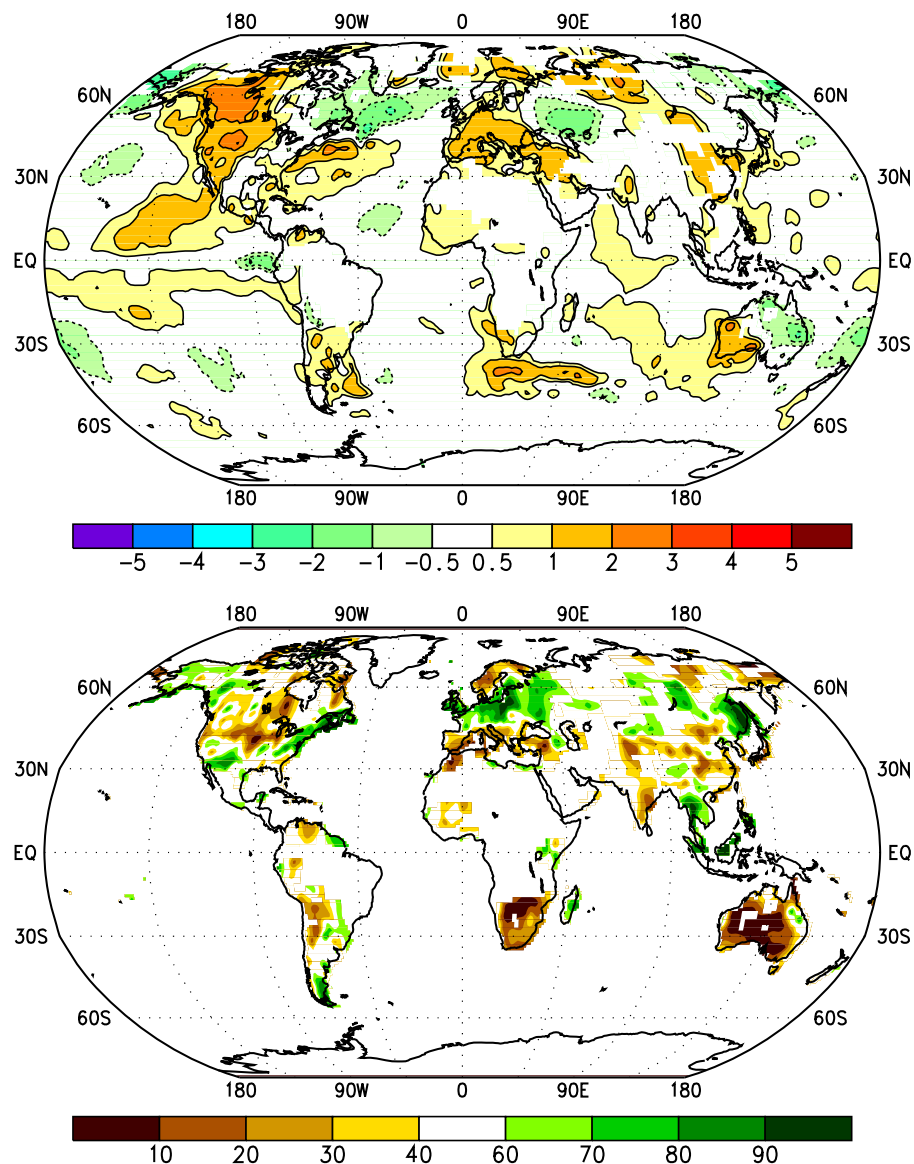
Figure 3.6 Surface temperature anomalies (°C) (top) and precipitation percentiles based on a gamma distribution fit to the 1961-1990 base period (bottom) for March - May 1994. Temperature anomalies are based on station data over land (1961-1990 base period) and sea surface temperature data (SST) over water (COADS/ICE climatology). Analysis omitted in data-sparse regions. (Source: CAC)
