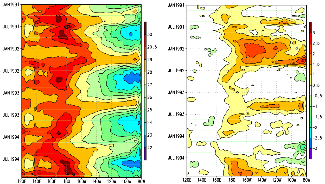
Figure 2.4 Time-longitude section of mean (left) and anomalous (right) sea surface temperature (SST) (°C) averaged from 5°N-5°S. Anomalies are departures from the adjusted OI climatology ( Reynolds and Smith 1995 ). (Data provided by the NMC Coupled Model Project.)
