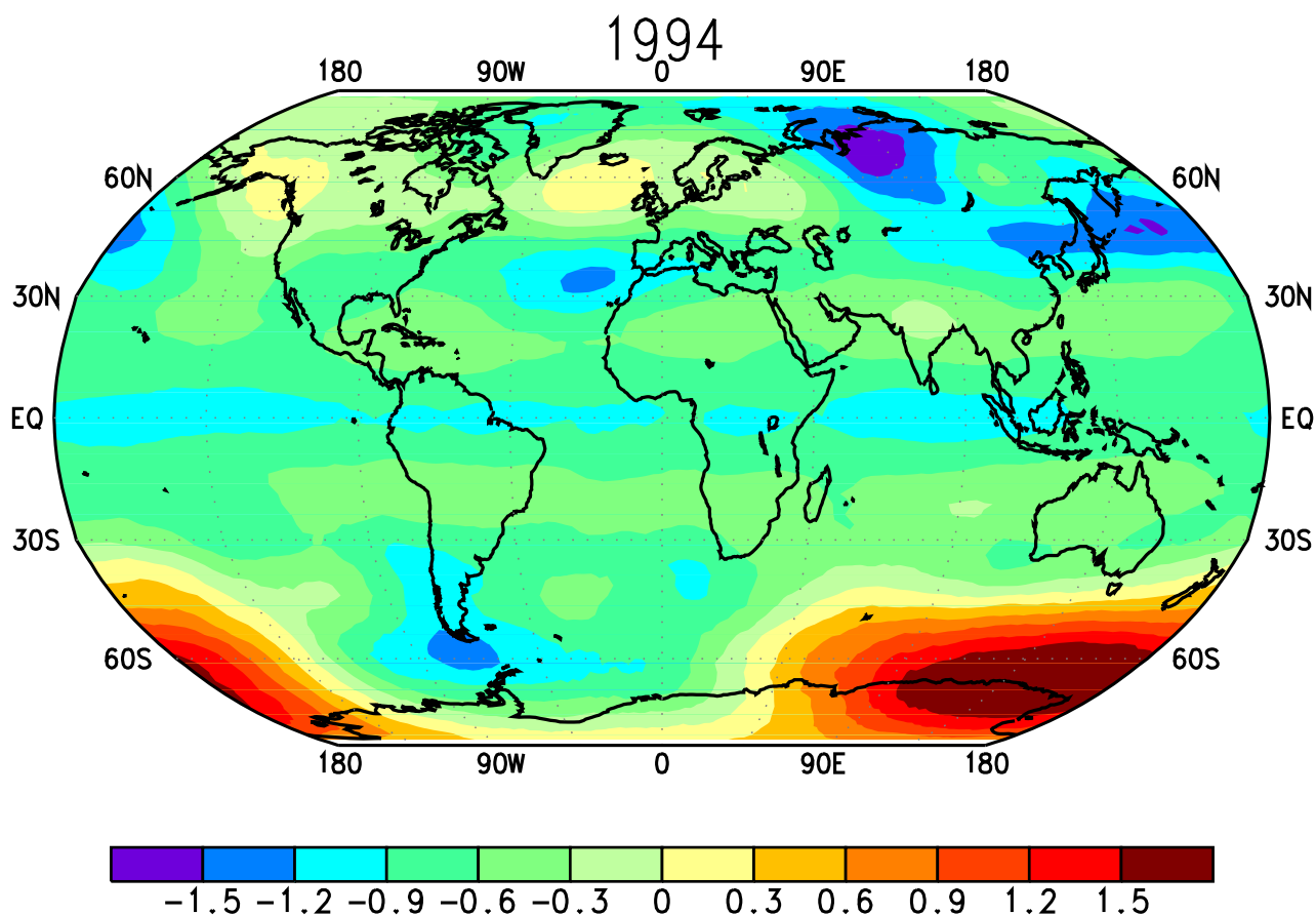
Figure 1.12 Mean annual stratospheric temperature anomalies for 1994 derived from the Microwave Sounding Unit (MSU) channel 4. Anomalies are departures from the 1982-1991 base period means. (Data provided by the University of Alabama at Huntsville.)
