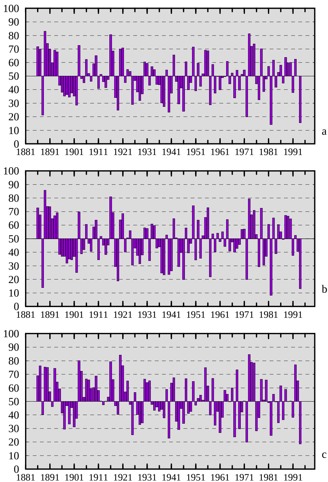
Figure 4.7 Precipitation index (average gamma percentiles of station precipitation within the region) for April - December for (a) Australia (south of 20°S), (b) eastern Australia and (c) central/western Australia. Percentiles are computed for the 1961-1990 base period means. (Source: CAC)
