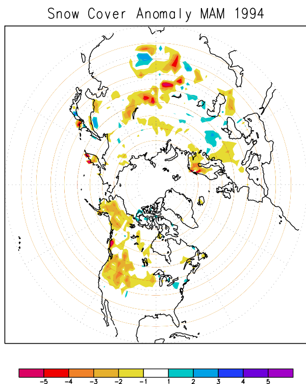
Figure 1.23 Spring (March - May) 1994 snow-cover anomaly in weeks, derived from subjective analysis of visual satellite imagery by NOAA/NESDIS. Anomalies are departures from the 1973-1993 base period. (Source: CAC)
