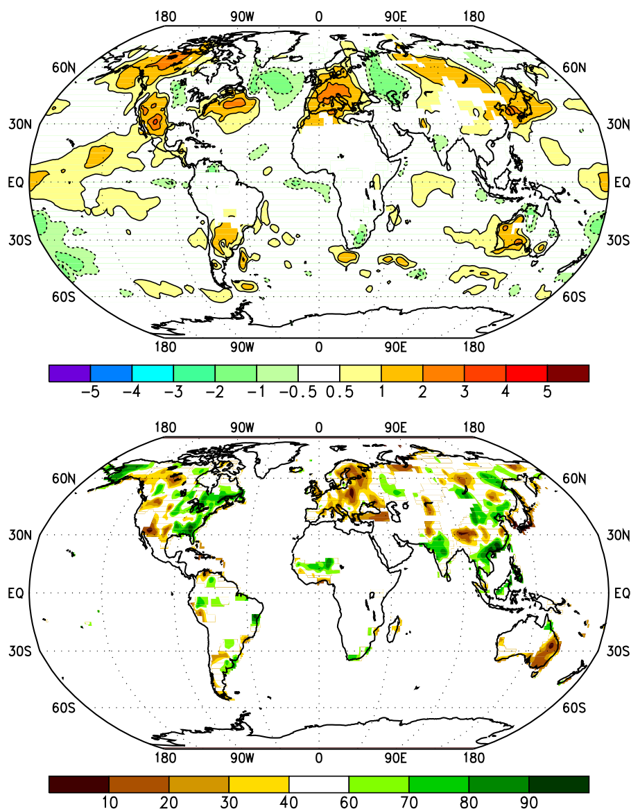
Figure 3.8 Surface temperature anomalies (°C) (top) and precipitation percentiles based on a gamma distribution fit to the 1961-1990 base period (bottom) for June - August 1994. Temperature anomalies are based on station data over land (1961-1990 base period) and sea surface temperature data (SST) over water (COADS/ICE climatology). Analysis omitted in data-sparse regions. (Source: CAC)
