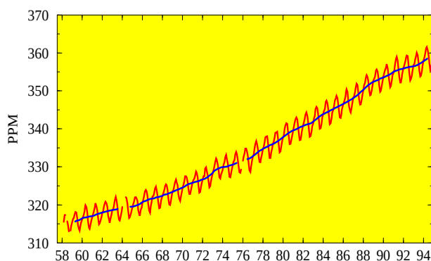
Figure 1.18 Monthly mean (red line) carbon dioxide concentrations (ppm) measured at Mauna Loa, Hawaii, 1958-1994. Blue line is the twelve-month running mean. The data through 1973 are from C. D. Keeling at Scripps Institute of Oceanography. (Data provided by the Climate Monitoring and Diagnostics Laboratory.)
