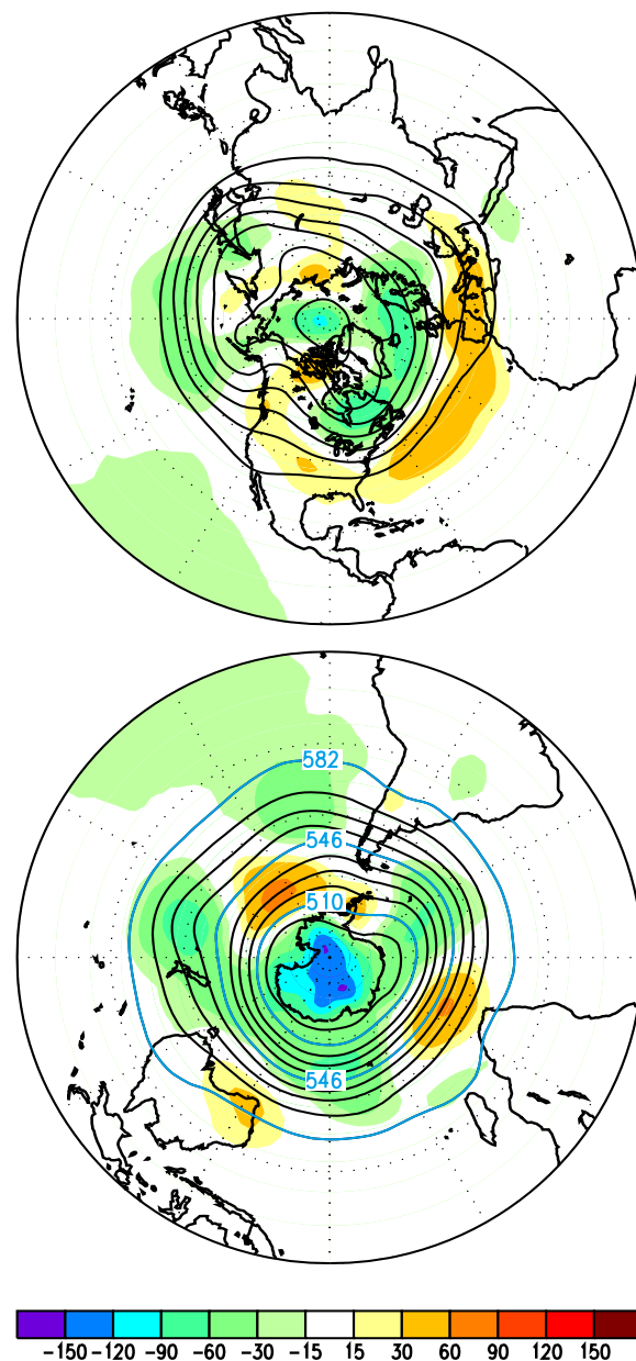
Figure 3.5 Northern Hemisphere (top) and Southern Hemisphere (bottom) 500-mb geopotential height (contours, interval is 9 dm) and anomalies (shading, in m) for March - May 1994. Anomalies are departures from the 1979-1988 base period means. (Source: CAC)
