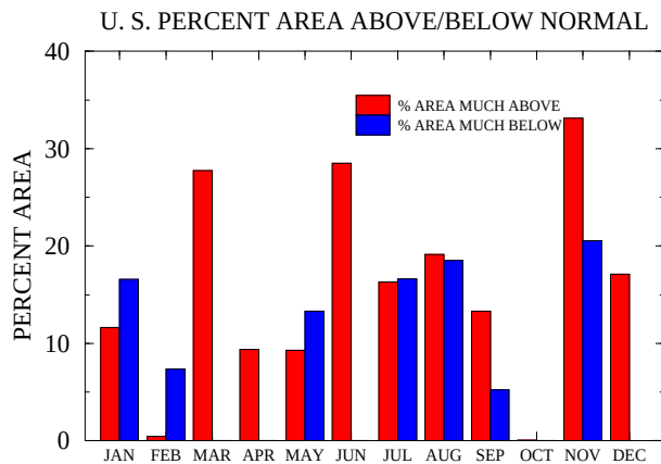
Figure 4.29 Percent area of the contiguous United States experiencing monthly mean temperatures in the upper and lower tenth percentile. (Data provided by the National Climate Data Center.)
