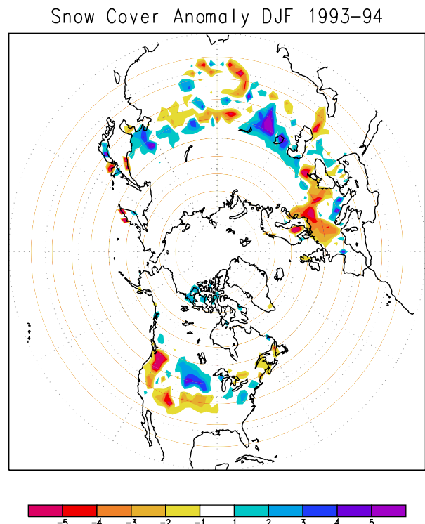
Figure 1.22 Winter (December 1993 - February 1994) snow-cover anomaly in weeks, derived from subjective analysis of visual satellite imagery by NOAA/NESDIS. Anomalies are departures from the 1973-1993 base period. (Source: CAC)
