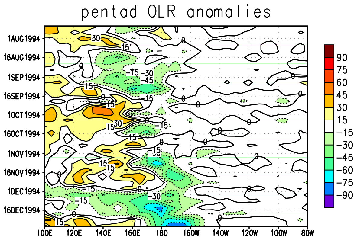
Figure 2.13 Time-longitude section of pentad anomalous outgoing longwave radiation (OLR) averaged for 5°N-5°S. Contour interval is 15 \text{Wm}^{-2} . Anomalies are departures from the 1979-1988 base period pentad means. (Source: CAC)
