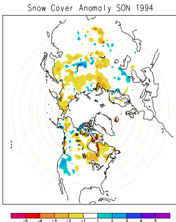
Figure 1.24 Fall (September - November) 1994 snow-cover anomaly in weeks, derived from subjective analysis of visual satellite imagery by NOAA/NESDIS. Anomalies are departures from the 1973-1993 base period. (Source: CAC)
