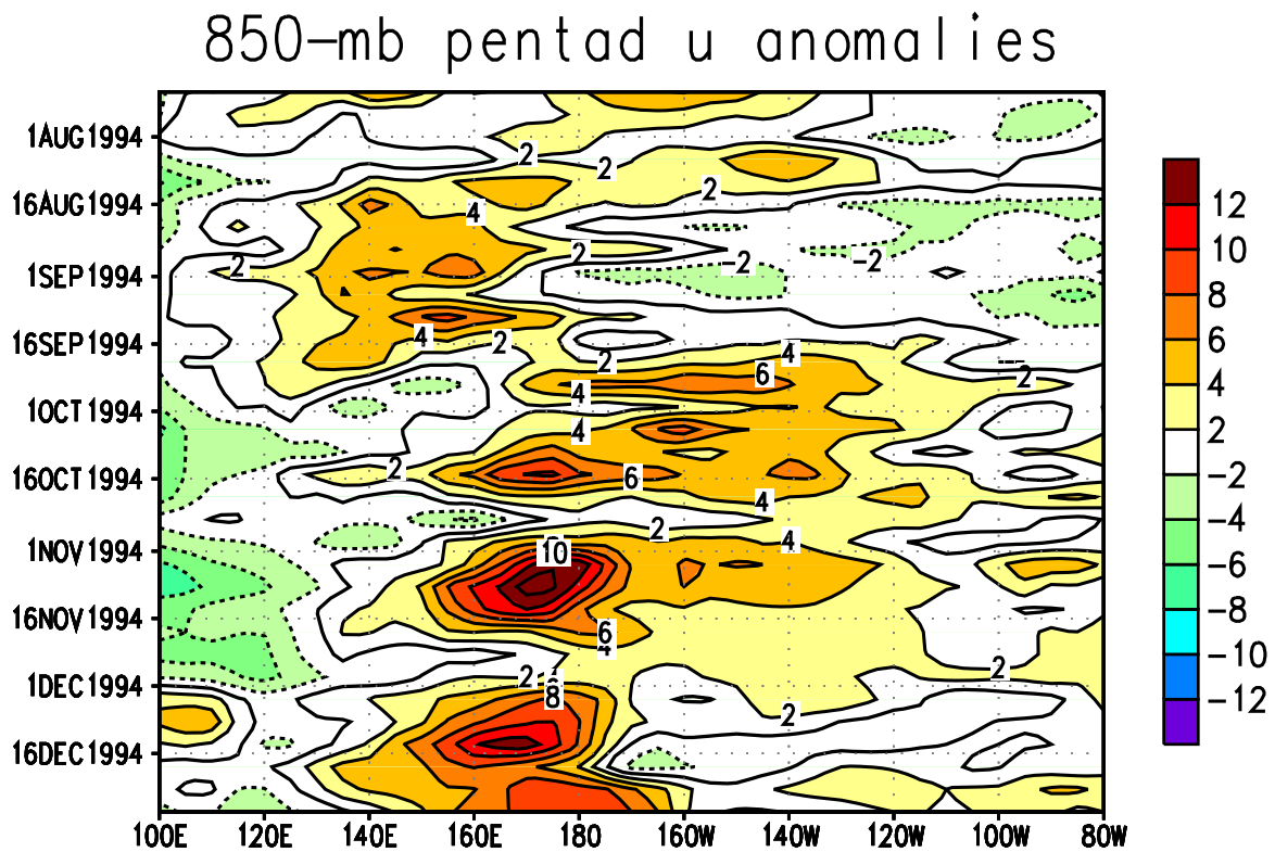
Figure 2.12 Time-longitude section of pentad mean (top) and anomalous (bottom) 850-mb zonal wind averaged for 5°N-5°S. Contour interval is 2 \text{m s}^{-1} . Anomalies are departures from the 1979-1988 base period pentad means. (Source: CAC)
