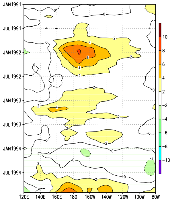
Figure 2.5 Time-longitude section of anomalous 850-mb zonal wind ( \text{ms}^{-1} ) averaged from 5^{\circ}\text{N} - 5^{\circ}\text{S} . Anomalies are departures from the 1979-1988 base period means. (Source: CAC)
