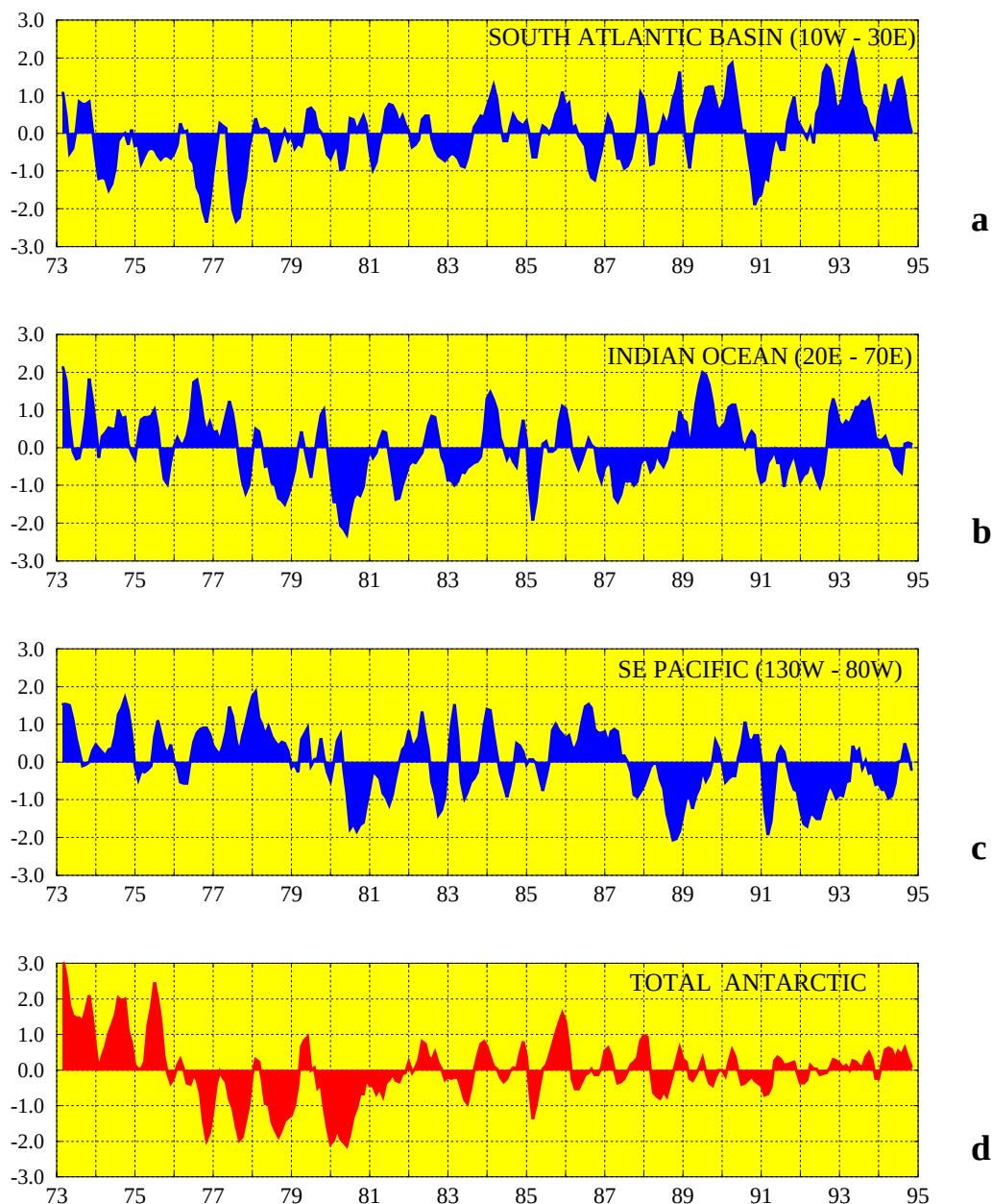
Figure 1.26 Standardized sea-ice area anomalies for the a) South Atlantic Basin, b) Indian Ocean, c) Southeast Pacific, and d) Total Antarctic. Values are standardized by the standard deviation for the 1973-1994 period. (Source: CAC)
