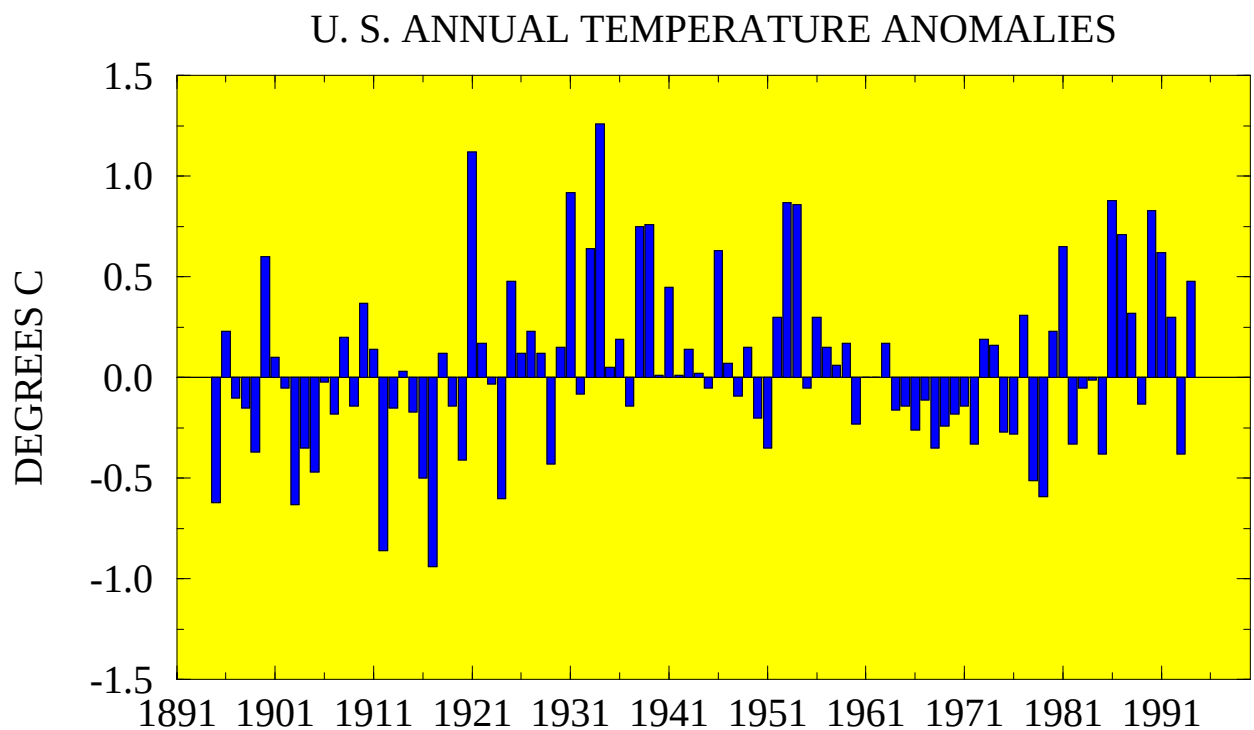
Figure 4.28 Annual surface temperature anomalies (°C) for the contiguous United States. Anomalies are departures from the 1961-1990 base period means. (Data provided by the National Climate Data Center.)
