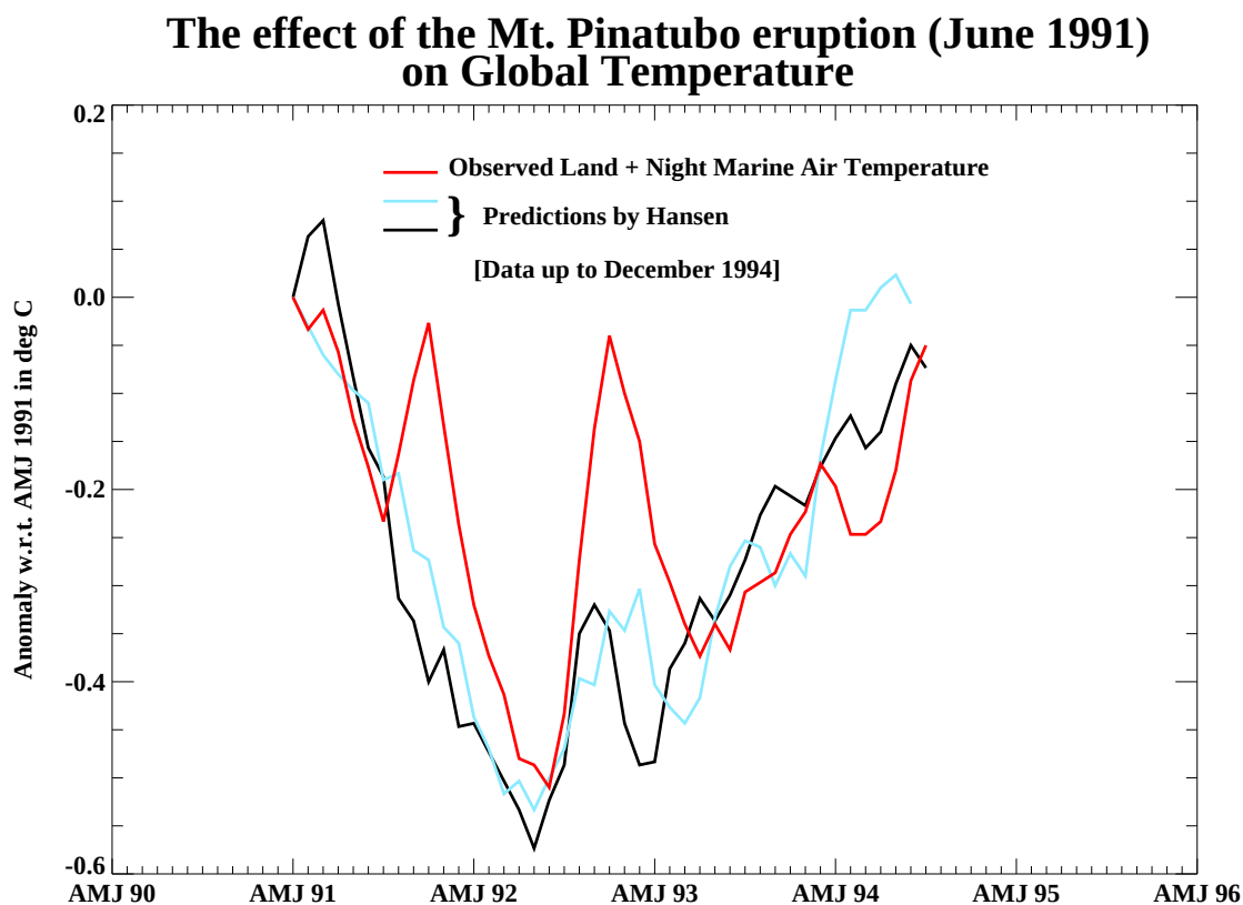
Figure 1.6 Global surface air temperature anomalies (red line) following the June 1991 eruption of Mt. Pinatubo, relative to the global anomaly for the 3-month period April-June 1991. Values are 3-month running mean anomalies ending with October - December 1994. Model results are indicated by blue and black lines. (Source: Hadley Centre for Climate Prediction and Research, UK)
