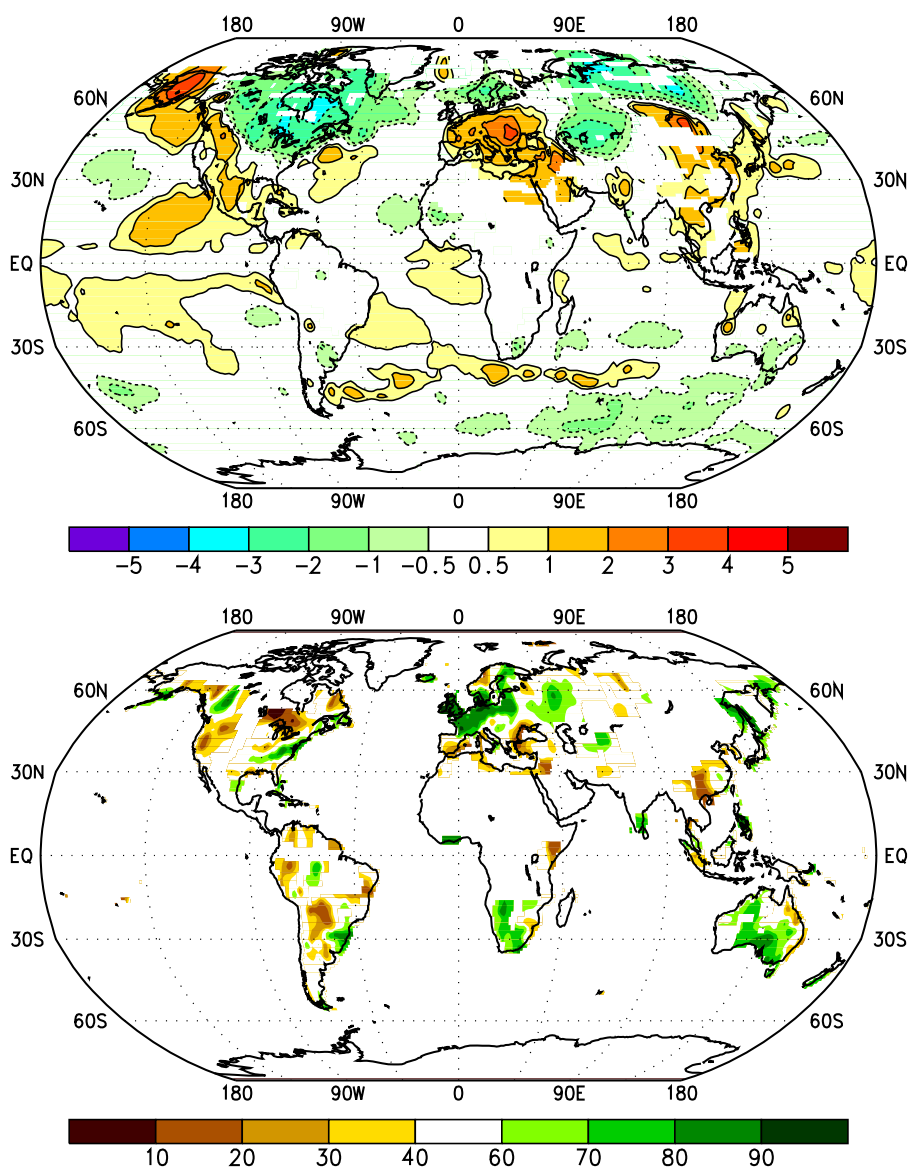
Figure 3.2 Surface temperature anomalies (°C) (top) and precipitation percentiles based on a gamma distribution fit to the 1961-1990 base period (bottom) for December 1993 - February 1994. Temperature anomalies are based on station data over land (1961-1990 base period) and sea surface temperature data (SST) over water (COADS/ICE climatology). Analysis omitted in data-sparse regions. (Source: CAC)
