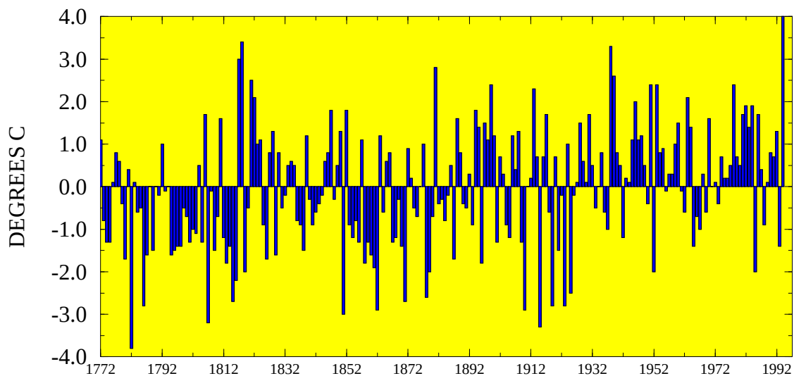
Figure 4.27 November temperature anomalies (°C) for central England. Anomalies are departures from the 1772-1994 base period means. (Data provided by the Hadley Centre for Climate Prediction and Research, UK.)
