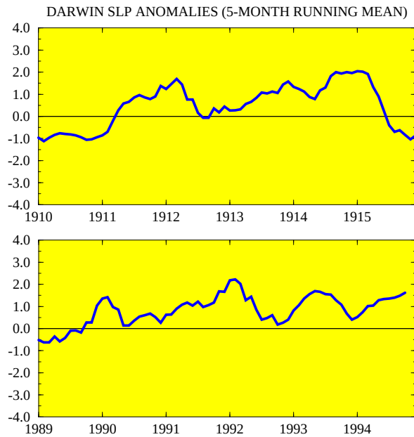
Figure 2.7 Five-month running mean of SLP anomalies (mb) at Darwin, Australia for 1910-1915 (top) and 1989-1994 (bottom). Anomalies are departures from the 1951-1980 base period monthly means. (Source: CAC)
