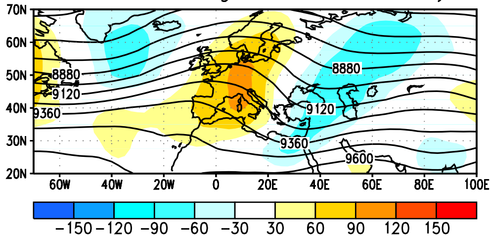
Figure 4.26 300-mb height (m) and anomaly (m) for November-December 1994. Anomalies are departures from the 1979-1988 base period means. (Source: CAC)
