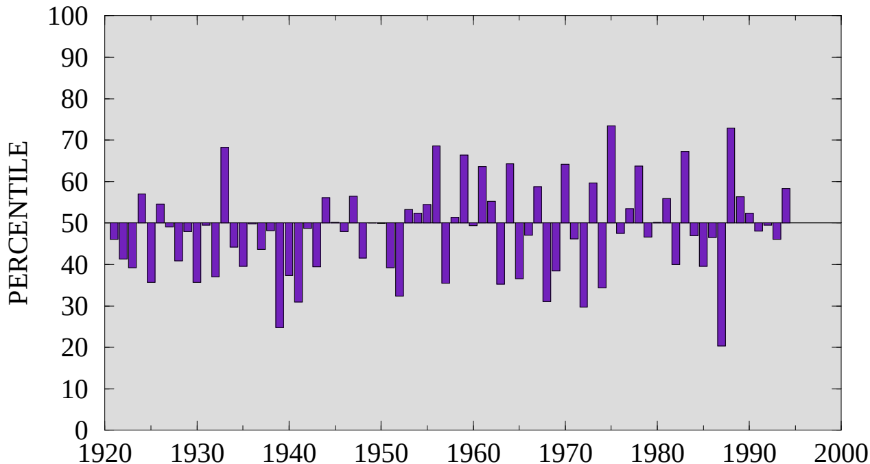
Figure 4.13 Precipitation index (average gamma percentiles of station precipitation within the region) for India for June - September. Percentiles are computed for the 1961-1990 base period. (Source: CAC)
