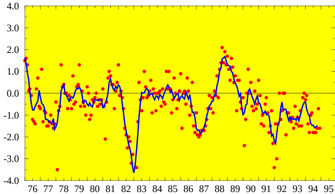
Figure 2.3 Five-month running mean of the Southern Oscillation Index (SOI). The SOI is computed as the standardized difference between the standardized pressure anomalies at Tahiti and Darwin (Tahiti minus Darwin). Individual monthly values are indicated by red dots. (Source: CAC)
