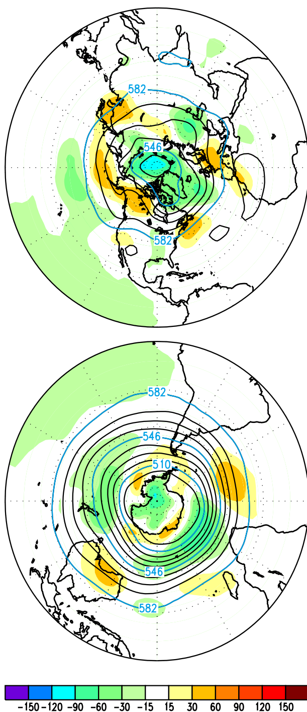
Figure 3.7 Northern Hemisphere (top) and Southern Hemisphere (bottom) 500-mb geopotential height (contours, interval is 9 dm) and anomalies (shading, in m) for June - August 1994. Anomalies are departures from the 1979-1988 base period means. (Source: CAC)
