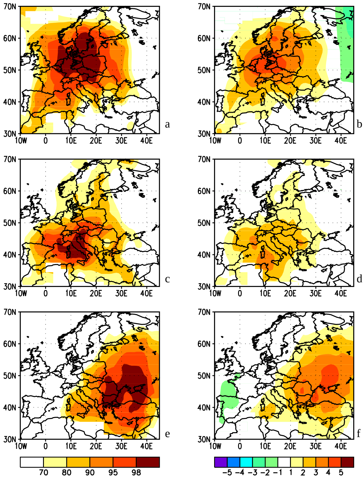
Figure 4.22 Temperature percentiles (a, c, e) and anomalies ( ^{\circ}\text{C} ) (b, d, f) for July (a, b), August (c, d) and September (e, f) 1994. Anomalies are departures from the 1961-1990 base period means. (Source: CAC)
