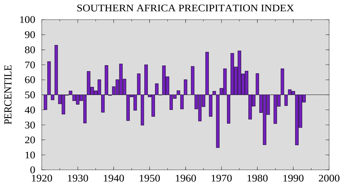
Figure 4.1 Precipitation index (average gamma percentiles of station precipitation within the region) for southern Africa for October - April. Percentiles are computed for the 1961-1990 base period. (Source: CAC)
