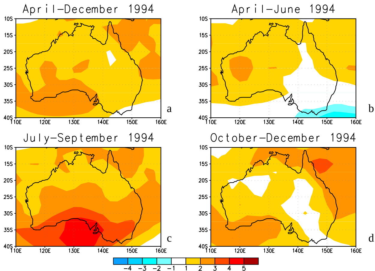
Figure 4.8 Sea level pressure anomalies over Australia for (a) April-December 1994, (b) April-June 1994, (c) July-September 1994, and (d) October-December 1994. Anomalies are departures from the 1979-1988 base period means. (Source: CAC)
