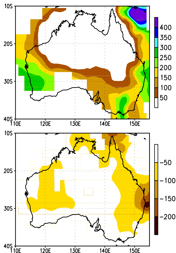
Figure 4.9 Total precipitation (mm, top) and anomalies (mm, bottom) during April - June 1994. Anomalies are departures from the 1961-1990 base period means. (Source: CAC)
