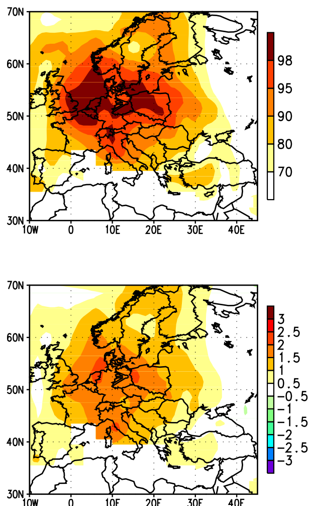
Figure 4.21 Temperature percentiles (top) and anomalies (°C) (bottom) for July - December 1994. Anomalies are departures from the 1961-1990 base period means. (Source: CAC)
