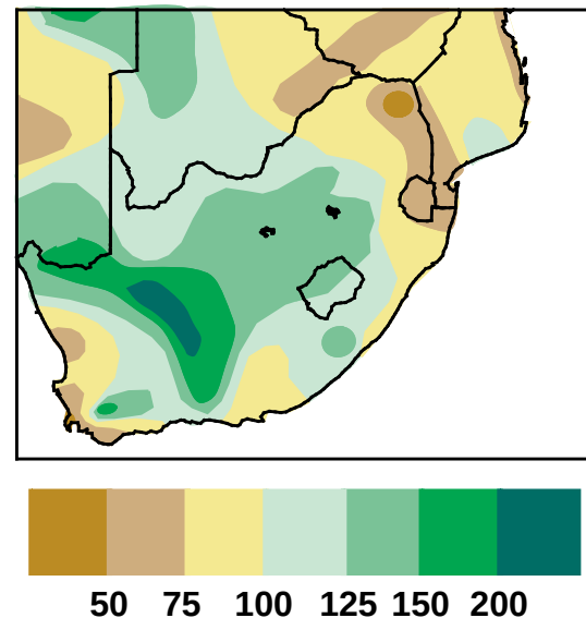
Figure 4.3 Percent of normal precipitation in southern Africa for October 1993 - April 1994, relative to the 1961-1990 base period. (Source: CAC)
