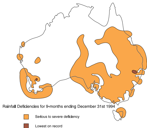
Figure 4.6 Rainfall deficiencies for April - December 1994. (Source: Australian Bureau of Meteorology)
