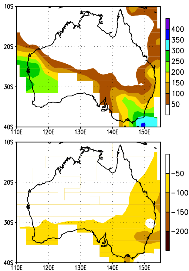
Figure 4.11 Total precipitation (mm, top) and anomalies (mm, bottom) during July - September 1994. Anomalies are departures from the 1961-1990 base period means. (Source: CAC)
