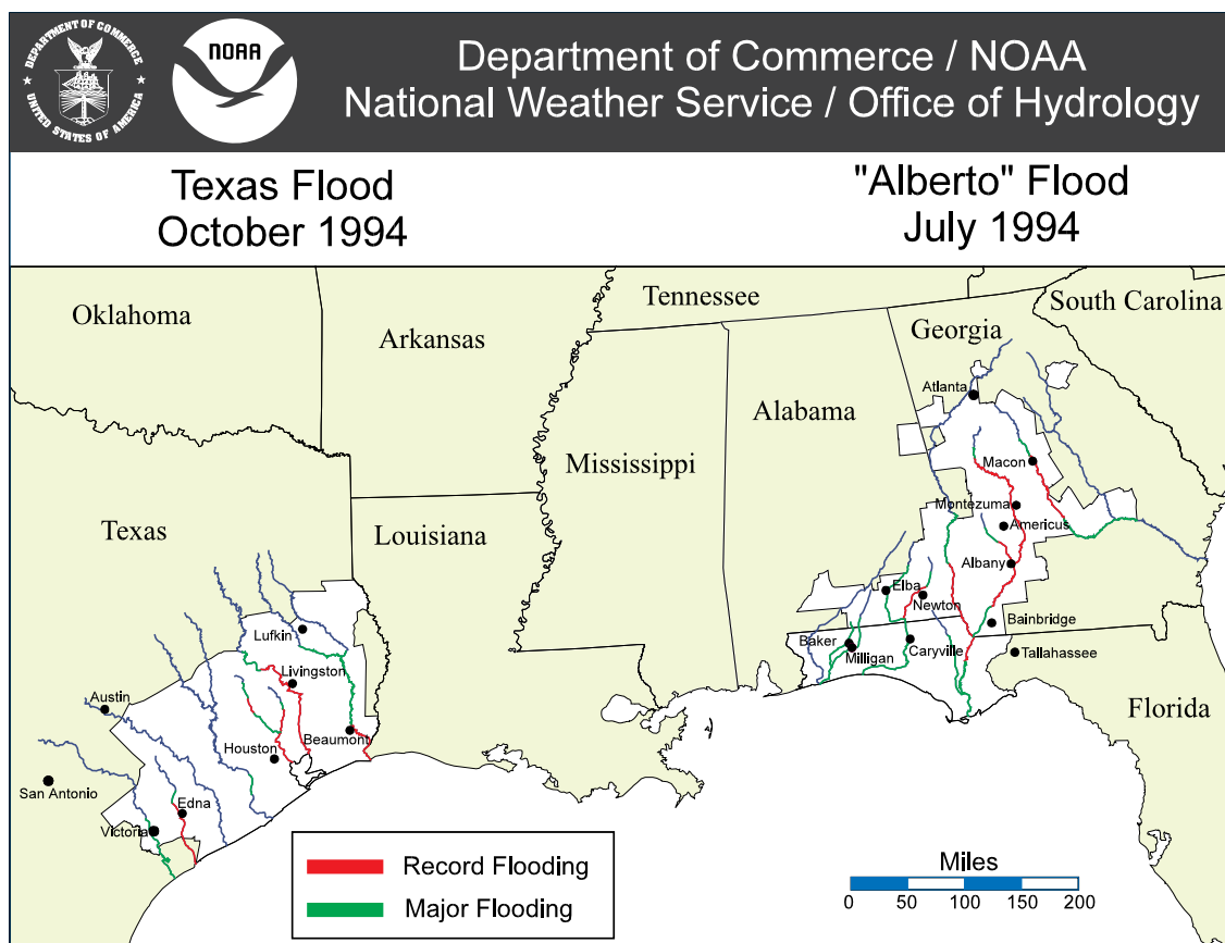
Figure 4.30 Major U. S. hydrologic events of 1994, showing: 1) the July 1994 flooding in the Southeast resulting from Tropical Storm "Alberto" and its remnants, and 2) the October 1994 flooding in Texas. Counties declared Federal disaster areas are colored white. (Source: Office of Hydrology)
