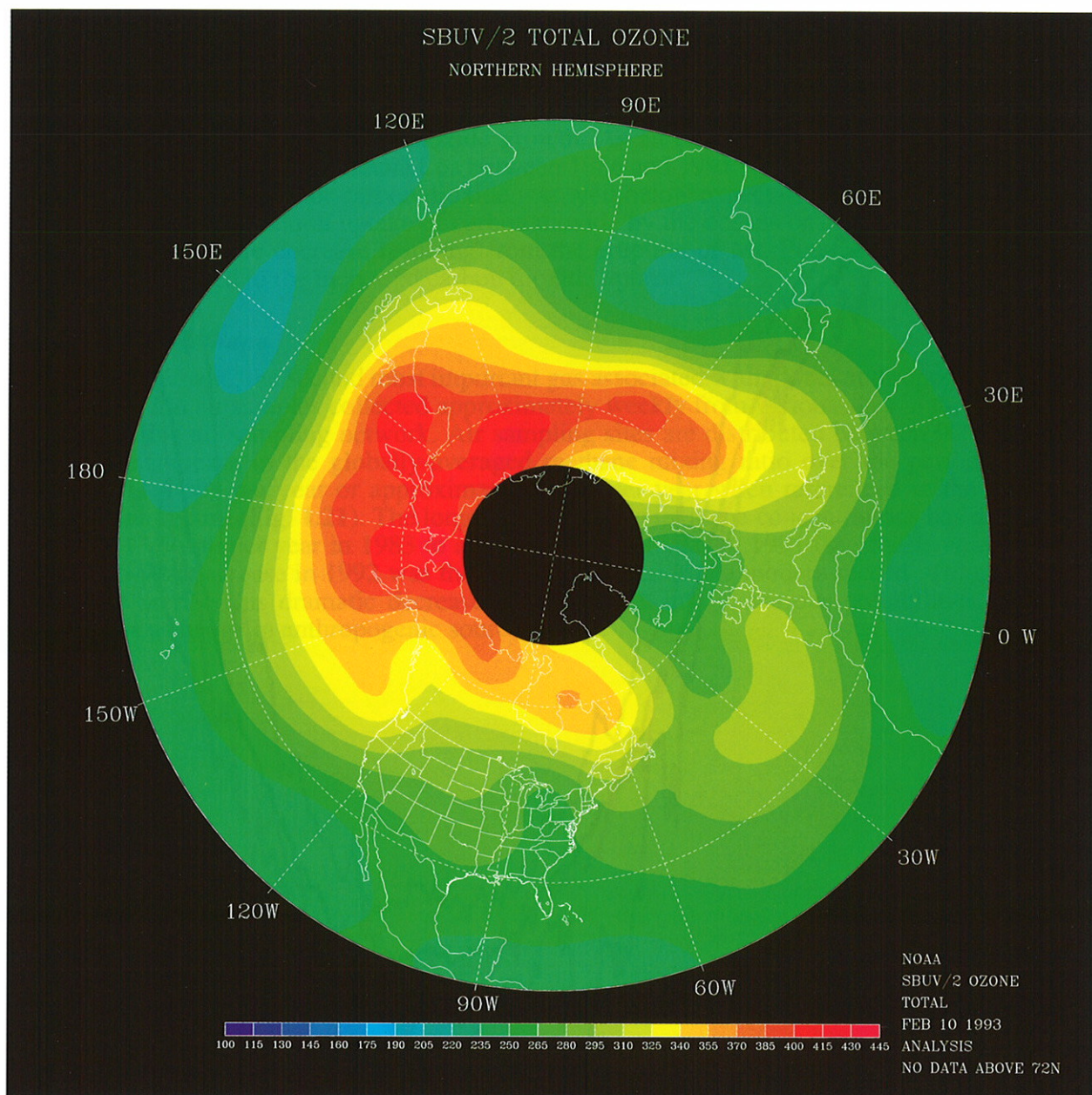
Figure 1.18 Northern Hemisphere NOAA-11 SBUV/2 total ozone (DU) for 10 February 1993. Areas of lowest ozone are shown in blue and purple, with highest values in yellow and red. Regions of no data are shown in black. (Source: CAC)
