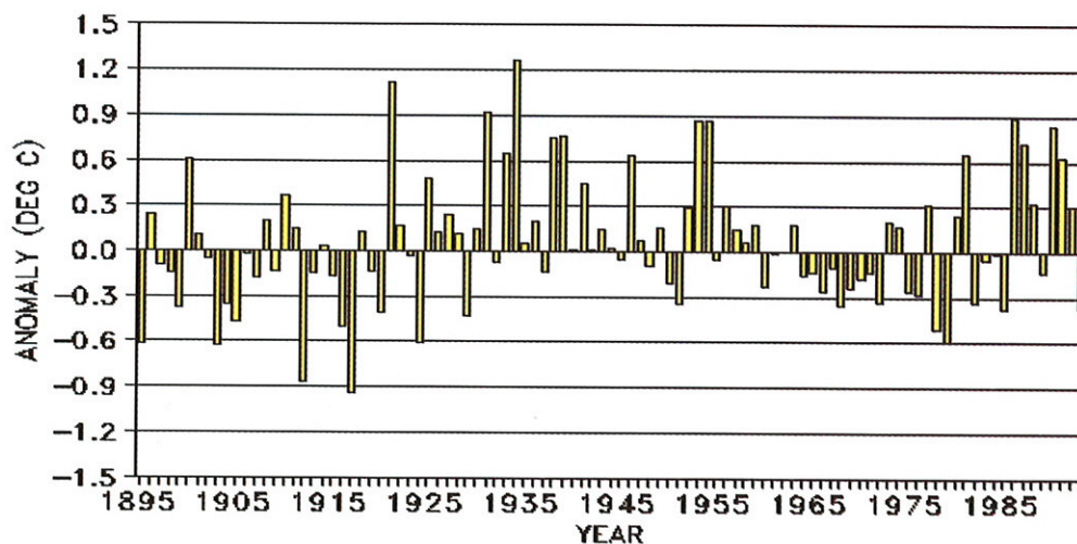
Figure 3.31 Annual surface temperature anomalies ( ^{\circ}\text{C} ) for the contiguous United States. Anomalies are computed from the 1961-1990 base period. (Source: NCDC)
