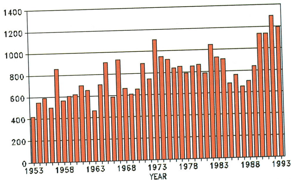
Figure 3.34 Annual number of observed tornadoes in the United States (1953-1993). (Source: NCDC)
