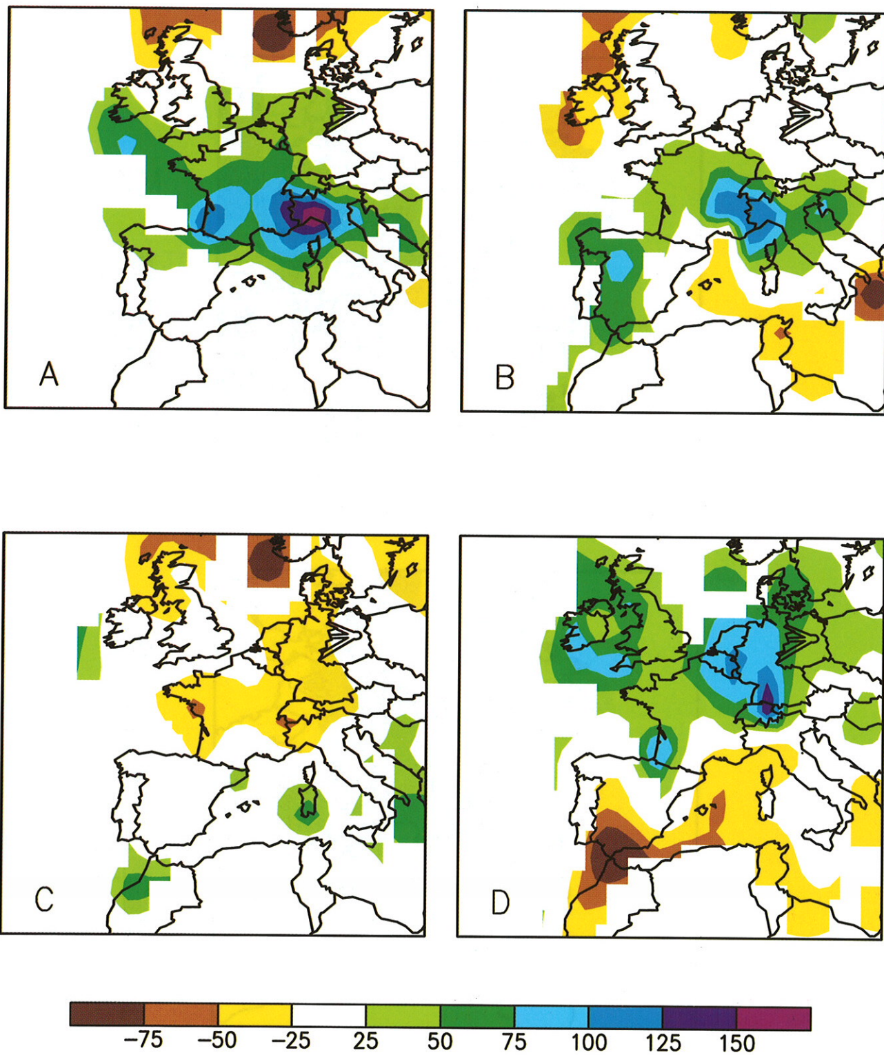
Figure 3.30 Anomalous precipitation (mm) for (a) September, (b) October, (c) November, and (d) December 1993. (Source: CAC)
