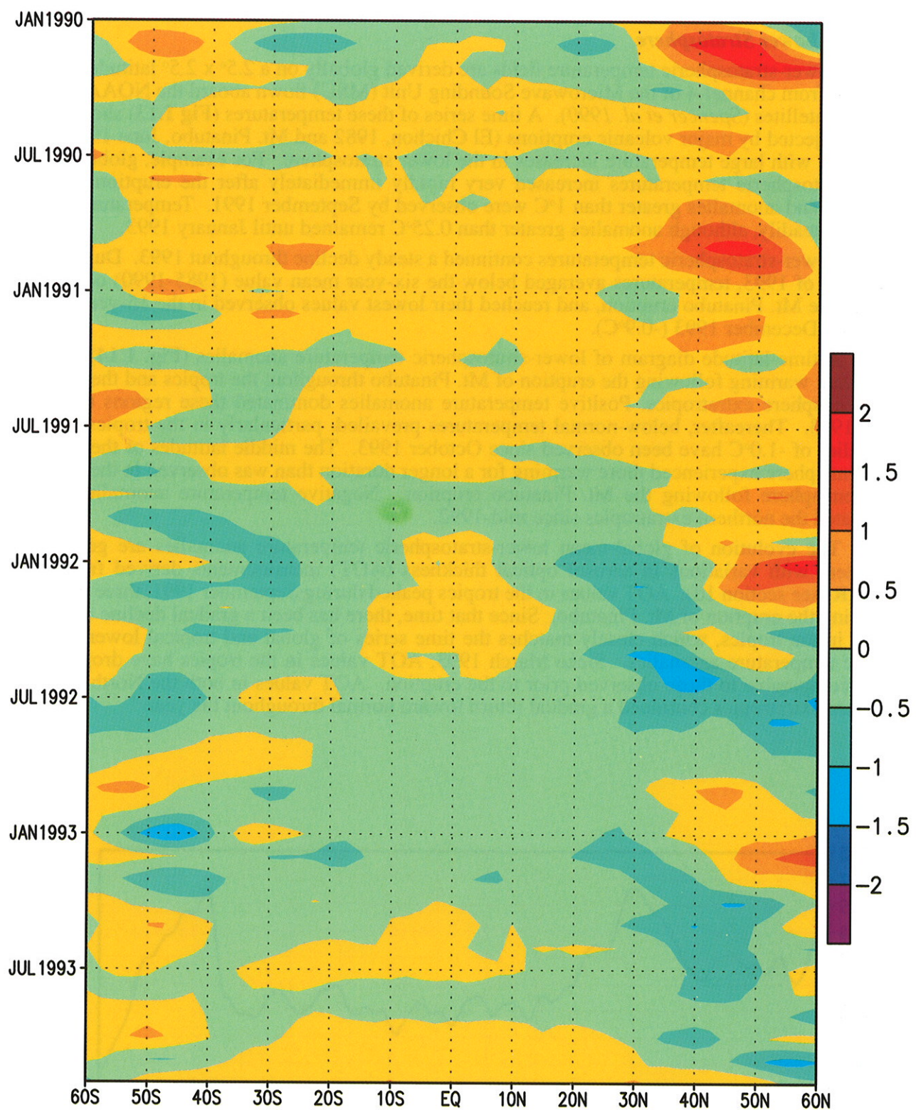
Figure 1.12 Time-latitude cross-section of zonally-averaged mean tropospheric temperature anomalies ( ^{\circ}\text{C} ) from the Microwave Sounding Unit (MSU) channel 2r. Anomalies are computed from the 1982-1991 base period. (Data provided by R. W. Spencer and J. R. Christy.)
