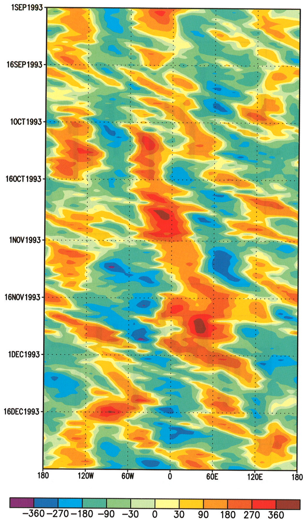
Figure 3.28 Time-longitude section of 500-mb height anomalies (m) during September - December 1993 averaged over the 5° latitude band centered on 60°N. (Source: CAC)
