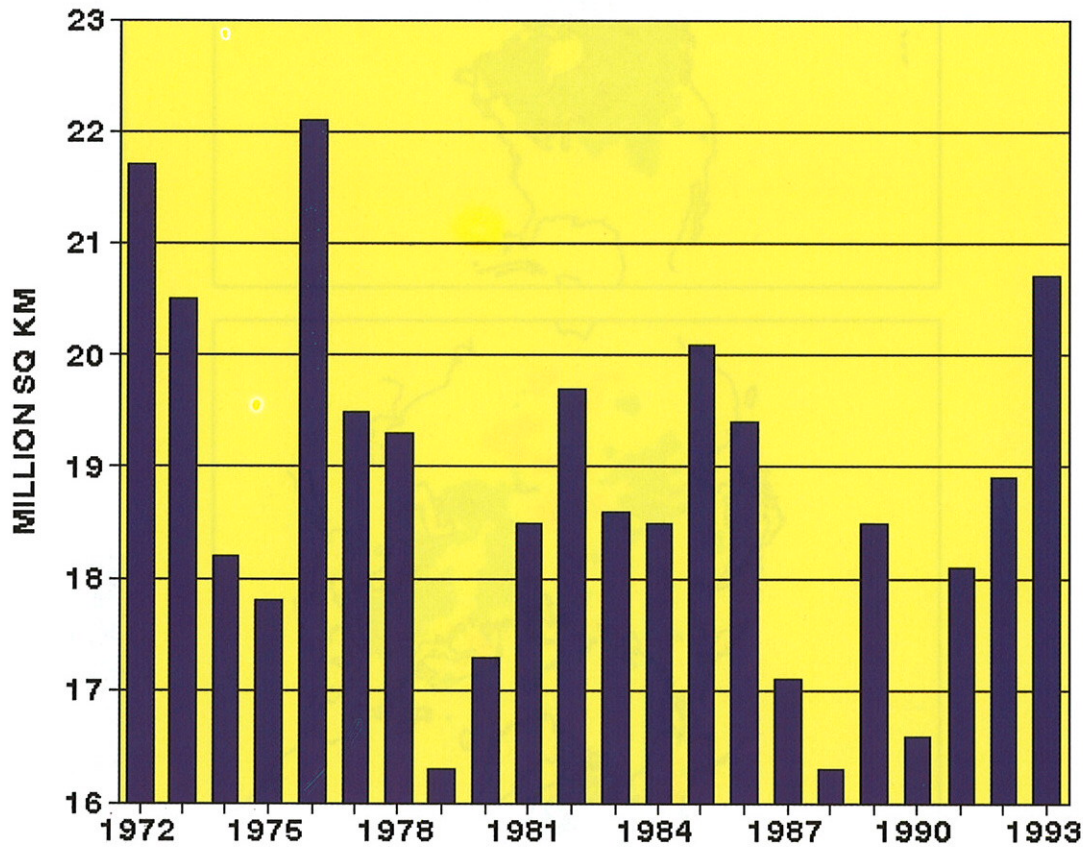
Figure 1.28 Time series of Northern Hemisphere snow-cover area ( 10^6 \text{ km}^2 ) for fall (September through November), estimated from satellite imagery. (Data provided by NOAA/NESDIS and D. Robinson, Rutgers University.)
