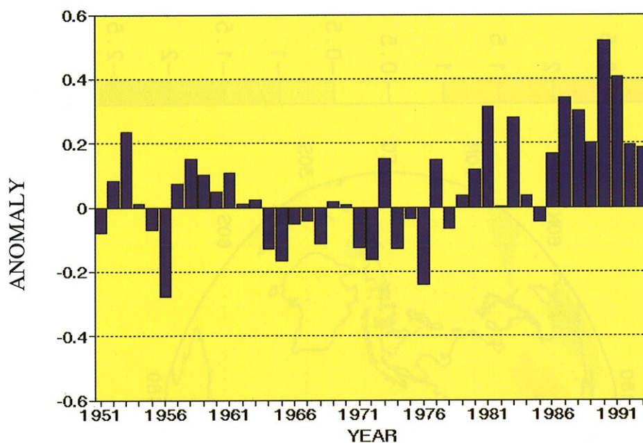
Figure 1.2 Annual global (land only) surface temperature anomalies ( ^{\circ}\text{C} ) computed from the 1951-1980 base period. (Source: CAC)
