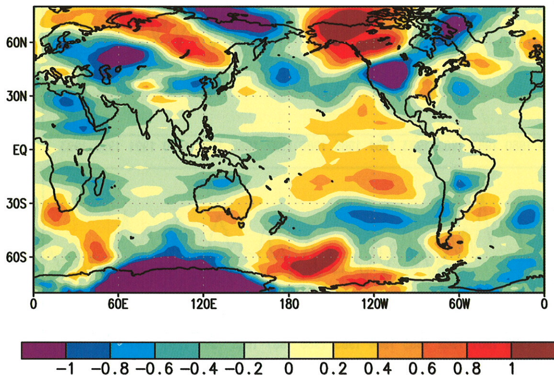
Figure 1.11. Mean annual tropospheric temperature anomalies for 1993 derived from the Microwave Sounding Unit (MSU) channel 2r. Anomalies are departures from the 1982-1991 base period. (Data provided by R. W. Spencer and J. R. Christy.)
