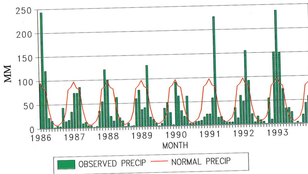
Figure 3.1 Normalized precipitation anomaly for California/Nevada during the December - February period (1951/52-1992/93) (top) and monthly mean precipitation totals (mm) in California (January 1986 - December 1993) (bottom). Solid red curve shows the mean annual cycle (1961-1990) of precipitation. (Source: (top) - CAC, (bottom) - NCDC)
