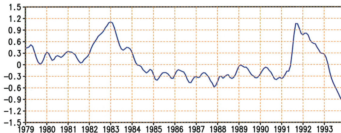
Figure 1.13 Lower-stratospheric temperature anomalies from the Microwave Sounding Unit (MSU) channel 4 for the globe ( 85^\circ\text{S} - 85^\circ\text{N} ). Anomalies are computed from the 1982-1991 base period. (Data provided by R. W. Spencer and J. R. Christy.)
