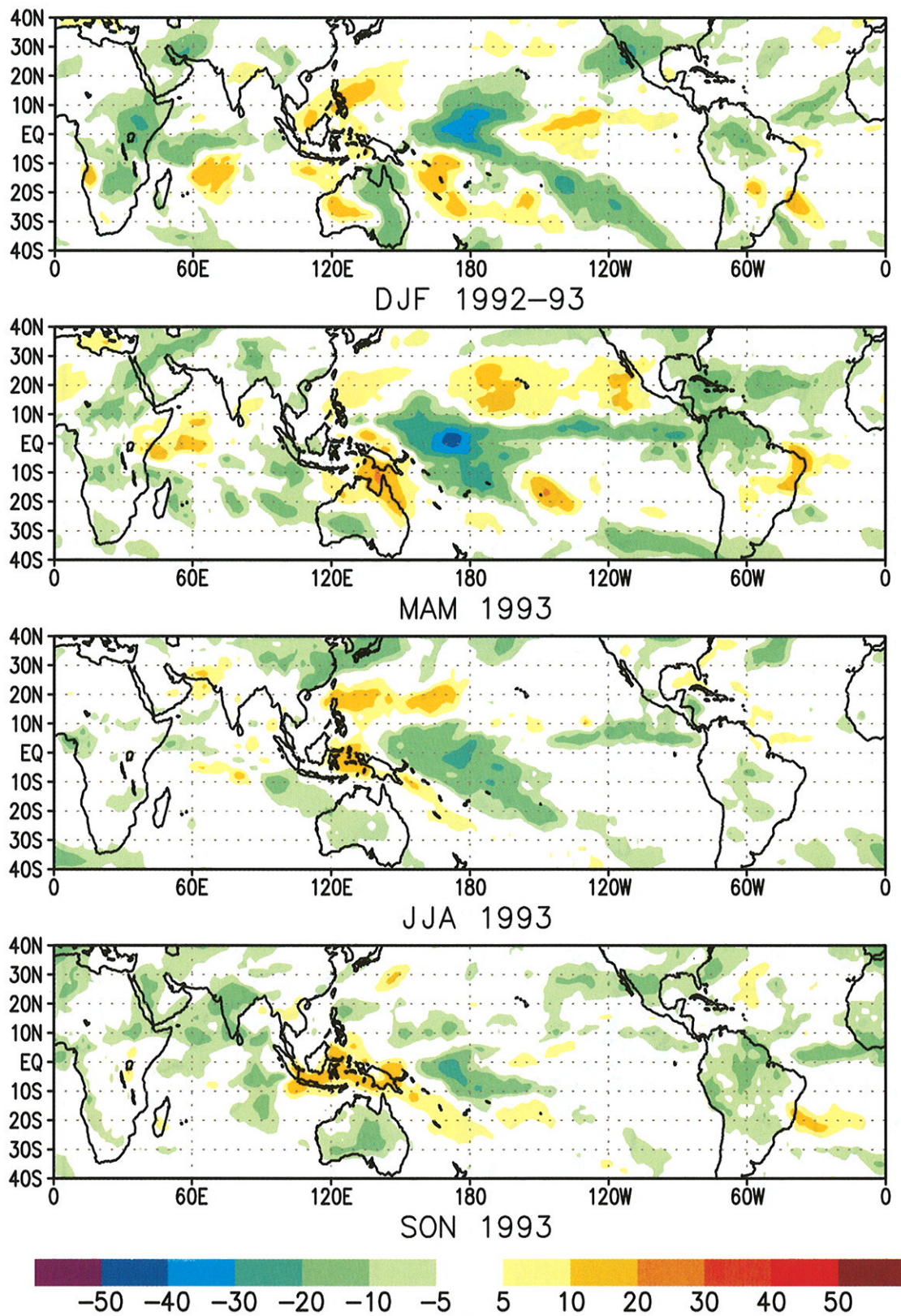
Figure 2.9 Seasonal outgoing longwave radiation (OLR) anomalies ( \text{WM}^{-2} ) computed as departures from the 1979-1988 base period. (Source: CAC)
