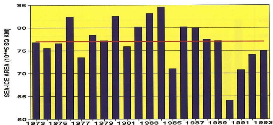
Figure 1.31 Time series of arctic sea ice ( 10^5 \text{ km}^2 ) for August. Solid red line depicts the 1973-1993 mean. (Source: CAC)
