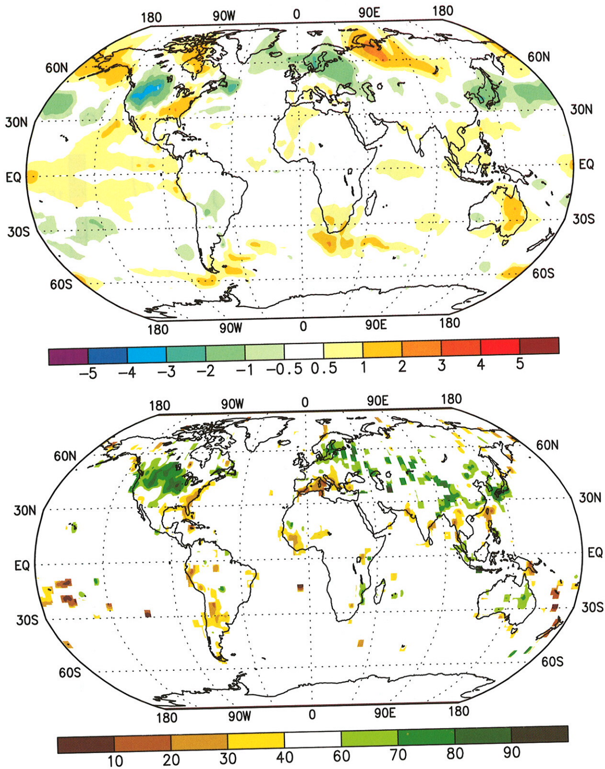
Figure 4.5 Surface temperature anomalies ( ^{\circ}\text{C} ) (top) and precipitation percentiles based on a gamma distribution fit to the 1961-1990 base period (bottom) for June - August 1993. Temperature anomalies are based on station data over land (1961-1990 base period) and sea surface temperature data (SST) over water (COADS/ICE climatology). Analysis omitted in data-sparse regions. (Source: CAC)
