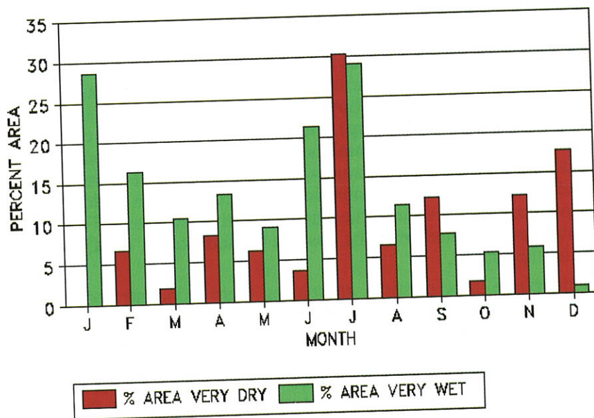
Figure 3.33 Percent area of the contiguous United States experiencing monthly mean precipitation totals in the upper and lower tenth percentile. Precipitation amounts in the upper tenth percentile are categorized as very wet and amounts in the lowest tenth percentile are categorized as very dry. (Source: NCDC)
