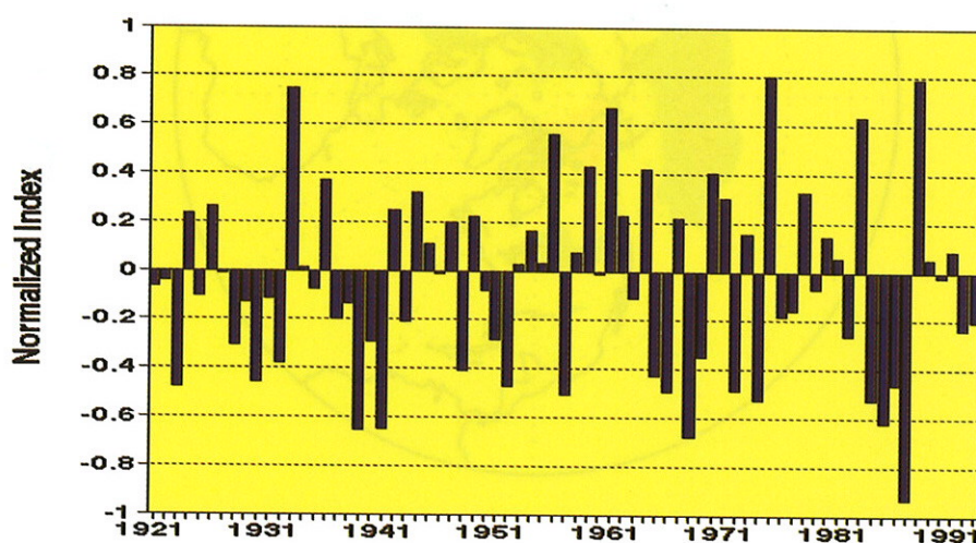
Figure 3.22 Precipitation index (average gamma percentiles of station precipitation within the region) for India (June - September). (Source: CAC)
