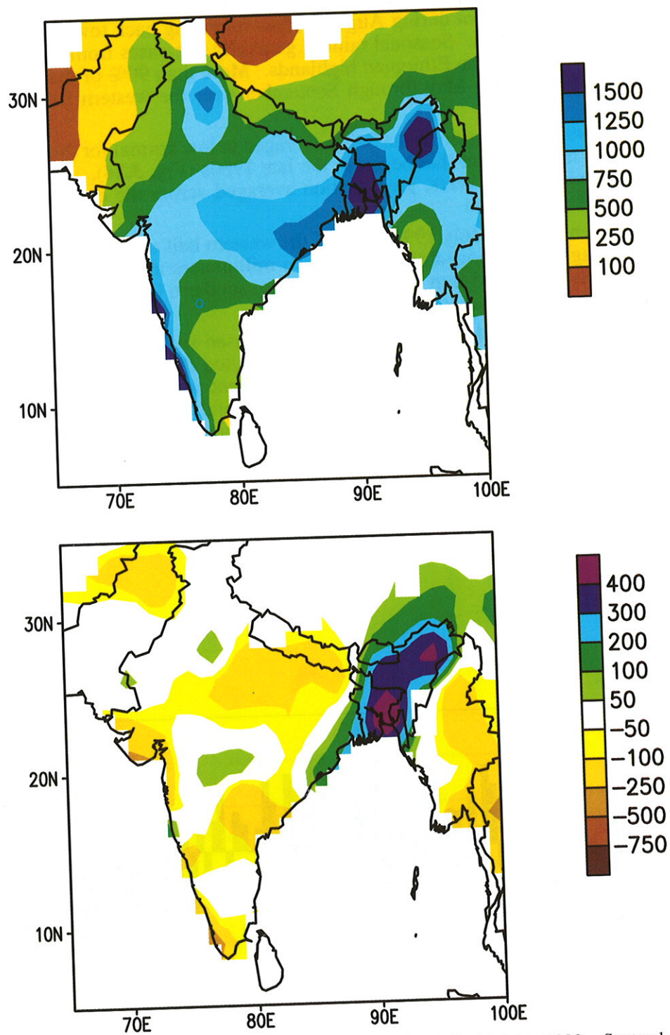
Figure 3.23 Precipitation (mm): total (top) and anomalous (bottom) for India for May 1993 - September 1993. (Source: CAC)
