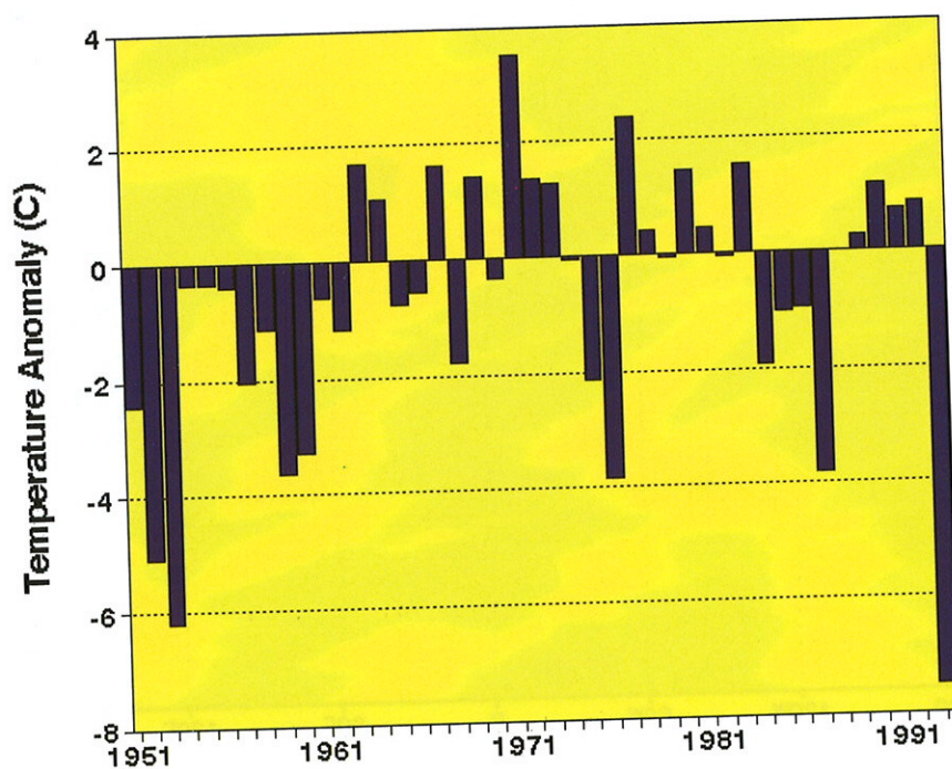
Figure 3.27 Time series of November temperature anomalies ( ^{\circ}\text{C} ) averaged over Europe (top) and western Asia (bottom). (Source: CAC)
