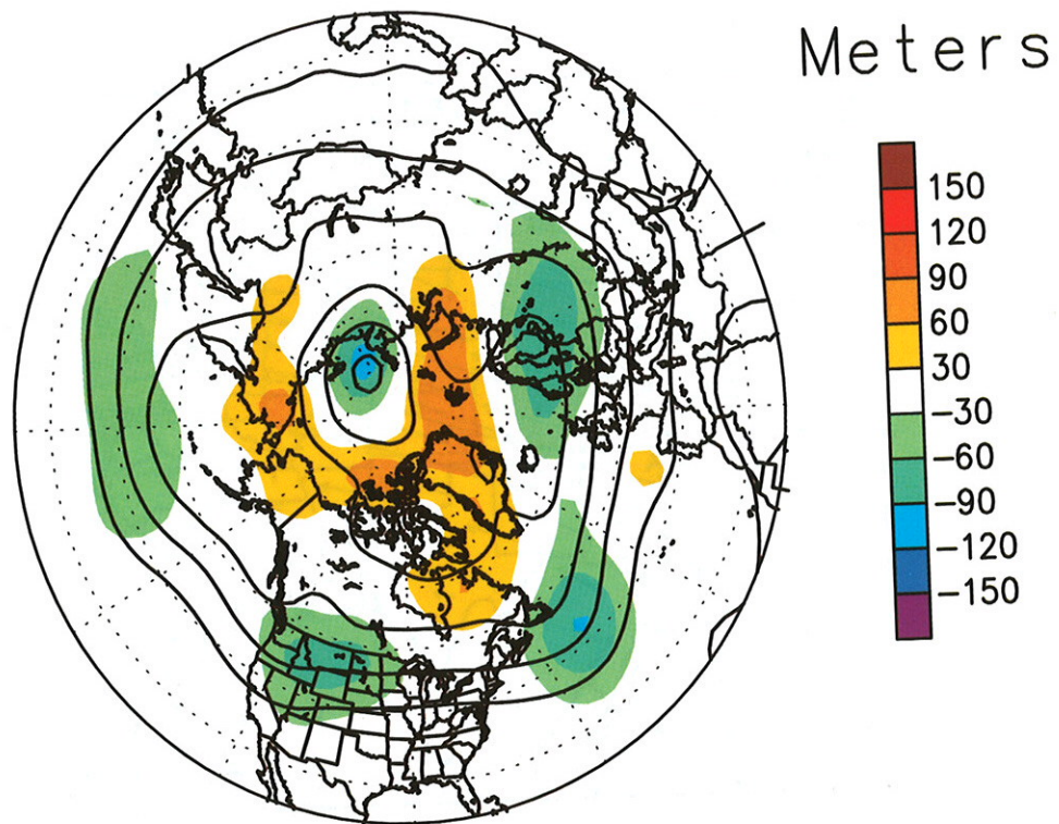
Figure 3.14 Mean 500-mb heights (contours, interval is 120 m) and anomalies (shaded) during June-July 1993. Anomalies are departures from the 1979-1988 base period. (Source: CAC)
