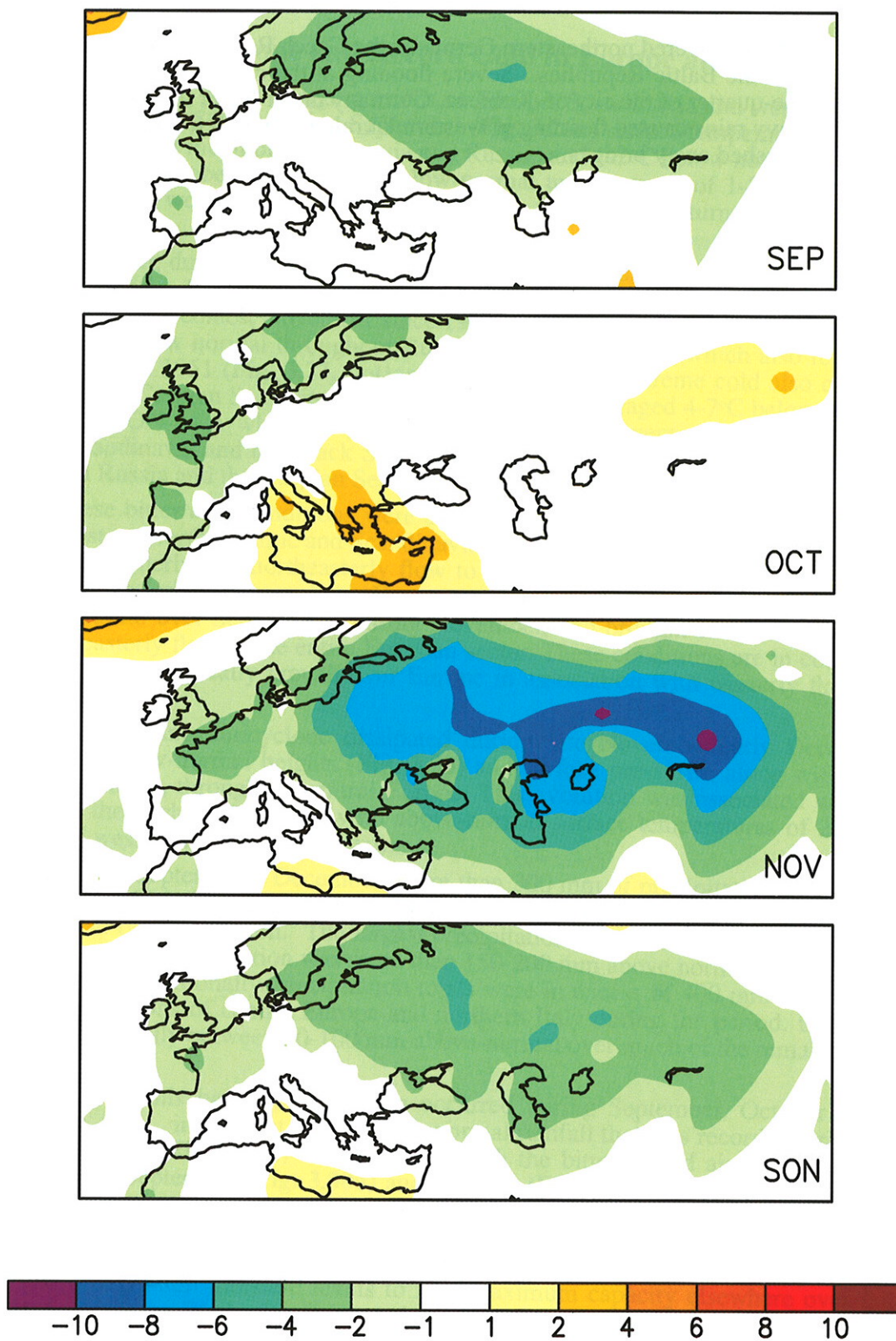
Figure 3.26 Surface temperature anomalies ( ^{\circ}\text{C} ) for: (a) September, (b) October, (c) November, and (d) September-November 1993 for Europe and western Asia. (Source: CAC)
