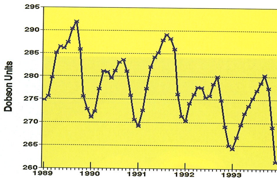
Figure 1.15 Time series of monthly NOAA-11 SBUV/2 total ozone (January 1989 to December 1993) for the region 50°N-50°S. (Source: CAC)
