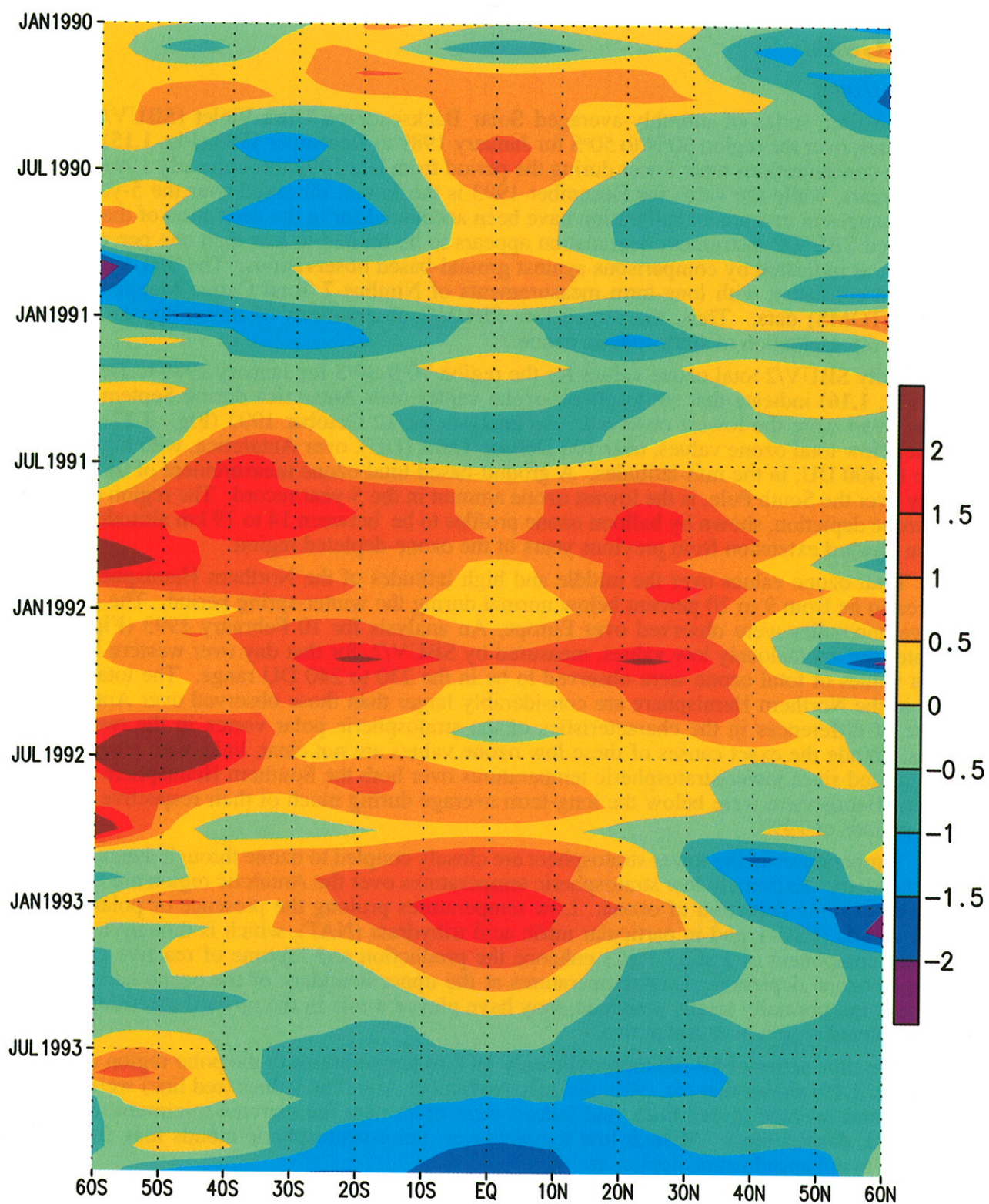
Figure 1.14 Time-latitude section of zonally-averaged lower-stratospheric temperature anomalies ( ^{\circ}\text{C} ) from the Microwave Sounding Unit (MSU) channel 4. Anomalies are computed from the 1982-1991 base period. (Data provided by R. W. Spencer and J. R. Christy.)
