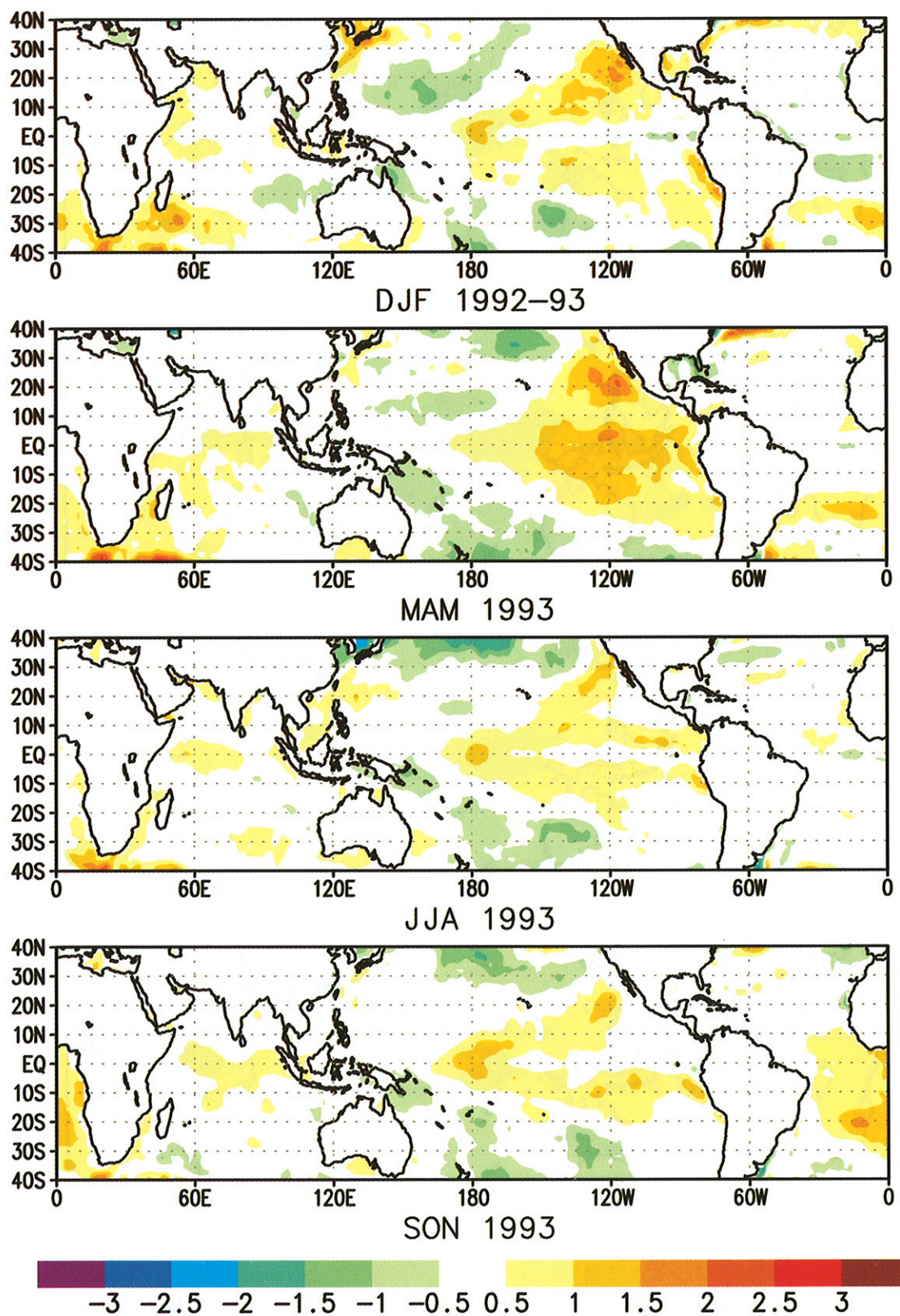
Figure 2.8 Seasonal sea surface temperature (SST) anomalies ( ^{\circ}\text{C} ) computed as departures from the COADS/ICE climatology (Reynolds 1988). (Data provided by the NMC Coupled Model Project.)
