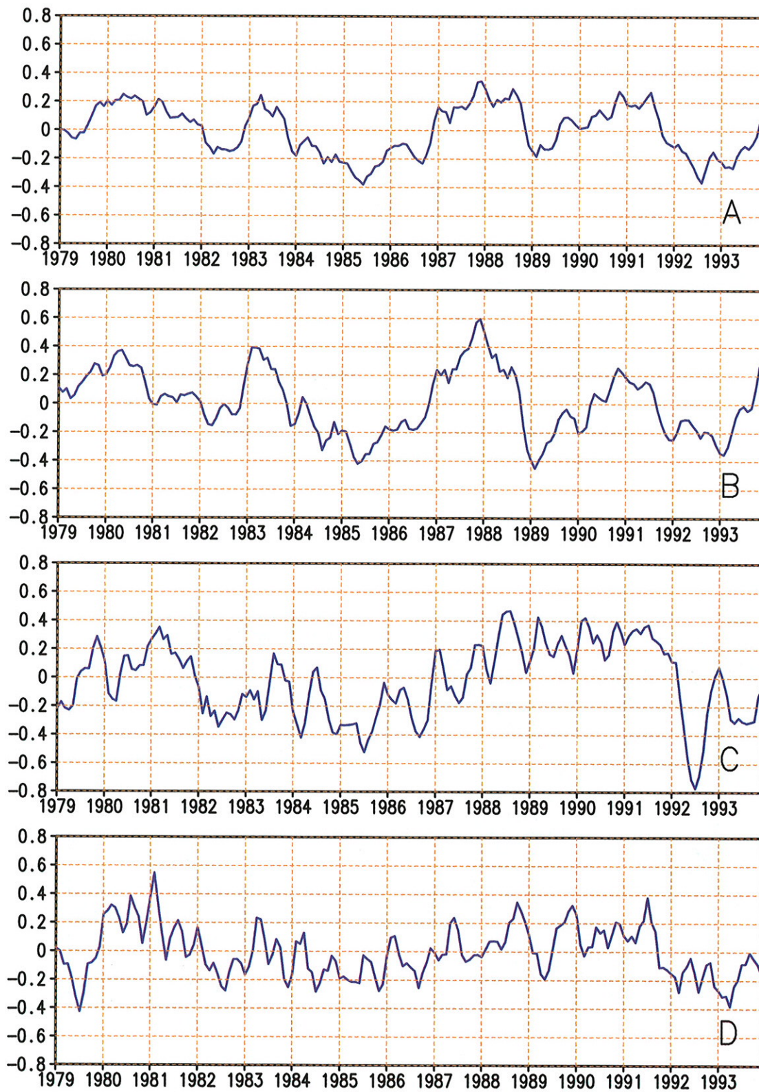
Figure 1.9 Mean tropospheric temperature anomalies from the Microwave Sounding Unit (MSU) channel 2r for the a) globe ( 85^{\circ}\text{S} - 85^{\circ}\text{N} ), b) tropics ( 30^{\circ}\text{N} - 30^{\circ}\text{S} ), c) Northern Hemisphere extratropics ( 30^{\circ}\text{N} - 85^{\circ}\text{N} ) and d) Southern Hemisphere extratropics ( 30^{\circ}\text{S} - 85^{\circ}\text{S} ). Anomalies are computed from the 1982-1991 base period. (Data provided by R. W. Spencer and J. R. Christy.)
