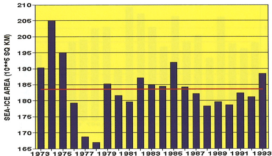
Figure 1.33 Time series of antarctic sea ice ( 10^5 \text{ km}^2 ) for August. Solid red line depicts the 1973-1993 mean. (Source: CAC)
