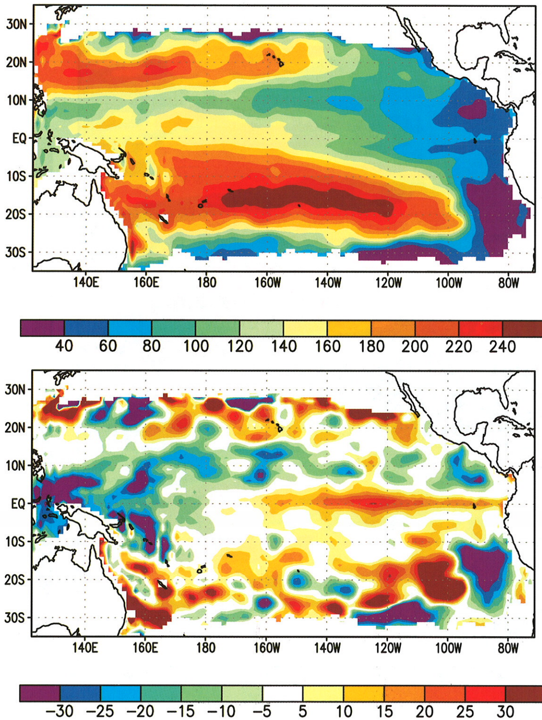
Figure 2.6 Mean (top) and anomalous (bottom) depth (m) of the 20°C isotherm for the period March - May 1993. Anomalies are departures from the 1983-1992 base period. (Data provided by the NMC Coupled Model Project.)
