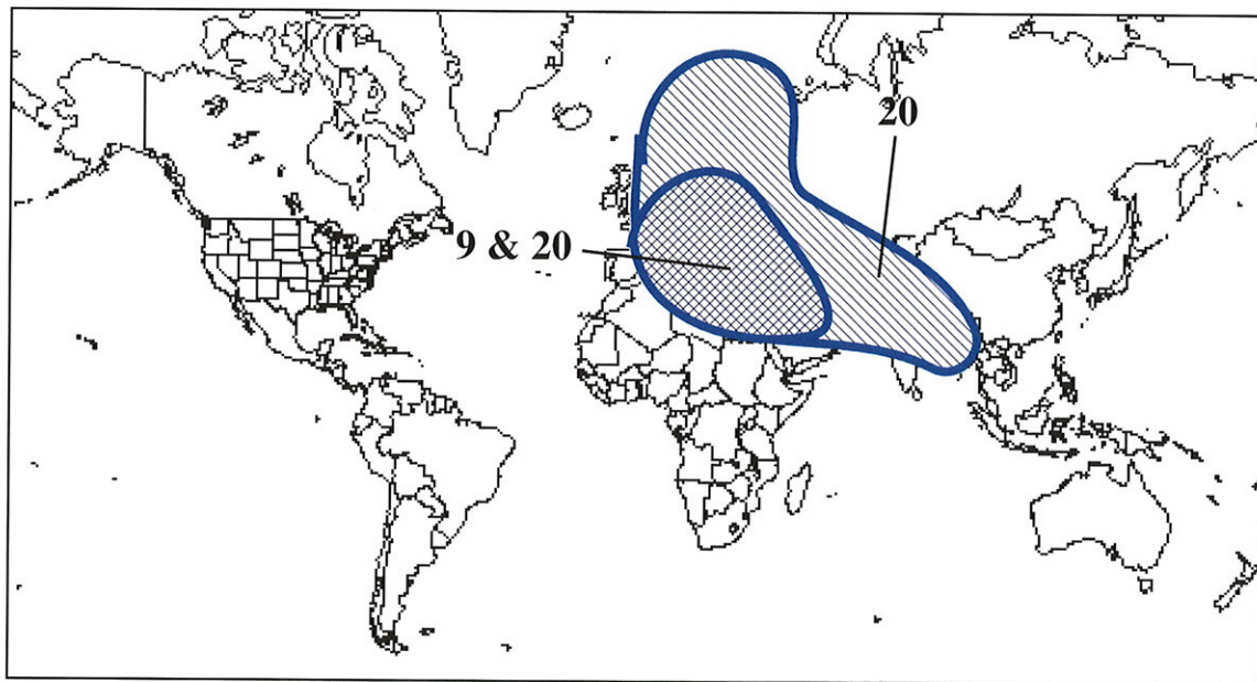
Figure 5.1 Significant above-normal temperature anomalies (top) and below-normal temperature anomalies (bottom) during 1993. The numbers are keyed to the descriptive paragraphs. (Source: CAC)
