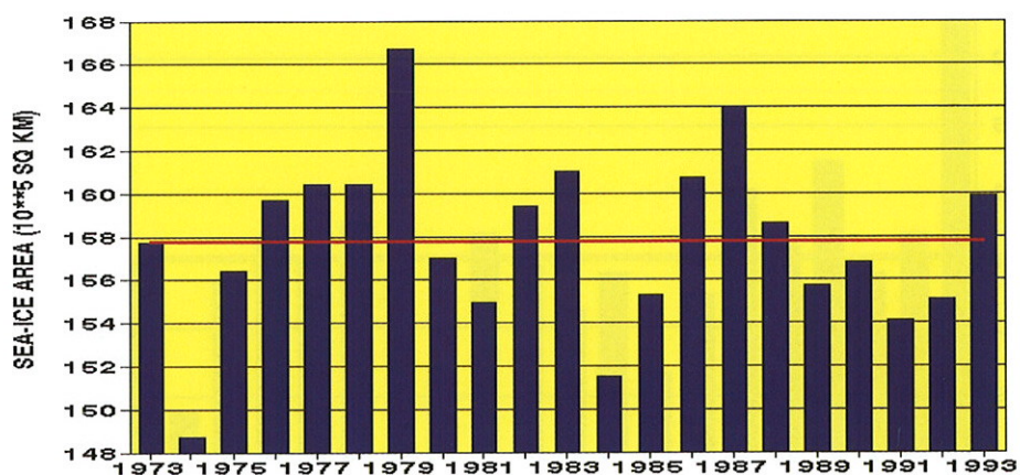
Figure 1.30 Time series of arctic sea ice ( 10^5 \text{ km}^2 ) for February. Solid red line depicts the 1973-1993 mean. (Source: CAC)
