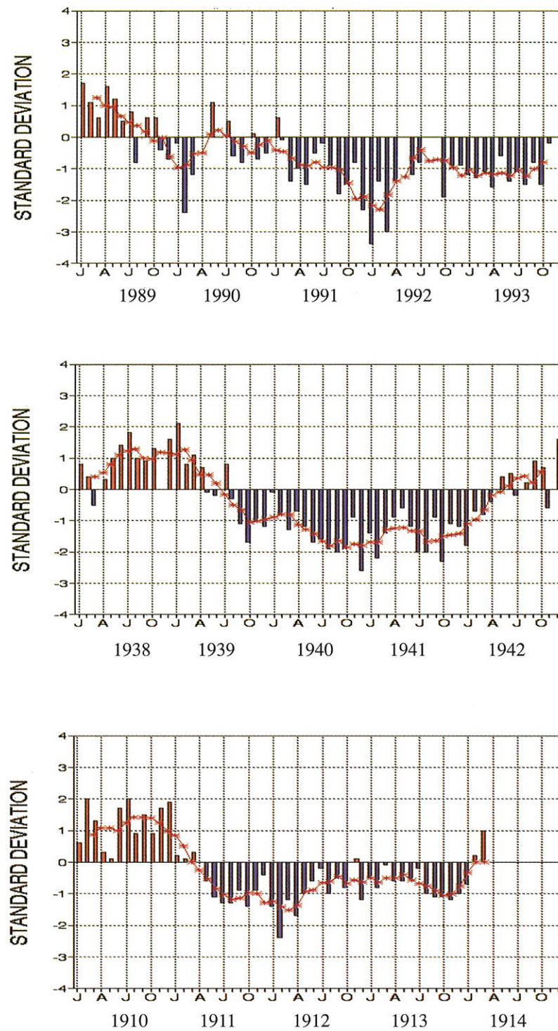
Figure 2.1 The Southern Oscillation Index (SOI) for the three longest warm episodes in the historical record. Monthly (five month running mean) values are indicated by the bar (red line) graph. (Source: CAC)
