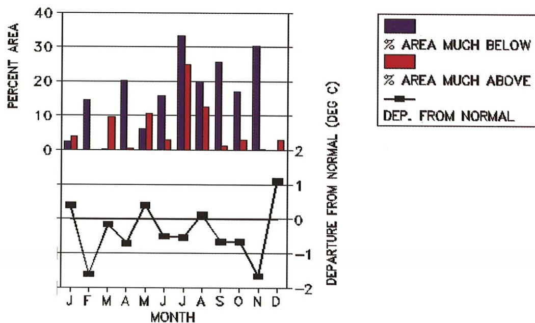
Figure 3.32 Percent area of the contiguous United States experiencing monthly mean temperatures in the upper and lower tenth percentile (top) and the monthly temperature departures from the 1961-1990 base period averaged across the contiguous U. S. (bottom). (Source: NCDC)
