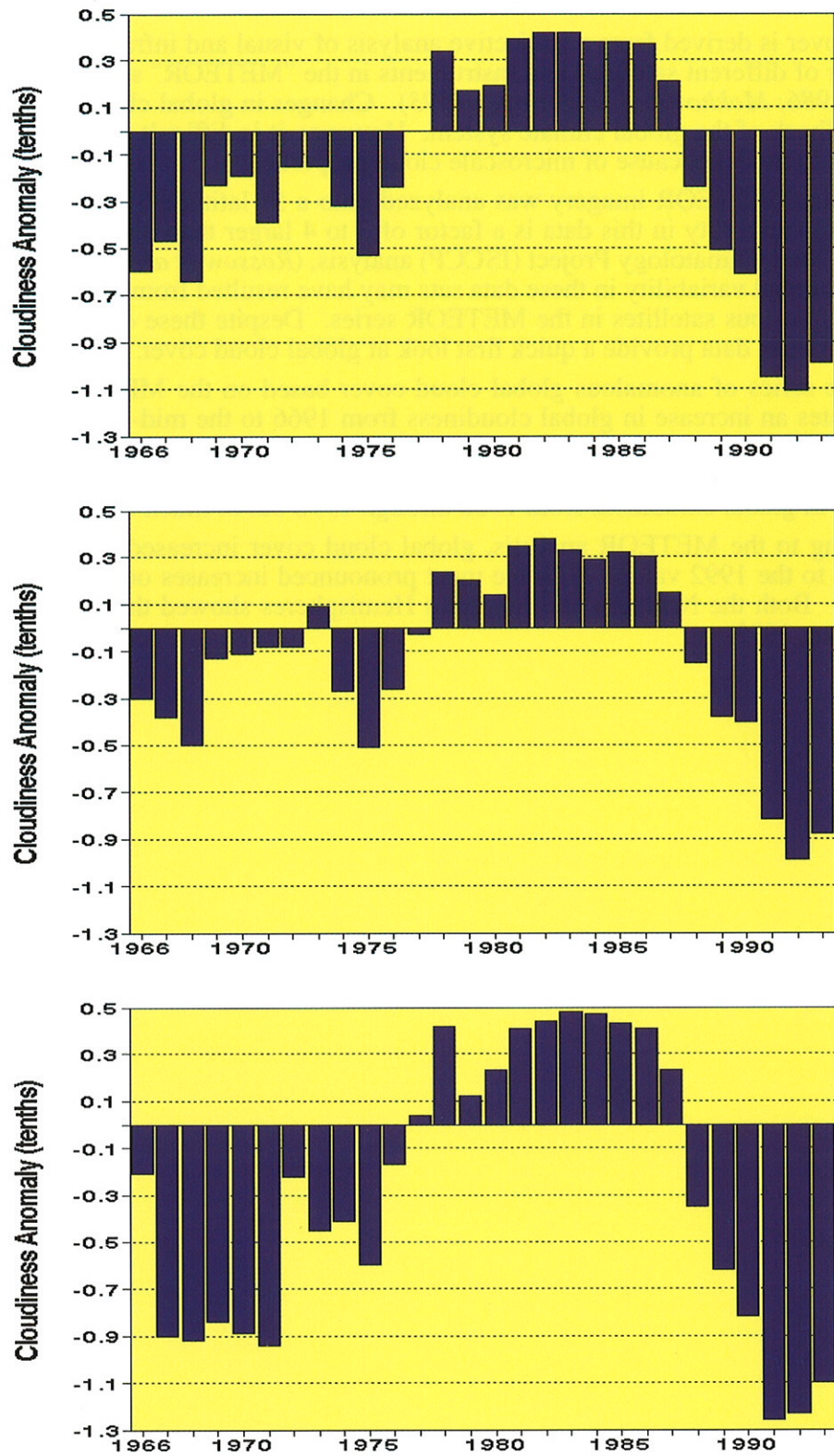
Figure 1.34. Regionally-averaged annual total cloud cover anomalies: global (top), Northern Hemisphere (middle), and Southern Hemisphere (bottom). Anomalies (expressed in tenths) are computed from the 1966-1985 base period. (Source: Institute for Global Climate and Ecology, Moscow)
