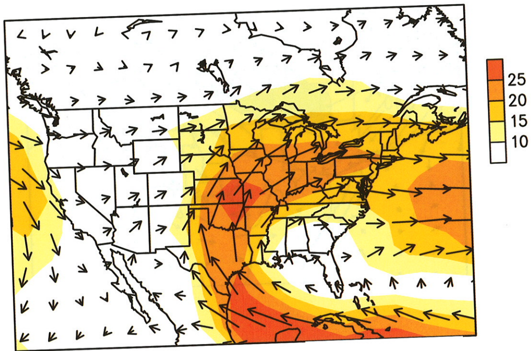
Figure 3.15 Mean vertically-integrated moisture transport (shaded, units are 10^{-3} \text{ kg m}^{-3} \text{ s}^{-1} ) and 850-mb vector wind ( \text{ms}^{-1} ) during June-July 1993. (Source: CAC)
