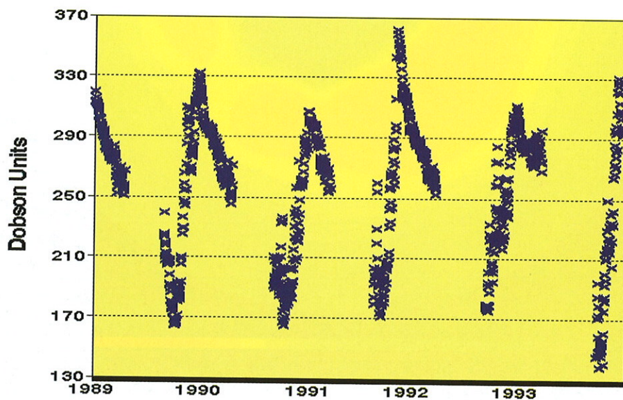
Figure 1.16 Time series of daily SBUV/2 total ozone (January 1989 to December 1993) for the 70°S-80°S region. Missing data occur each winter due to a lack of sunlight when SBUV/2 views the polar region. (Source: CAC)
