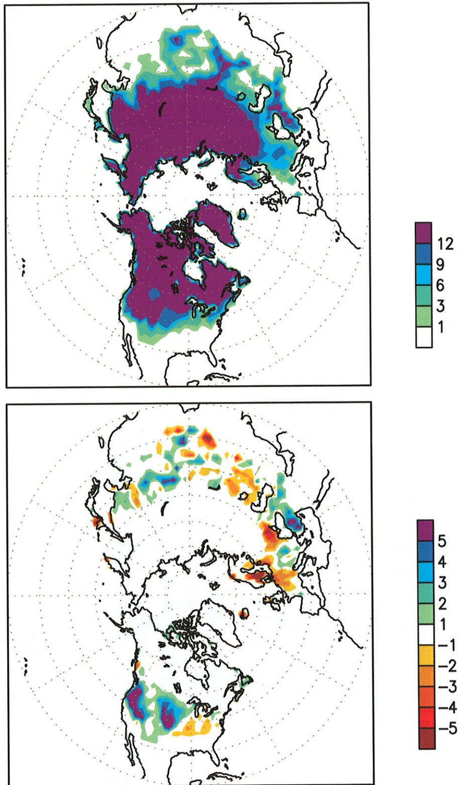
Figure 1.25 Winter snow-cover extent in weeks of snow cover (top) and anomaly (bottom), derived from subjective analysis of visual imagery by NOAA/NESDIS. Anomalies are departures from the 1973-1993 base period. (Source: CAC)
