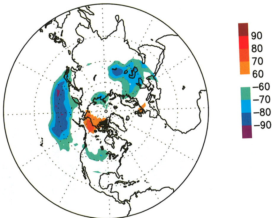
Figure 3.21 Percentage of days in which positive (red shading) and negative (blue shading) low-pass filtered (retaining periods > 30 days) height anomalies at 500 mb were observed between February - July 1993. (Source: CAC)
