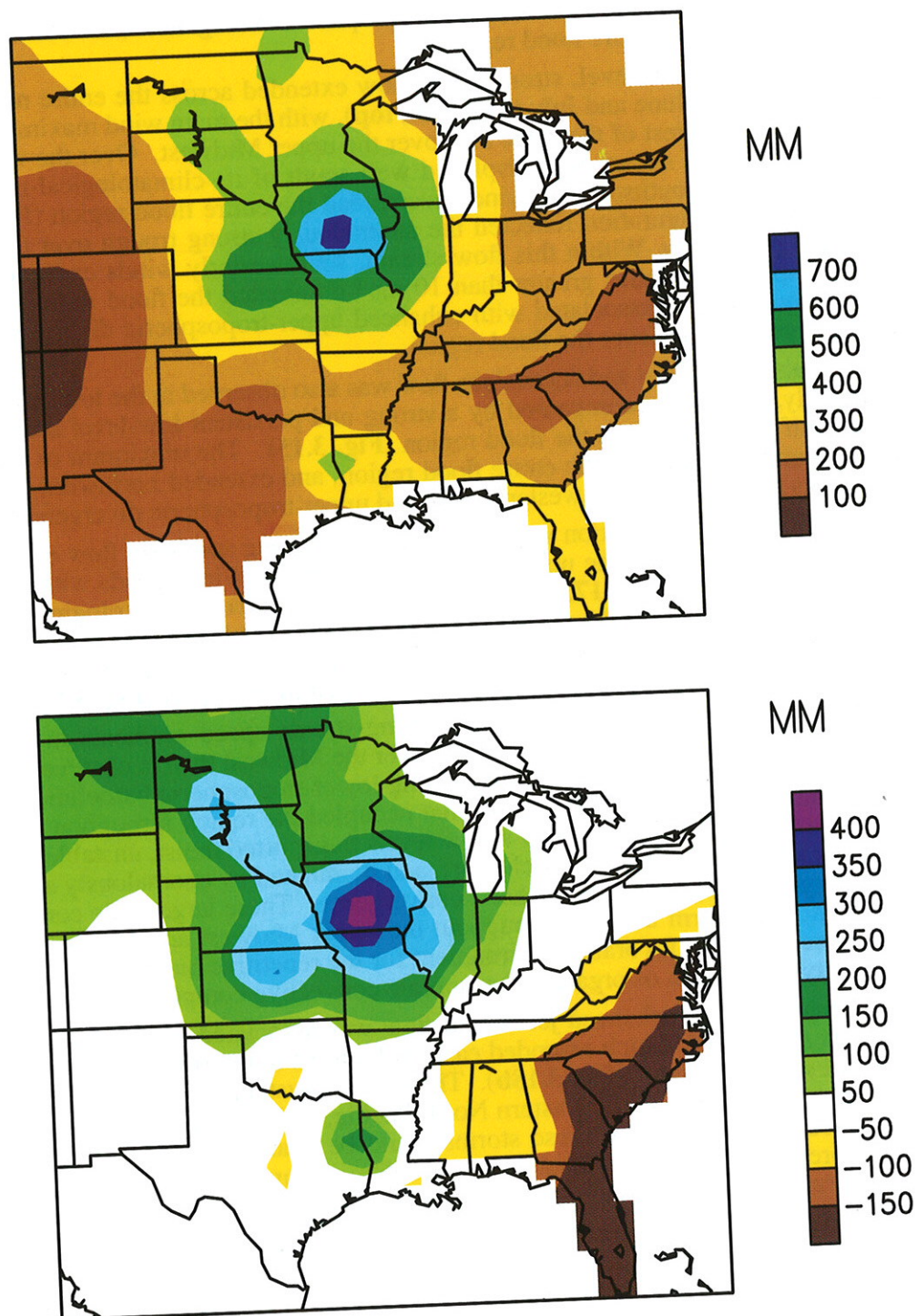
Figure 3.13 Precipitation: total (top) and anomalous (mm) (bottom) during June-August 1993. Anomalies are computed with respect to the 1961-1990 base period. (Source: CAC)
