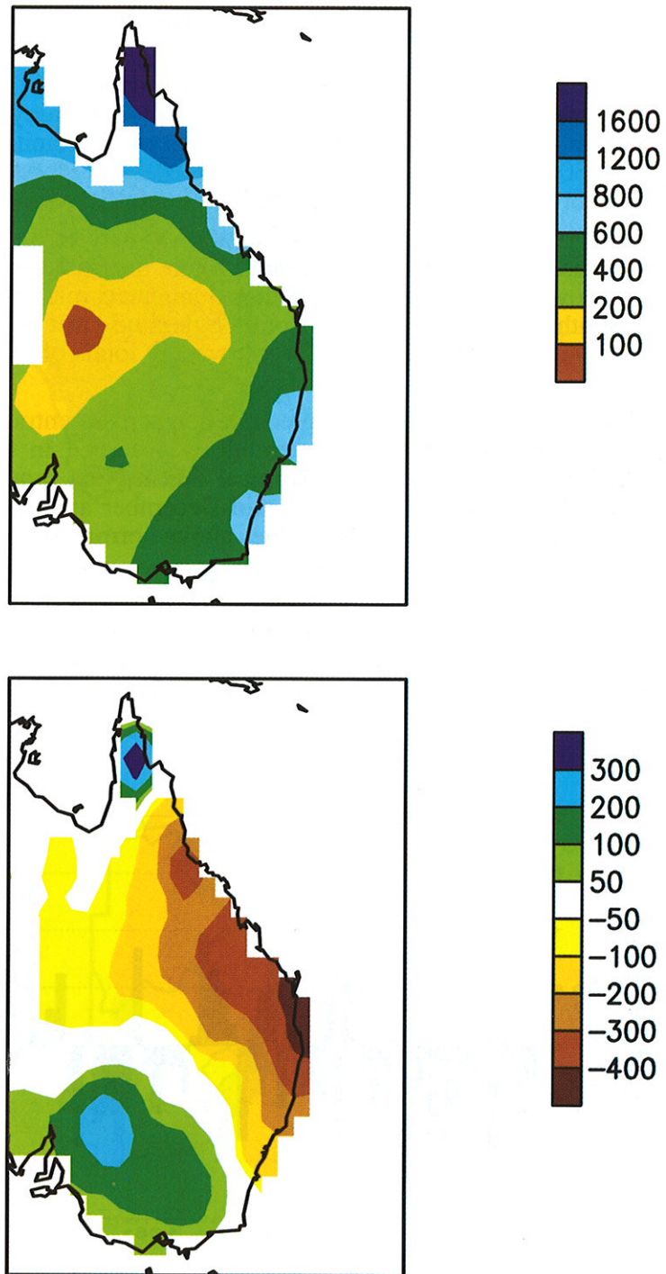
Figure 3.9 Total precipitation (top) and departure from normal (mm) (bottom) for eastern Australia for October 1992 - May 1993. (Source: CAC)
