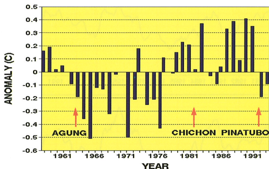
Figure 1.10 Annual global tropospheric (850-300 mb) temperature anomalies derived from radiosonde data. Annual values of global tropospheric temperature anomalies are based on a 63-station network and computed from the 1958-1991 base period. (Data provided by J. Angell.)
