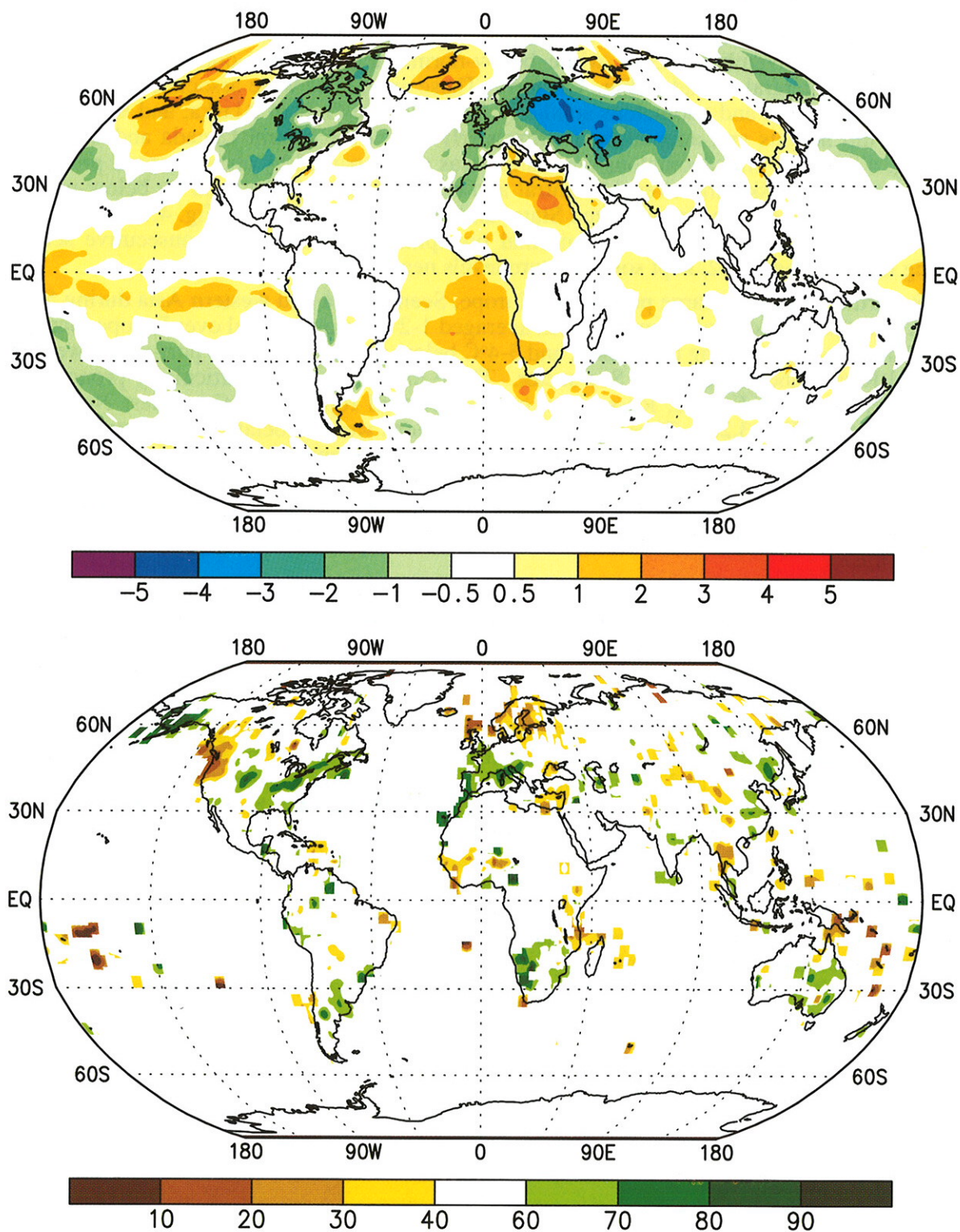
Figure 4.7 Surface temperature anomalies ( ^{\circ}\text{C} ) (top) and precipitation percentiles based on a gamma distribution fit to the 1961-1990 base period (bottom) for September - November 1993. Temperature anomalies are based on station data over land (1961-1990 base period) and sea surface temperature data (SST) over water (COADS/ICE climatology). Analysis omitted in data-sparse regions. (Source: CAC)
