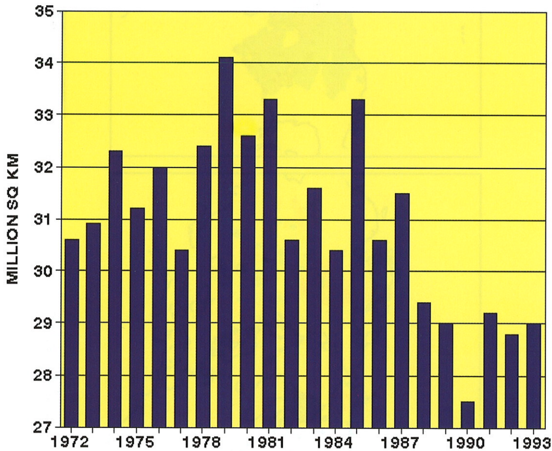
Figure 1.26 Time series of Northern Hemisphere snow-cover area ( 10^6 \text{ km}^2 ) for spring (March through May), estimated from satellite imagery. (Data provided by NOAA/NESDIS and D. Robinson, Rutgers University.)
