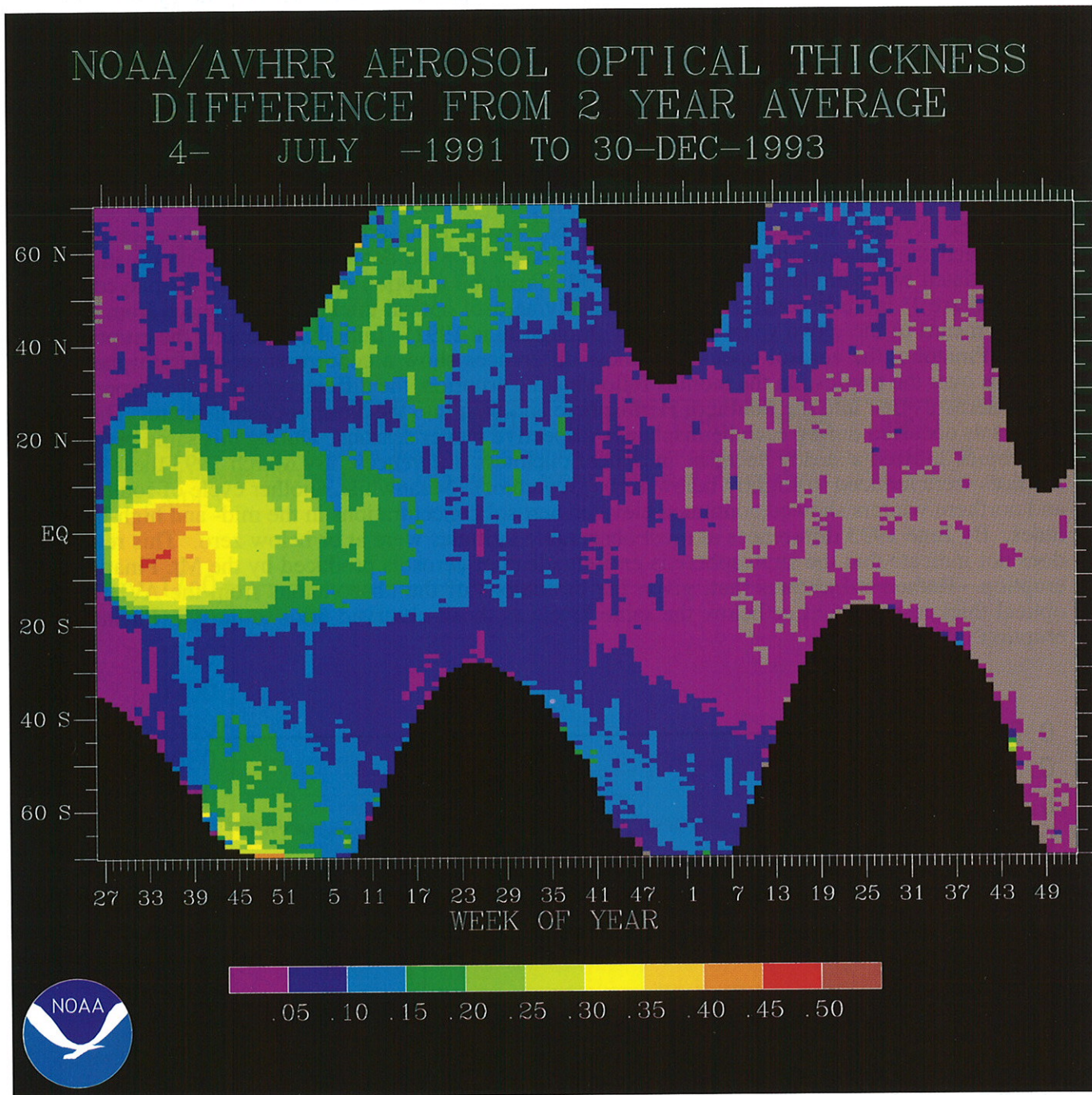
Figure 1.23 Weekly zonal averages of the aerosol optical thickness (AOT) differences from 70°S to 70°N for the period 4 July 1991 through 30 December 1993. Differences are from the July 1989 - June 1991 base period. (Data provided by L. Stowe.)
