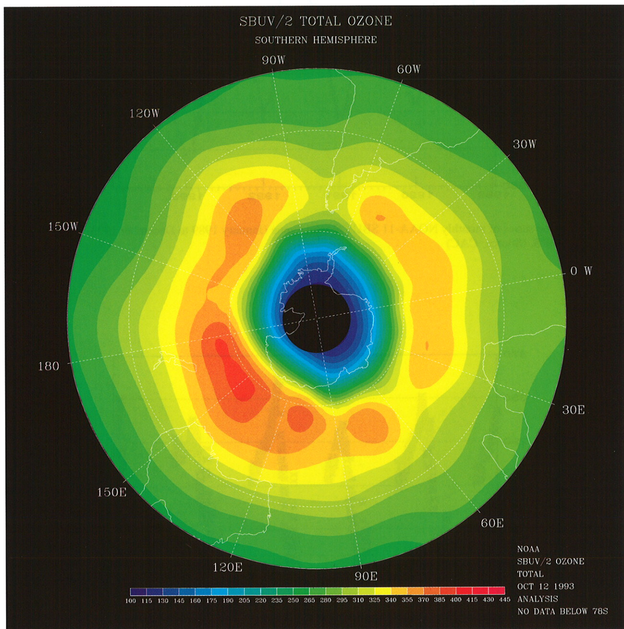
Figure 1.17 Southern Hemisphere NOAA-11 SBUV/2 total ozone (DU) for 12 October 1993. Areas of lowest ozone are shown in blue and purple, with highest values in yellow and red. Regions of no data are shown in black. (Source: CAC)
