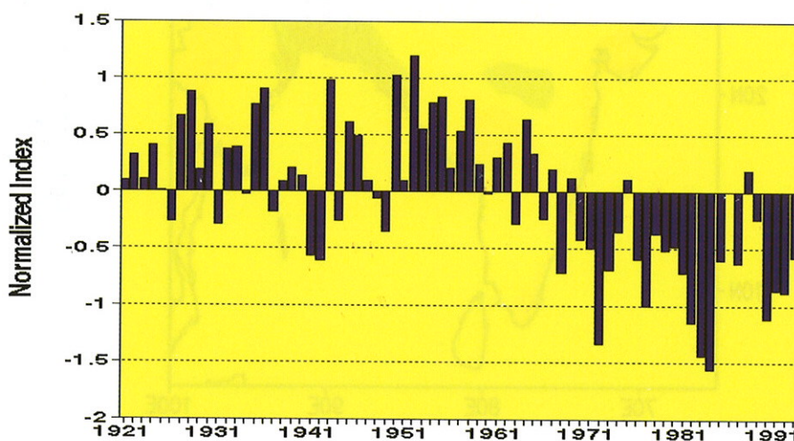
Figure 3.24 Precipitation index (average gamma percentiles of station precipitation within the region) for the western Sahel (June - September). (Source: CAC)
