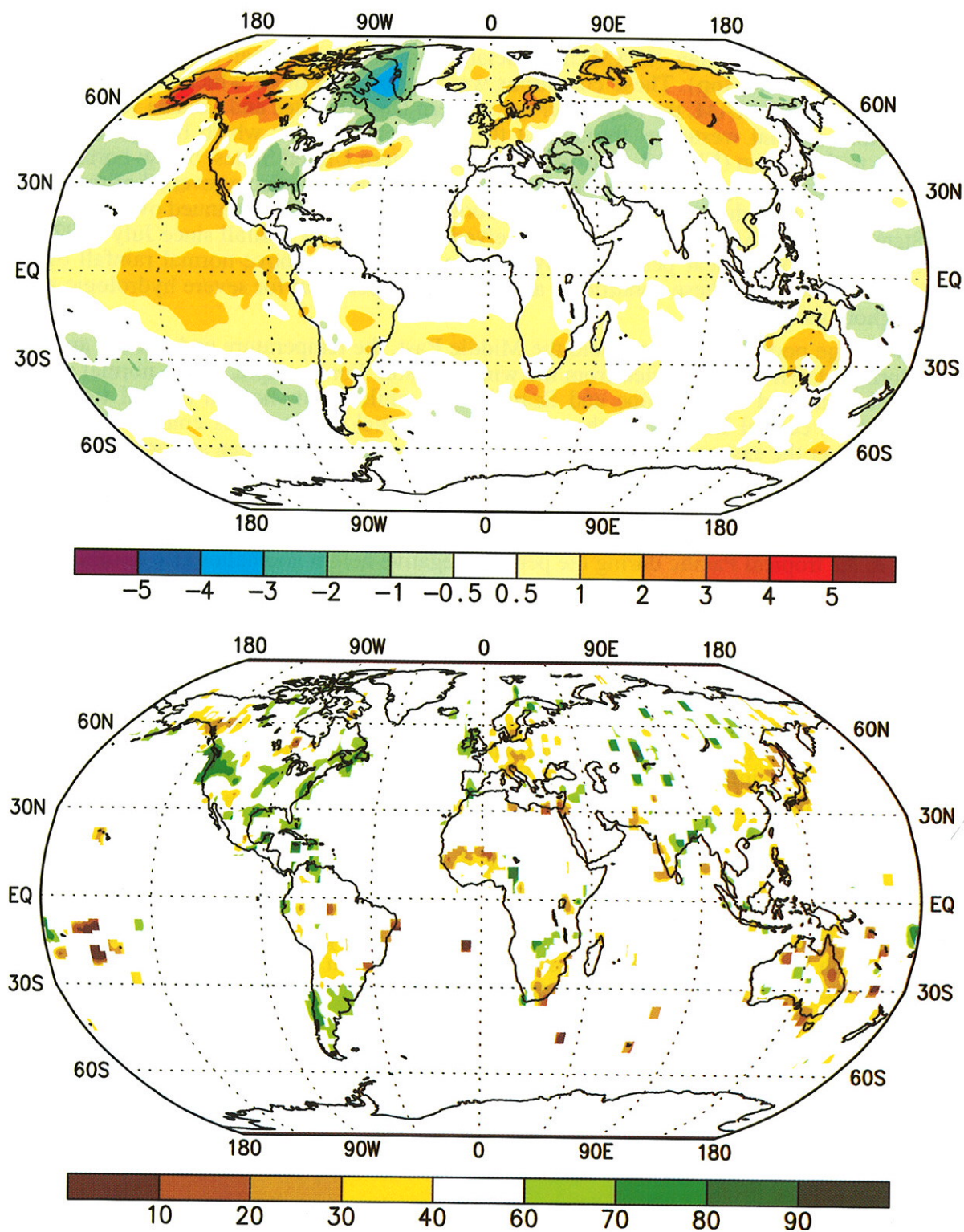
Figure 4.3 Surface temperature anomalies ( ^{\circ}\text{C} ) (top) and precipitation percentiles based on a gamma distribution fit to the 1961-1990 base period (bottom) for March - May 1993. Temperature anomalies are based on station data over land (1961-1990 base period) and sea surface temperature data (SST) over water (COADS/ICE climatology). Analysis omitted in data-sparse regions. (Source: CAC)
