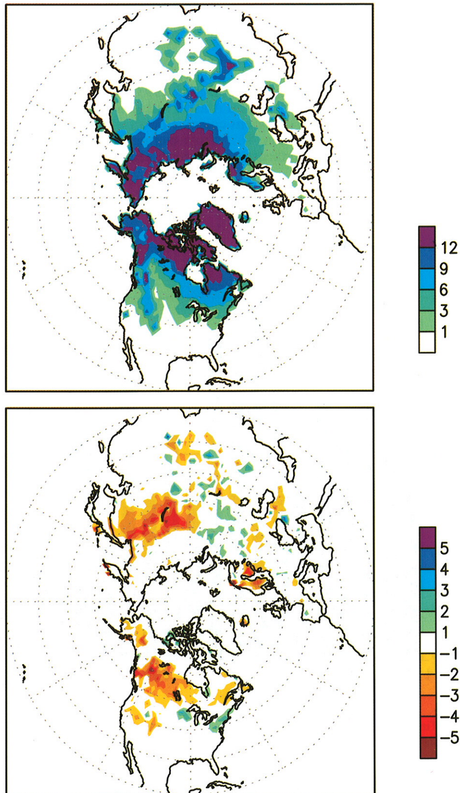
Figure 1.27 Spring snow-cover extent in weeks of snow cover (top) and anomaly (bottom), derived from subjective analysis of visual imagery by NOAA/NESDIS. Anomalies are departures from the 1973-1993 base period. (Source: CAC)
