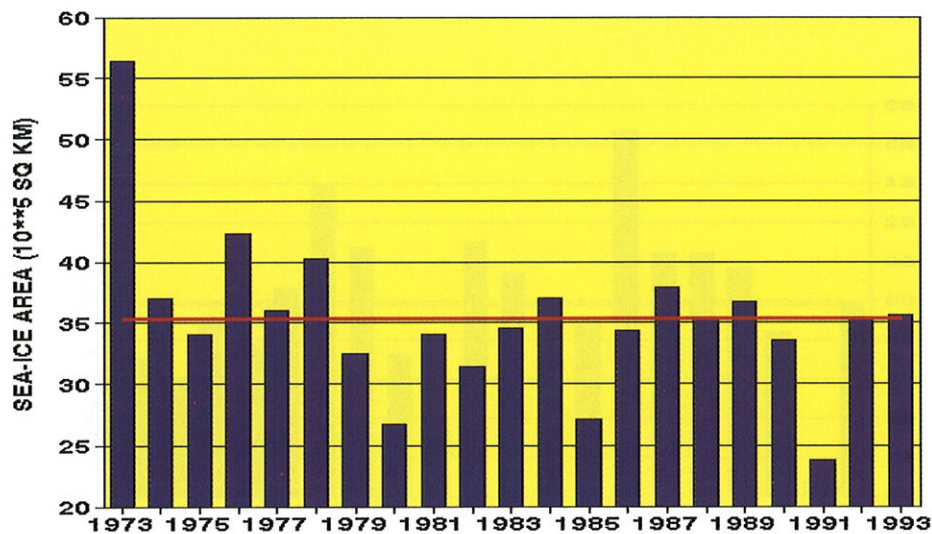
Figure 1.32 Time series of antarctic sea ice ( 10^5 \text{ km}^2 ) for February. Solid red line depicts the 1973-1993 mean. (Source: CAC)
