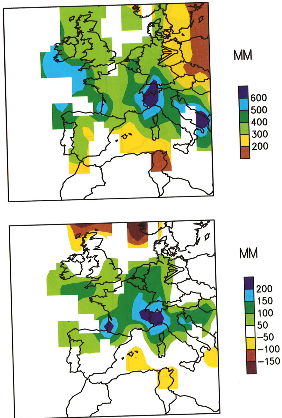
Figure 3.29 Precipitation (mm): total (top) and anomalous (bottom) for September - December 1993. (Source: CAC)
