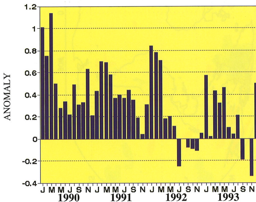
Figure 1.3 Monthly global (land only) surface temperature anomalies ( ^{\circ}\text{C} ) from January 1990 - December 1993 computed from the 1951-1980 base period. (Source: CAC)
