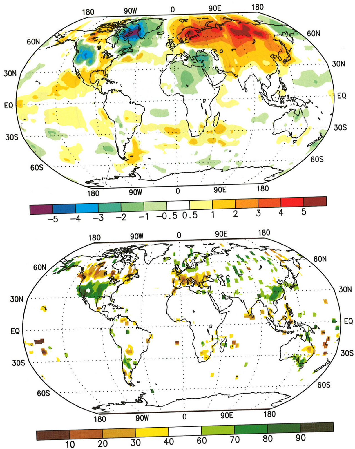
Figure 4.1 Surface temperature anomalies ( ^{\circ}\text{C} ) (top) and precipitation percentiles based on a gamma distribution fit to the 1961-1990 base period (bottom) for December 1992 - February 1993. Temperature anomalies are based on station data over land (1961-1990 base period) and sea surface temperature data (SST) over water (COADS/ICE climatology). Analysis omitted in data-sparse regions. (Source: CAC)
