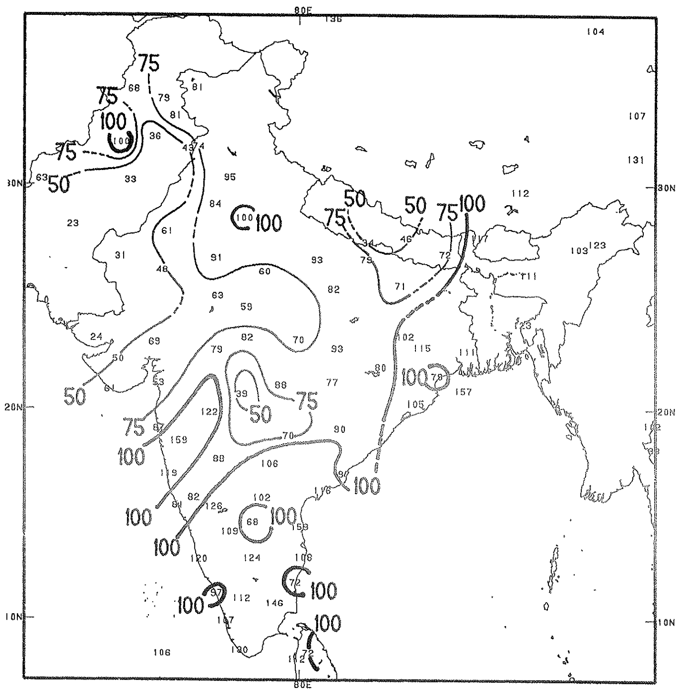
Fig. 30. Percent of normal precipitation during May 1 - September 30, 1991. Isopleths drawn for 50%, 75%, and 100% (thick line).
