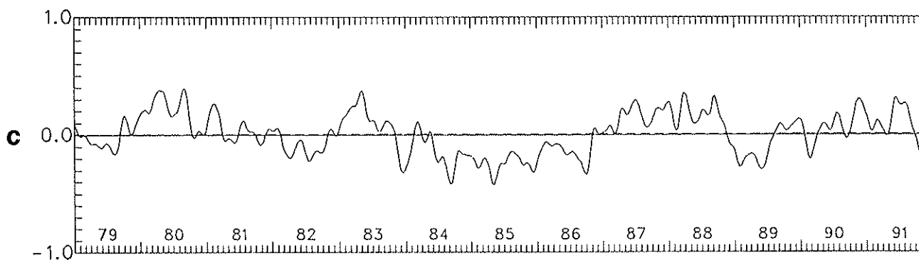
Fig. 38. Time series of a) global, b) Northern Hemisphere and c) Southern Hemisphere lower tropospheric temperature anomalies derived from satellite Microwave Sounding Unit (MSU) observations.
