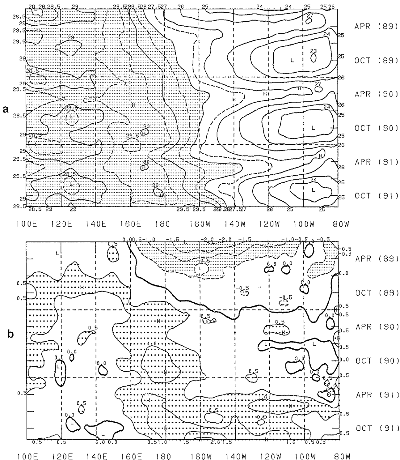
Fig. 1. Time-longitude section of monthly sea surface temperature a) mean and b) anomalous. Contour interval is 1°C and 0.5°C, respectively. SST values greater than 28°C and anomalies less than -0.5°C are shaded. Stippled areas indicate anomaly values greater than 0.5°C. Anomalies are computed based on the COADS/ICE climatology (Reynolds 1988). A 1-2-1 filter in time is used on all points prior to the current month.
