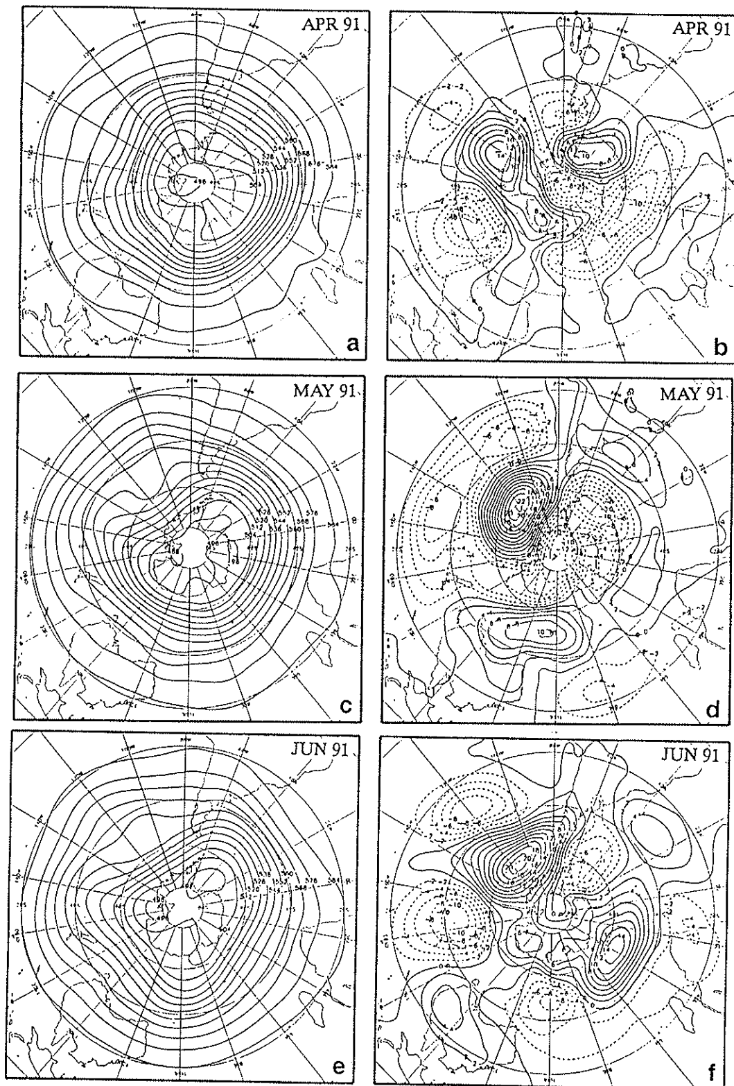
Fig. 51. Monthly mean 500 mb heights (interval is 80 m) and anomalies (interval is 20 m) for (a,b) April 1991, (c,d) May 1991 and (e,f) June 1991, respectively.
