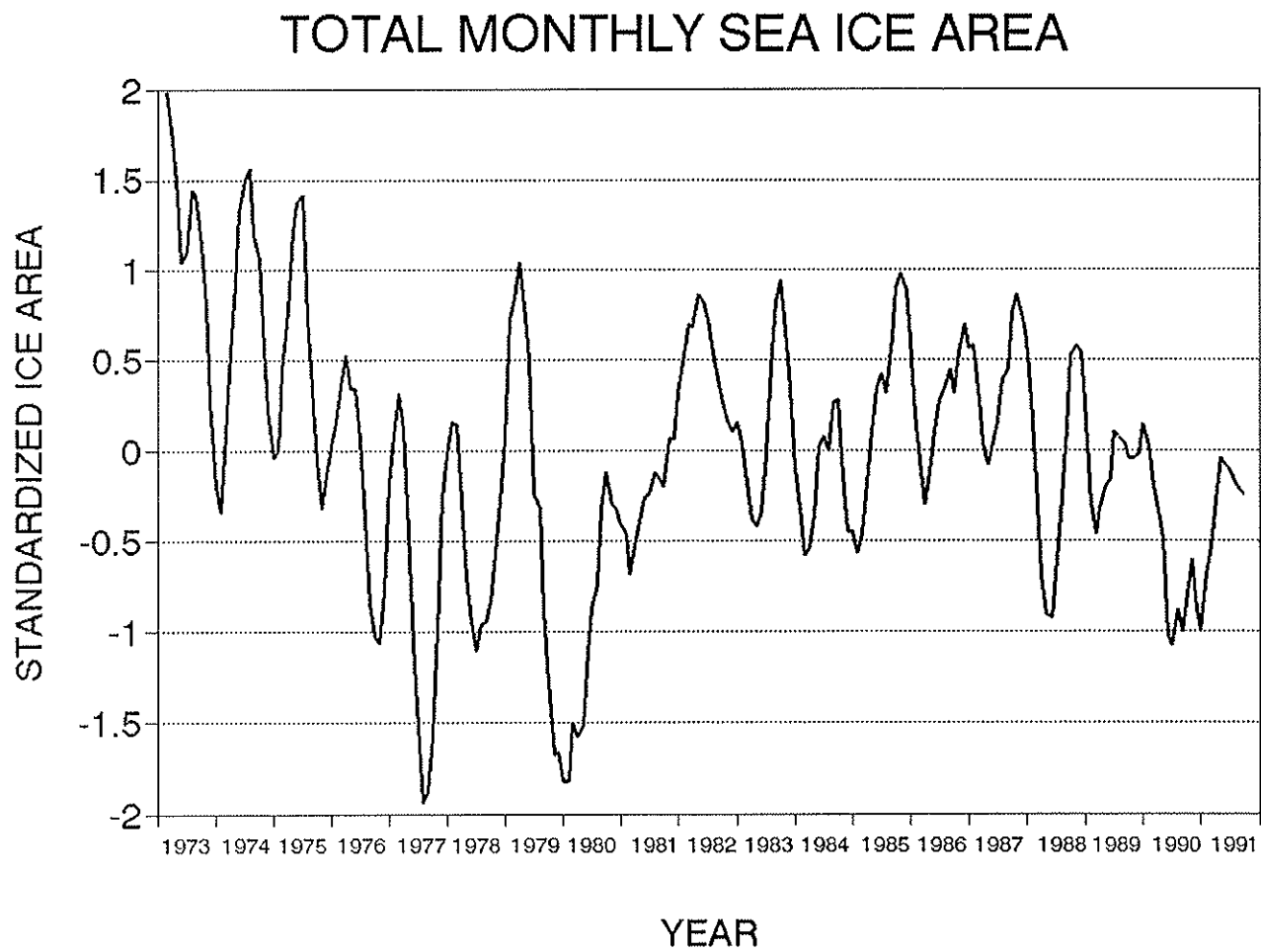
Fig. 37. Five month running mean of the standardized global (Arctic and Antarctic) sea ice area anomalies computed from the 1973 - 1991 base period.
