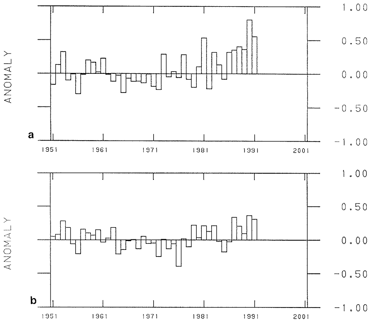
Fig. 13. Time series of estimated Northern Hemisphere surface temperature anomalies for a) January - June and for b) July - December. Global temperature anomaly estimates are formed from area weighted averages of station anomalies over a 2^{\circ} latitude by 2^{\circ} longitude grid.
