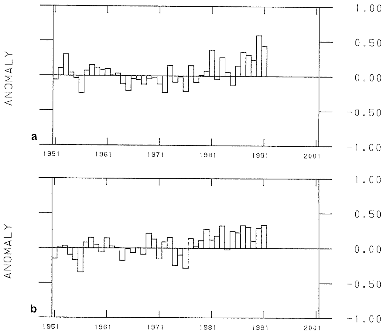
Fig. 10. Time series of estimated a) Northern Hemisphere and b) Southern Hemisphere surface temperature anomalies for the calendar year. Temperature anomaly estimates are formed from area weighted averages of station anomalies over 2^{\circ} latitude by 2^{\circ} longitude grids.
