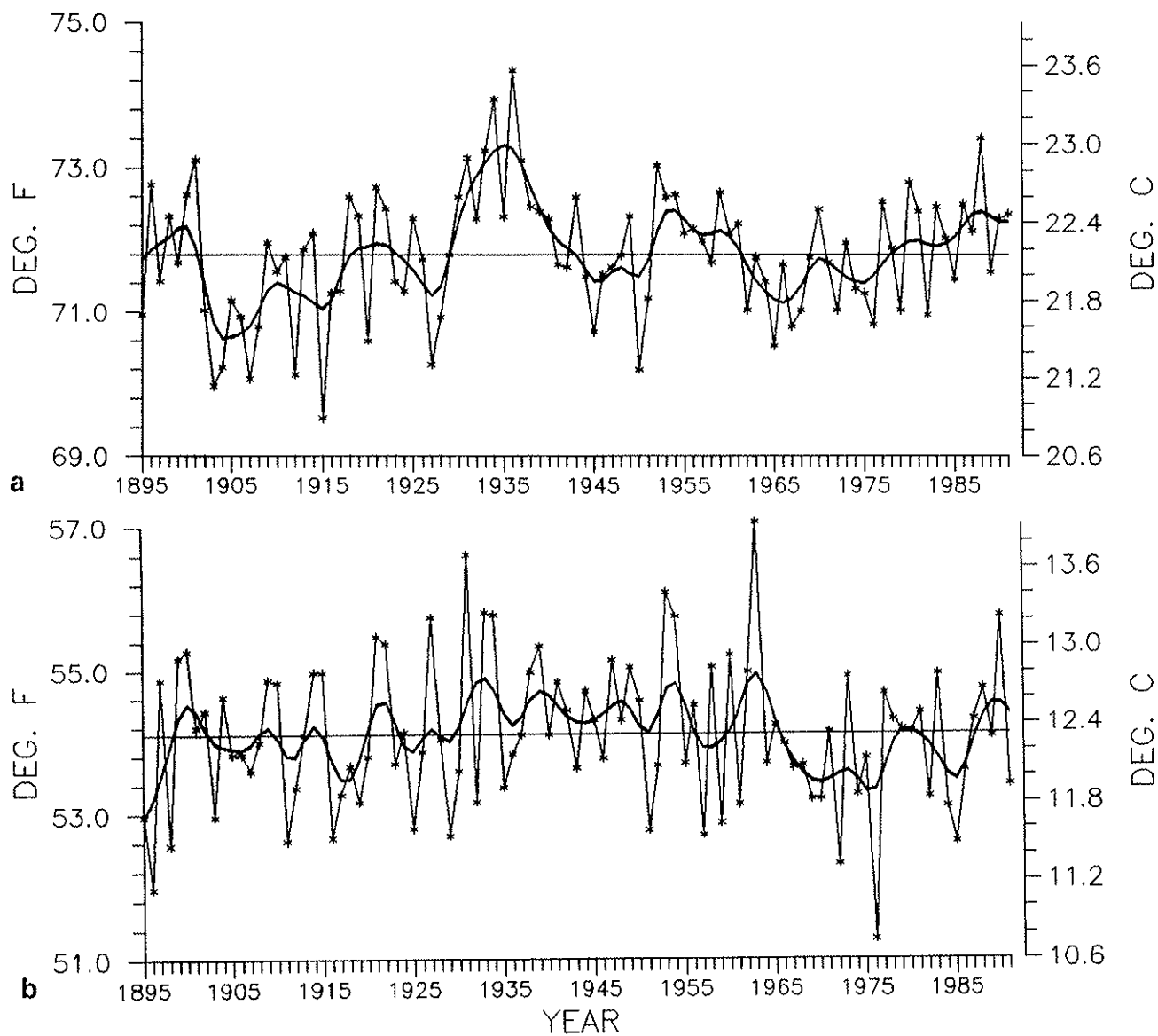
Fig. 18. Time series of temperature averaged over the contiguous United States and a binomially filtered curve for a) JJA and b) SON 1991.
