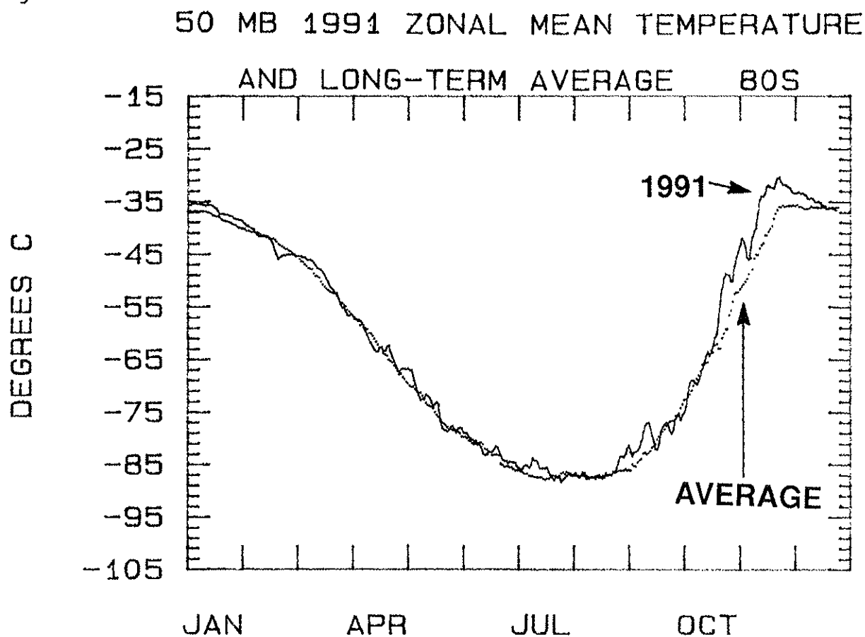
Fig. 43. Daily zonal average 80^{\circ}\text{S} 50 mb (approx. 20 KM) temperatures for 1991 (solid line) relative to the 1978-1991 average (dashed line).
