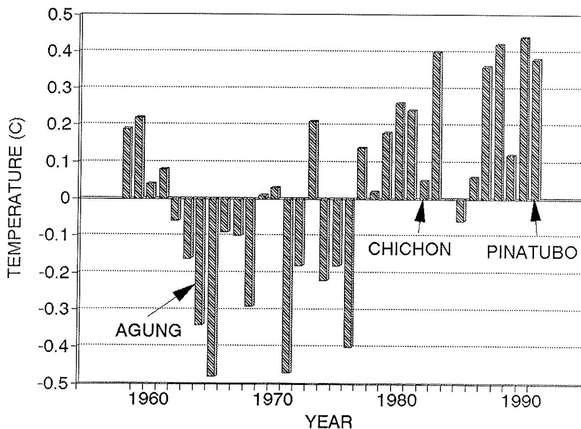
Fig. 39. Time series of global tropospheric (850 - 300 mb) temperature anomalies derived from radiosonde data, data supplied by Jim Angell.
