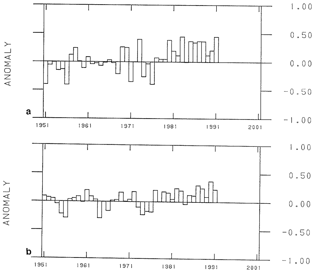
Fig. 14. Time series of estimated Southern Hemisphere surface temperature anomalies for a) January - June and for b) July - December. Global temperature anomaly estimates are formed from area weighted averages of station anomalies over a 2^{\circ} latitude by 2^{\circ} longitude grid.
