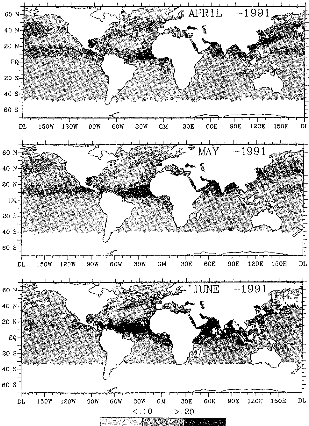
Fig. 46. Monthly mean aerosol optical thickness at a wavelength of 0.5 micrometers as derived from the AVHRR instrument on the NOAA-11 satellite for April through June of 1991. White represents no measurements possible, either due to poor solar illumination, persistent cloud cover, or land areas.
