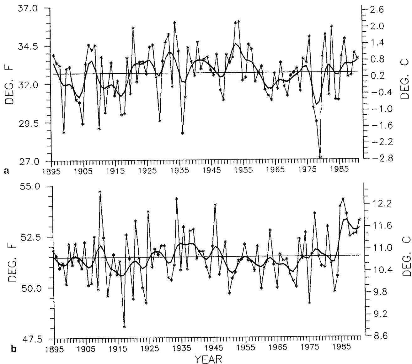
Fig. 17. Time series of temperature averaged over the contiguous United States and a binomially filtered curve for a) DJF 1990-91 and b) MAM 1991.
