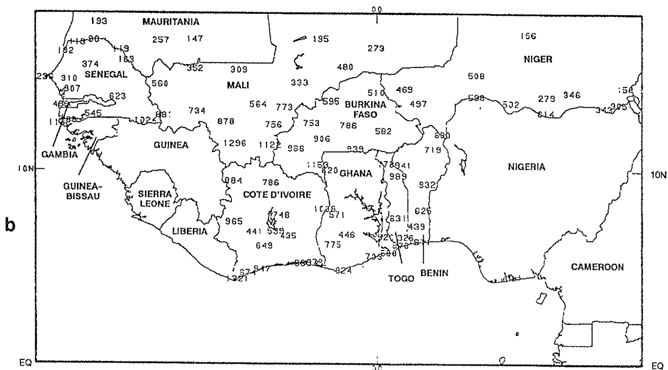
Fig. 32. a) West African Sahel percent of normal precipitation during May 1 - September 30, 1991 and b) West African Sahel total precipitation (mm) during May 1 - September 30, 1991.
