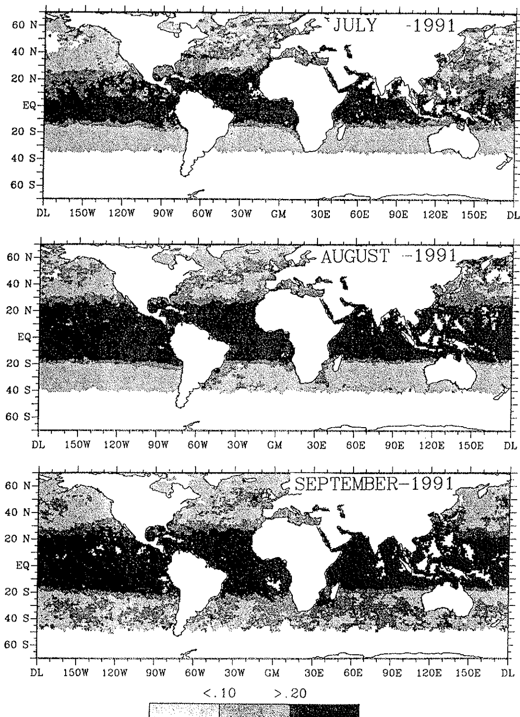
Fig. 47. Monthly mean aerosol optical thickness at a wavelength of 0.5 micrometers as derived from the AVHRR instrument on the NOAA-11 satellite for July through September of 1991. White represents no measurements possible, either due to poor solar illumination, persistent cloud cover, or land areas.
