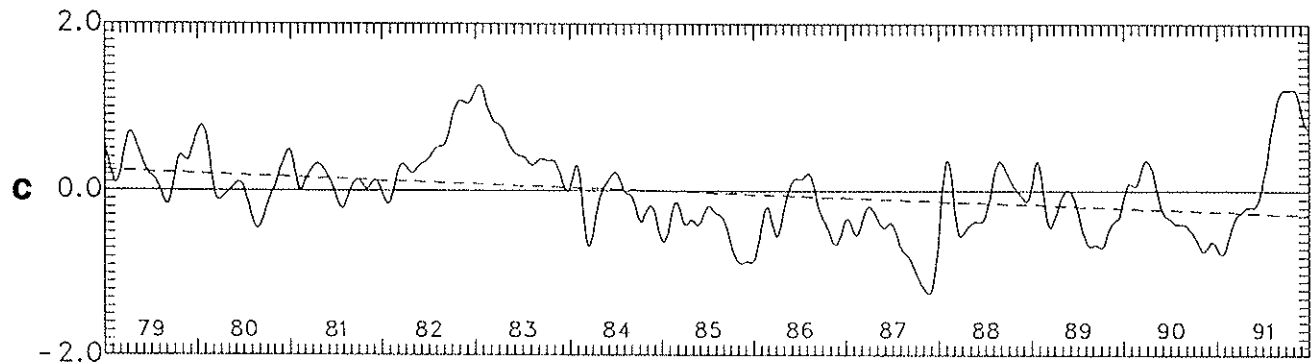
Fig. 41. Time series of a) global, b) Northern Hemisphere and c) Southern Hemisphere lower stratospheric temperature anomalies derived from satellite Microwave Sounding Unit (MSU) observations.
