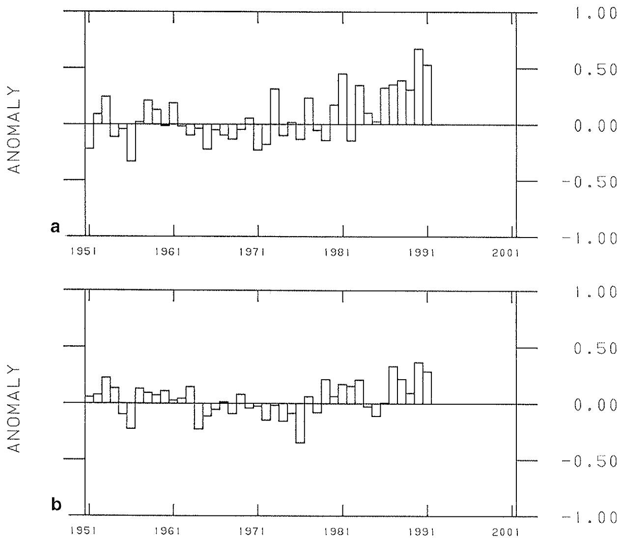
Fig. 11. Time series of estimated global surface temperature anomalies for a) January - June and for b) July - December. Global temperature anomaly estimates are formed from area weighted averages of station anomalies over a 2^{\circ} latitude by 2^{\circ} longitude grid.
