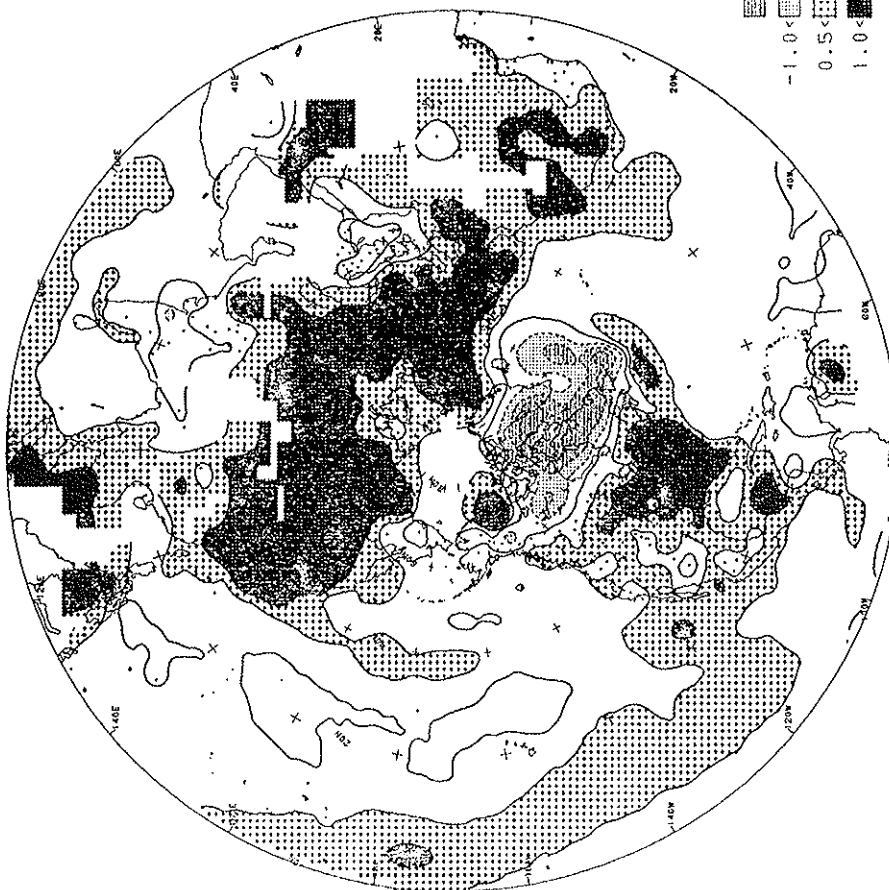
Fig. 7. Northern Hemisphere surface temperature anomaly for 1990. Analysis based on station data over land and sea surface temperature (SST) over the water. Anomalies for station data are from the 1951-80 base period, while SST anomalies are computed as departures from the COADS/ICE climatology (Reynolds, 1988). Contour interval is 0.5^{\circ}\text{C} .
