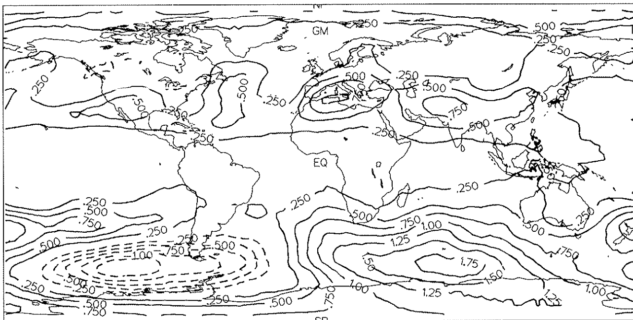
Fig. 42. Lower stratospheric temperature anomalies for 1991 computed from the 1979-1991 base period. Contour interval is 0.25^{\circ}\text{C} , negative anomalies are dashed.
