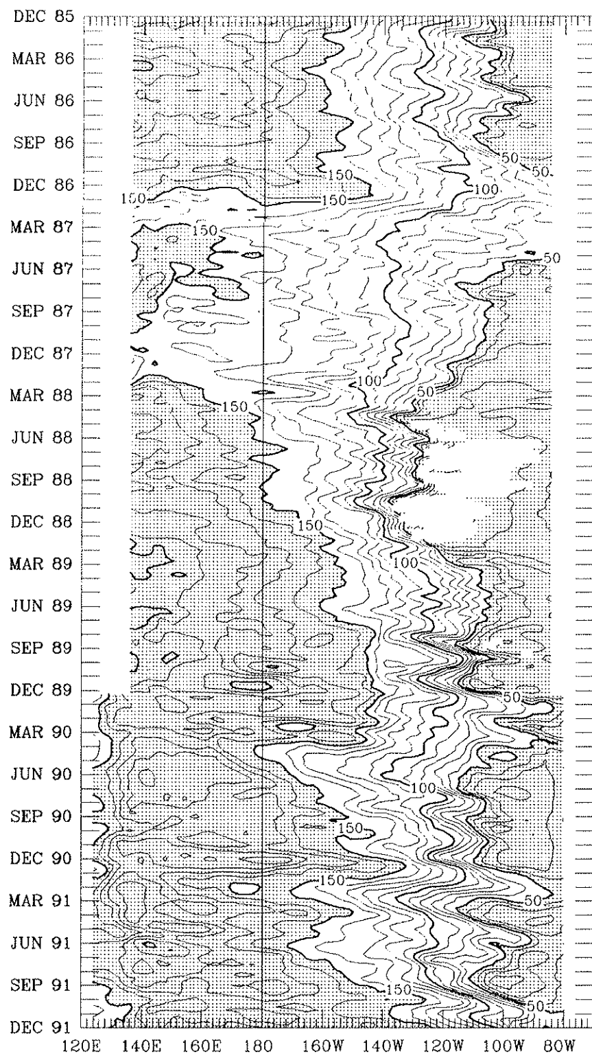
Fig. 2. Depth of the 20°C isotherm along the equator in the Pacific Ocean. Data are derived from an analysis system which assimilates oceanic observations into an oceanic GCM (Leetmaa and Ji 1989). The contour interval is 10 m with shading for values less than 50 m and also for values greater than 150 m.
