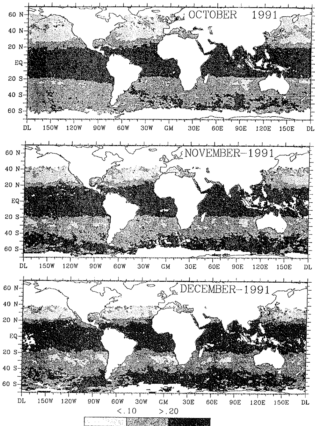
Fig. 48. Monthly mean aerosol optical thickness at a wavelength of 0.5 micrometers as derived from the AVHRR instrument on the NOAA-11 satellite for October through December of 1991. White represents no measurements possible, either due to poor solar illumination, persistent cloud cover, or land areas.
