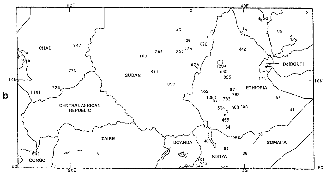
Fig. 33. a) East African Sahel percent of normal precipitation during May 1 - September 30, 1991 and b) East African Sahel total precipitation (mm) during May 1-September 30, 1991.
