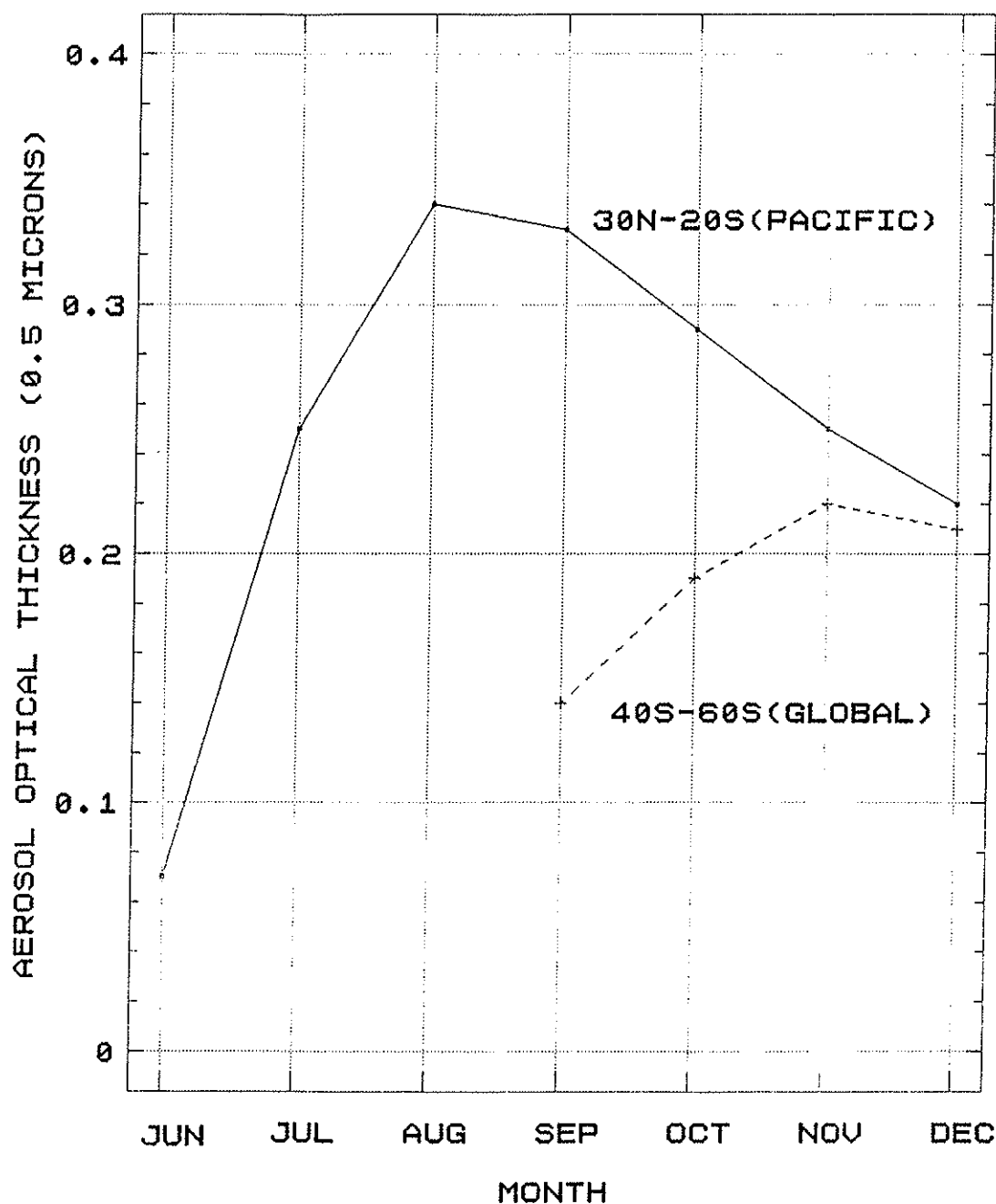
Fig. 49. Total monthly mean aerosol optical thickness as function of month for two latitude bands, one confined to the Pacific Ocean between 20^{\circ}\text{S} and 30^{\circ}\text{N} containing the Mt. Pinatubo aerosol layer, and another from 40^{\circ}\text{S} to 60^{\circ}\text{S} , containing both Mt. Pinatubo and Mt. Hudson aerosol.
