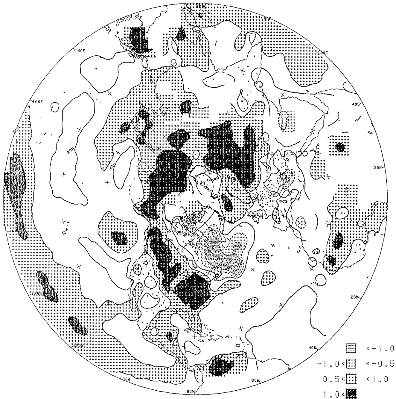
Fig. 5. Northern Hemisphere surface temperature anomaly for 1991. Analysis based on station data over land and sea surface temperature (SST) over the water. Anomalies for station data are from the 1951-1980 base period, while SST anomalies are computed as departures from the COADS/ICE climatology (Reynolds, 1988). Small plus signs indicate locations of data over land. Contour interval is 0.5^{\circ}\text{C} , with negative anomalies dashed.
