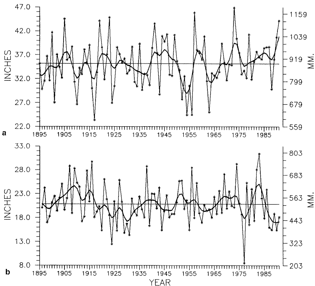
Fig. 27. a) Annual total precipitation for the South region of the United States from 1895 through 1991 and b) October-March total precipitation for the West region of the United States from 1895-96 through 1990-91. Asterisks are actual values; binomially filtered values are indicated by the solid line.
