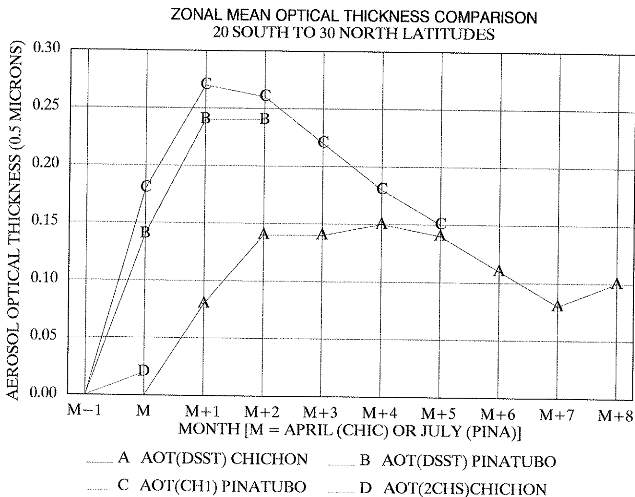
Fig. 50. Monthly mean stratospheric aerosol optical thickness (tropospheric mean of 0.07 removed) as a function of month for the latitude band 20°S to 30°N after El Chichon and Mt. Pinatubo. Curves A and B were derived from sea surface temperature error analyses, and curves C and D from reflected radiation retrieval algorithms.
