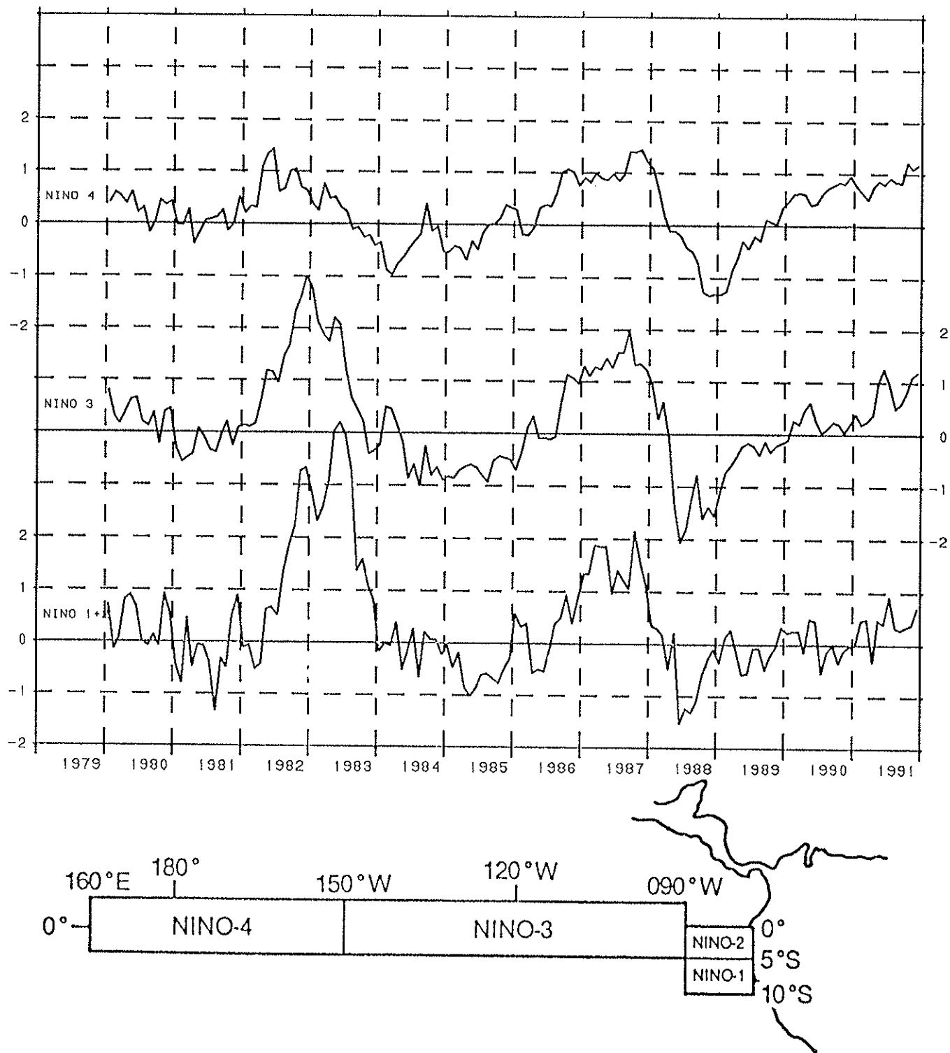
Fig. 4. Equatorial Pacific sea surface temperature anomaly indices ( ^{\circ}\text{C} ) for the areas indicated at the bottom of the figure. Niño 1+2 is the average over the Niño 1 and Niño 2 areas. Anomalies are computed with respect to the COADS/ICE climatology (Reynolds 1988).
