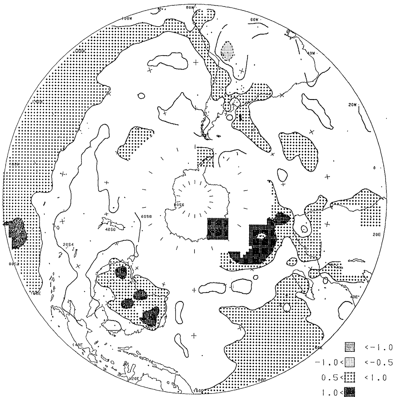
Fig. 6. Southern Hemisphere surface temperature anomaly for 1991. Analysis based on station data over land and sea surface temperature (SST) over the water. Anomalies for station data are from the 1951-1980 base period, while SST anomalies are computed as departures from the COADS/ICE climatology (Reynolds, 1988). Small plus signs indicate locations of data over land. Contour interval is 0.5^{\circ}\text{C} , with negative anomalies dashed.
