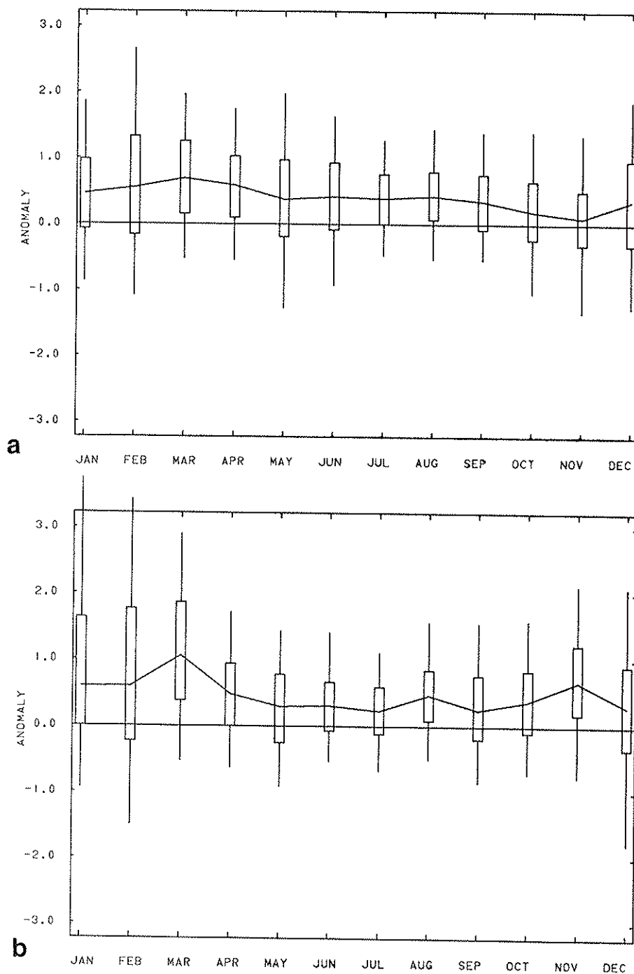
Fig. 12. Global monthly surface temperature index based on the average temperature anomalies in 2^{\circ} latitude by 2^{\circ} longitude areas over land for a) 1991 and for b) 1990. The solid line in each panel represents the 50%, or median, temperature anomaly for each month. Each "box" delineates the temperature anomalies at the 70th and 30th percentiles while the "whiskers" (lines) delineate the 90th and 10th percentile values. The anomalies are taken with respect to the 1951 to 1980 base period.
