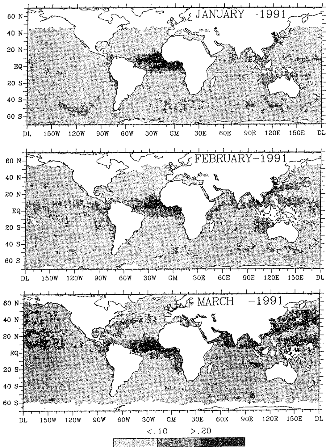
Fig. 45. Monthly mean aerosol optical thickness at a wavelength of 0.5 micrometers as derived from the AVHRR instrument on the NOAA-11 satellite for January through March of 1991. White represents no measurements possible, either due to poor solar illumination, persistent cloud cover, or land areas.
