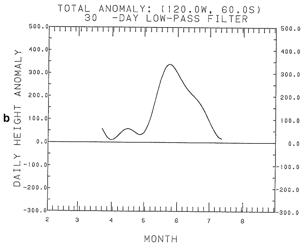
Fig. 52. Time series of daily (a) total height anomalies and (b) intermonthly (periods greater than 30 days) height anomalies during April-June 1991. Units of anomalies are meters.
