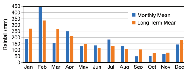
FIG. 7.32. 2016 monthly precipitation totals (mm; 1981–2010 base period) in Mauritius. (Source: Mauritius Meteorological Services.)
