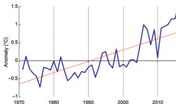
FIG. 7.6. Annual mean temperature anomalies (°C, blue line; 1981–2010 base period) for Mexico. Red line represents the linear trend over this period. (Source: Meteorological Service of México.)
