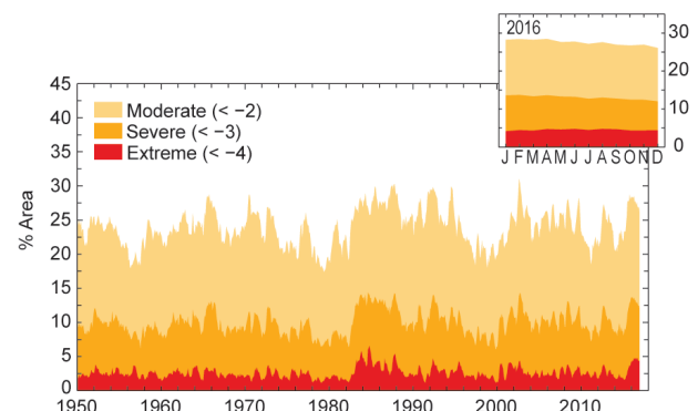
FIG. 2.29. Percentage of global land area (excluding ice sheets and deserts) with scPDSI indicating moderate ( <-2 ), severe ( <-3 ) and extreme ( <-4 ) drought for each month of 1950–2016. Inset: 2016 monthly values.
