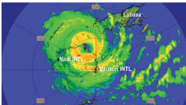
FIG. 7.57. Radar image showing Tropical Cyclone Winston making landfall over Viti Levu, Fiji, on 20 Feb 2016 (Source: Fiji Meteorological Service.)
