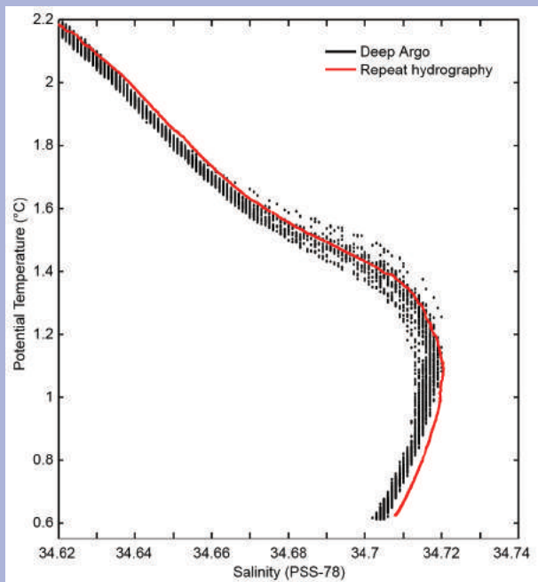
FIG. SB3.3. Temperature/salinity ( \theta/S ) relationship in the southwest Pacific basin. Black symbols indicate 75 Deep SOLO float profiles spread over 30.4°–35.2°S and 172.8°–174.5°W between Feb 2016 and Jan 2017 ( www.usgodae.org/ftp/outgoing/argo/dac/aoml/5902447 ). The red line is a single cast at 35°S from the PI5S repeat hydrographic transect of June 2016 (Source: data courtesy of Bernadette Sloyan, CSIRO.)
