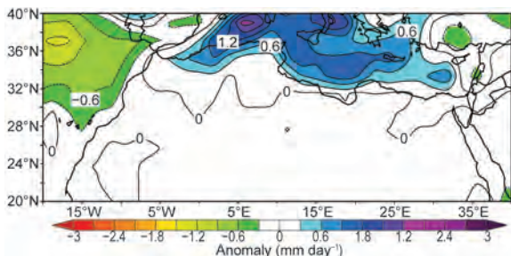
FIG. 7.15. Dec–Feb 2014/15 mean precipitation anomaly ( \text{mm day}^{-1} ; base period 1981–2010). (Source: NCEP–NCAR reanalysis.)
