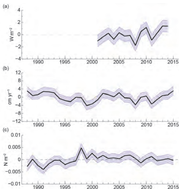
Fig. 3.14. Annual-mean time series of global averages of (a) net surface heat flux ( Q_{\text{net}} ) from the combination of CERES EBAF SW+LW and OAF flux LH+SH, (b) net freshwater flux ( P-E ) from the combination of GPCP P and OAF flux E, and (c) wind stress magnitude from OAF flux high-resolution vector wind analysis. Shaded areas indicate one standard deviation of annual-mean variability.
