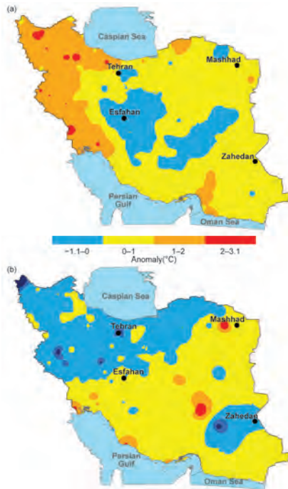
FIG. 7.49. Seasonal mean surface temperature anomalies ( ^{\circ}\text{C} ) in (a) summer (Jun–Aug) and (b) autumn (Sep–Nov). (Source: I.R. of Iran Meteorological Organization & National Center for Drought and Disaster Risk Management.)
