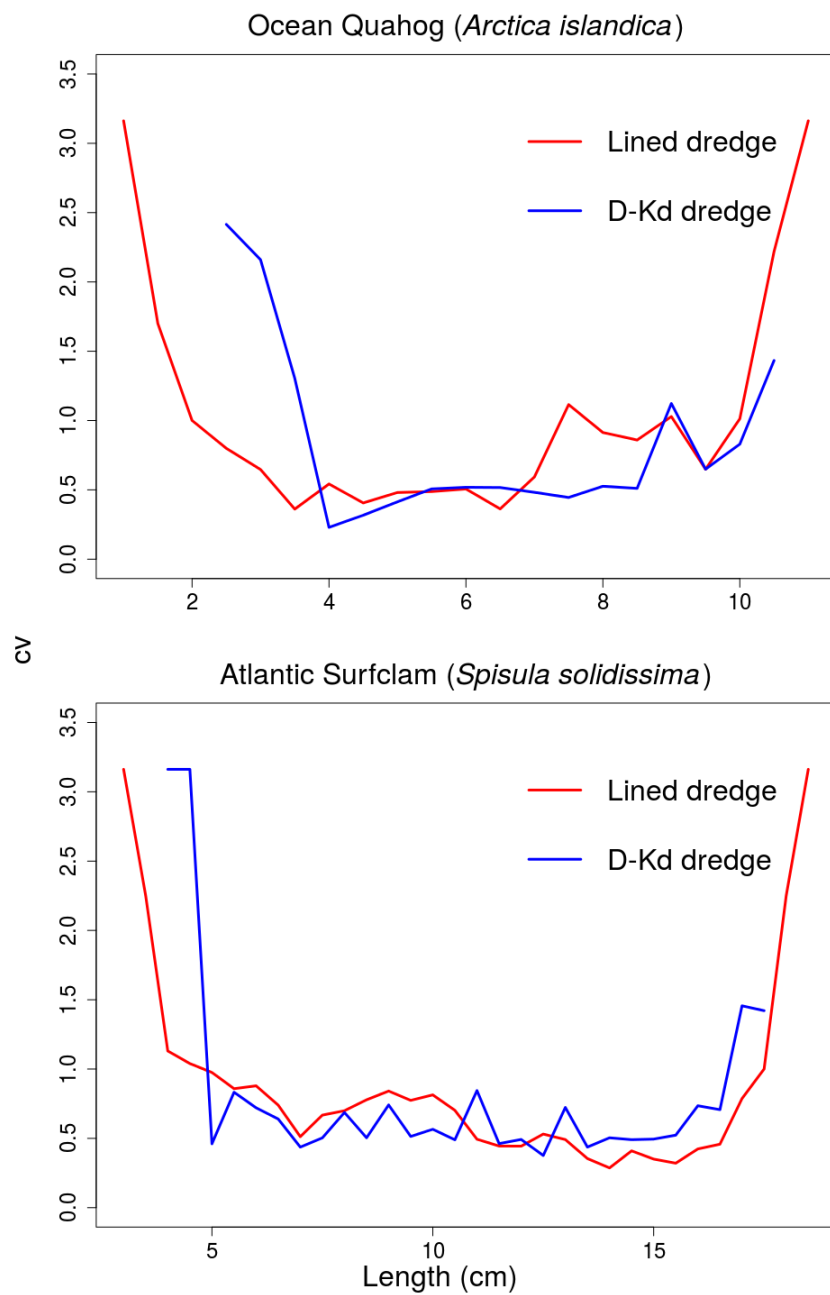
Figure 4. Coefficient of variation (cv) in catch at size for each dredge fishing Atlantic surfclam ( Spisula solidissima ; n=10 tows; 5 mm size bins) and ocean quahogs ( Arctica islandica ; n=10 tows; 5 mm size bins).
