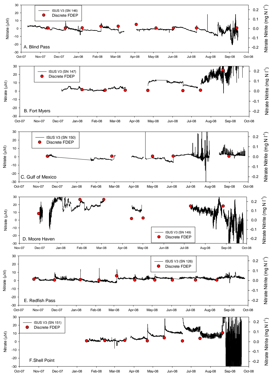
Figure 2-8A-F. Time-series of nitrate concentrations at instrument depth determined optically by the ISUS and standard method chemical assays of total nitrates (nitrate plus nitrite). Burst optical data were collected hourly and data was binned to 10 seconds average calls of nitrate concentration at a sampling rate of 1 Hz. (Photo courtesy of Dr. Eric Milbrandt/Sanibel-Captiva Conservation Foundation)
