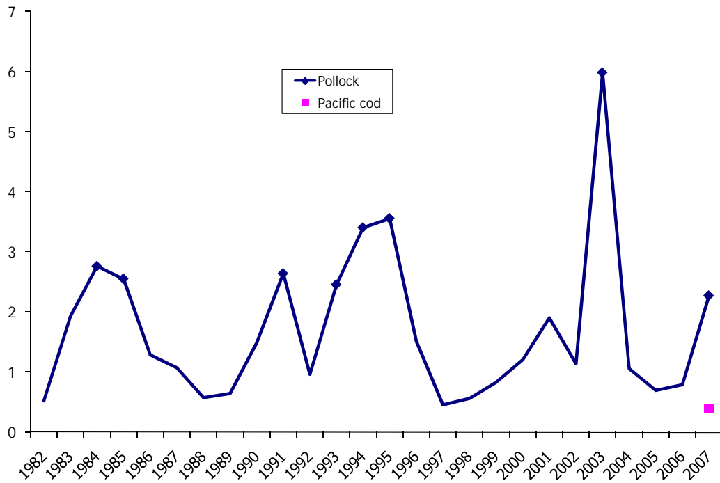
Figure 4.15 Ratio of average NMFS summer trawl survey CPUE inside Steller sea lion critical habitat over the average CPUE outside of critical habitat by year (top panel) and by 5-year periods (bottom panel) for pollock and Pacific cod.
