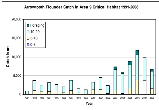
Figure RCA 4.7. (Continued). Note: the scale of these figures may differ from those on the previous page – in some cases by several orders of magnitude.
