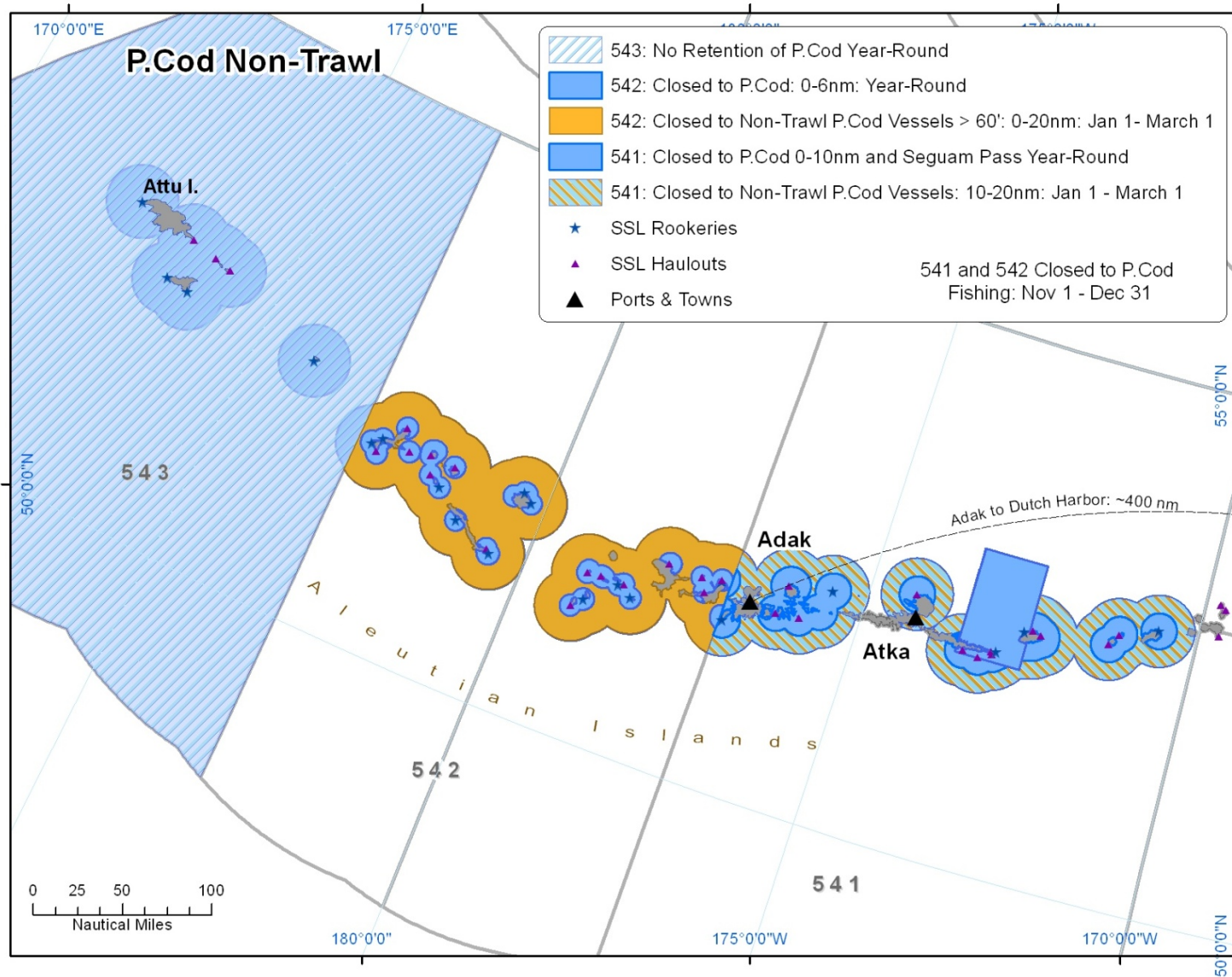
Figure 8.5. Map of the RPA for Pacific cod nontrawl fisheries in Areas 543, 542, and 541.
