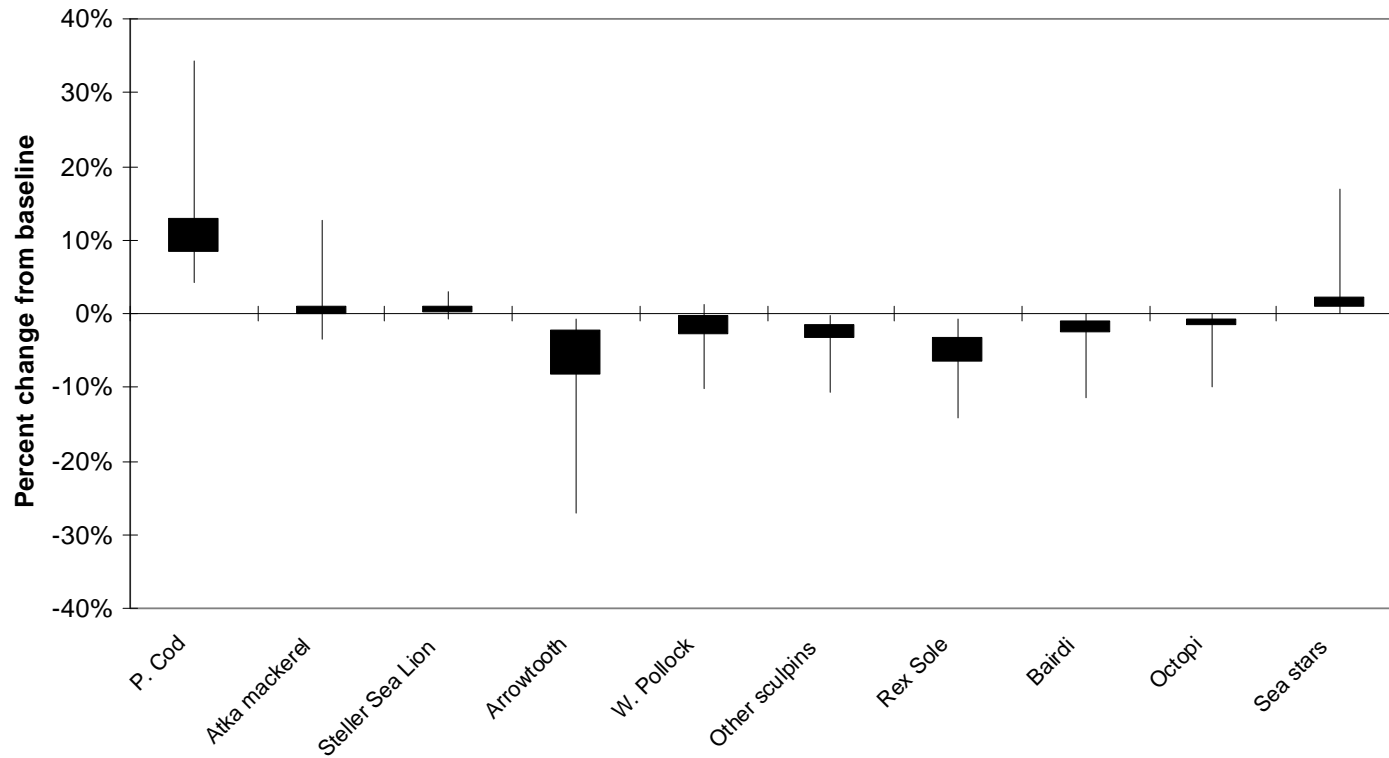
Figure 8.6. The effects on the Aleutian Islands food web model (percent change of biomass from baseline) of reducing Pacific cod mortality by 10% (manipulated species shown by arrow). Only selected species are shown. Bars and lines show 50% and 95% of results obtained from 500 ecosystems drawn from parameter distributions based on uncertainty in input parameters of biomass, production rates, consumption rates, and diets, as described in Aydin et al. 2007 (Source: Aydin 2010).
