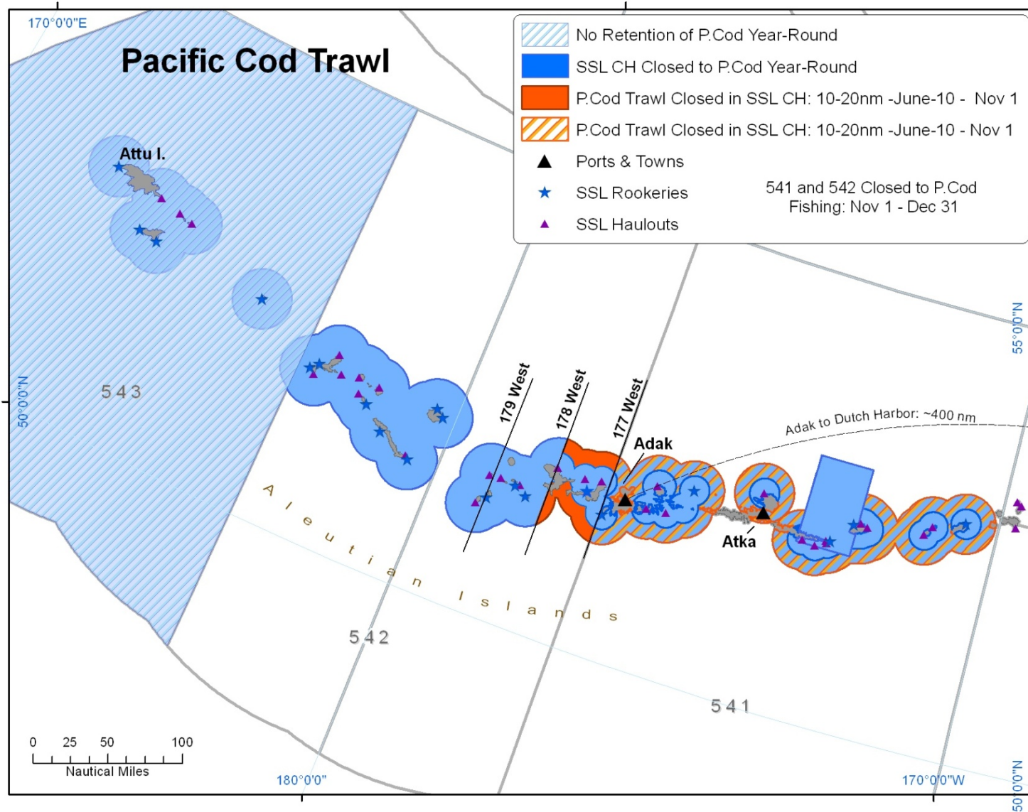
Figure 8.4. Map of the RPA for Pacific cod trawl fisheries in Areas 543, 542, and 541.
