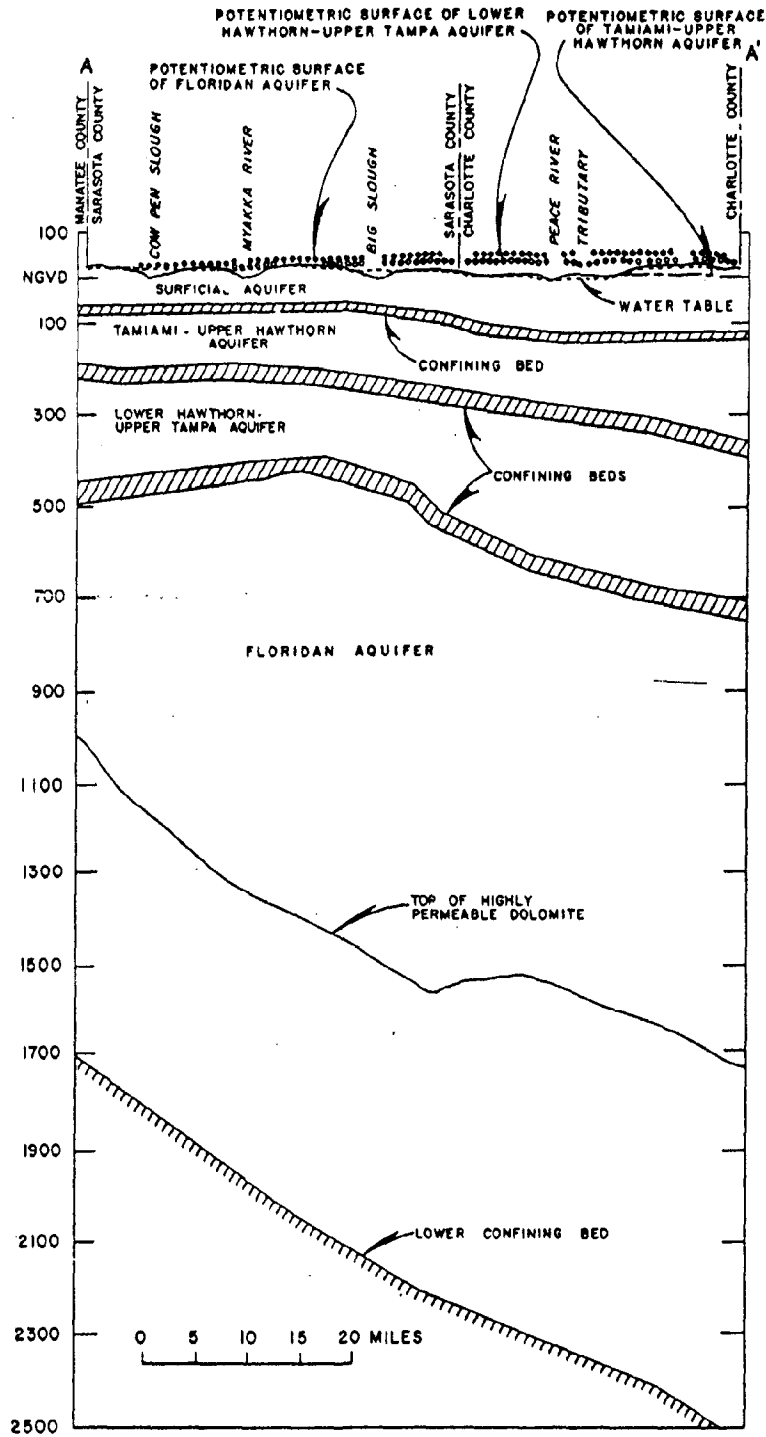
Figure 20. Generalized hydrogeologic section along a line extending from the Manatee-Sarasota County line northwest of Myakka River State Park to the Charlotte-Lee County line just east of U.S. Route 41. It crosses the Myakka River just above Lower Myakka Lake (Wolansky 1983).
