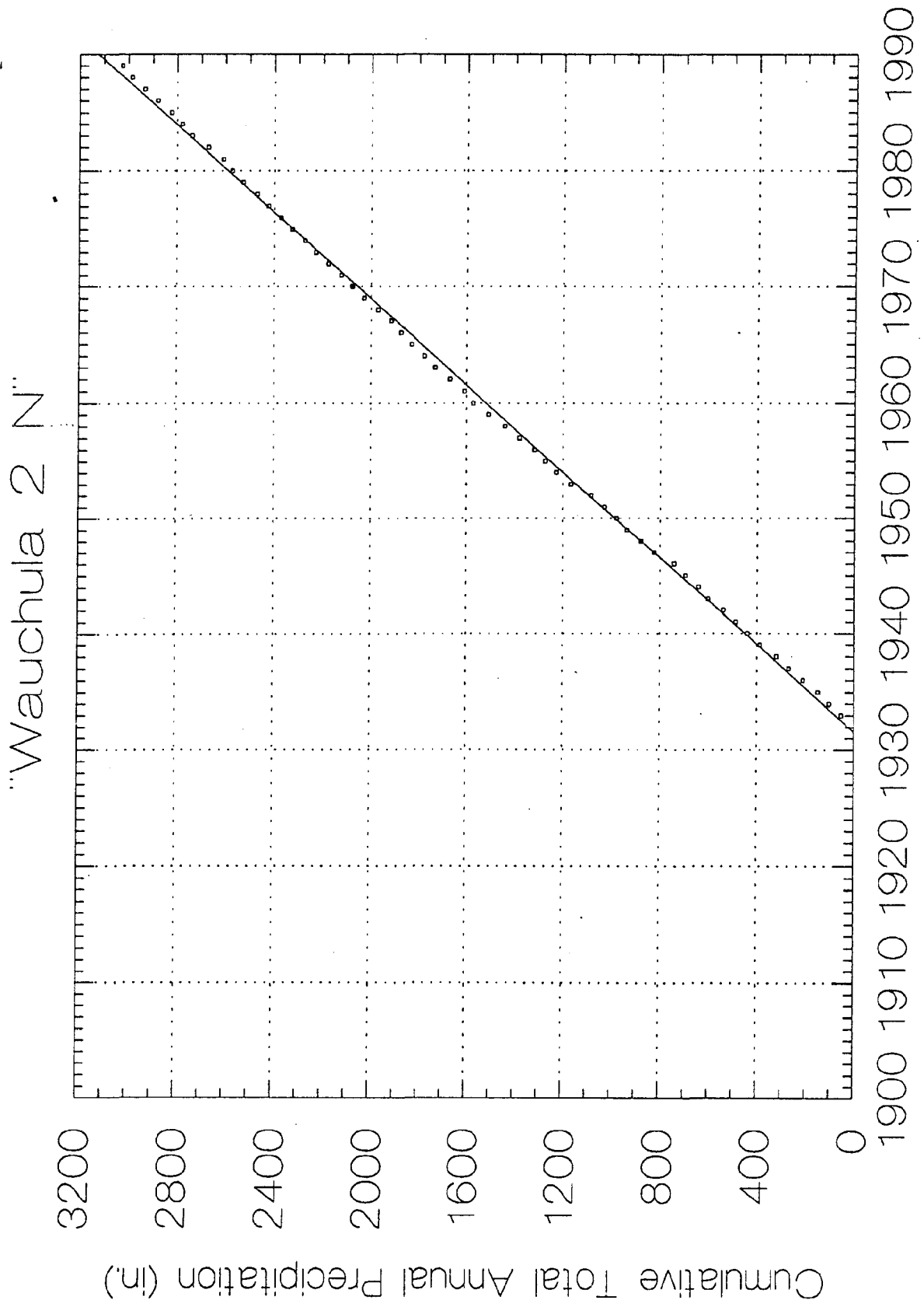
Figure 15. Cumulative total annual precipitation at Wauchula 2 N.
