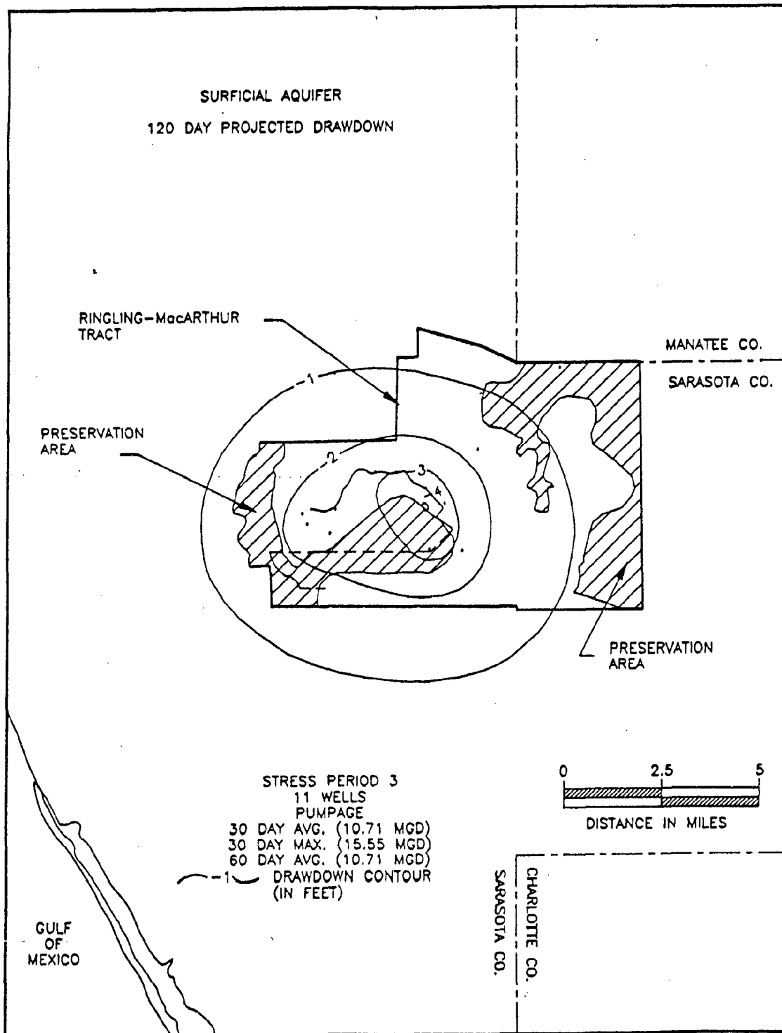
Figure 32. The projected drawdown in the Surficial Aquifer resulting from a 120-day stress test on pumping from the Floridan Aquifer on the Carlton Reserve (Dames and Moore 1988).
