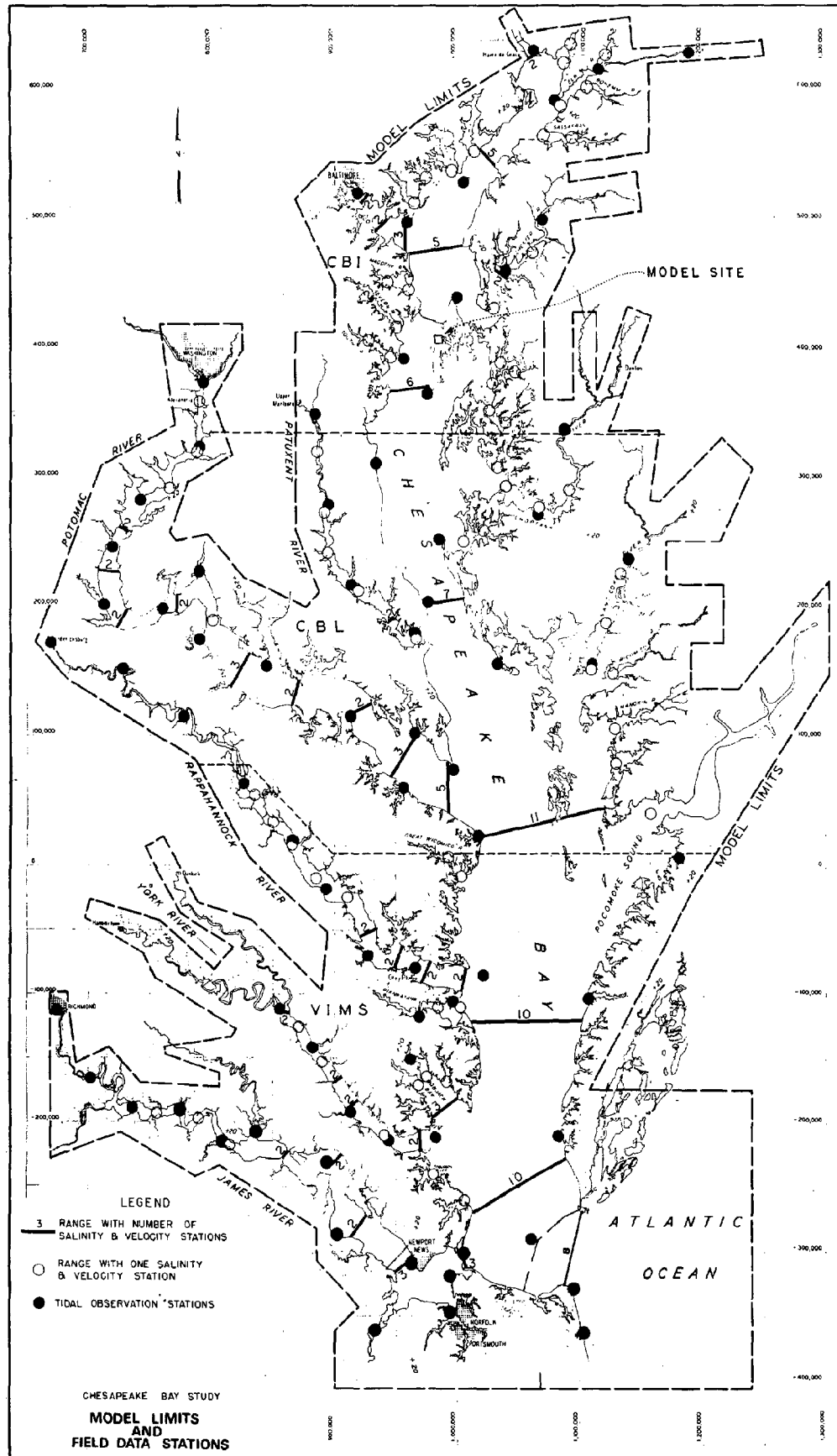
Figure 16-3: Model Limits and Field Data Stations
