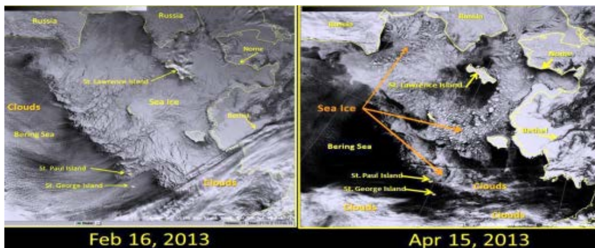
VIIRS image comparison between February 16th and April 15 th , 2013 shows sea ice melt, especially near St. Lawrence Island and south of Nunivak Island. Image courtesy of NWS Alaska.
