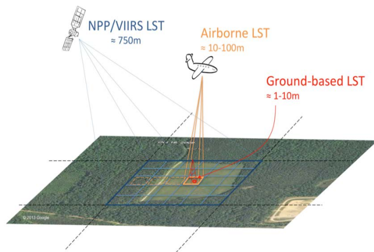
Impact of the spatial resolution on the LST derived from satellite, aircraft and ground station measurements.
