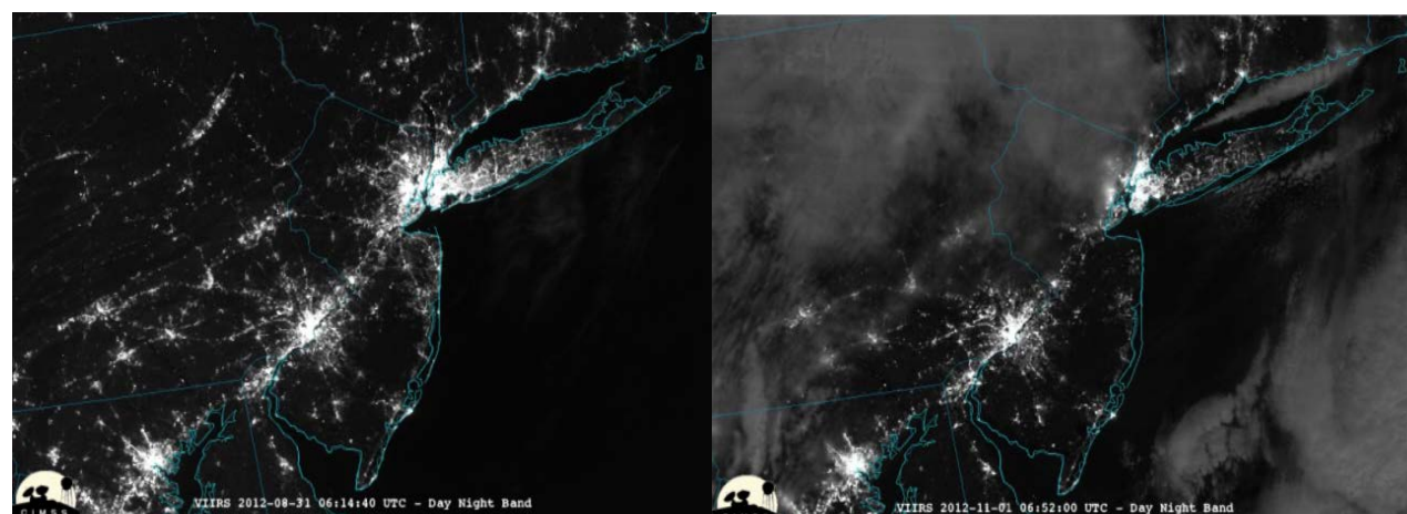
Suomi-NPP VIIRS 0.7 \mu m Day/Night Band images (pre-Sandy, and post-Sandy).
