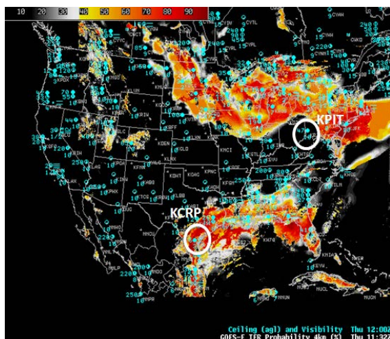
IFR probabilities computed from GOES-E
