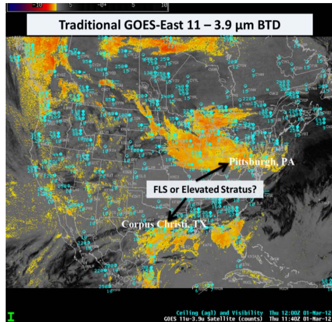
This image is a depiction of the BT product that has been traditionally used in the past to detect nighttime FLS. Yellow/orange represents FLS.
