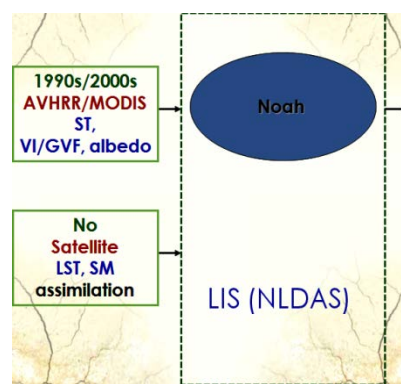
Current Noah LSM runs
