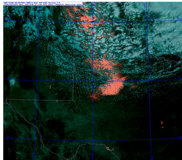
VIIRS/MODIS dust enhancement imagery over Eastern Colorado and Northern Texas.
