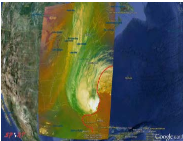
The SNPP VIIRS RGB Air Mass image using Google Earth 10/27/12 Everything to the right of the red line is very dry air at high altitude that is cutting into Sandy's tropical environment
