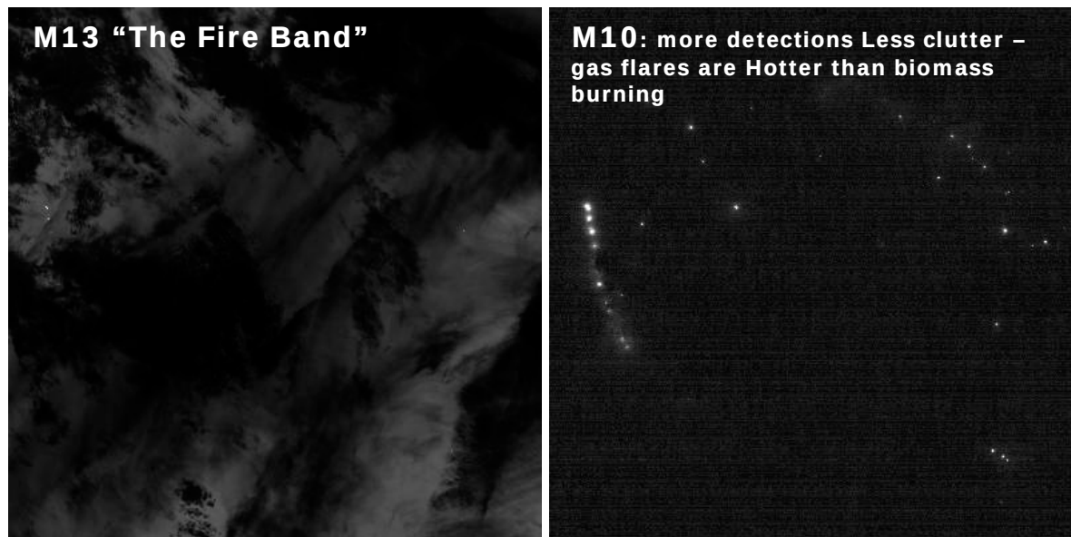
Detection of Combustion Sources Basra, Iraq Region at Night
