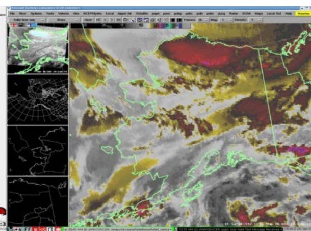
GOES Infrared (IR)
