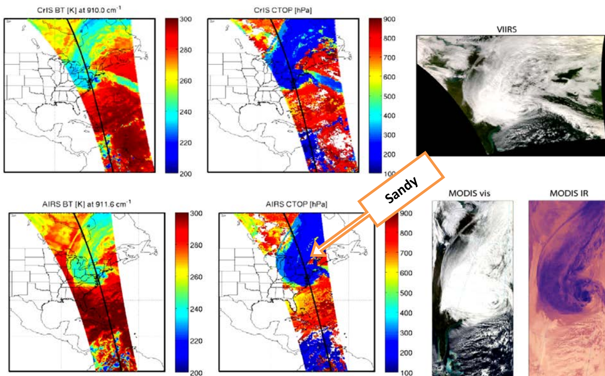
Figure 4: Hurricane Sandy (29 Oct 2012). The CrIS BT and CTOP products (Top left and middle), and the AIRS BT and CTOP products (bottom left and middle), provide a quantitative interpretation of the VIIRS (Top right), and MODIS Vis and IR images (bottom right)
