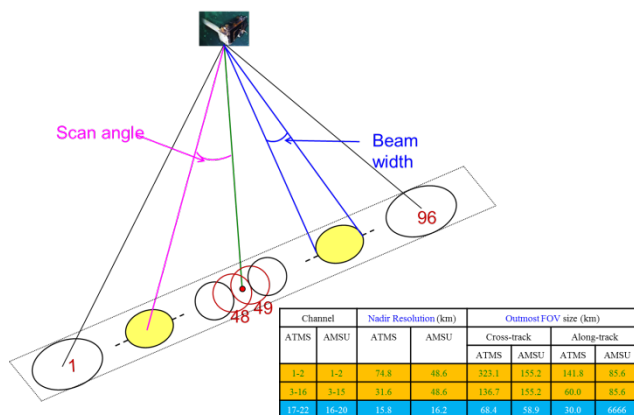
ATMS Scan Angle and Beam Width
