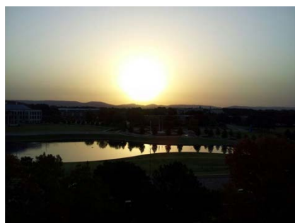
Dust-scattered sunrise over Huntsville
