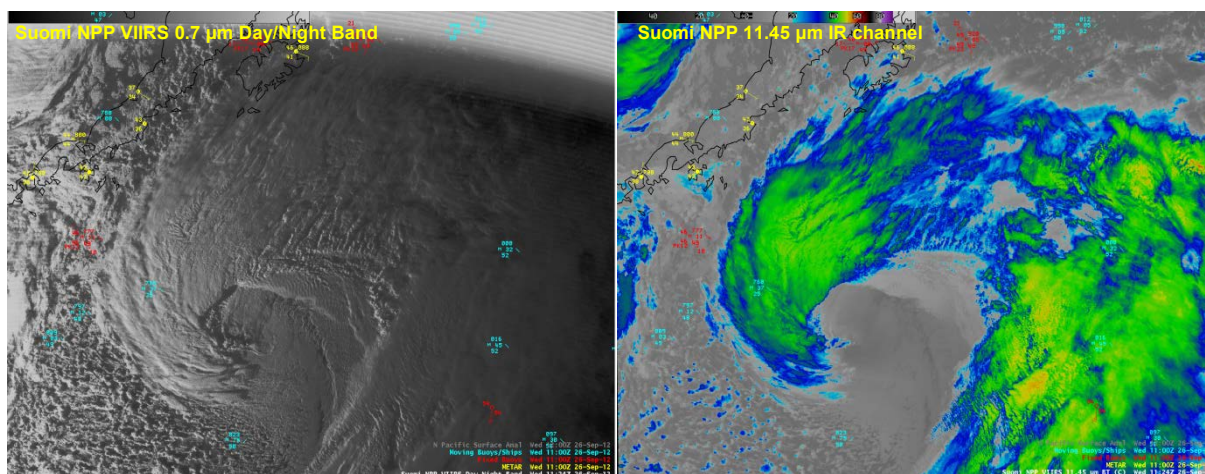
Figure 6: Powerful Gulf of Alaska Storm
