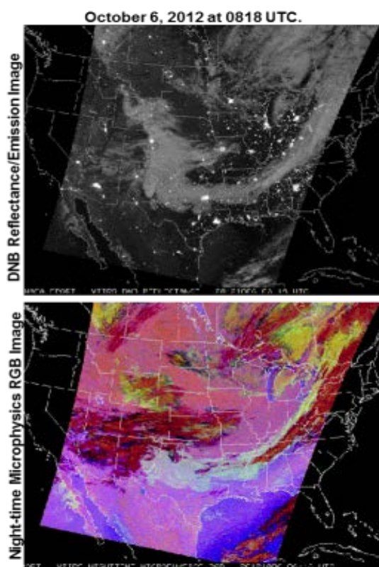
Low clouds tend to be a bright aqua color (TX and LA) Further north, low clouds exhibit a more yellow tone due to lower temperatures (WY and Great Lakes areas) Higher clouds are red and purple shades, depending on their thickness.
