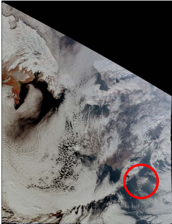
VIIRS True Color image, October 30, 2012
