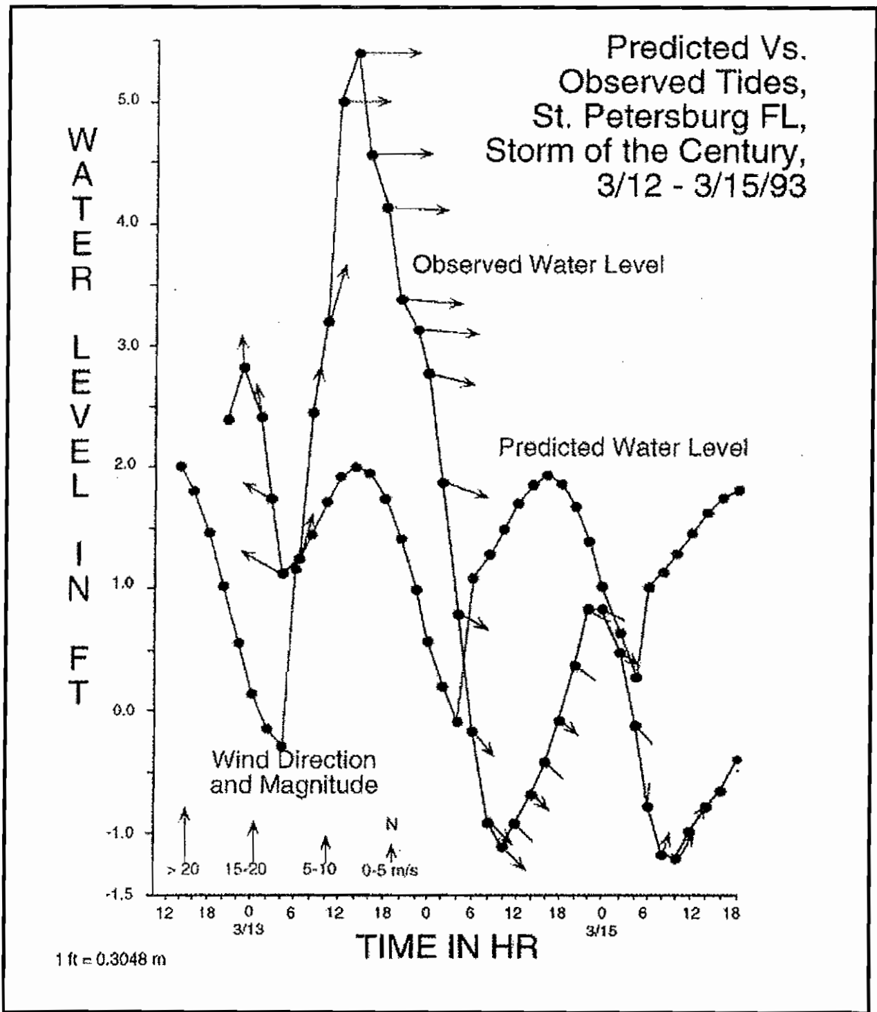
FIG. 9. Predicted vs observed tides at Saint Petersburg, Florida from 12-15 March 1993 (Department of Marine Science, University of South Florida)
