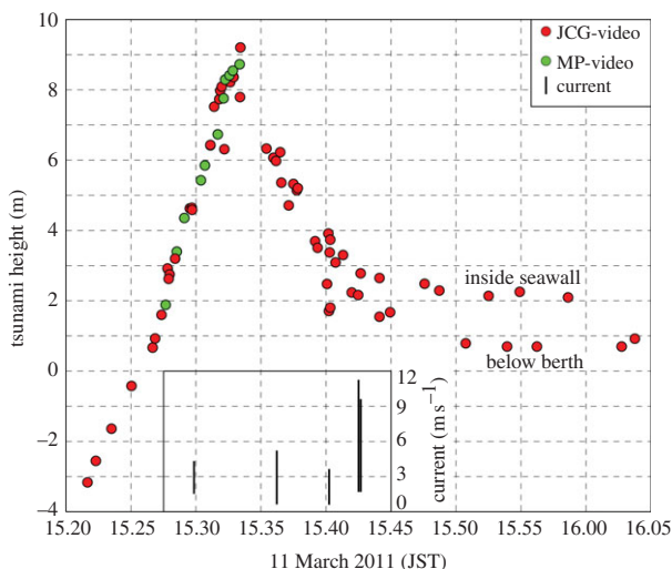
Figure 4. Hydrograph measurements using lidar, and then with high-end particle tracking methodologies, near a surviving coast guard building during the 2011 Japan tsunami. Adapted from Fritz et al. [124].
