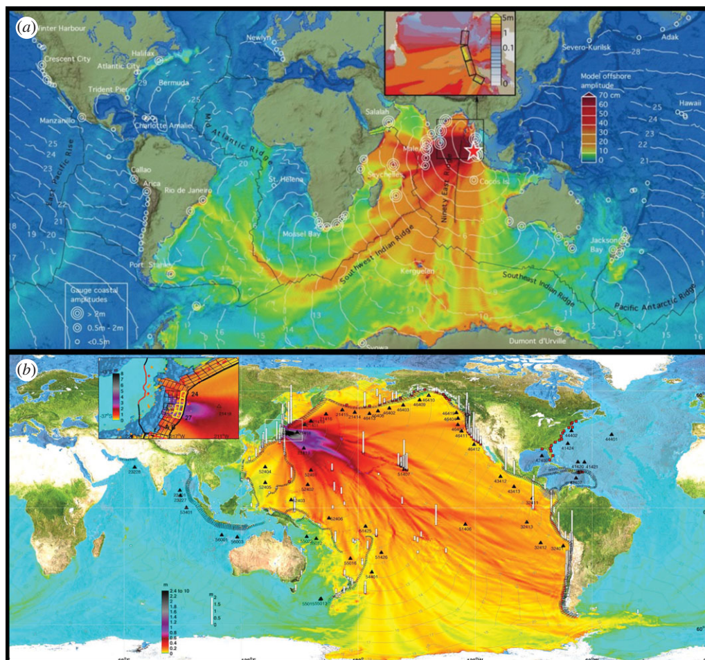
Figure 1. Global computed maximum tsunami heights of (a) the 26 December 2004 [17] and (b) the 11 March 2011 [18] tsunamis calculated from numerical model of Method of Splitting Tsunami (MOST). Contours show computed tsunami travel time. Colour-filled contours show predicted maximum tsunami amplitudes in deep water.
