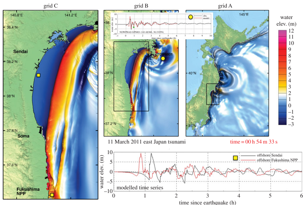
Figure 5. Results of numerical experiment that uses NOAA forecast methodology for modelling impact of the 2011 Tohoku tsunami at a portion of east coast of Japan, including the Sendai area and Fukushima NPP location. The model uses the tsunami source obtained from real-time assessment of DART data. Computations are done with MOST, using telescoping set of grids with high-resolution flooding simulation, the same method as in NOAA tsunami flooding forecast. The simulation shows up to 10 m amplitudes offshore Fukushima and Sendai, sufficient to flood a few miles into the Sendai Plain and produce over 13 m run-up at Fukushima. Modern computers with parallelized MOST can run such a model in only few minutes, potentially reducing the computations to seconds. The source definition depends entirely on the measurement data availability. The time of data inversion is negligible. Therefore, forecasts of this accuracy, even with existing data and computational capabilities, are possible within 1 h. With better measurements as planned along Japan coasts and faster computations, such forecast could be obtained in just a few minutes after an earthquake within a decade.
