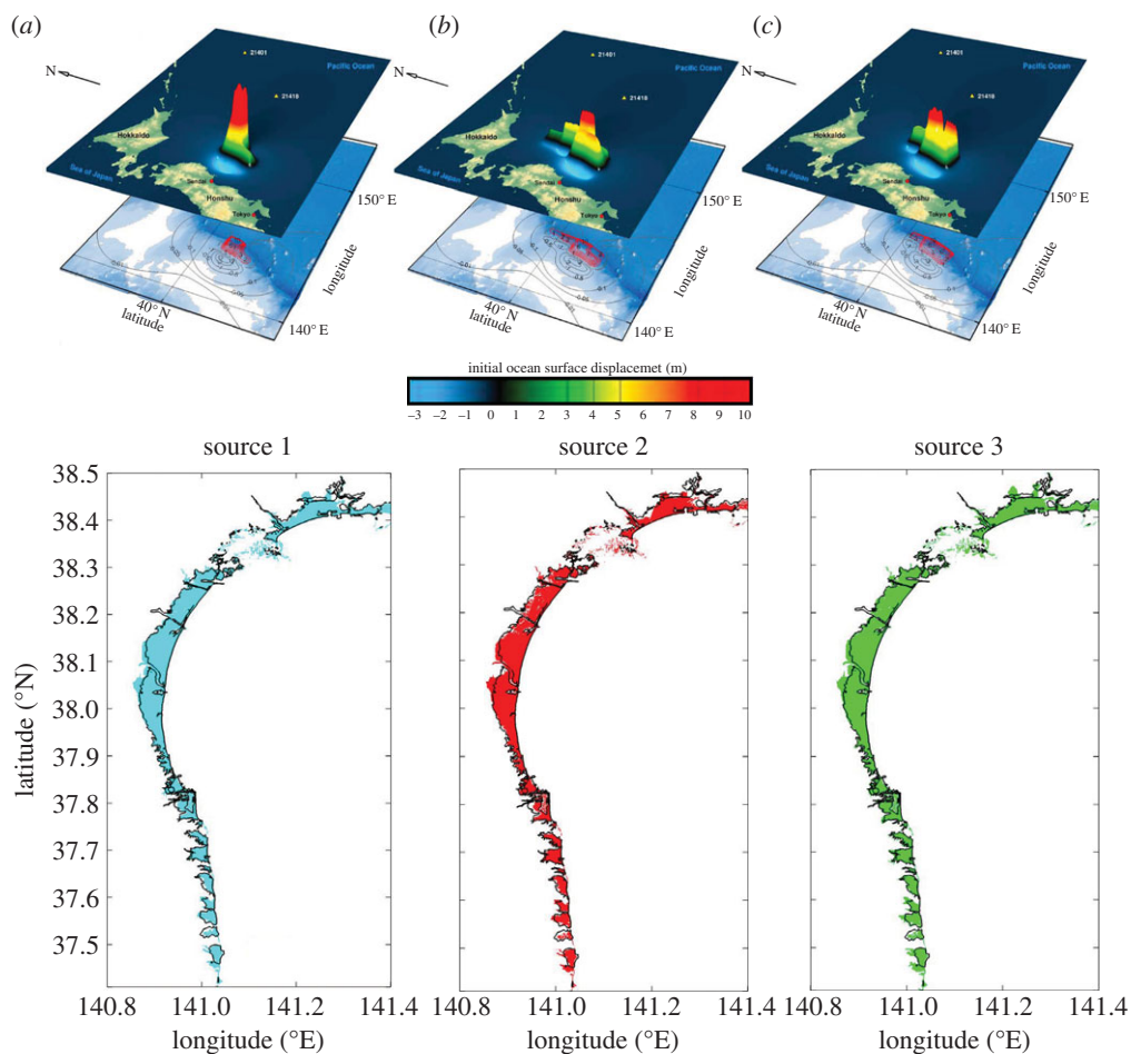
Figure 3. Run-up distribution along the Japan coast after the 2011 tsunami using MOST and inversion from one, two, and three tsunameter inversion. The timings of the inversions were approximately 40 min, 1.2 h, and 1.75 h after the event, respectively. The solid line is the field measurements.
