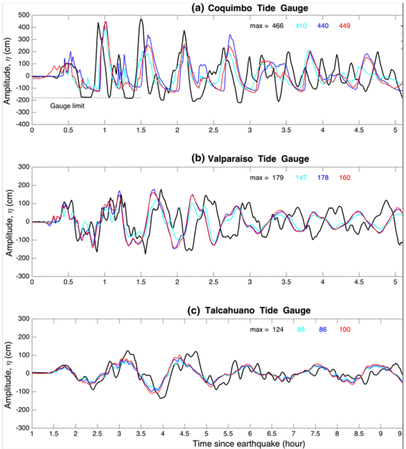
Figure 7 shows that all three tsunami sources obtained in real time are capable of producing good near-field model-data comparisons for several consecutive tsunami waves amplitudes, following the general trend of observed tsunami time series for almost 6 h. Crude model bathymetry near sea-level gages explains the time shift between model observed waves peaks, since mismatch between model and real bottom in a shallow bay would result
