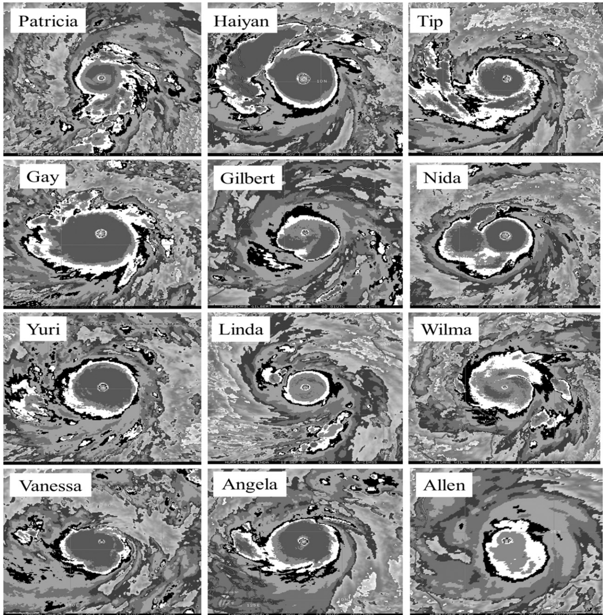
FIG. 1. IR images with the Dvorak BD enhancement applied to the 12 TCs in Table 2 at their respective maximum intensities, remapped to a common projection and scale.
