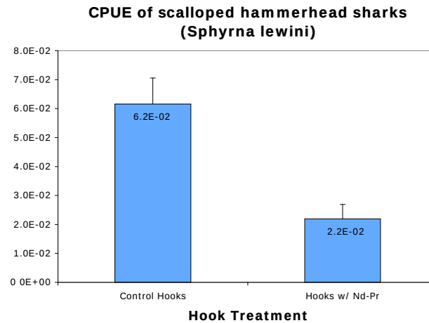
Figure A1.3. Catch per unit effort of scalloped hammerhead sharks on longlines with Nd/Pr alloy attached versus control hooks.
