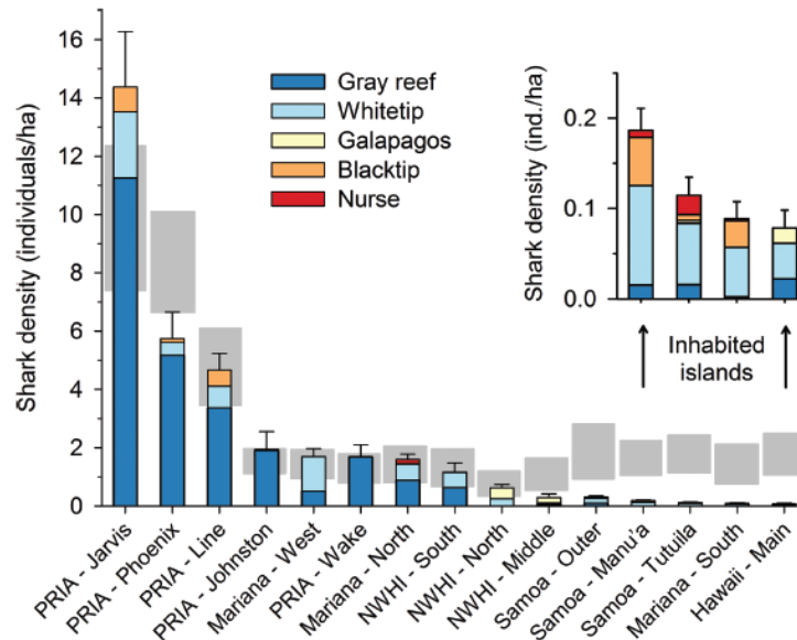
Figure A1.1. Mean (SE) observed densities of reef sharks in the U.S. Pacific. Colors represent actual densities; gray rectangles represent model predictions in the absence of humans.
