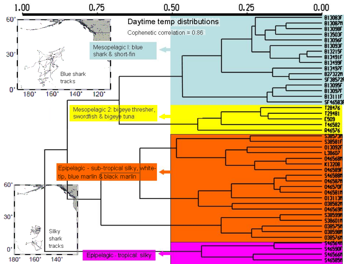
Figure A1.2. Clustered relationships among pelagic animals using daytime temperature preferences from pop-up satellite archival tags (PSATs). B = blue shark, SF = shortfin mako, T = bigeye thresher, E = bigeye tuna, R = swordfish, S = silky shark, O = oceanic whitetip shark, K = black marlin, L = blue marlin, M = male, and F = female. Inset maps show the horizontal movement patterns.
