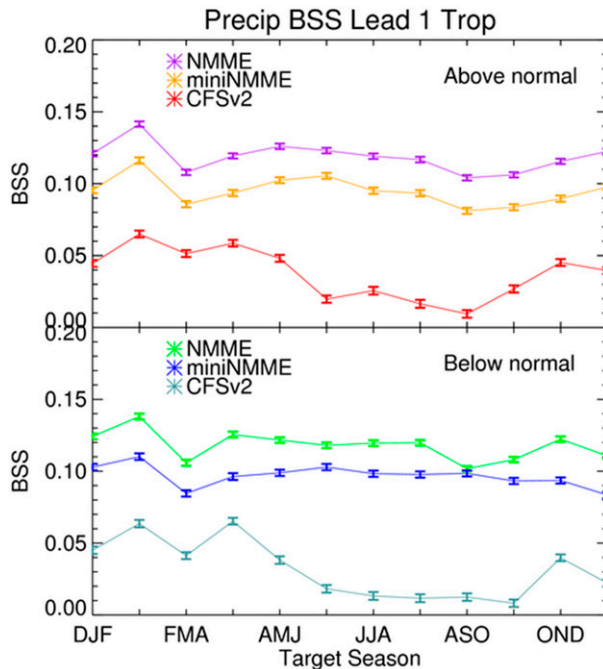
FIG. 5. As in Fig. 1, but for precipitation rate forecasts for all grid points in the tropics ( 23^{\circ}\text{S} – 23^{\circ}\text{N} ).
