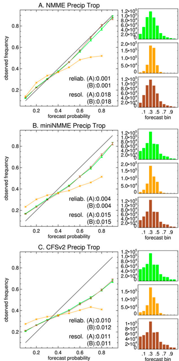
FIG. 6. As in Fig. 2, but for precipitation rate in the tropics ( 23^{\circ}\text{S} – 23^{\circ}\text{N} ). Green indicates forecasts in the above tercile, brown the below, and orange the near-normal.
