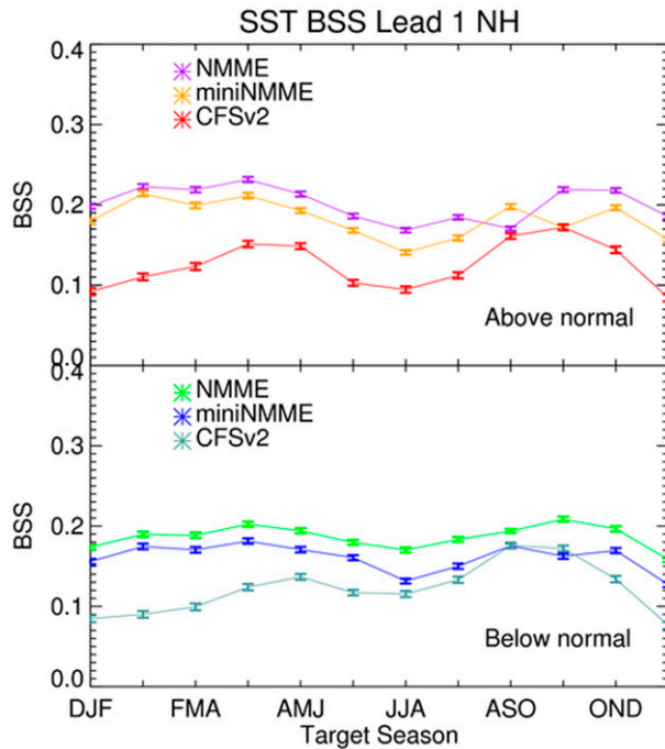
FIG. 3. As in Fig. 1, but for SST in the Northern Hemisphere (NH; all ocean grid points 23^{\circ} – 75^{\circ} N).
