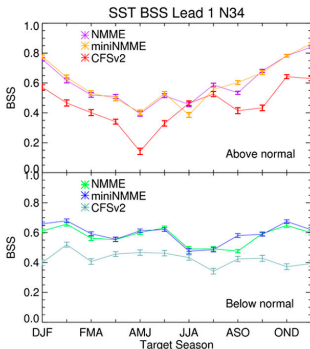
FIG. 1. Brier skill score (BSS) area-aggregated for all lead-1 seasonal probabilistic forecasts of SST in the Niño-3.4 region ( 5^{\circ}\text{S} – 5^{\circ}\text{N} , 190^{\circ} – 240^{\circ}\text{E} ). Forecasts for the (top) above-normal and (bottom) below-normal terciles are shown for three forecasting systems: all members of the 6-model NMME (75 members), a mini-NMME comprising 4 members from each of the 6 models (24 members), and the CFSv2 alone (24 members). The lead-1 forecast for December–February (DJF) is made using November initial conditions, etc. Bars show the 95% confidence interval from 1000 bootstrap samples.
