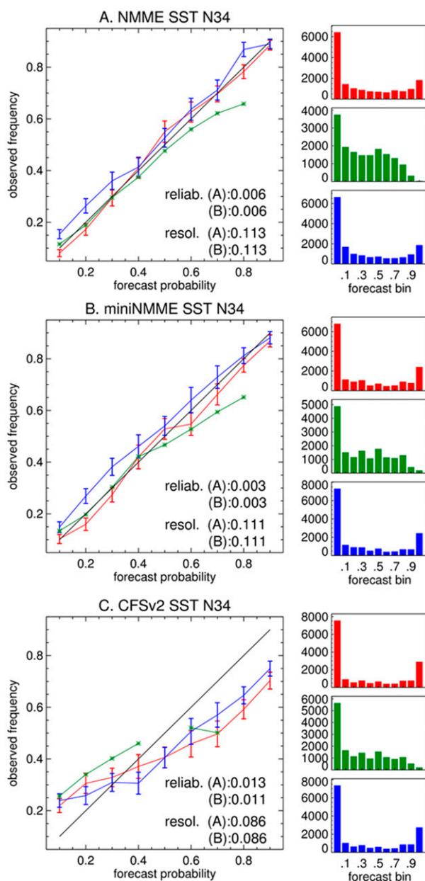
FIG. 2. Reliability diagrams for probabilistic forecasts of sea surface temperature (SST) in the Niño-3.4 region ( 5^{\circ}\text{S} – 5^{\circ}\text{N} , 190^{\circ} – 240^{\circ}\text{E} ) for the (a) NMME, (b) mini-NMME, and (c) CFSv2, aggregated for the lead-1 season from all initial conditions. Red lines indicate forecasts in the above tercile, blue the below, and green the near-normal. Lines closer to the black diagonal mean the forecast event frequency (y axis) is close to the forecast probability (x axis), and therefore the forecasts are more reliable. Histograms indicate how often each forecast bin is used; numbers on the y axis has been divided by 1000. All diagrams use 10 bins of size 0.1. Alphanumeric insets show the reliability and resolution terms of the Brier score for the above (A) and below (B) terciles. As Brier score = reliability – resolution + uncertainty, higher-resolution values and lower reliability values are desirable. Bars indicate the 95% confidence intervals derived from 1000 bootstrapping tests.
