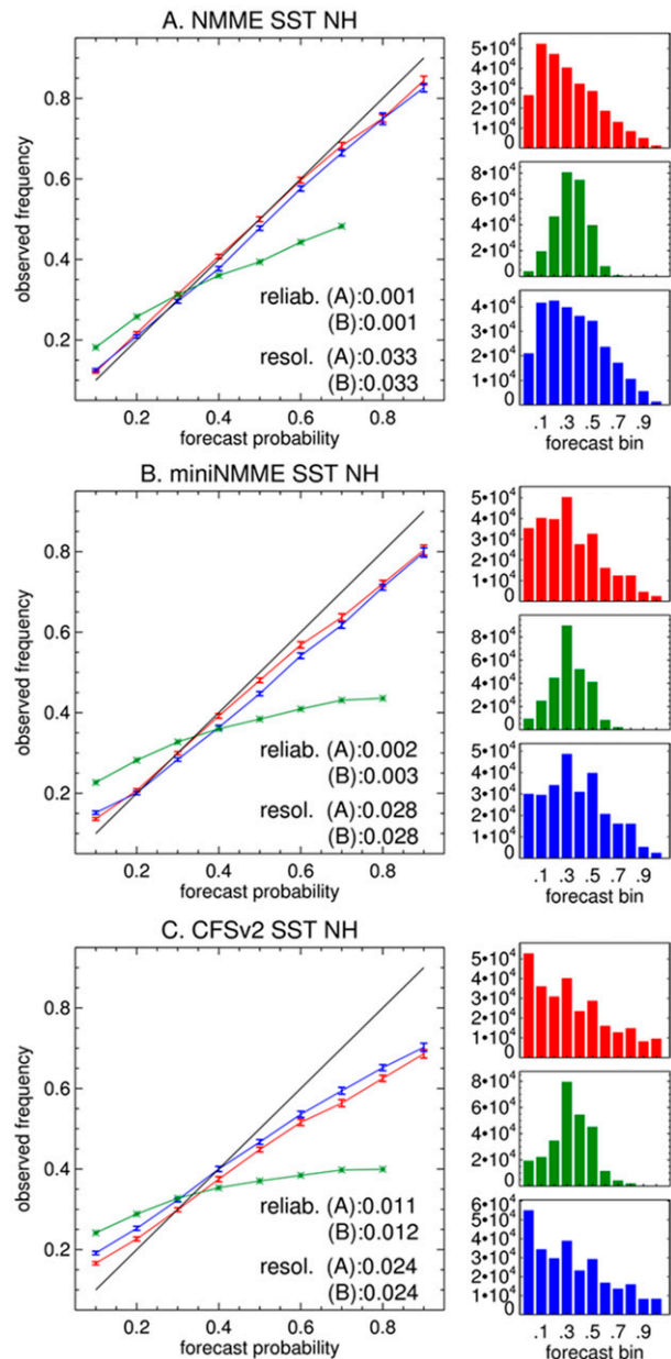
FIG. 4. As in Fig. 2, for SST in the NH ( 23^{\circ} – 75^{\circ} N).
