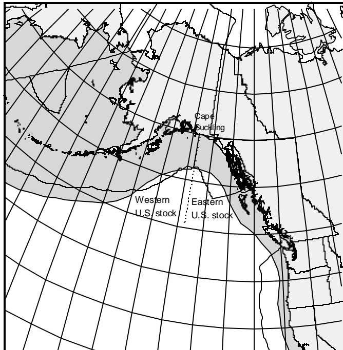
Figure 3. Approximate distribution of Steller sea lions in the eastern North Pacific (shaded area).
