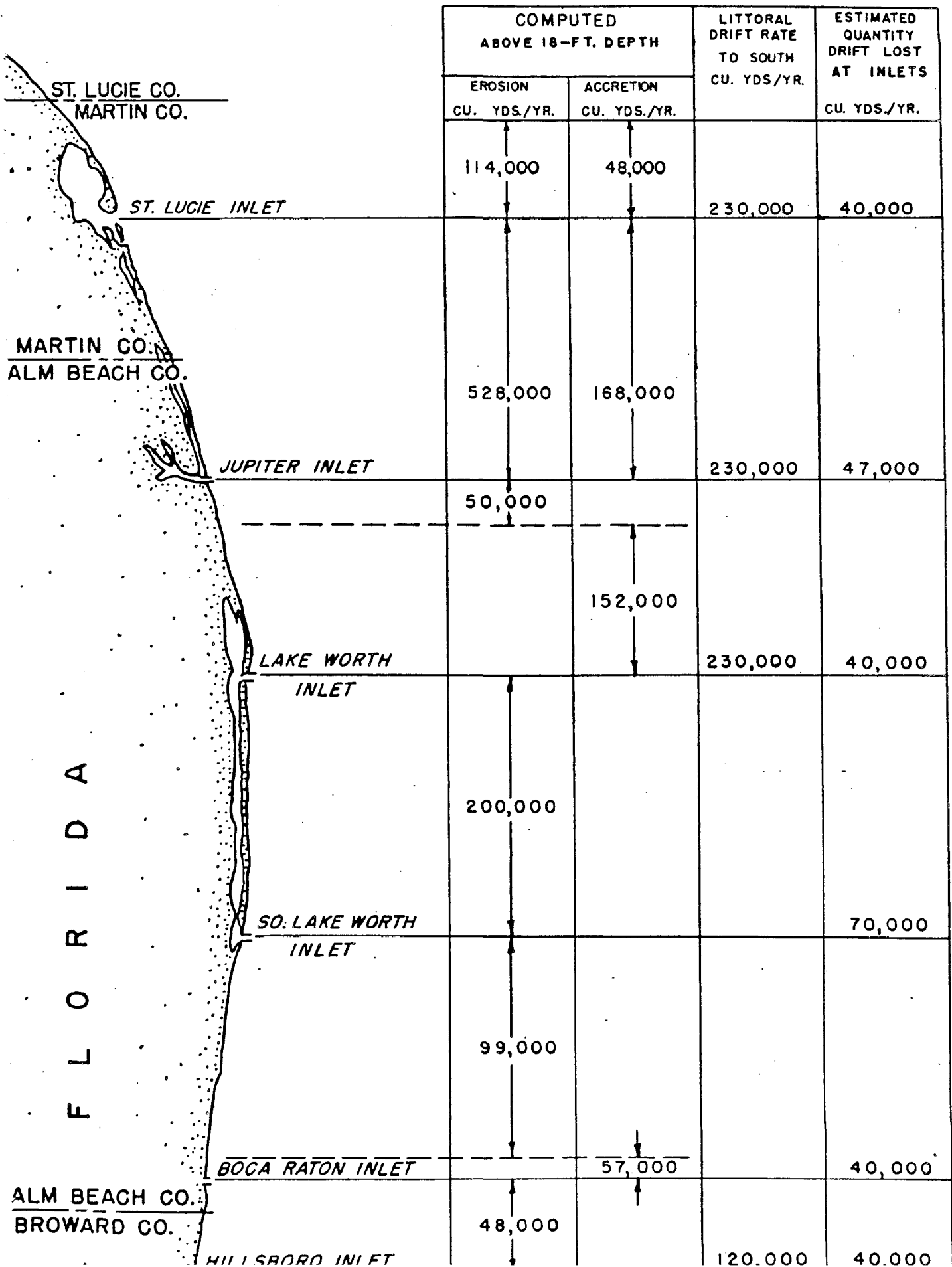
Figure 7. LITTORAL DRIFT RATES (Corp of Engineers, 1968)
