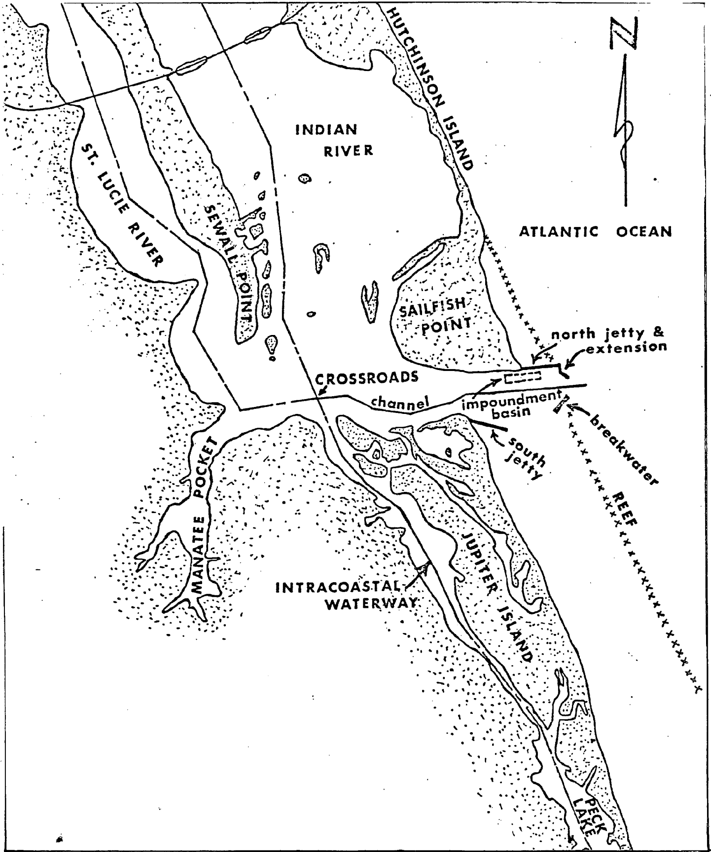
Figure 9. ST. LUCIE INLET IMPROVEMENT PROJECT
