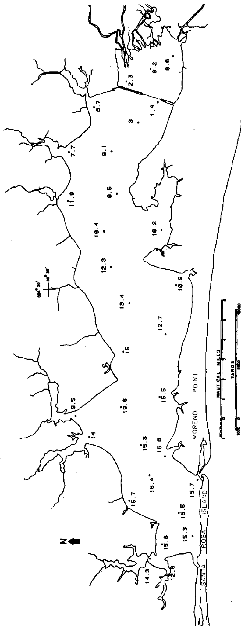
Figure : Salinity (ppt) in surface waters of Choctawhatchee Bay on September 25-26, 1975.
