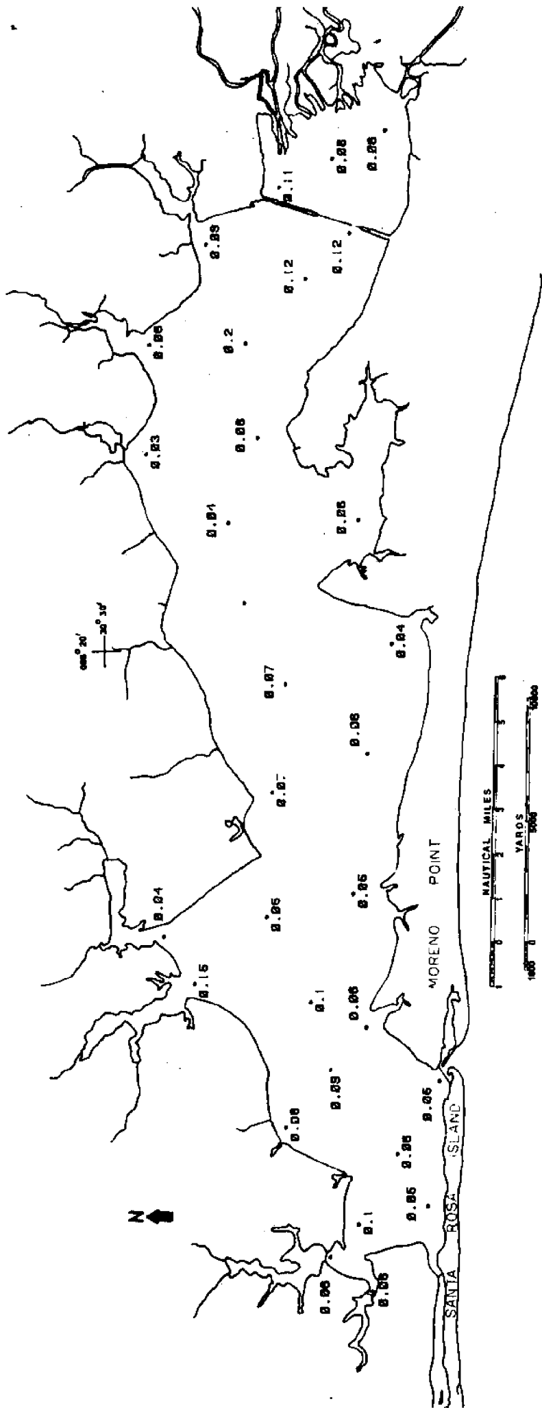
Figure : Ammonia concentration (mg/l-N) in mid-depth waters of Choctawhatchee Bay on December 15, 1975.
