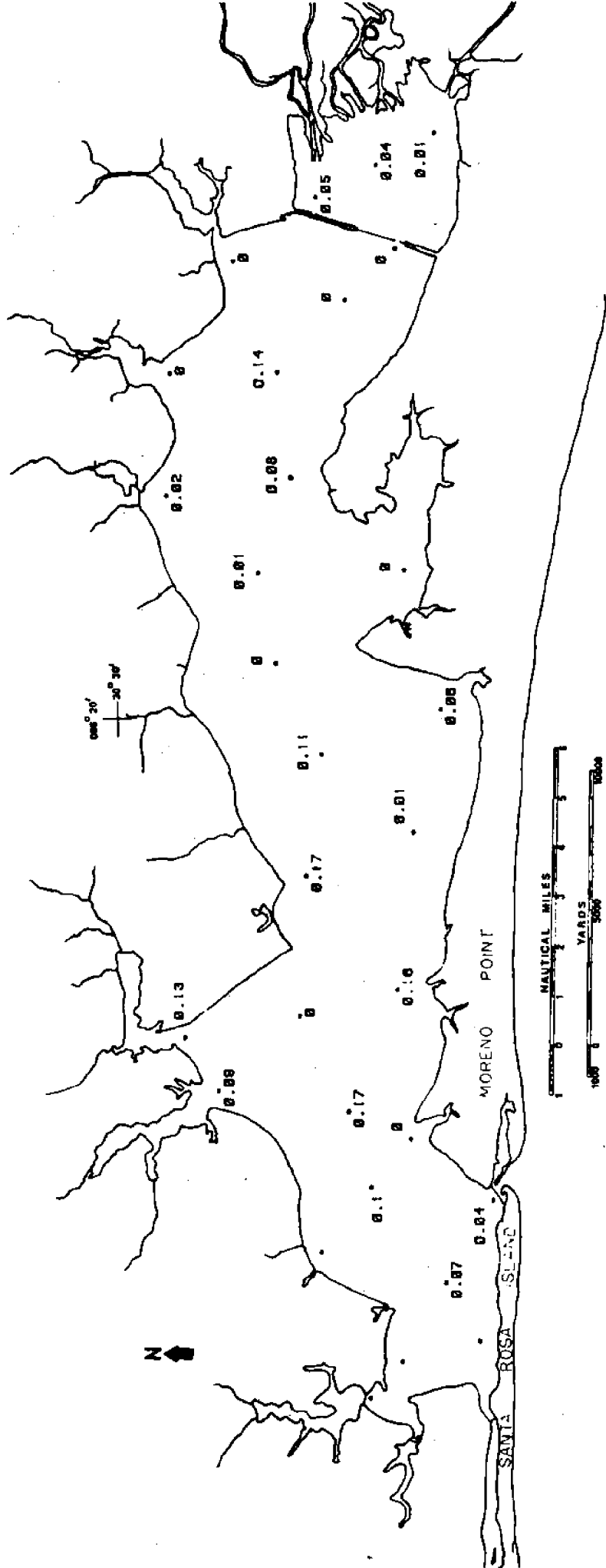
Figure : Ammonia concentration (mg/l-N) in mid-depth waters of Choctawhatchee Bay on May 20-21, 1975.
