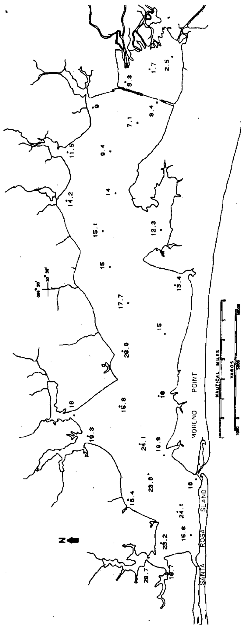
Figure : Salinity (ppt) in bottom waters of Choctawhatchee Bay on September 25-26, 1975.
