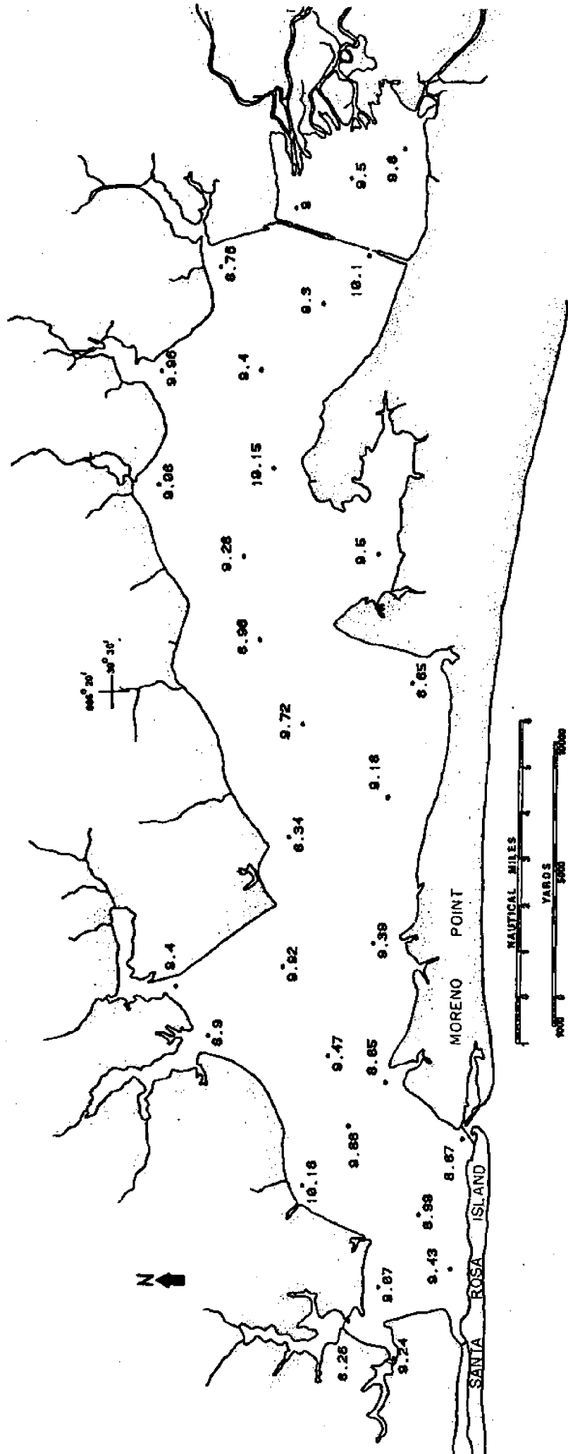
Figure : Dissolved oxygen concentration (mg/l) in surface waters of Choctawhatchee Bay on April 21-22, 1975.
