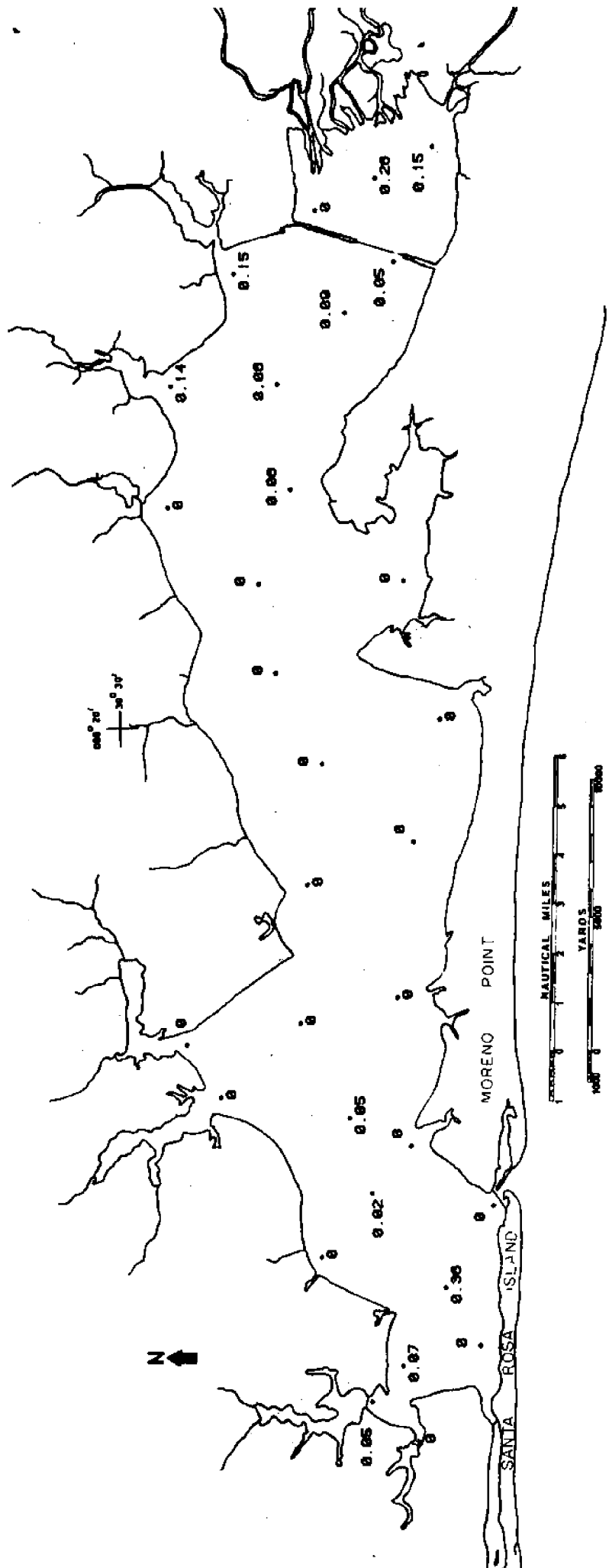
Figure : Ammonia concentration (mg/l-N) in bottom waters of Choctawhatchee Bay on June 21-22, 1975.
