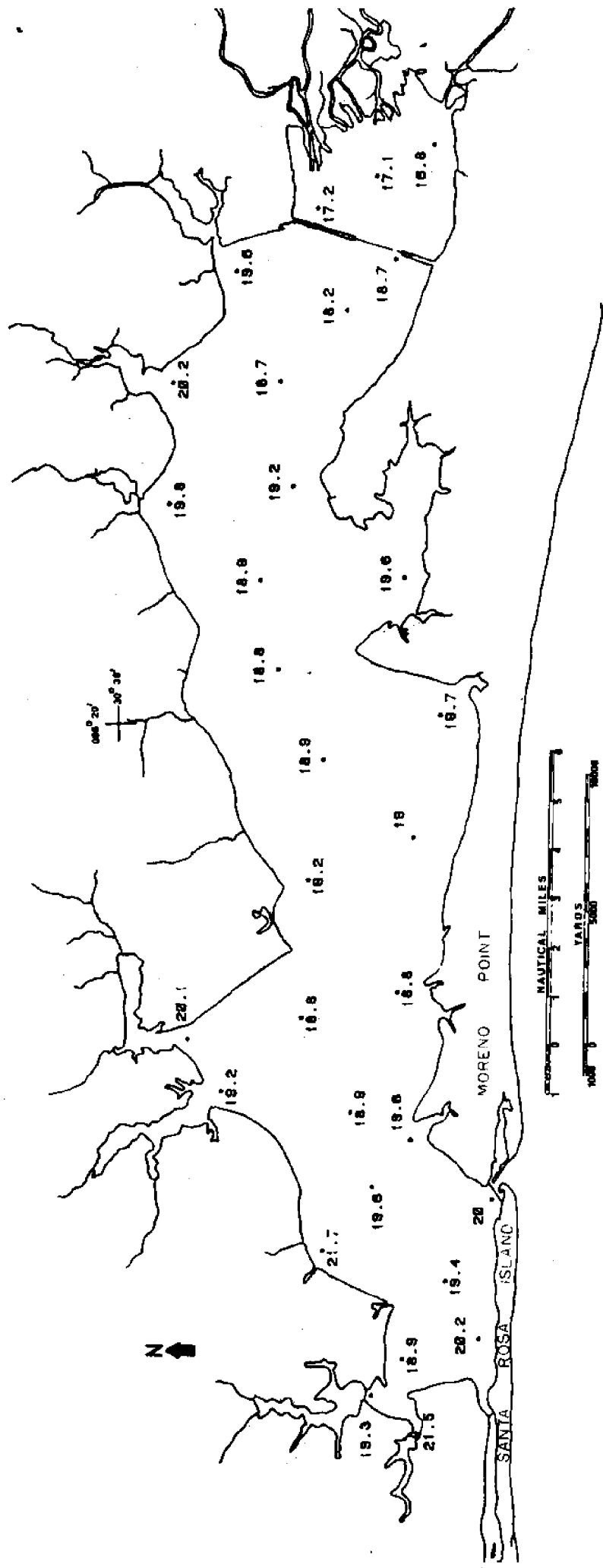
Figure : Water temperature (Celsius) in bottom waters of Choctawhatchee Bay on April 21-22, 1975.
