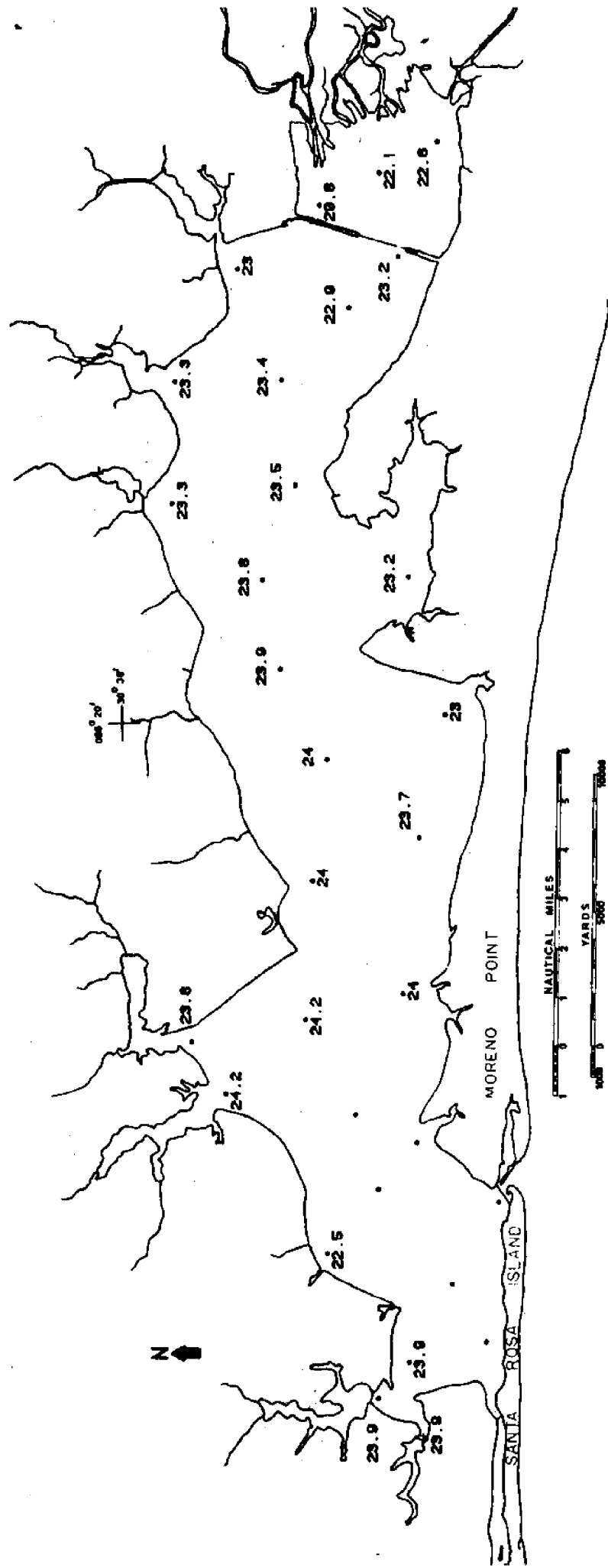
Figure : Water temperature (Celsius) in bottom waters of Choctawhatchee Bay on October 29-30, 1975.
