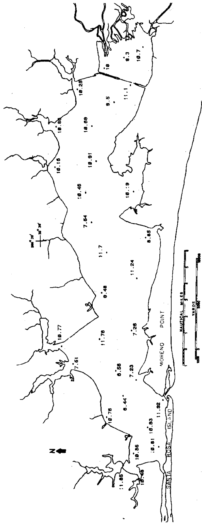
Figure : Dissolved oxygen concentration (mg/l) in mid-depth waters of Choctawhatchee Bay on April 21-22, 1975.
