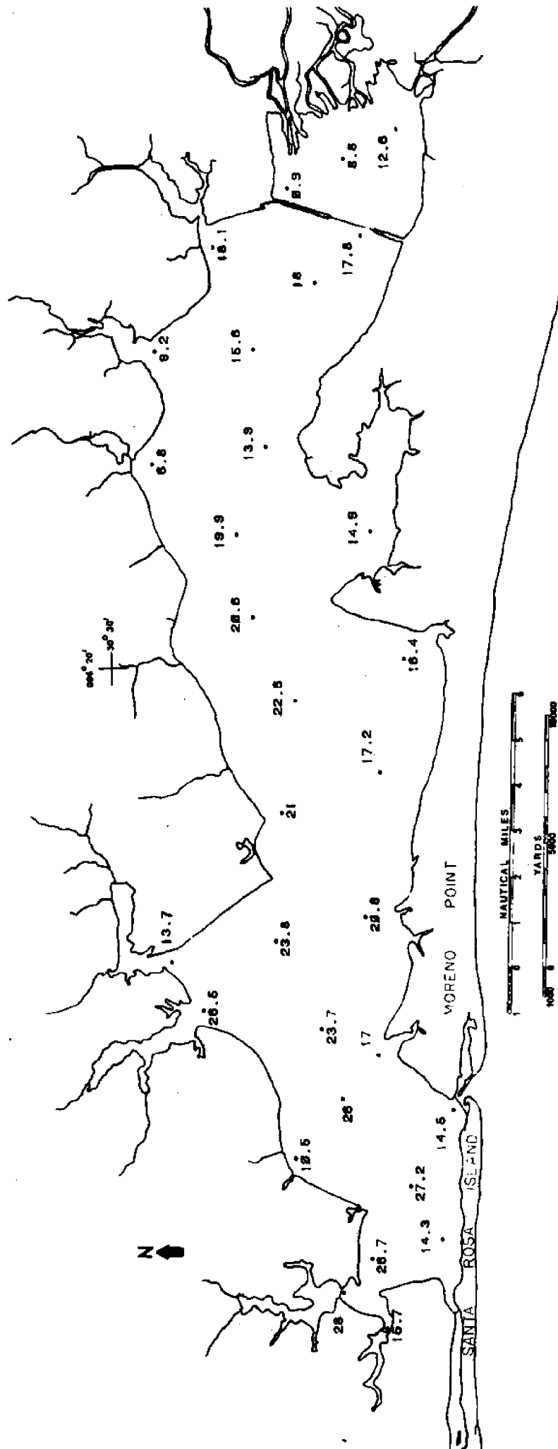
Figure : Salinity (ppt) in mid-depth waters of Choctawhatchee Bay on January 28-29, 1975.
