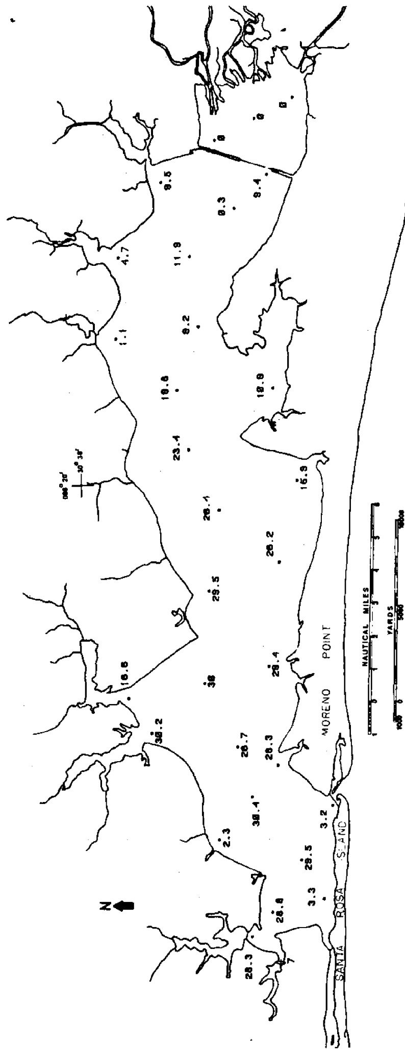
Figure : Salinity (ppt) in bottom waters of Choctawhatchee Bay on April 21-22, 1975.
