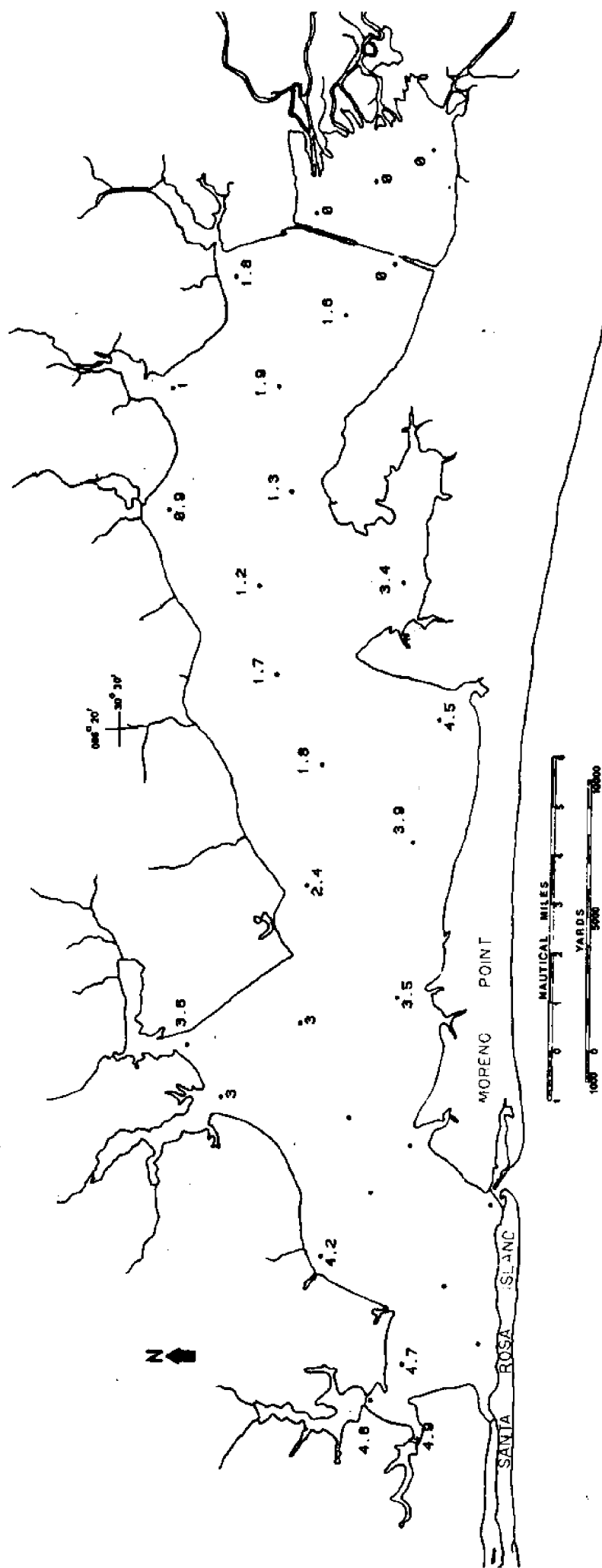
Figure : Salinity (ppt) in surface waters of Choctawhatchee Bay on October 29-30, 1975.
