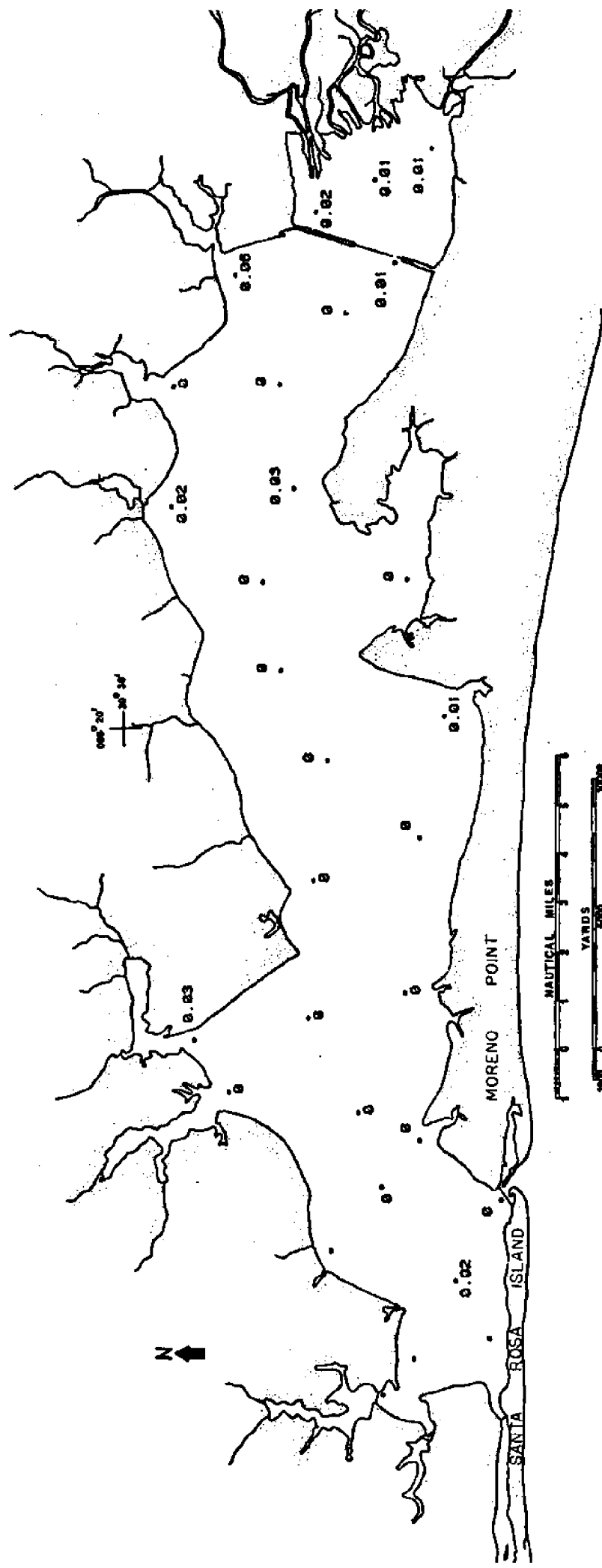
Figure : Ammonia concentration (mg/l-N) in surface waters of Choctawhatchee Bay on May 20-21, 1975.
