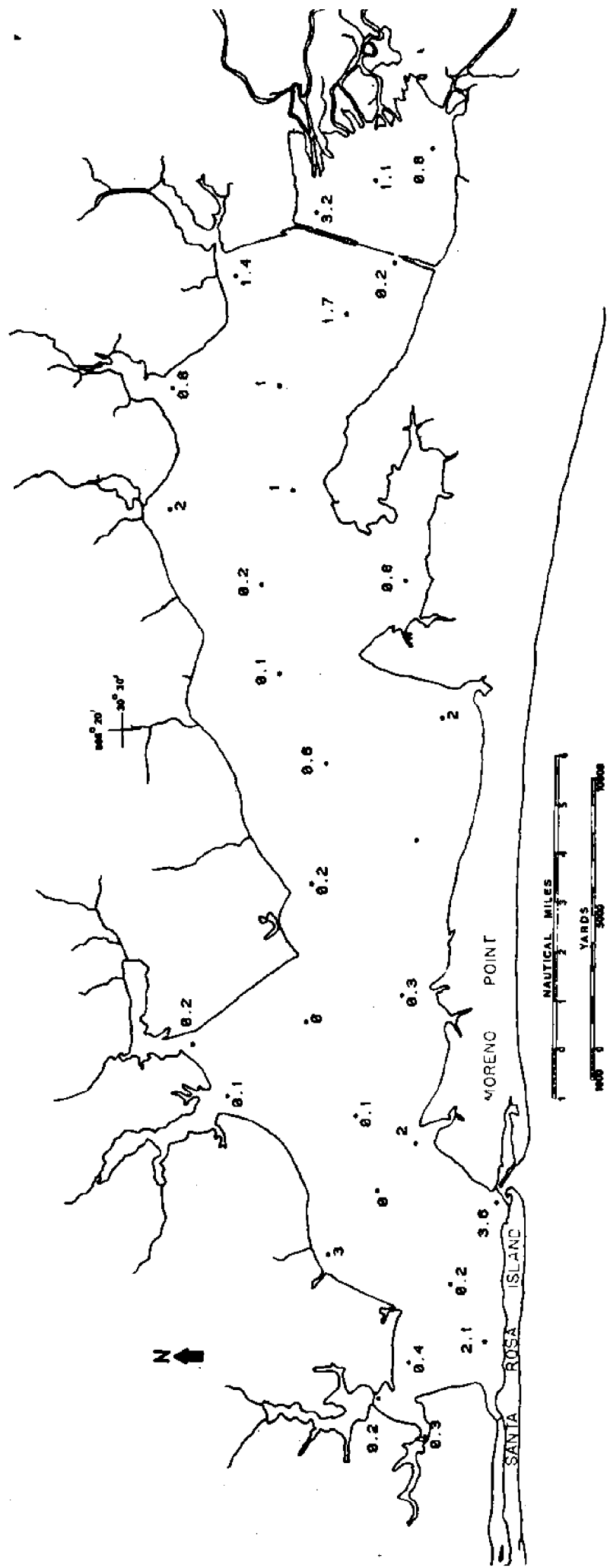
Figure : Dissolved oxygen concentration (mg/l) in bottom waters of Choctawhatchee Bay on July 19 & 23, 1975.
