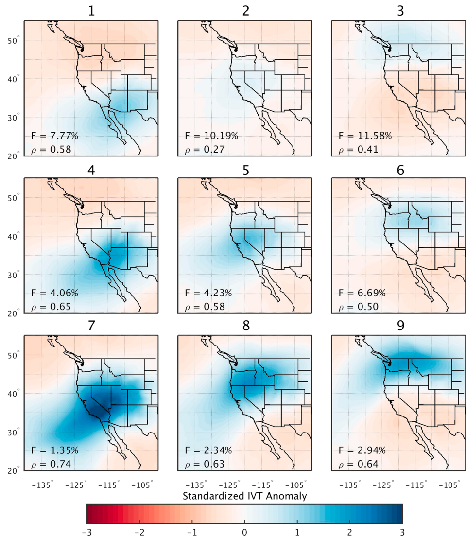
Figure 2. A 3 \times 3 SOM composite of standardized integrated vapor transport anomaly, |IVT|' .
