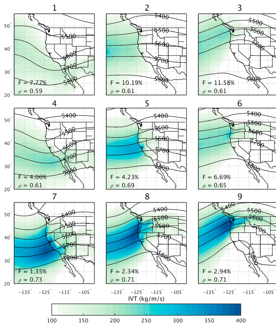
Figure 3. A 3 \times 3 SOM composite of integrated vapor transport, IVT. Overlaid on the IVT contours are contours of the 500 hPa geopotential height (m).
