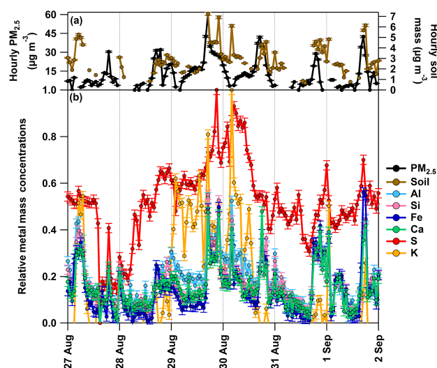
Figure 12. (a) Time series of hourly \text{PM}_{2.5} and soil mass concentrations as measured by PX-375 between 27 August and 2 September 2015 and (b) hourly mass concentrations of select individual metals relative to their maximum concentration observed during the study time period, including an error of \pm 2\% . Only data higher than the LDLs are shown. PX-375 data overlapped with event 3.
