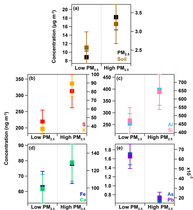
Figure 13. Averages of (a) \text{PM}_{2.5} and soil concentrations and (b–e) select metal mass concentrations during non-event days (i.e., cleaner conditions) compared to averages from haze event days (i.e., influence from fires haze) for 26 August–2 September 2015. “Low” and “high” correspond to the \text{PM}_{2.5} concentration values. Error bars represent the 90 % confidence intervals. Concentration averages were statistically significant based on t tests of two samples of unequal variances.
