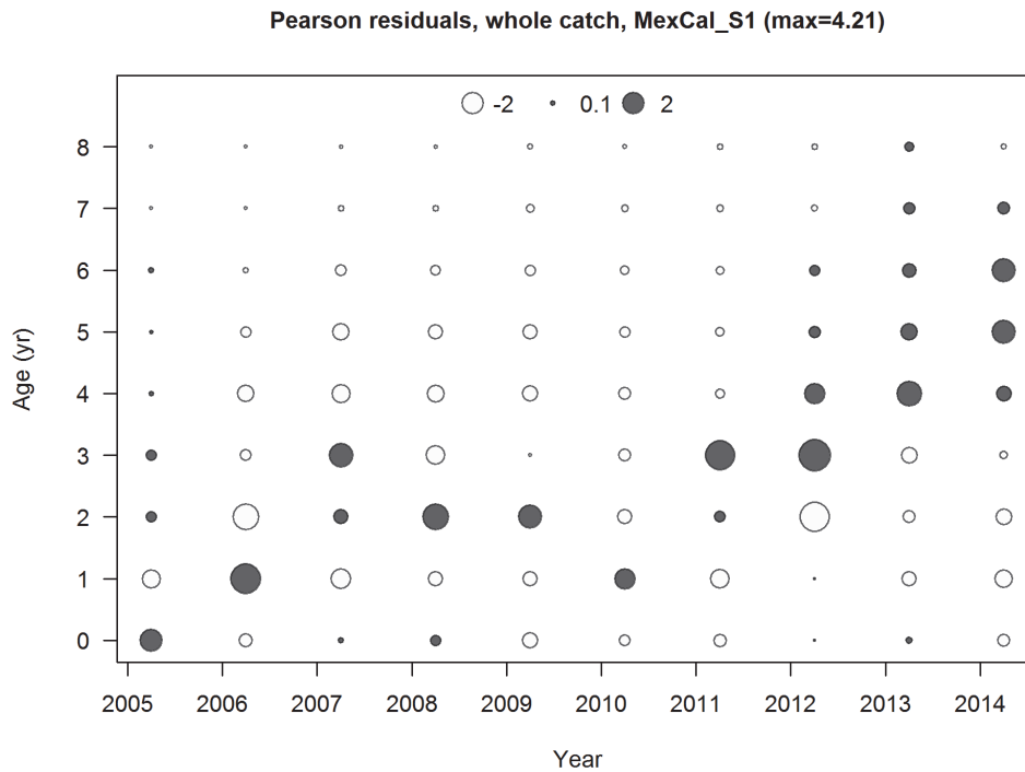
Figure 23. . Fit to age-composition time series and residual plot for the MEXCAL_S1 fleet in model ALT. N represents input sample sizes and effN is the effective sample size given overall statistical fit in the model.
