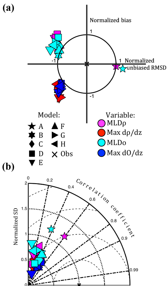
Figure 6. Normalized summary (a) target and (b) Taylor diagram illustrating model skill of MLD_{\rho} and MLD_{O_2} , \max d\rho/dz , and \max dO_2/dz at 13 Chesapeake Bay stations for 2004–2005. The “x” represents the skill of a model that perfectly reproduces the observations. Since RMSD of stratification is only computed at stations where both the observations and model exhibit stratification, the Model Mean is not calculable for these variables.
