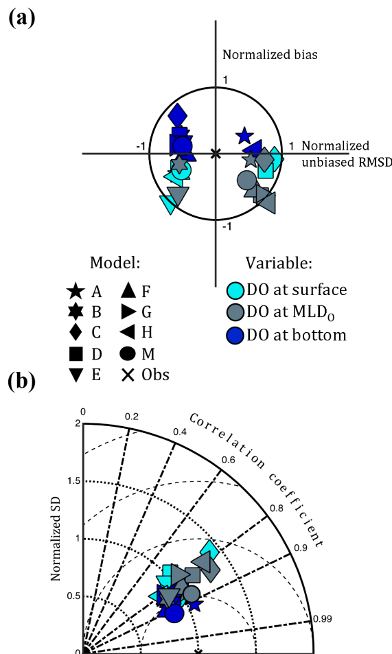
Figure 4. Normalized summary (a) target and (b) Taylor diagrams illustrating model skill of dissolved oxygen at the surface, MLD_O , and bottom for 13 Chesapeake Bay stations in 2004–2005. The “x” represents the skill of a model that perfectly reproduces the observations. The dotted, dashed-dot, and dashed lines on the Taylor diagram represent lines of constant standard deviation, correlation coefficient, and unbiased RMSD, respectively.
