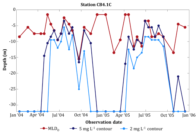
Figure 12. Time series of observations of dissolved oxygen and MLD_0 contours at Station CB4.1C for 2004 and 2005.
