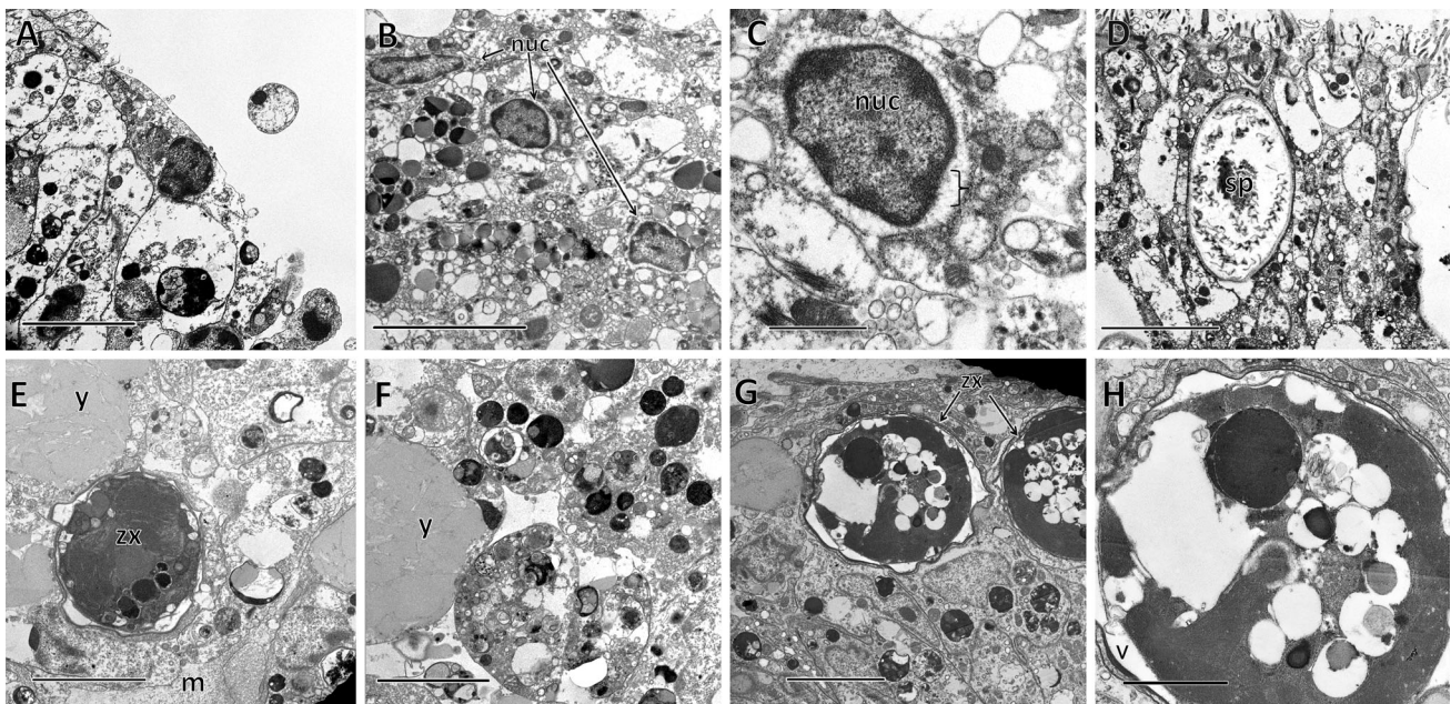
Fig. 4 Transmission electron microscopy of Stylophora pistillata planula exposed to 228 parts per billion ( \mu\text{g/L} ) benzophenone-3 for 8 h in the light. a Surface of the epidermal layer; indicating a lack of cilia and cells dying either via necrosis or autophagic cell death; bar indicates 5000 nm. b Epidermal tissue where cells exhibit an abundance of vacuolated bodies, especially the presence of vacuolated nuclei ( nuc ); bar indicates 5000 nm. c Magnification of vacuolated nuclei ( nuc ) that completely lacks nuclear blebbing (a sign of apoptosis). “}” indicates vacuolization of delaminated nuclear double membrane; bar indicates 1000 nm. d Epidermal layer with
