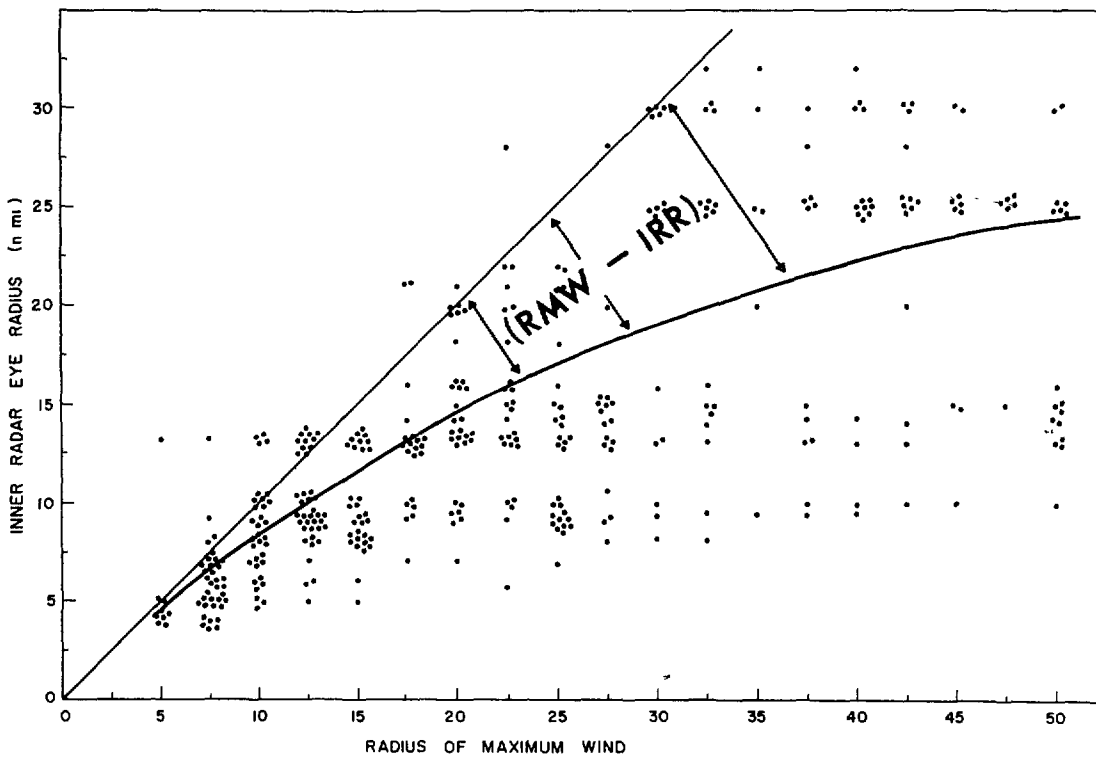
Figure 15.--Radius of maximum winds (RMW) vs. inner radar eye radius (IRR). Points falling on the 45° line are those where the RMW and IRR coincide. The curved line indicates the best fit curve (from Shea 1972).
