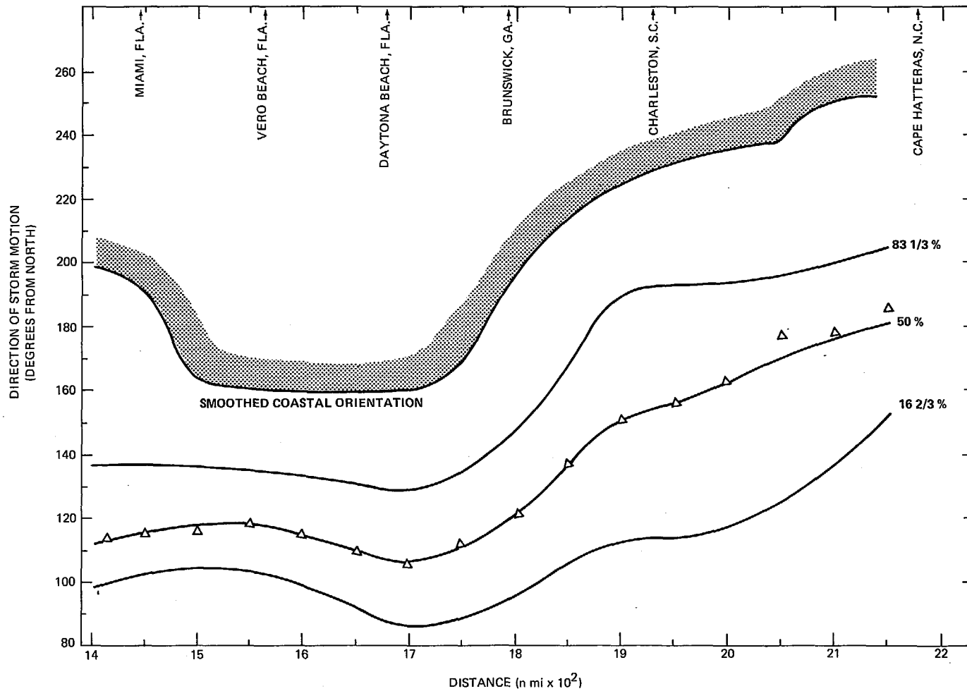
Figure 28a.--Probability distribution of direction of landfalling storm motion for east coast, south of Cape Hatteras, N.C. Notations are the same as figure 27.
