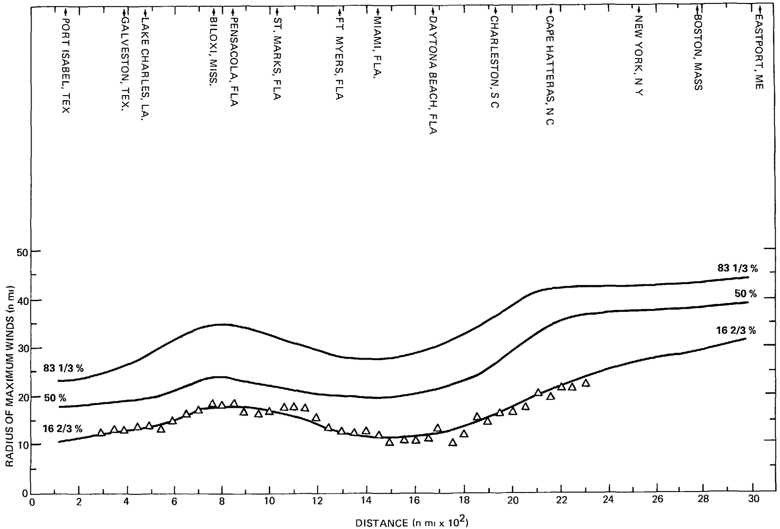
Figure 19.--Probability distribution of radius of maximum winds of hurricanes, gulf and east coasts (1900-73). Numbered lines denote the percent of storms with R equal to or less than the value indicated along the ordinate. Plotted points (▲) are taken from frequency analyses at 50-n.mi. intervals for the 16-2/3 percentile (sec. 4.2).
