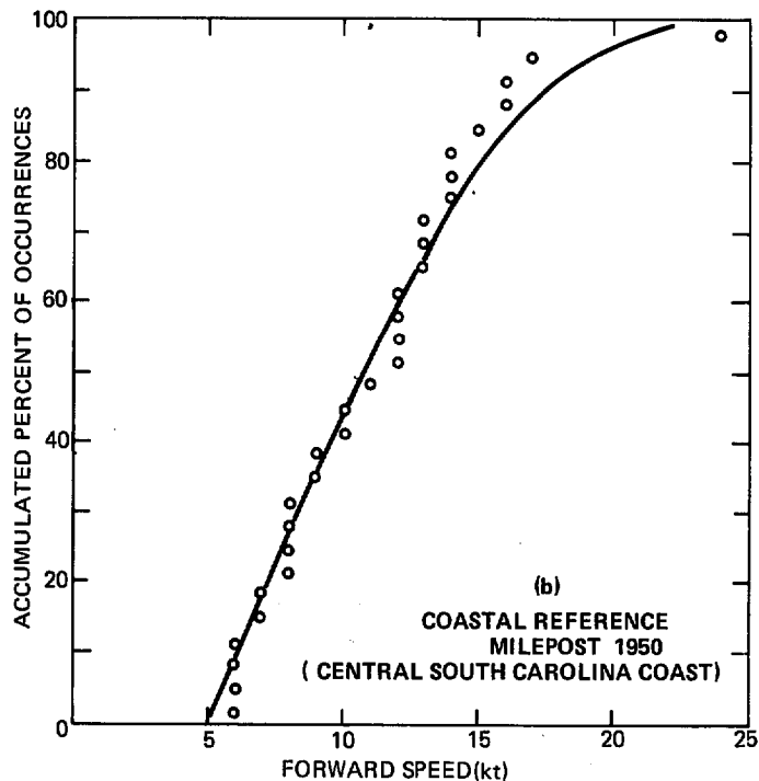
Figure 22.--Landfalling hurricanes, forward speed vs. cumulative percent of occurrences, (a) Gulf of Mexico (milepost 750) near Bay St. Louis, Miss., (b) east coast (milepost 1950) along central South Carolina coast.
