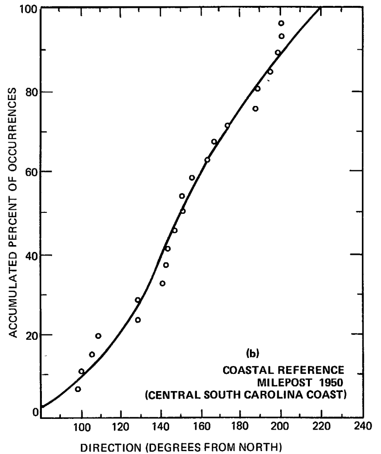
Figure 26.--Landfalling hurricanes and tropical storms, direction of motion vs. cumulative percent of occurrences, (a) Gulf of Mexico (milepost 750) near Bay St. Louis, Miss., (b) east coast (milepost 1950) along central South Carolina coast.
