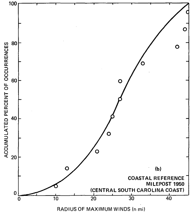
Figure 18.--Graphs of radius of maximum winds vs. cumulative percent of occurrences (a) Gulf of Mexico (milepost 750), near Bay St. Louis, Miss., where hurricane Camille went ashore and (b) east coast (milepost 1950), along central South Carolina coast.
