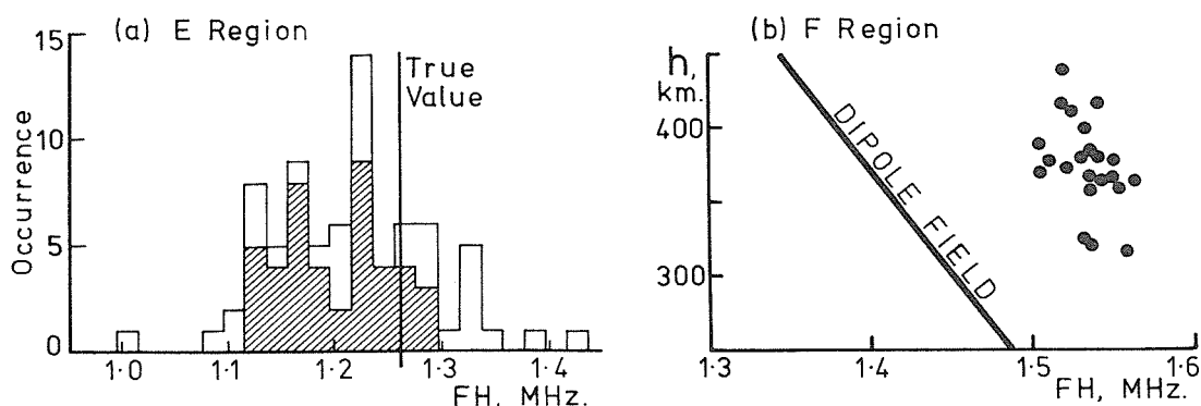
Figure C1. Values of gyrofrequency FH calculated from measurements on corresponding O and X ray cusps. Results (a) are for the E region, at a dip angle of 67^\circ (the shaded area applies to the more accurate measurements); (b) are from F region measurements at Brisbane (Ellis, 1957).
