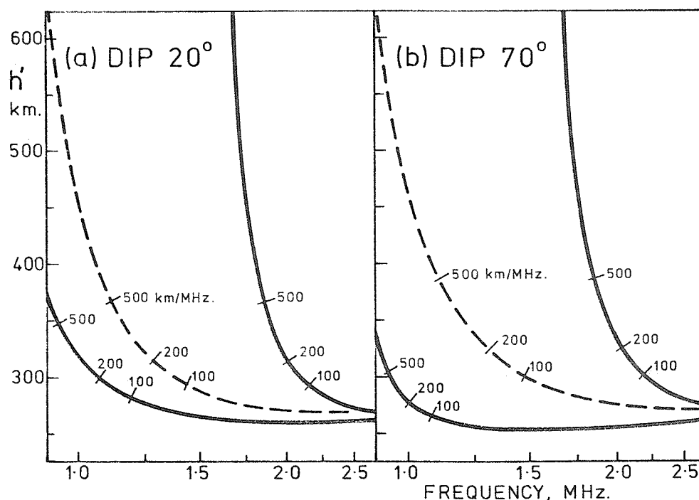
Figure 14. Virtual heights for the ordinary and extraordinary rays, calculated using the model profile 3B, at dip angles of 20° and 70°.
