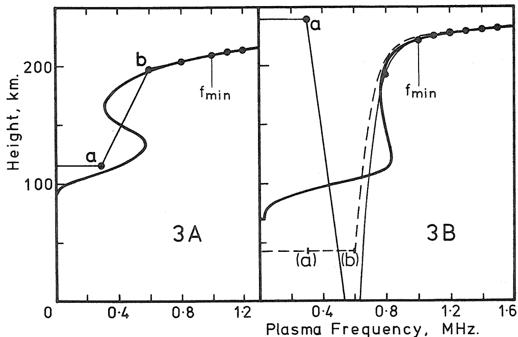
Figure C6. Starting calculations using a fixed gyrofrequency f_{FH} = 1.2 MHz, at a dip angle of 70^\circ . Heavy lines give the original model profiles, while solid dots are the result of starting calculations with f_{min} = 1.0 MHz. The broken line for model 3B is the solution obtained if the thickness of the underlying slab a,b is constrained to be zero instead of negative.
