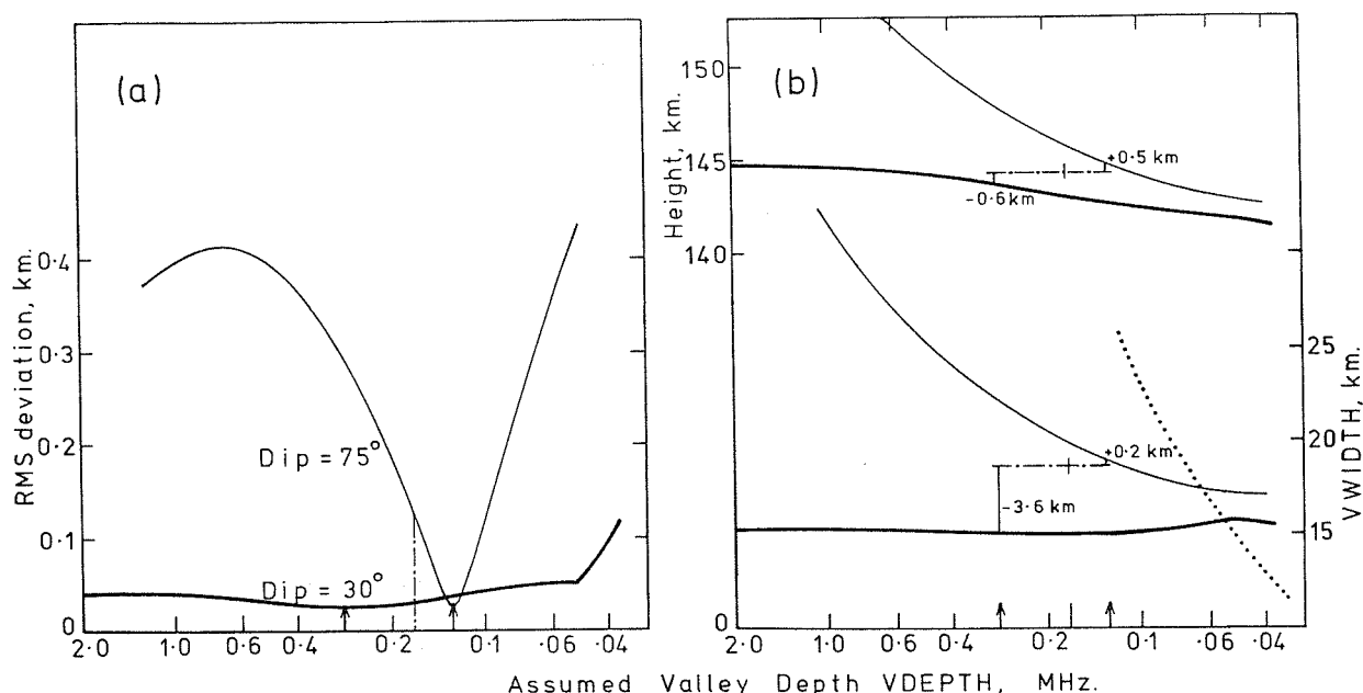
Figure 22. Analysis of virtual-height data corresponding to the profile V5, at two values of dip angle, using different assumed values for the valley depth. Ordinary and extraordinary ray data were used at six frequencies, corresponding to plasma frequencies at reflection from foE + 0.05 MHz to foE + 0.3 MHz in steps of 0.05 MHz. Chain lines show the true values of VDEPTH , VWIDTH and real height (at foE + 0.3 MHz). Arrows mark the values corresponding to a minimum in the RMS virtual-height fitting error.
