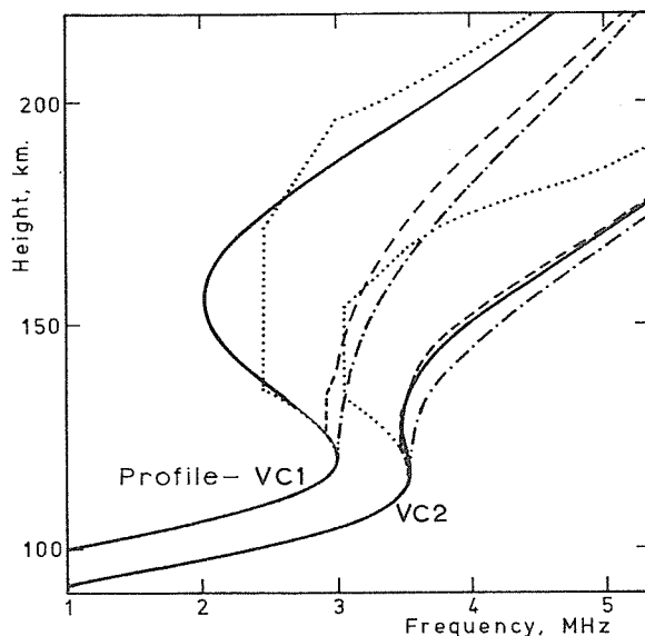
Figure 8. Dual-Chapman profiles for conditions near sunrise or sunset (VC1), and near noon (VC2). Broken lines give the profile calculated by POLAN at a dip angle of 50^\circ , using the standard valley ( HVAL=0 or 1 ). Upper and lower limit calculations (obtained with HVAL=5 or 10 respectively) are shown by dotted and chain lines.
