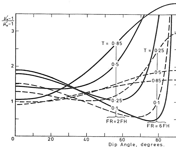
Figure B2. The group delay ratio R_{X,O} = (\mu'_x - 1)/(\mu'_o - 1) as a function of dip angle, for plasma frequencies at reflection (FR) of twice and six times the gyrofrequency. The curves at T = 0.85, 0.5, 0.25 and 0.1 correspond to FN/FR = 0.53, 0.87, 0.97 and 0.997 respectively.
