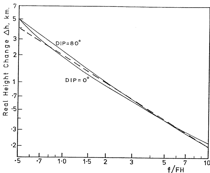
Figure A2. Changes in real height, beginning at a frequency f of half the gyrofrequency FH, that produce no change in the virtual height of the ordinary ray. Results are shown for dip angles of 0^\circ and 80^\circ , assuming a change of 5 km in the real height at plasma frequencies of 0 to 0.5FH .
