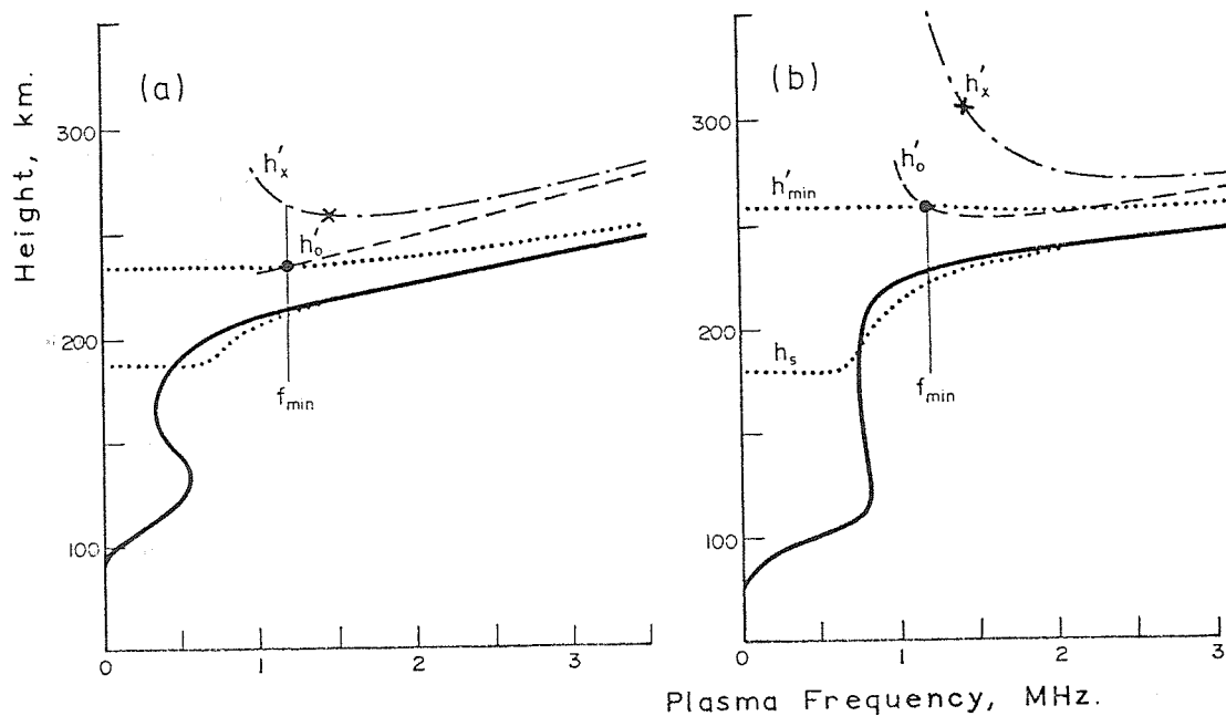
Figure 16. Analysis of the two basic types of start profile, at a dip angle of 70^\circ . Upper dotted lines show the result of a direct O-ray analysis from f_{\min} = FH = 1.2 MHz. The lower dotted lines are obtained using the single-point procedure in SPOLAN, with a starting frequency f_s of 0.6 MHz.
