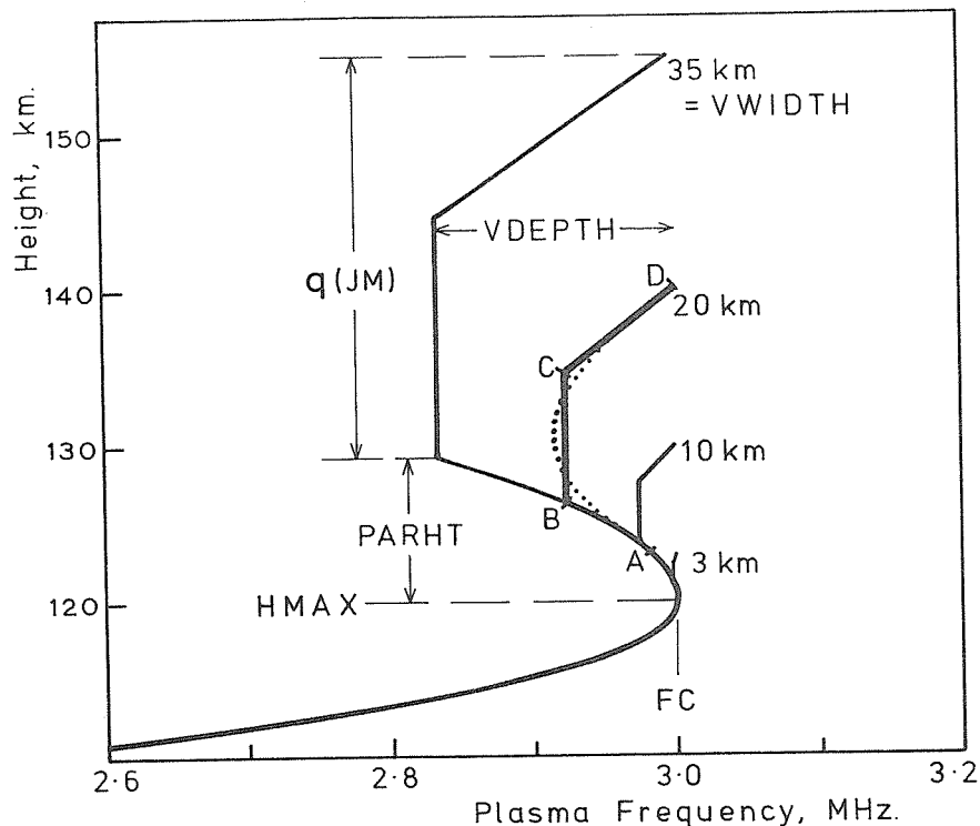
Figure 17. The shape of the standard valley, for different values of the single parameter VWIDTH . The dotted line shows a possible form for the true variation of plasma frequency with height in an E-F valley; this will give (very closely) the same virtual heights as the solid line model. A to D show the four points which are added to the calculated real height data, to define the valley region.
