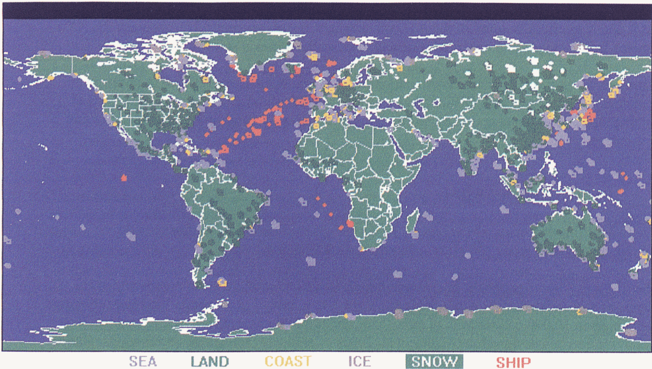
Figure 1: The global distribution of clear and cloudy collocations stored on the First Guess Libraries from NOAA-15 observed on September 6, 2000.
