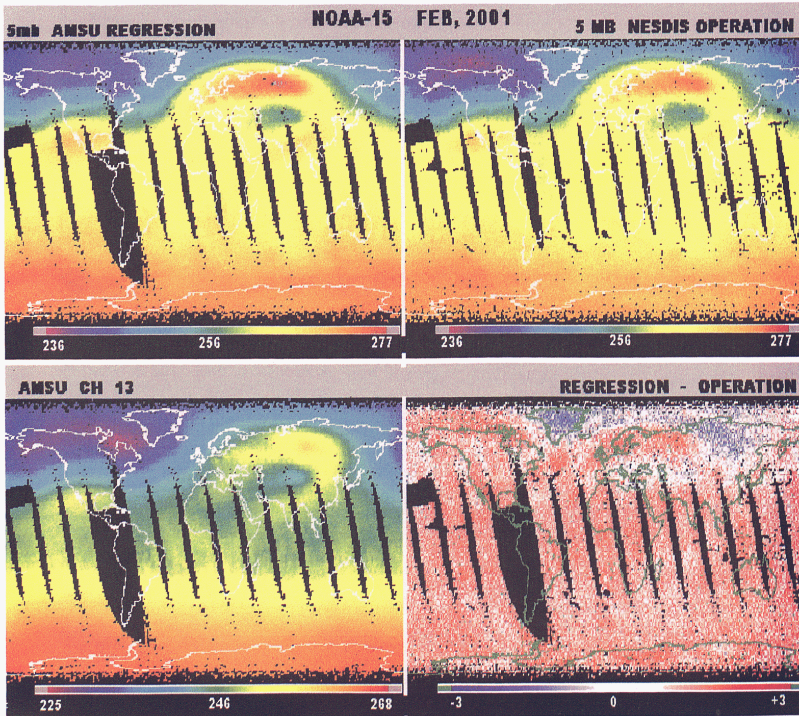
Figure 3: Temperature at 5mb derived from AMSU-only Regression (upper left), the NESDIS Operation (upper right), the corresponding AMSU channel 13 radiance temperature measurements sensitive at the 5 mb level (lower left), and the Regression minus Operation differences at 5 mb (lower right), during February, 2001.
