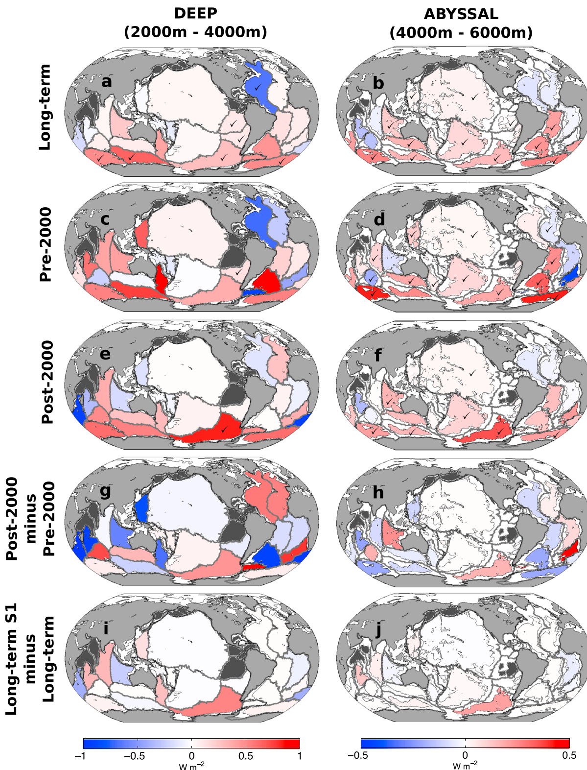
Figure 3. Spatial distributions of local heat content trend Q (in \text{W m}^{-2} ) within (a, c, e, g, and i) the deep 2000–4000 m layer and (b, d, f, h, and j) the abyssal 4000–6000 m layer from the long-term estimate (Figures 3a and 3b), the pre-2000 estimate (Figures 3c and 3d), the post-2000 estimate (Figures 3e and 3f), the difference between post-2000 and pre-2000 estimates (Figures 3g and 3h), and the difference between the long-term S1 and the long-term estimates (Figures 3i and 3j). Basins colored in black have not been sampled by repeat hydrography during the relevant time span. Tick symbols in Figures 3a–3f highlight the OHC trends statistically different from zero at 95% confidence. Color scale for the deep layer is twice that for the abyssal layer.
