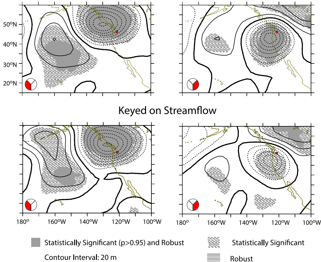
FIG. 10. (top) The 500-hPa geopotential height anomalies (m; negative values shown with a dashed line) associated with the three regional circulation categories (see text for definitions) keying on rainfall events (daily totals > 0.25 in.) in the Klickitat River watershed. The sectors for the anomalous 500-hPa flow associated with each category are indicated by pie charts in the lower-left corner of each panel. Anomalies are shaded where statistically significant (based on a two-tailed Student's t test) and "robust," meaning in this case that at least 80% of the composited events have anomalies of the same sign. The composites shown are based on 74, 44, and 9 events for the southwesterly, southeasterly, and northerly (not shown) types, respectively. (bottom) As in the top panels, but keyed on streamflow events (daily increase > 1.2 normalized standard deviations) on the Klickitat River, and based on 57, 37, and 9 July–September events for type southwesterly, southeasterly, and northerly (not shown) atmospheric circulation patterns, respectively.
