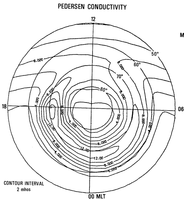
Fig. 4d Assumed height-integrated Pedersen and Hall conductivities.
