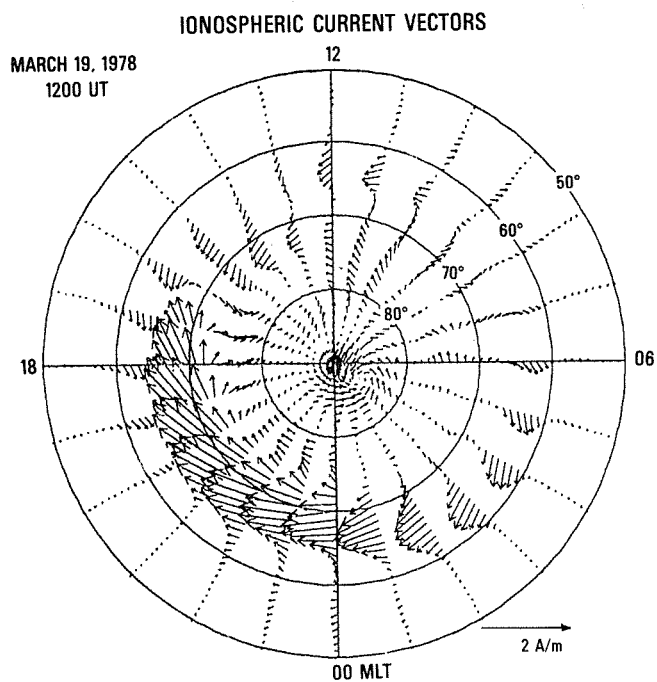
Fig. 4g Ionospheric current vectors.
