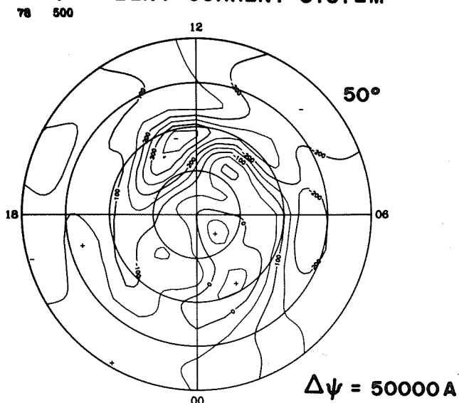
EQUIVALENT CURRENT SYSTEM
