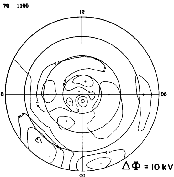
ELECTRIC POTENTIAL
