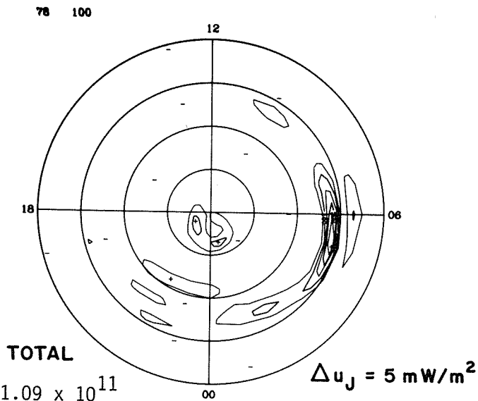
JOULE HEATING
