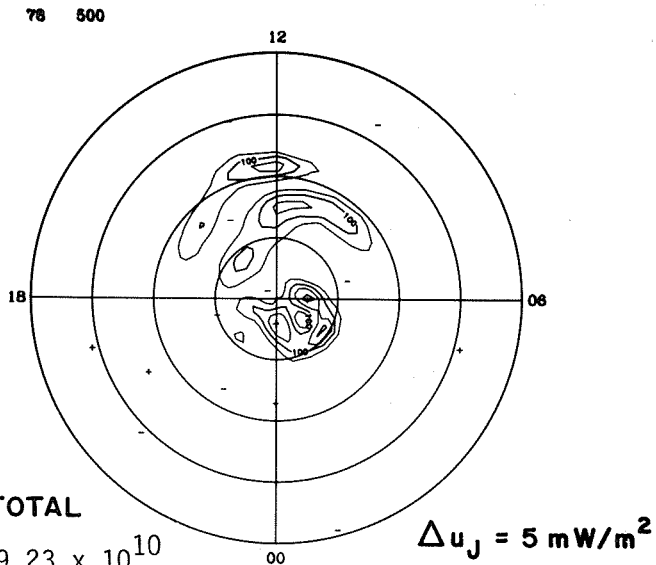
JOULE HEATING
