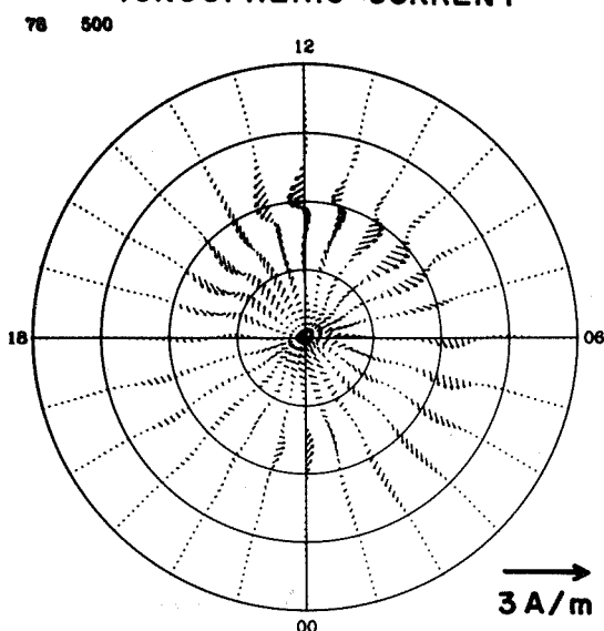
IONOSPHERIC CURRENT
