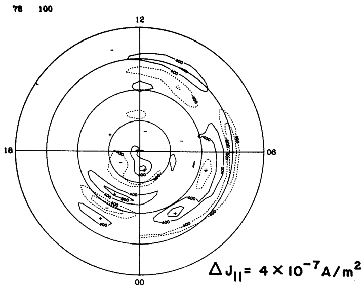
FIELD-ALIGNED CURRENT
