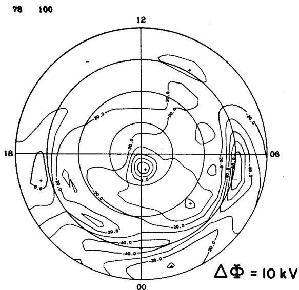
ELECTRIC POTENTIAL
