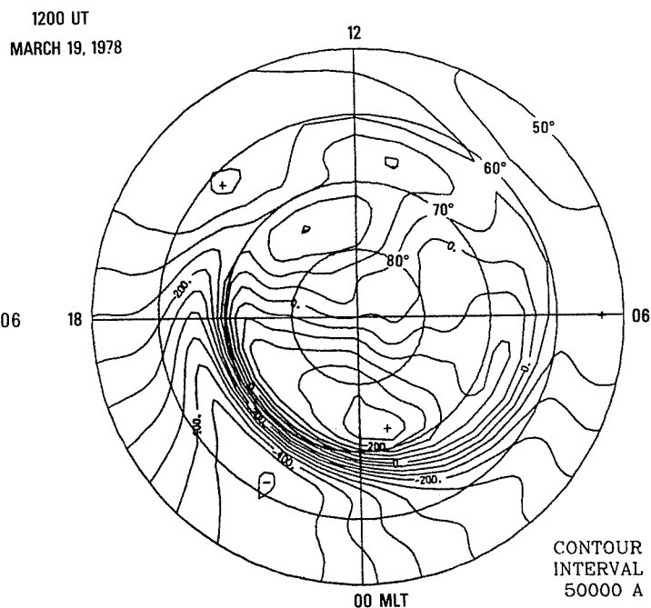
Fig. 4b Calculated equivalent current functions.
