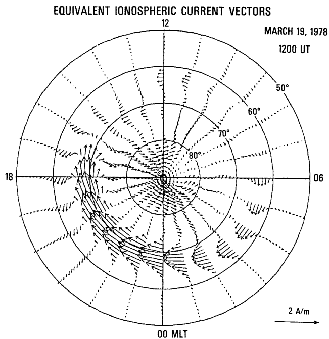
Fig. 4c Equivalent current vectors calculated at the grid points.
