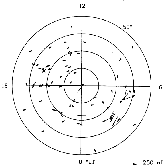
EQUIVALENT CURRENT
