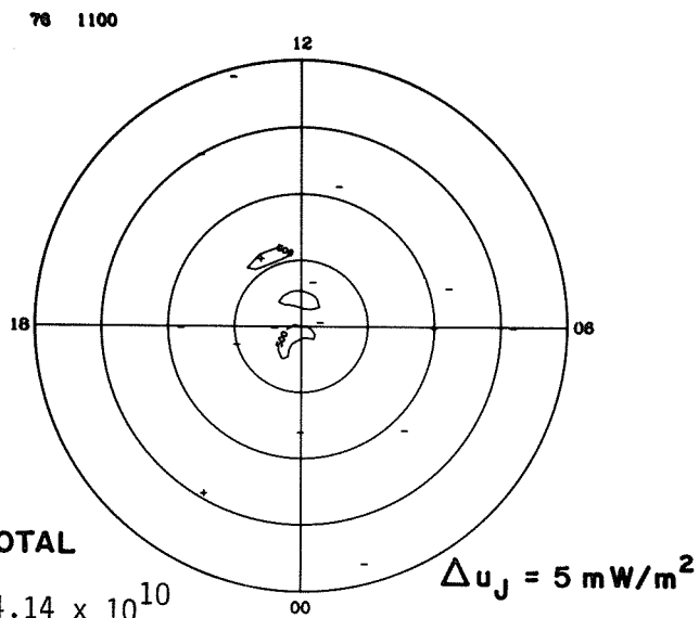
JOULE HEATING
