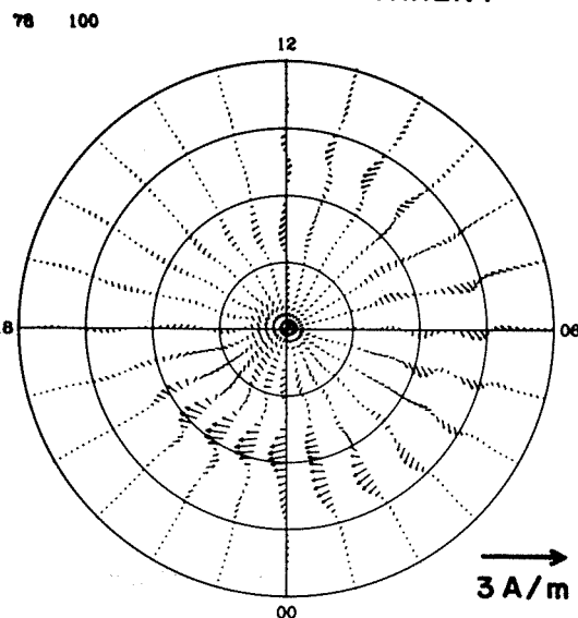
IONOSPHERIC CURRENT
