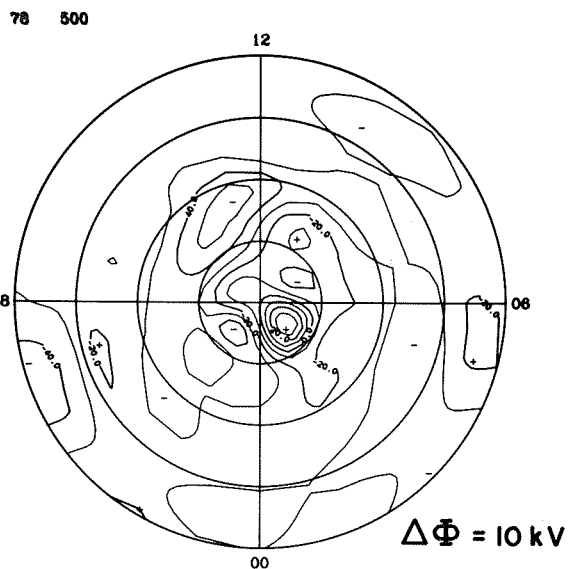
ELECTRIC POTENTIAL
