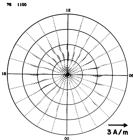
IONOSPHERIC CURRENT
