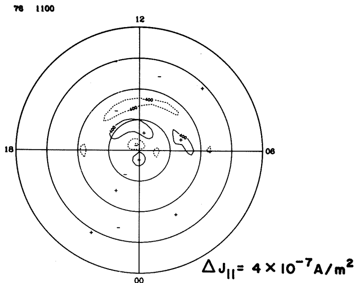
FIELD-ALIGNED CURRENT
