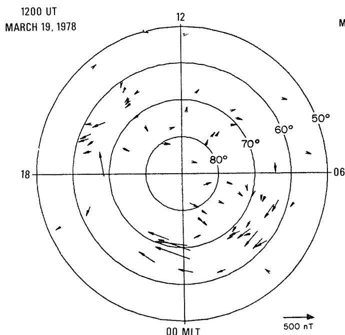
Fig. 4a Examples of the outputs from the calculation. Equivalent current vectors deduced from observed magnetic perturbations.
