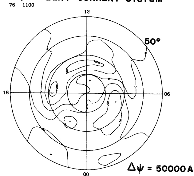
EQUIVALENT CURRENT SYSTEM
