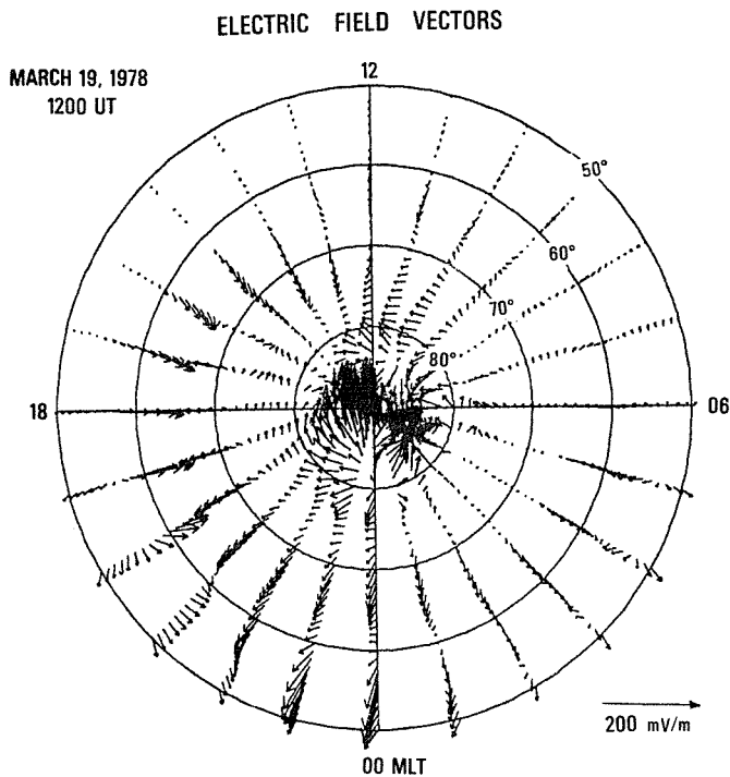
Fig. 4f Electric field vectors.
