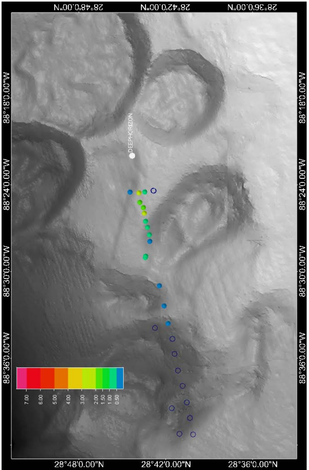
Figure E38: Mean Fluorescence ppb (QSDE) between 1000 and 1300 m on 28 May 2010
