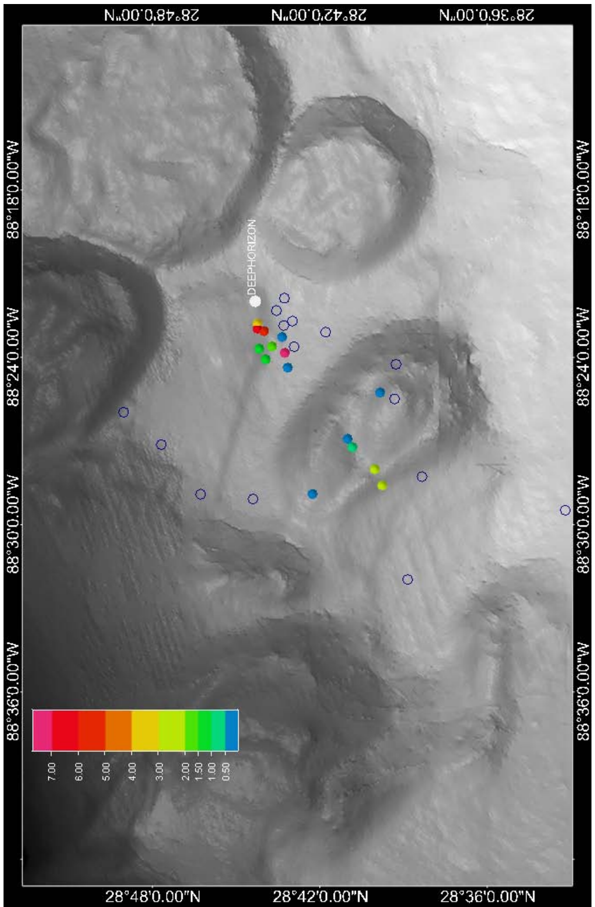
Figure E43: Mean Fluorescence ppb (QSDE) between 1000 and 1300 m on 02 June 2010
