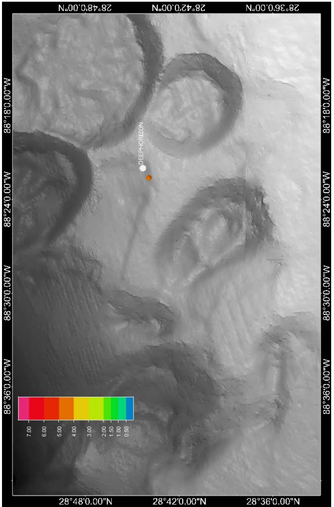
Figure 16: Mean Fluorescence ppb (QSDE) between 1000 and 1300 m on 23 May 2010
