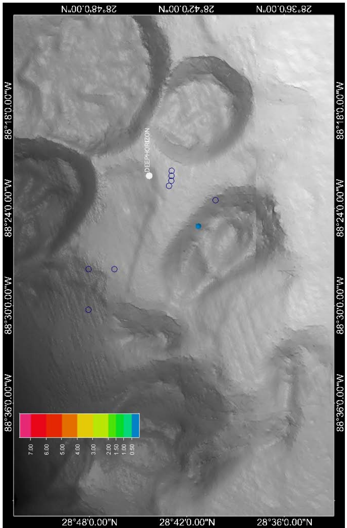
Figure E50: Mean Fluorescence ppb (QSDE) between 1000 and 1300 m on 09 June 2010
