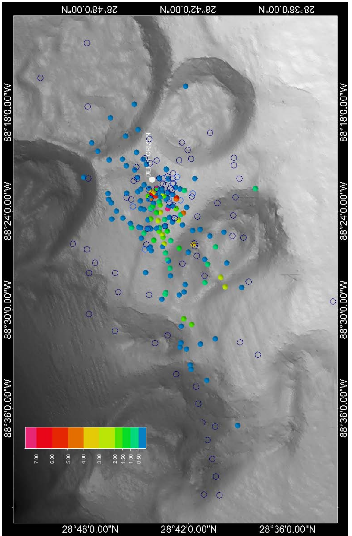
Figure E85: Mean Fluorescence ppb (QSDE) between 1000 and 1300 m from 19 May through 13 July
