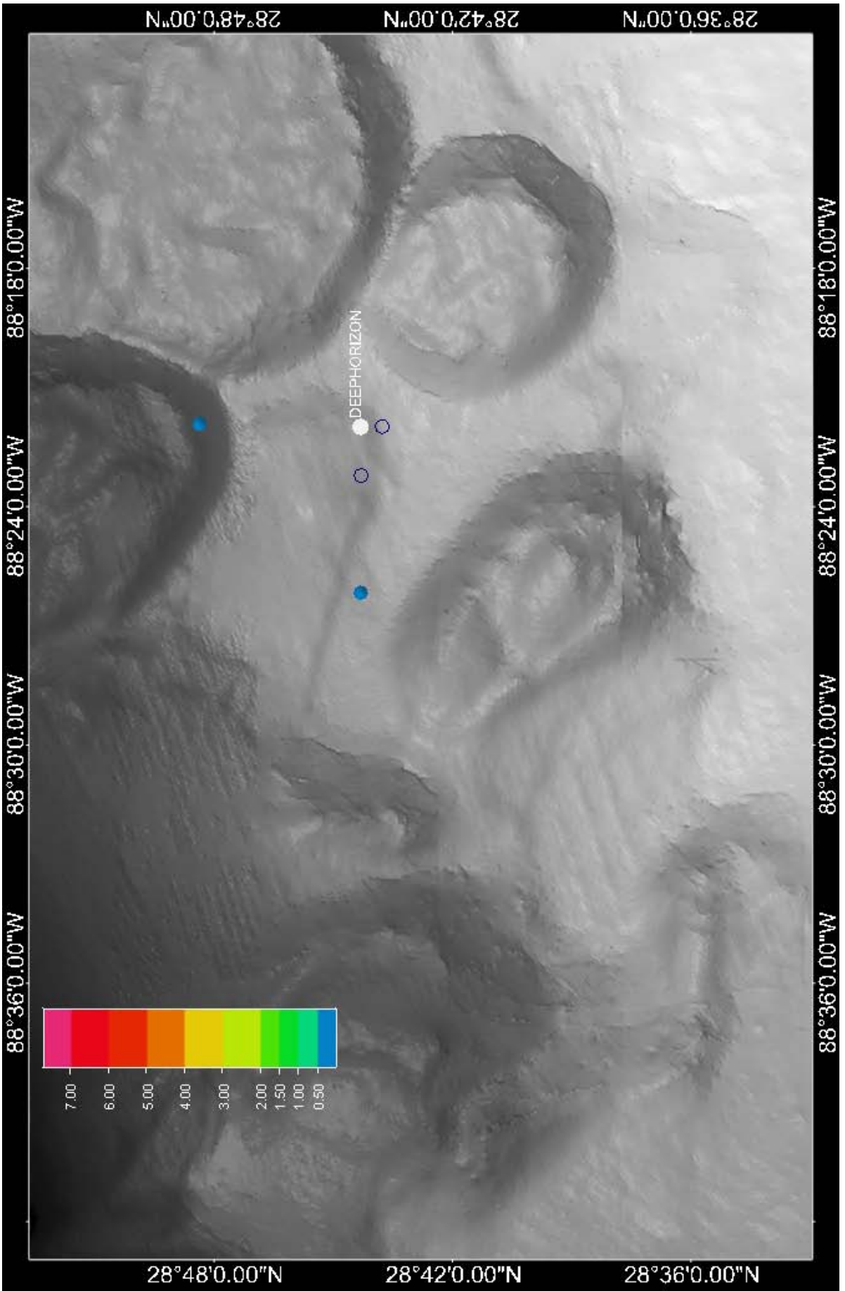
Figure 42: Mean Fluorescence ppb (QSDE) between 1000 and 1300 m on 18 June 2010
