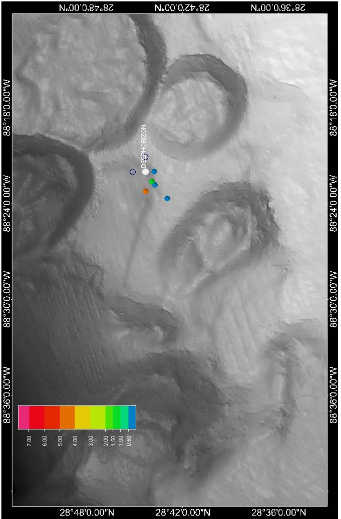
Figure E31: Mean Fluorescence ppb (QSDE) between 1000 and 1300 m on 21 May 2010
