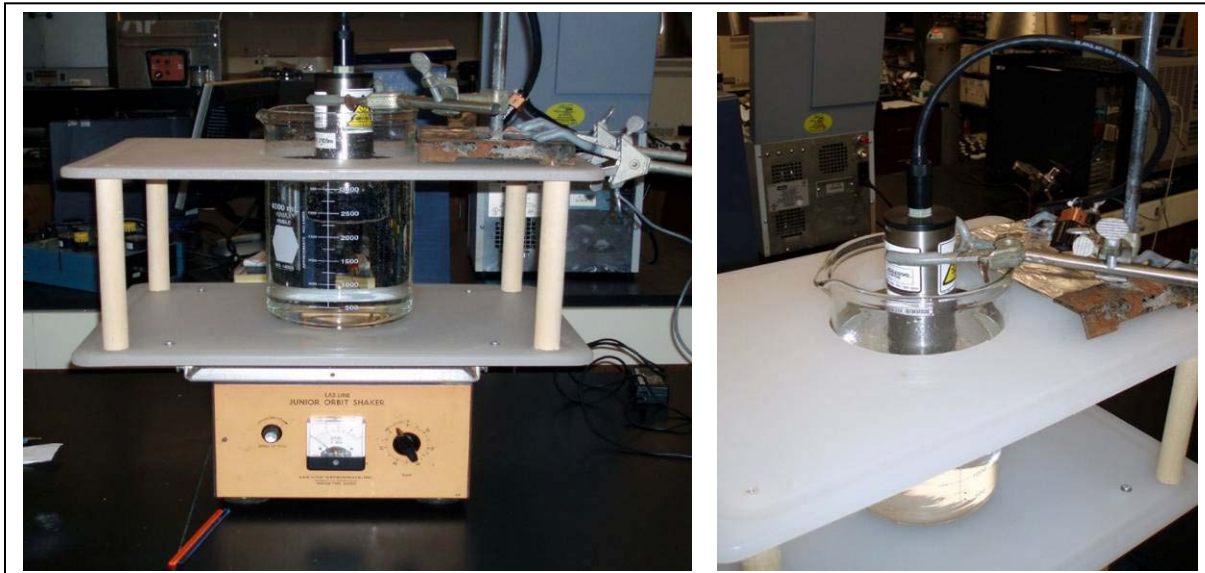
Figure 1. ECO CDOM fluorometer setup for calibration testing.
