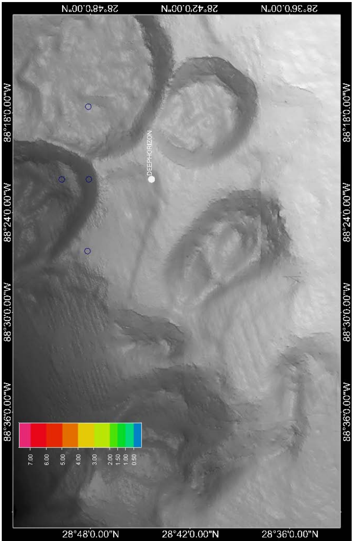
Figure 43: Mean Fluorescence ppb (QSDE) between 1000 and 1300 m on 19 June 2010
