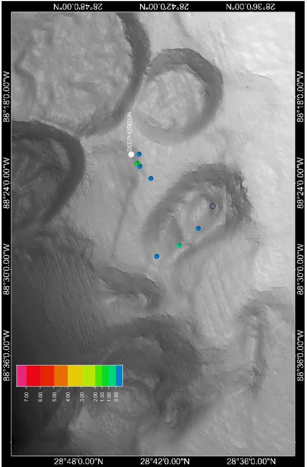
Figure 13: Mean Fluorescence ppb (QSDE) between 1000 and 1300 m on 20 May 2010
