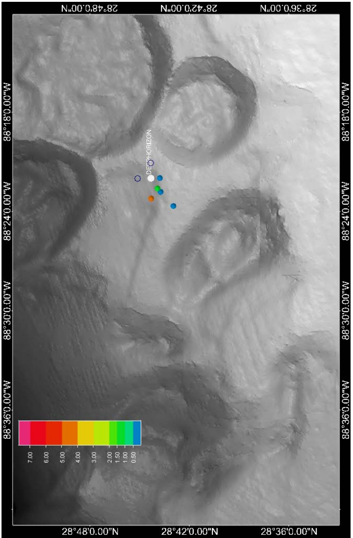
Figure 14: Mean Fluorescence ppb (QSDE) between 1000 and 1300 m on 21 May 2010
