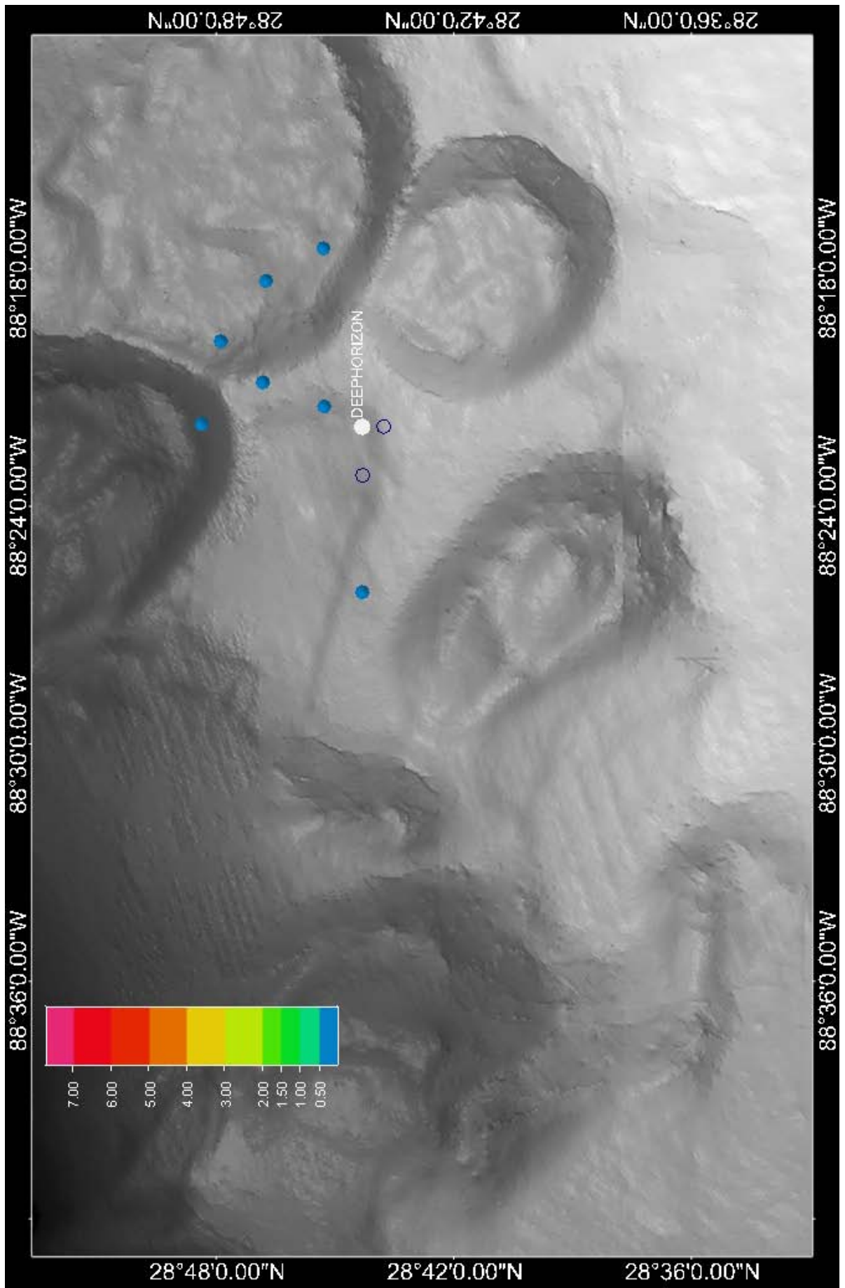
Figure 41: Mean Fluorescence ppb (QSDE) between 1000 and 1300 m on 17 June 2010
