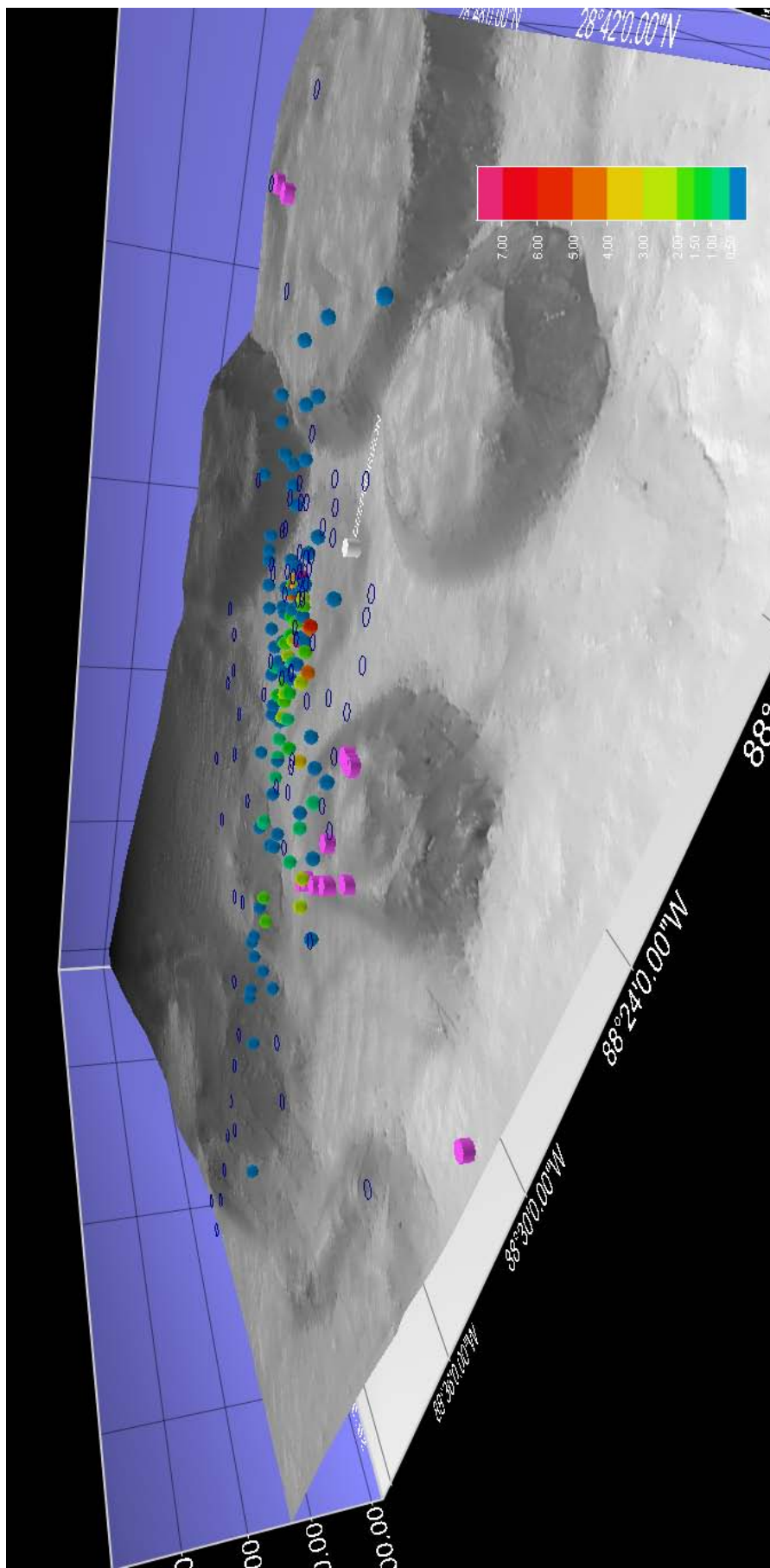
Figure 46: Mean Fluorescence ppb (QSDE) between 1000 and 1300 m from 19 May through 19 June
