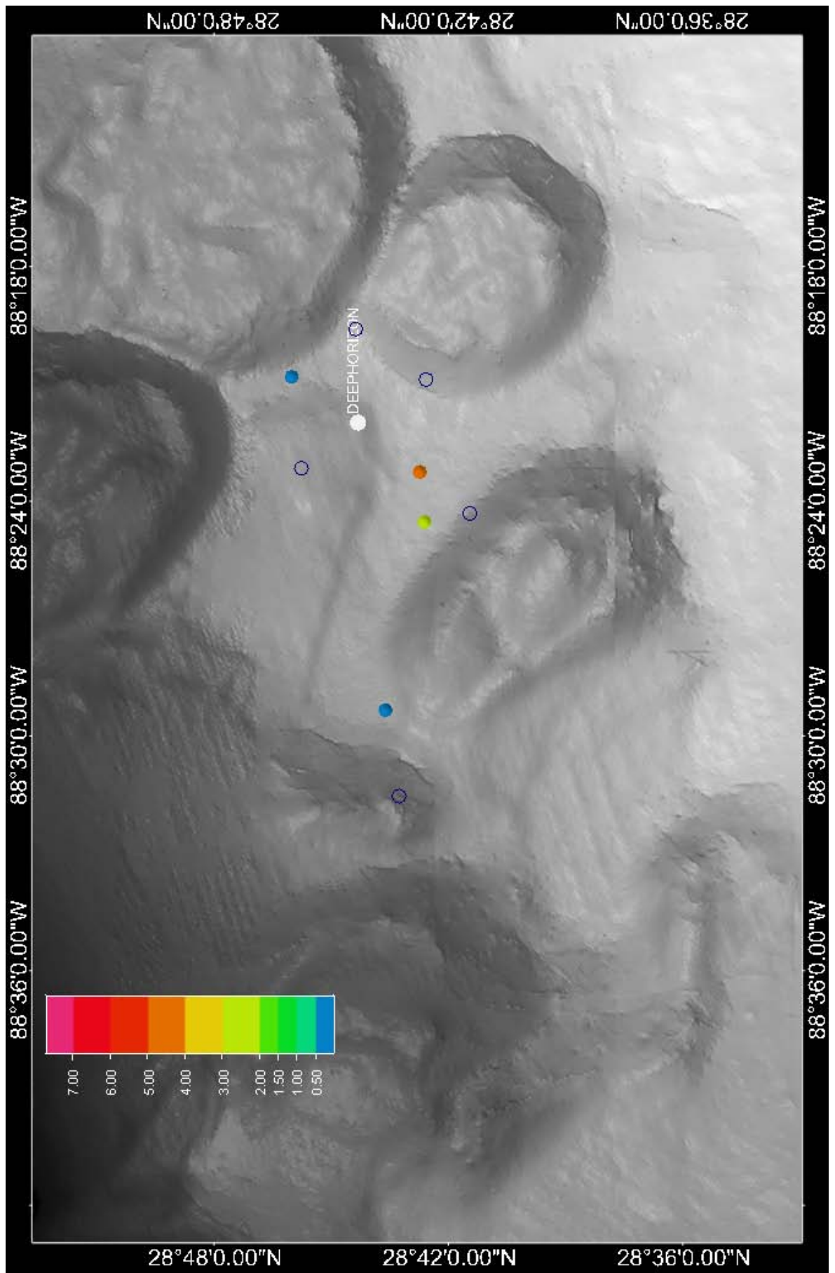
Figure E40: Mean Fluorescence ppb (QSDE), between 1000 and 1300 m on 30 May 2010
