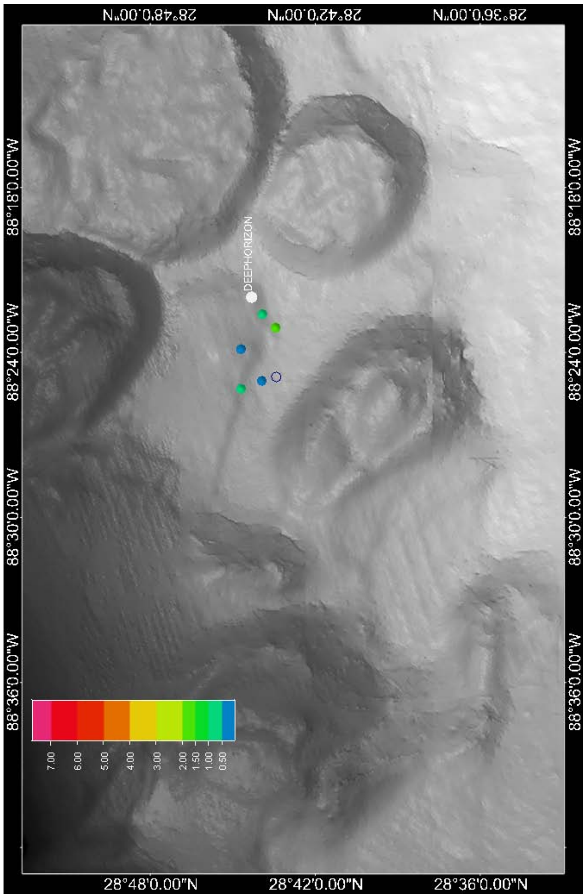
Figure E52: Mean Fluorescence ppb (QSDE) between 1000 and 1300 m on 11 June 2010
