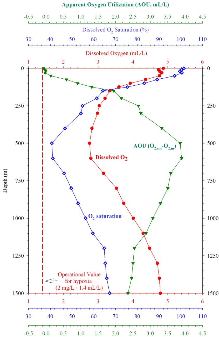
Spring (April-June) climatological average values for dissolved oxygen, percent oxygen saturation, and Apparent Utilization as a function of depth. Values based on the 1-degree horizontal resolution NODC World Ocean Atlas 2009 near 28.5°N and 88.5°W.
