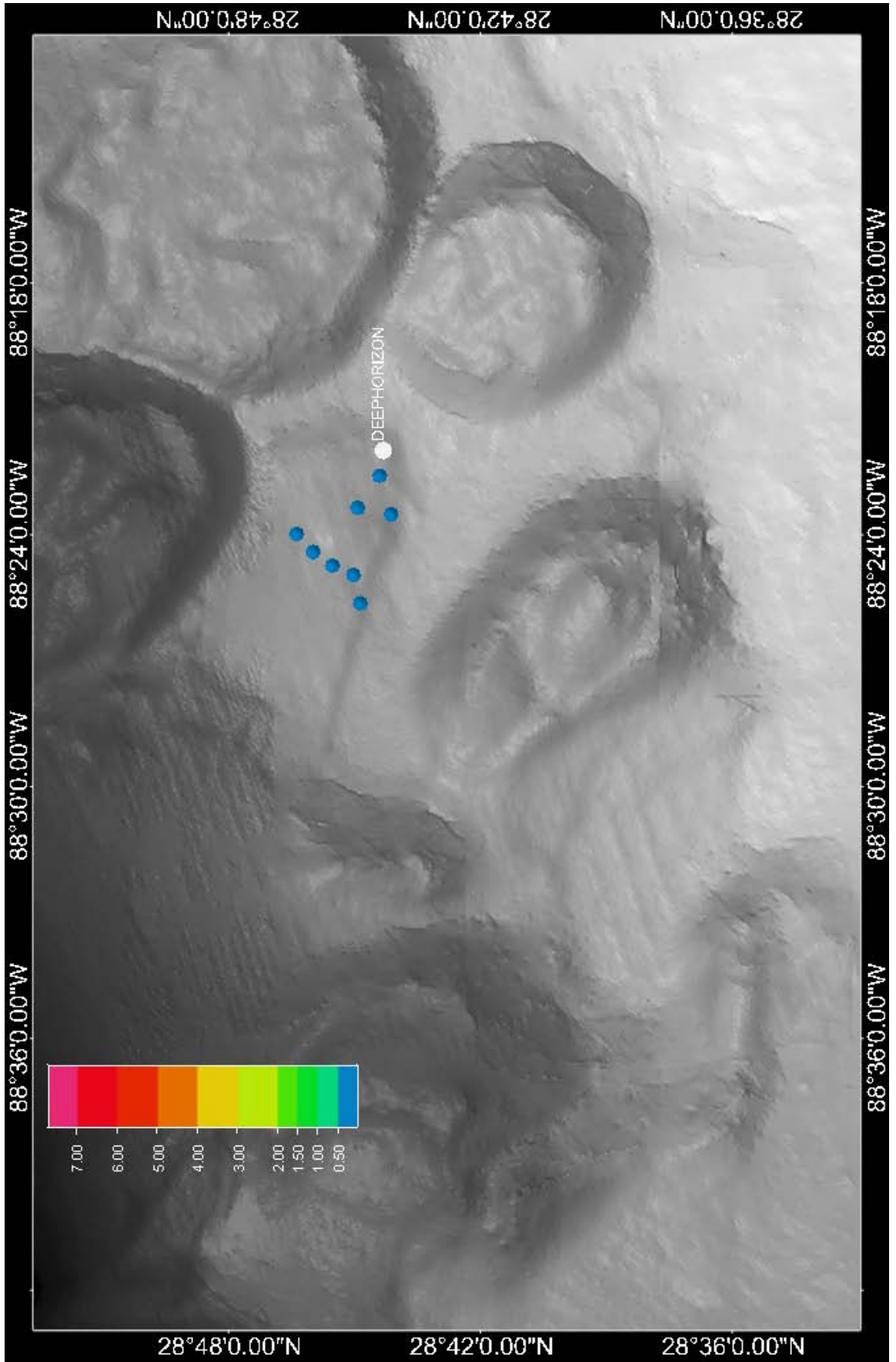
Figure E54: Mean Fluorescence ppb (QSDE) between 1000 and 1300 m on 13 June 2010
