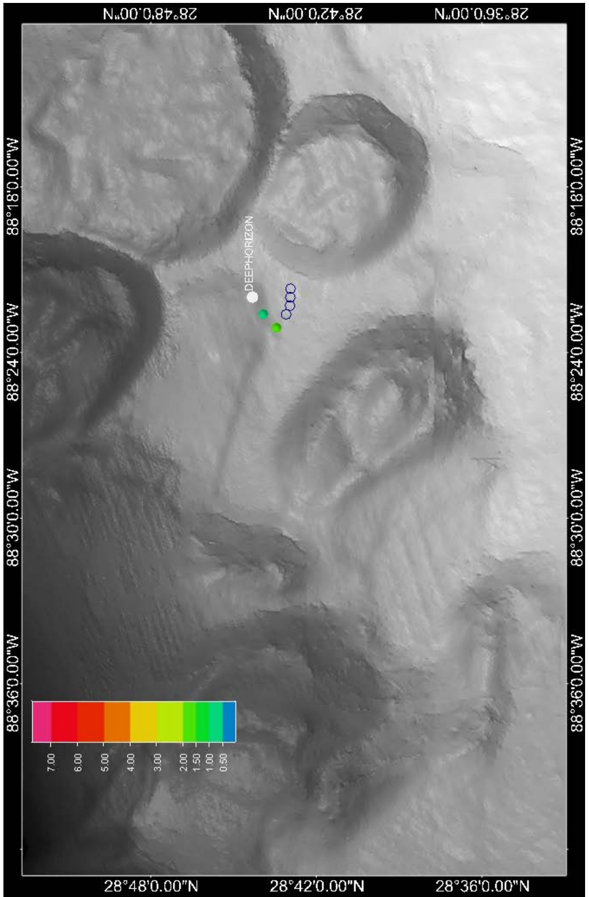
Figure 34: Mean Fluorescence ppb (QSDE) between 1000 and 1300 m on 10 June 2010
