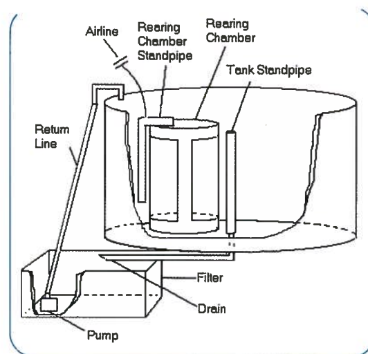
Fig. 4. Recirculating larval rearing system
