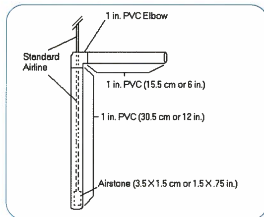
Fig. 6. Stand pipe used in the hatching and rearing chamber
