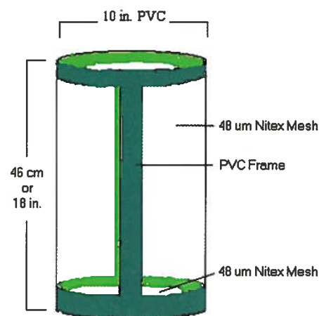
Fig. 5. Rearing chamber
