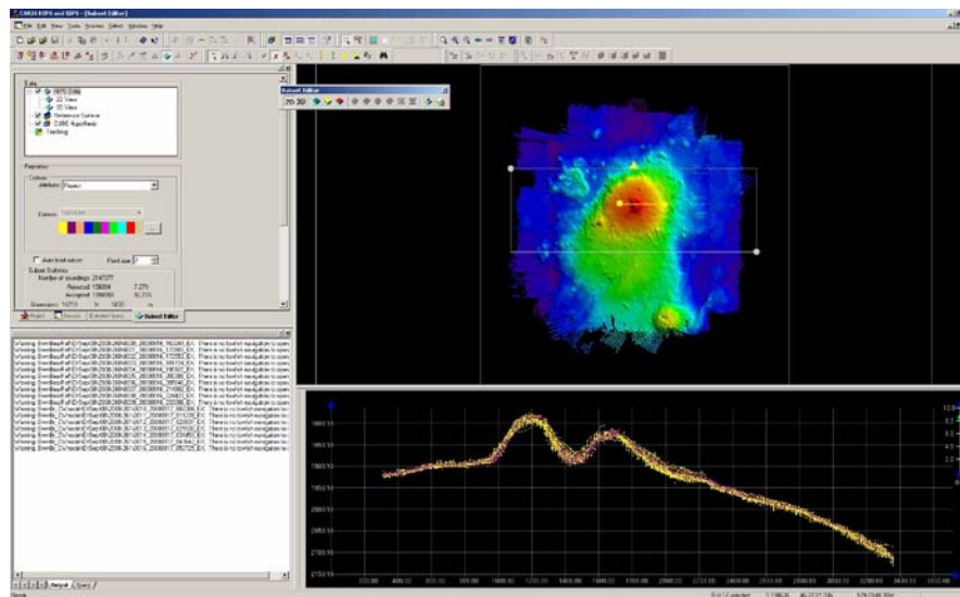
Figure 16. Screen grab taken in CARIS showing EX data collected in FM and CW modes to be in agreement to <0.01% water depth.
