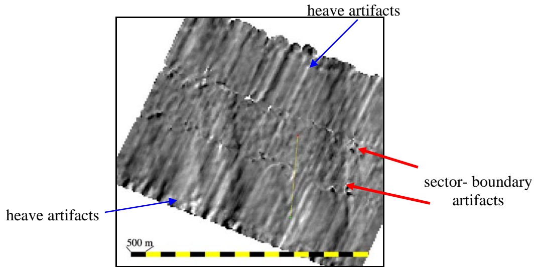
Figure 7. Transit test line 43 showing heave. Water depth 4400 m.
