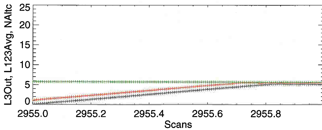
Figure 8: L3Out , L123Avg , NAlt (in meters) for flight 1, second flux leg (scan 2955). Black line is the corrected laser 3 data; red is the three laser signals averaged together; green is the offset GPS signal.
